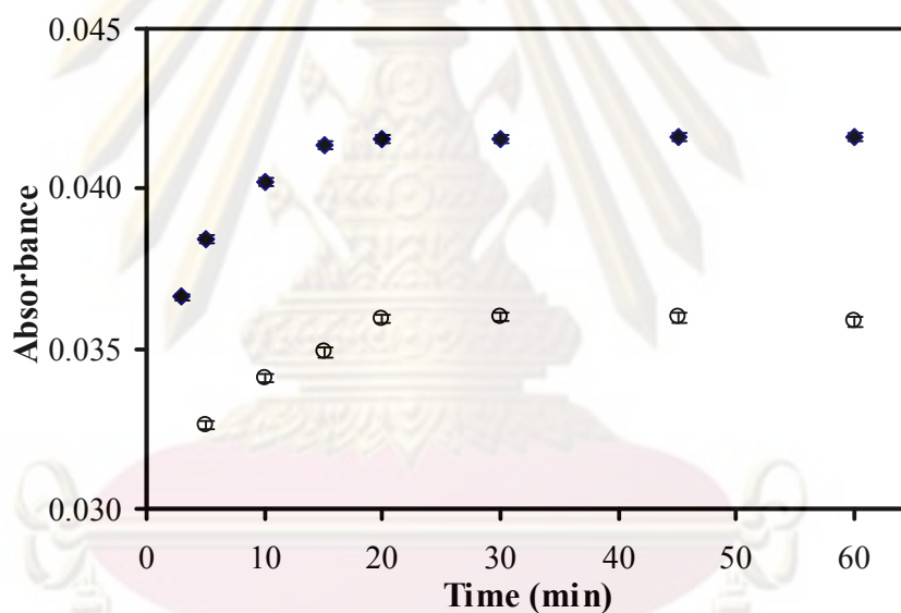
Figure 4.4 Response time of optode membrane in the presence of ○ 1.00 \times 10^{-5} and ◆ 3.16 \times 10^{-5} \text{ mol L}^{-1} of \text{Pb}^{2+} .
