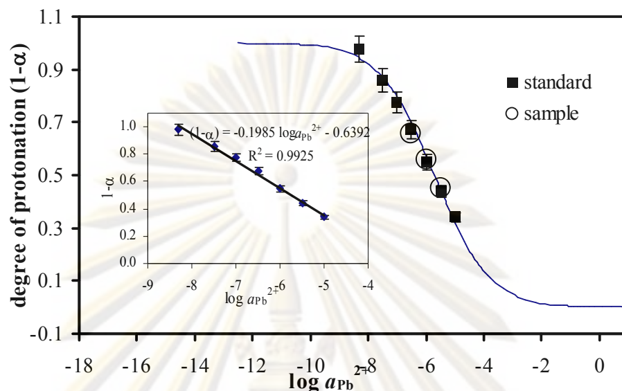
Figure 4.21 The response curve plot of degree of protonation versus log activity of Pb 2+ . The inset figure showed a calibration curve used to determine Pb 2+ in tap water sample in flow-through system.
