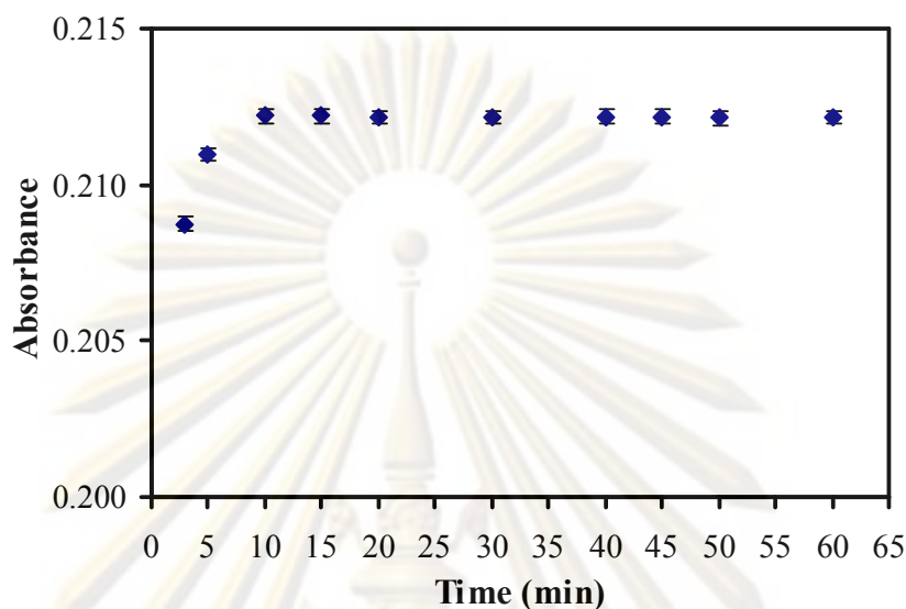
Figure 4.15 Response time of the optode membrane in Tis buffer solution (pH 7.0) containing 3.16 \times 10^{-6} \text{ mol L}^{-1} \text{ Pb}^{2+} at a flow rate of 1.6 \text{ mL min}^{-1} .
