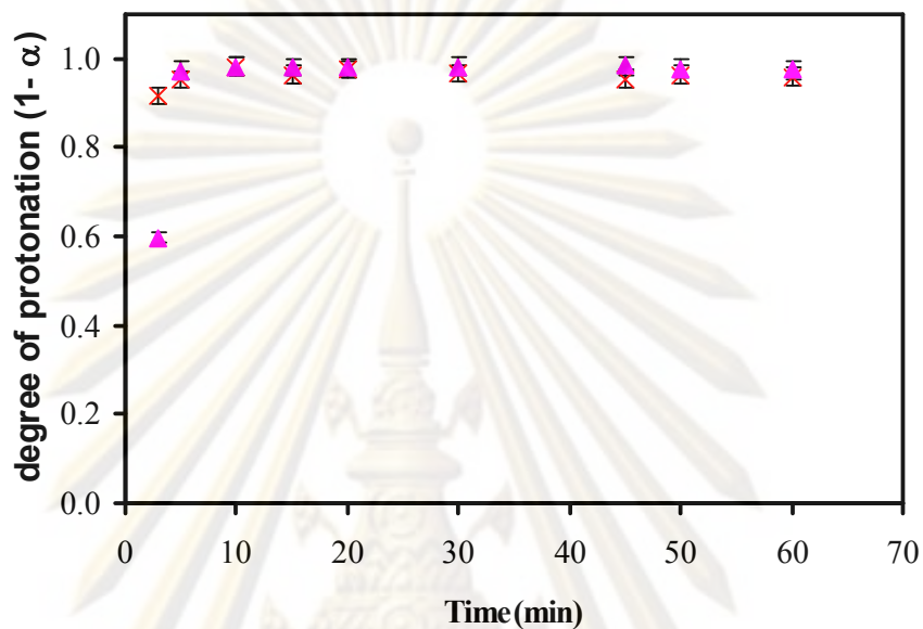
Figure 4.5 The response of optode membrane at 660 nm as a function of time in different conditioning solutions; \blacktriangle 1.00 \times 10^{-3} mol L -1 Tris buffer, \times 0.01 mol L -1 HCl.
