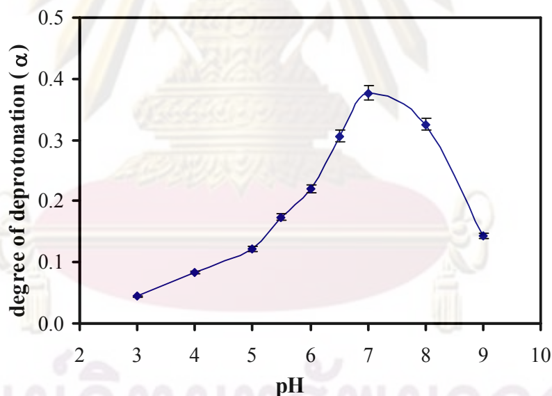
Figure 4.1 The effect of pH on the response of optode membrane at 660 nm in the presence of 3.16 \times 10^{-6} mol L -1 of Pb 2+ .
