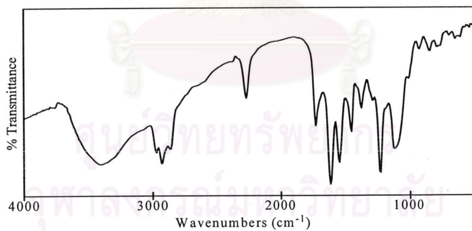
Figure A.8 IR spectrum of Ni-PP-X (with catalyst) before heating
