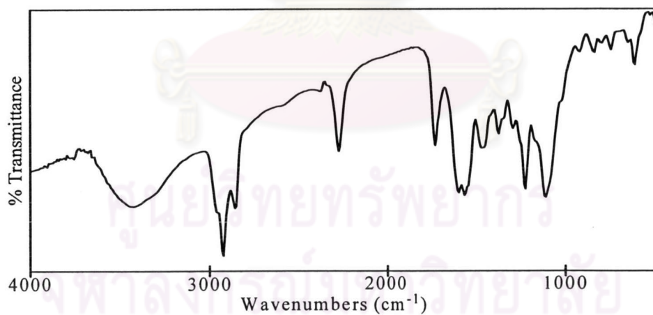
Figure A.2 IR spectrum of Mn-PP (with catalyst) before heating
