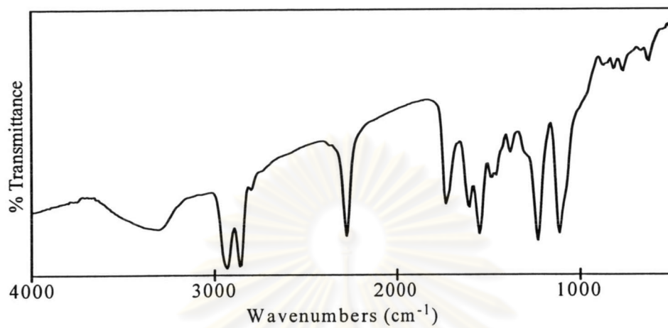
Figure A.5 IR spectrum of Mn-PB-X (with catalyst) before heating
