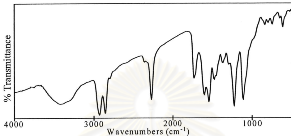
Figure A.1 IR spectrum of Mn-PB (with catalyst) before heating
