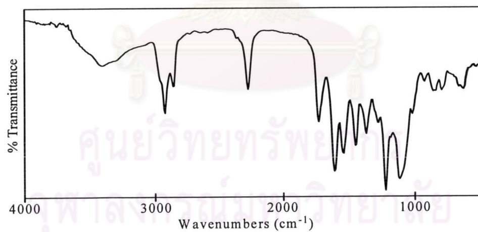
Figure A.4 IR spectrum of Ni-PP (with catalyst) before heating
