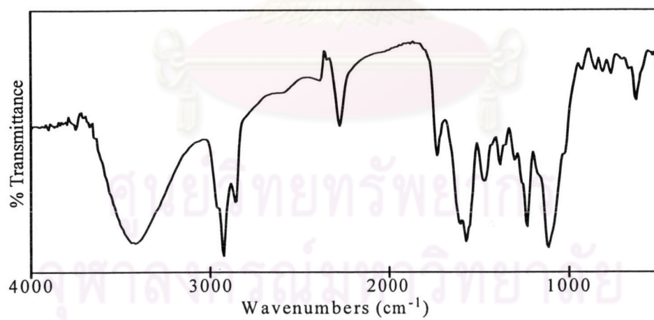
Figure A.6 IR spectrum of Mn-PP-X (with catalyst) before heating
