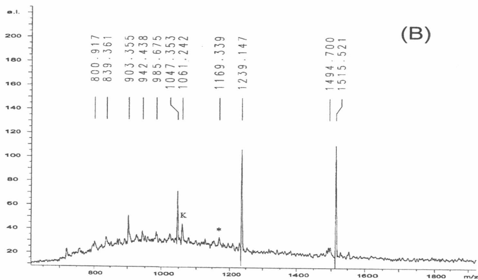
Figure 3.3 Tryptic Fragments Mass Spectra from 7 Protein Spots: (A) Spot No. 1; (B) Spot No. 2; (C) Spot No. 3; (D) Spot No. 4; (E) Spot No. 5; (F) Spot No. 6. Peaks marked with K letter and asterisks are keratin contamination and tryptic autolysis products.
