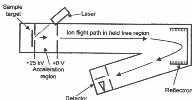
Figure 1.6 Reflectron Time of Flight Mass Spectrometer.
