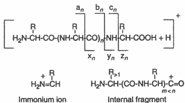
Figure 1.13 Imonium Ion and Internal Fragment.
