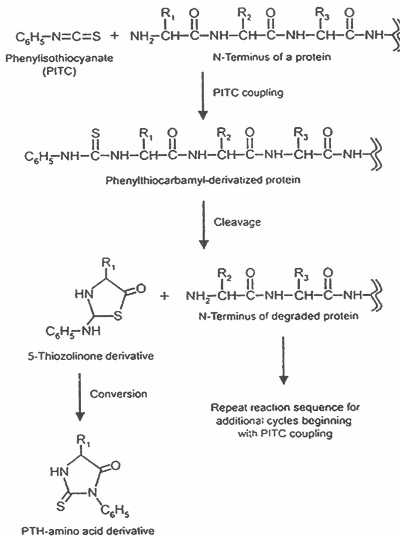
Figure 1.14 The Edman Reaction.
