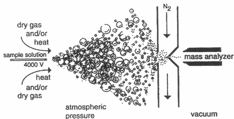
Figure 1.7 The Electrospray Ionization Source
