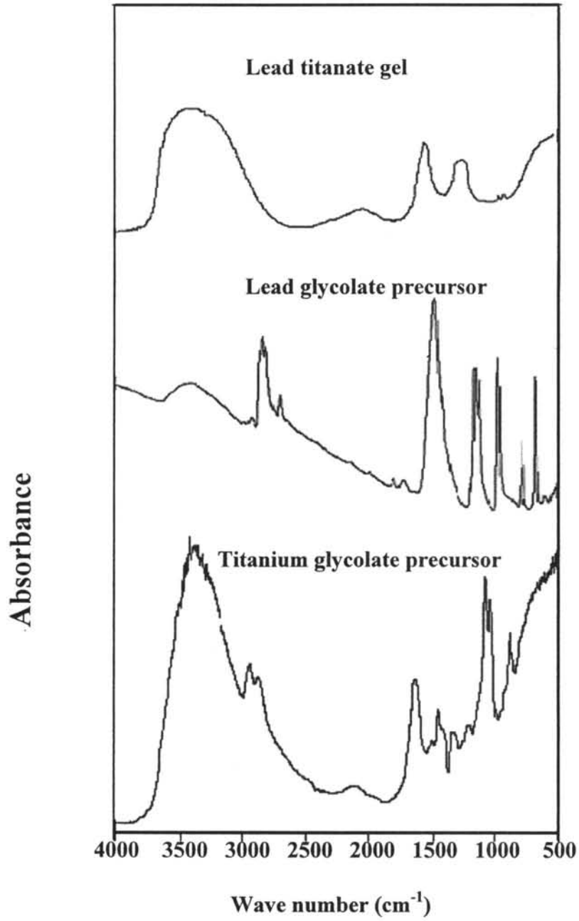
Figure 5.1 FTIR spectra of lead glycolate, titanium glycolate and dried lead titanate gel.
