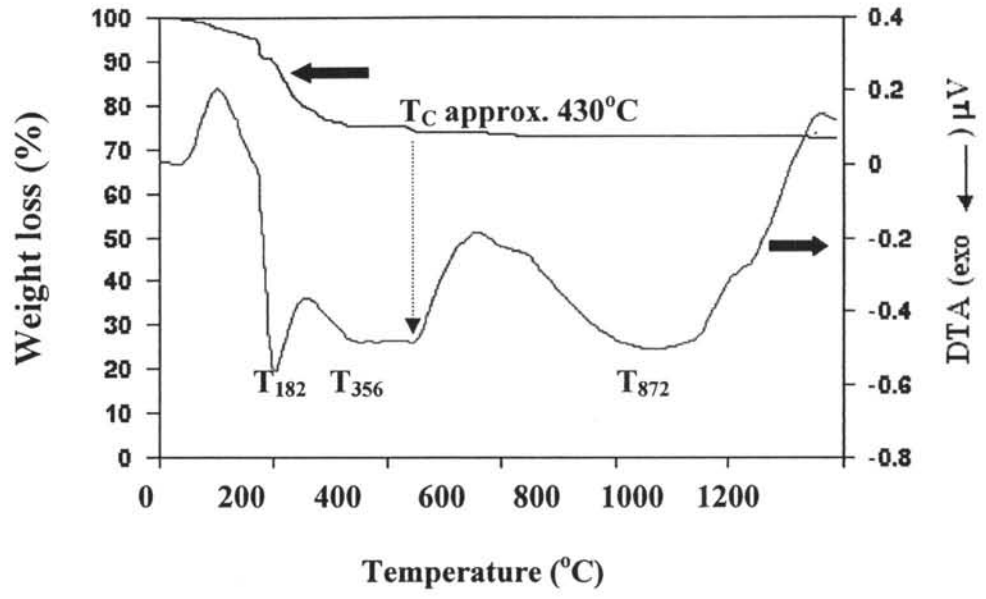
Figure 5.3 DTA and TGA thermograms of dried lead titanate gel.
