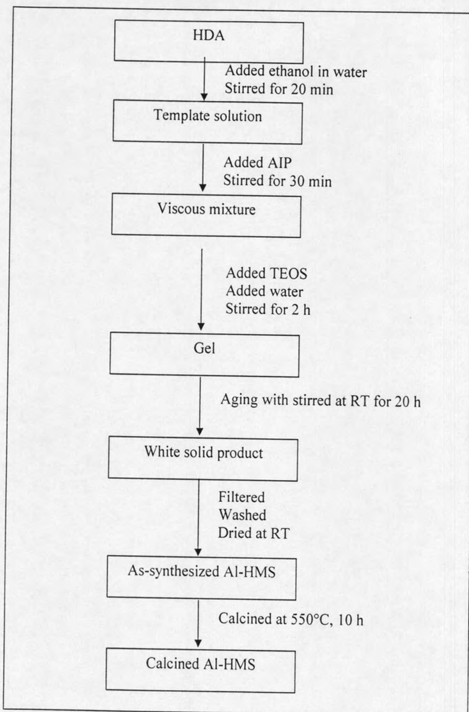
Scheme 3.4 Diagram of Al-HMS synthesis.
