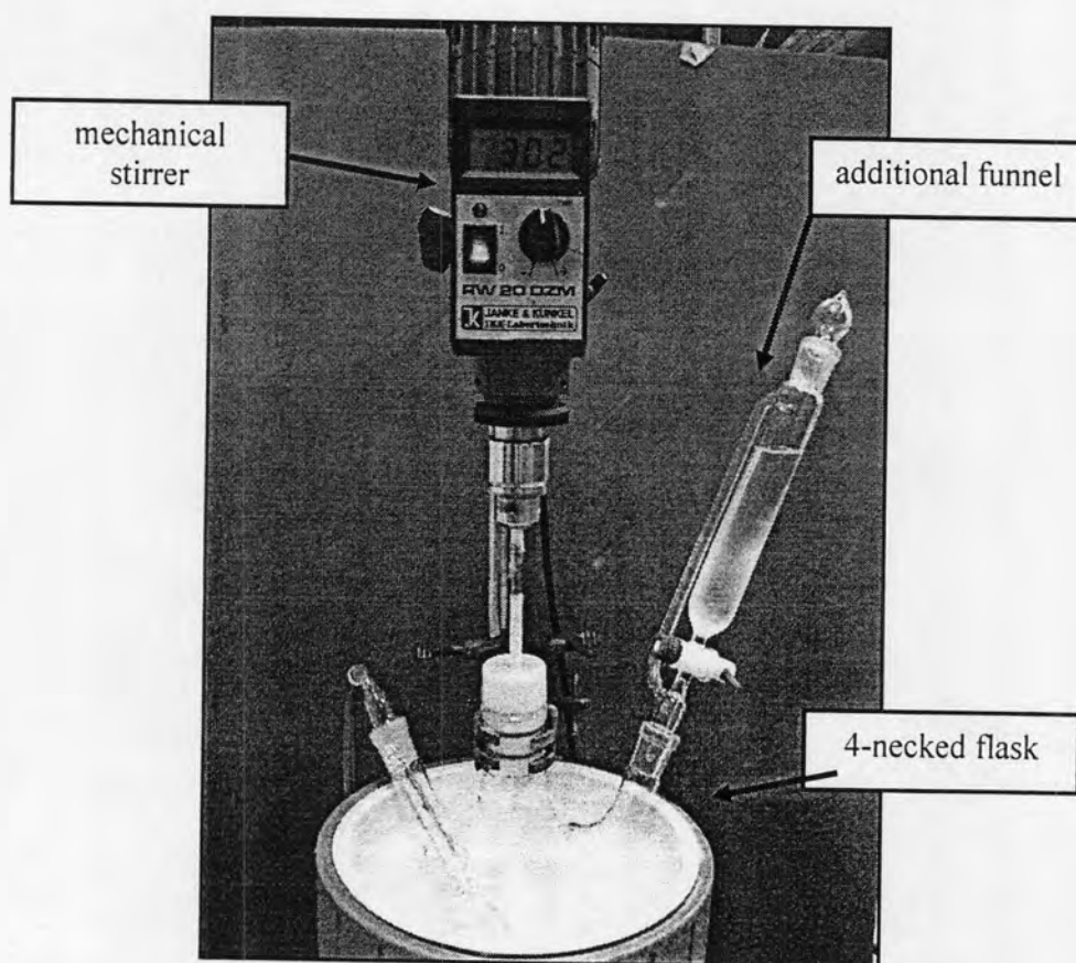
Figure 3.2 Zeolite beta synthesis apparatus.
