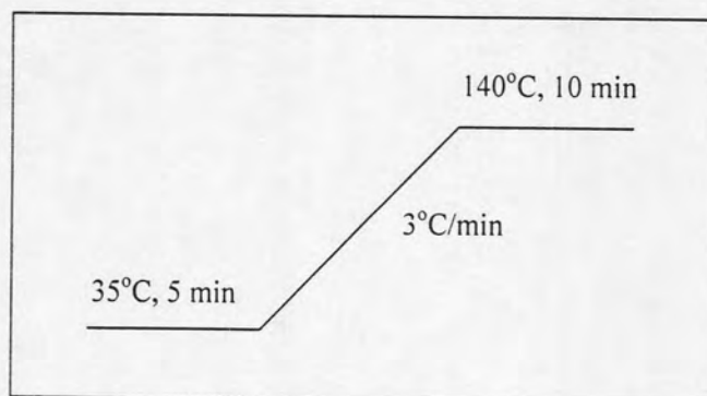
Scheme 3.1 The column heating program for gas analysis.
