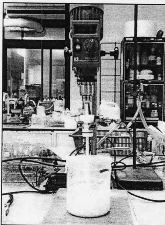
Figure 3.3 Al-HMS synthesis apparatus.
