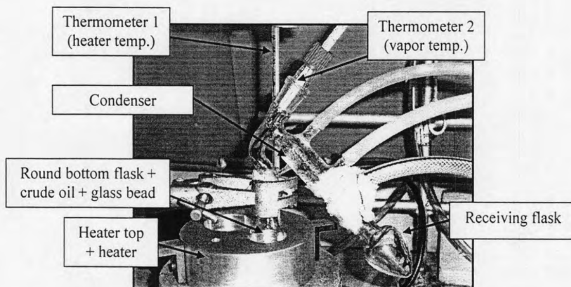
Figure 3.5 Vacuum distillation apparatus.
