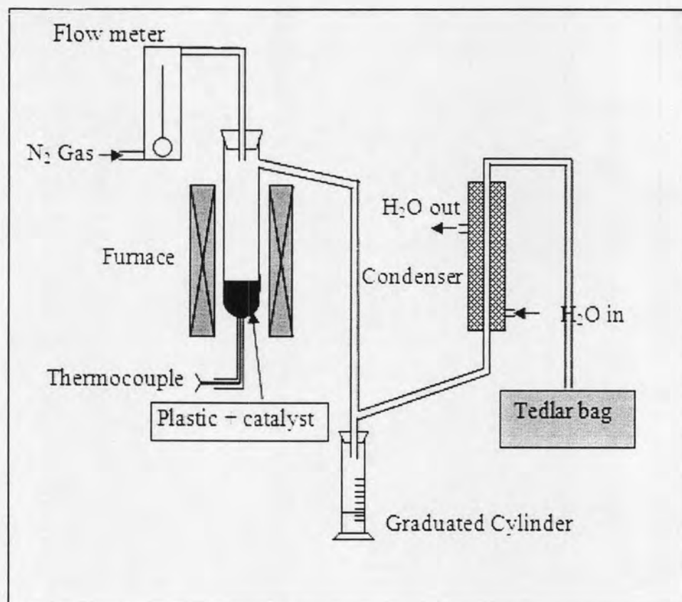
Figure 3.4 Catalytic cracking apparatus.
