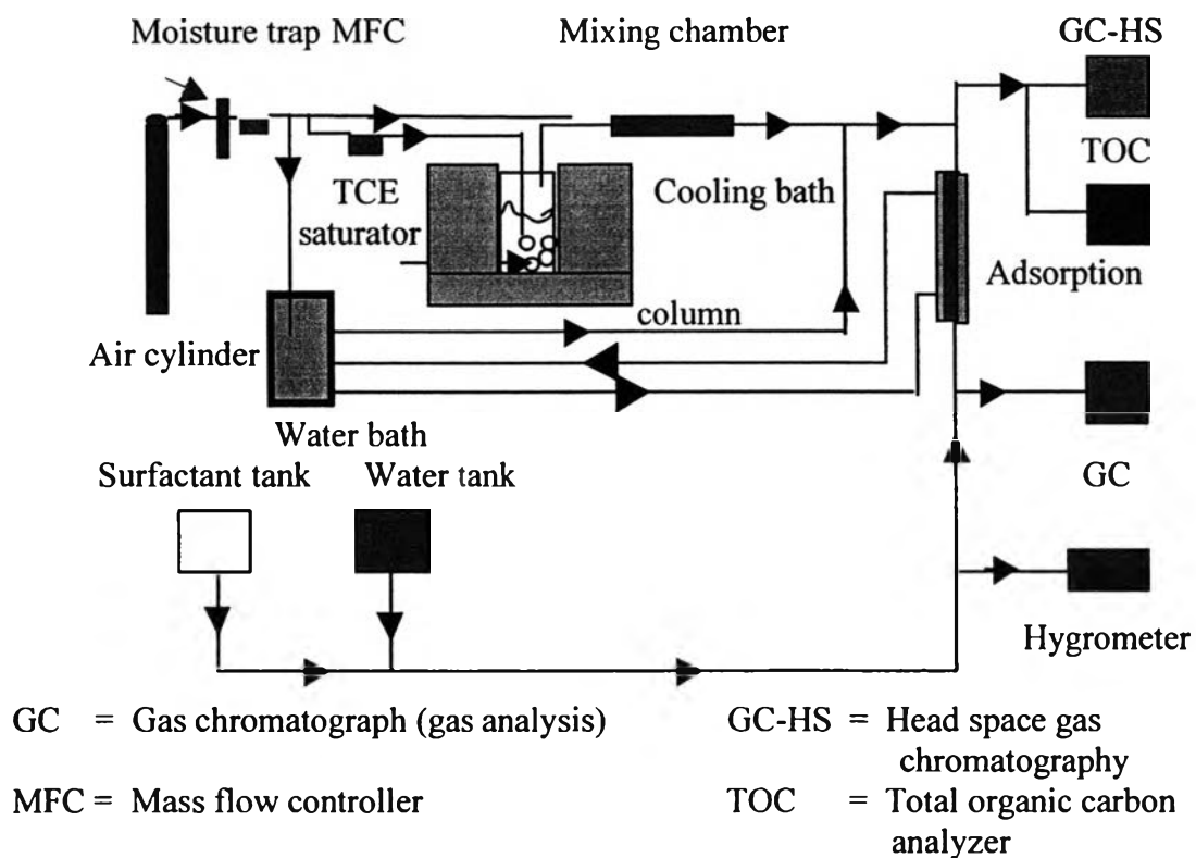
Figure 7.1 Schematic diagram of the experimental apparatus.
