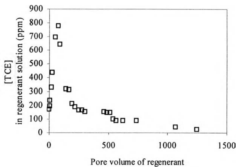
Figure 7.3 TCE concentration in effluent regenerant solution with [SDS] of 0.1 M and flow rate of 5 mL/min.
