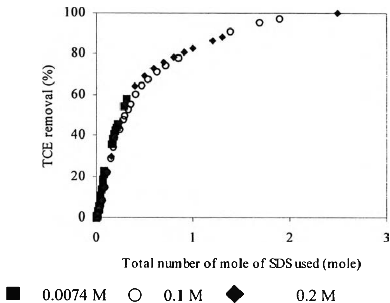
Figure 7.8 Fractional TCE removal during regeneration with [SDS] of 0.074, 0.1 and 0.2 M at a flow rate of 5 mL/min.
