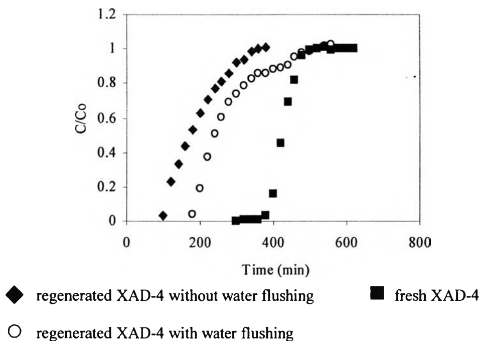
Figure 7.2 a Breakthrough curves for TCE in air with fresh and regenerated resin. (C = Effluent TCE concentration, C_0 = Inlet TCE concentration).
