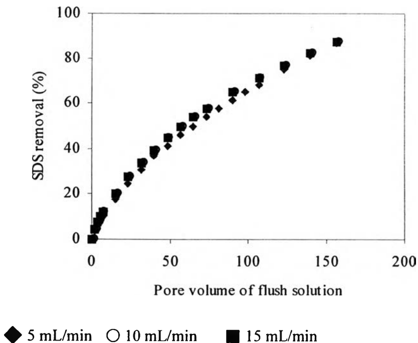
Figure 7.9 Fractional SDS removal during flush with water at several flow rates.
