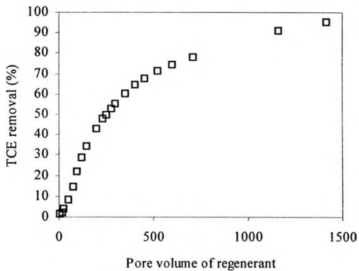
Figure 7.4 Fractional TCE removal during regeneration with [SDS] of 0.1 M and a flow rate of 5 mL/min.
