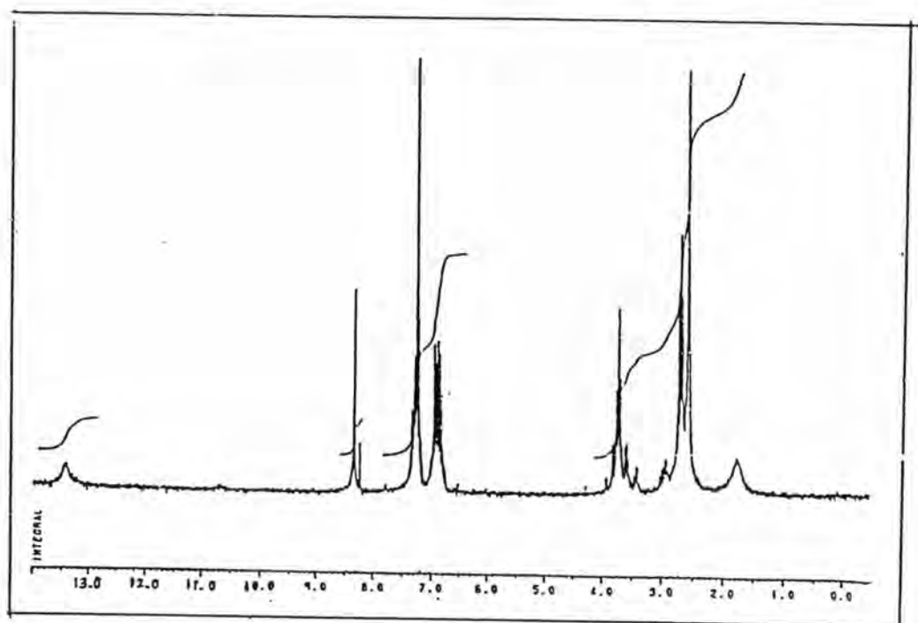
Fig. 8a: 1 H NMR spectrum of Compound 3
