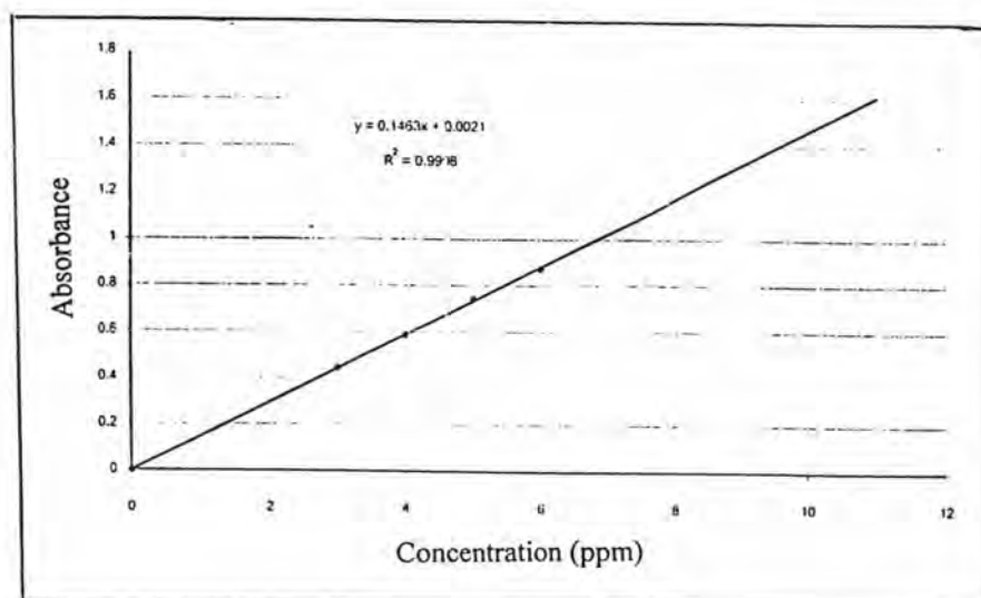
Fig. 21a: Calibration curve of Dye 2
