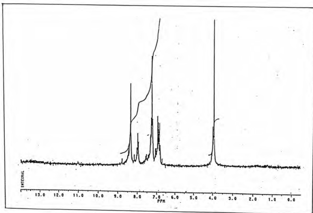
Fig. 11a: 1 H NMR spectrum of Dye 1
