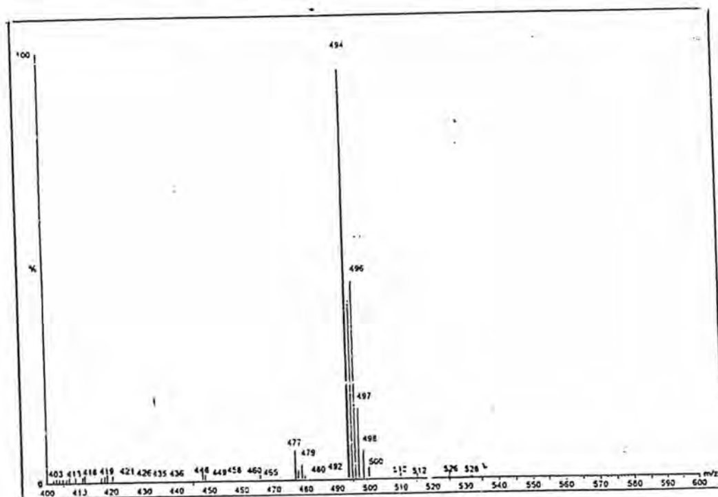
Fig. 49a: Mass spectrum of Dye 7
