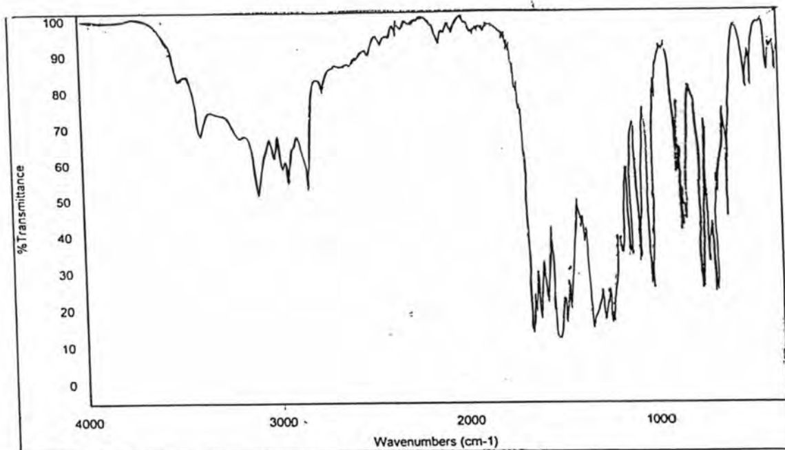
Fig.76a: IR spectrum of Dye 12
