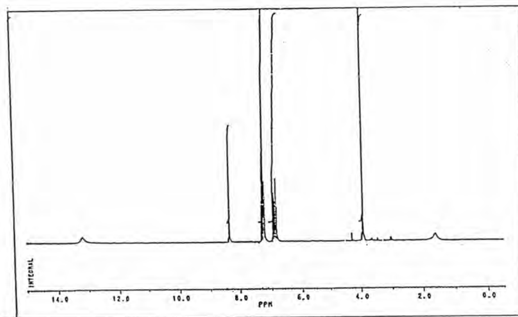
Fig. 2a: 1 H NMR spectrum of Compound 1
