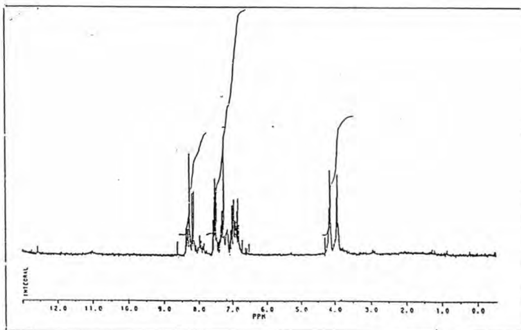
Fig. 35a: 1 H NMR spectrum of Dye 5
