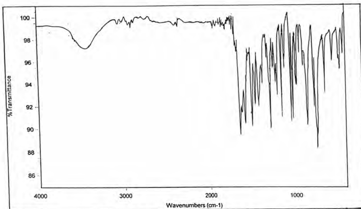
Fig. 1a: IR spectrum of Compound 1
