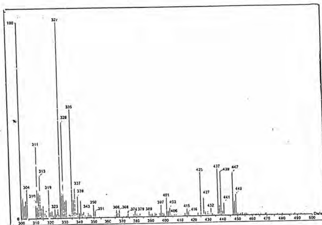
Fig. 31a: Mass spectrum of Dye 4
