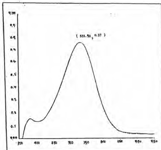
Fig. 14a: UV/VIS spectrum of Dye 1
