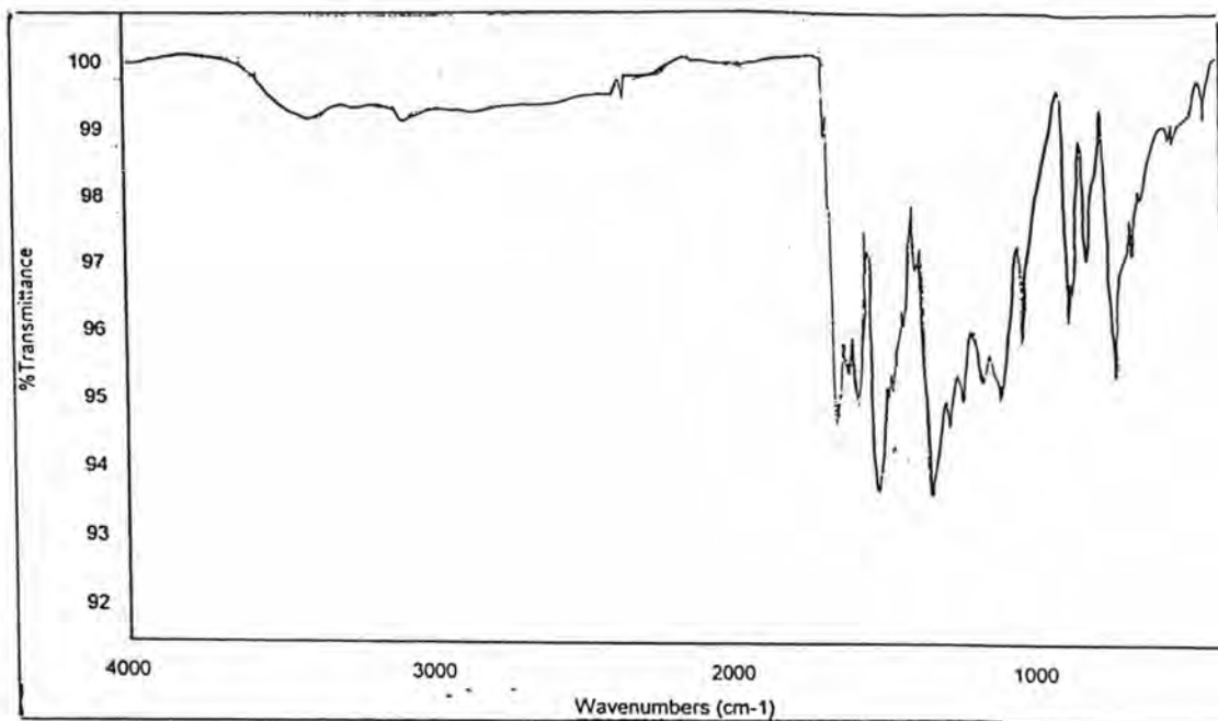
Fig. 64a: IR spectrum of Dye 10
