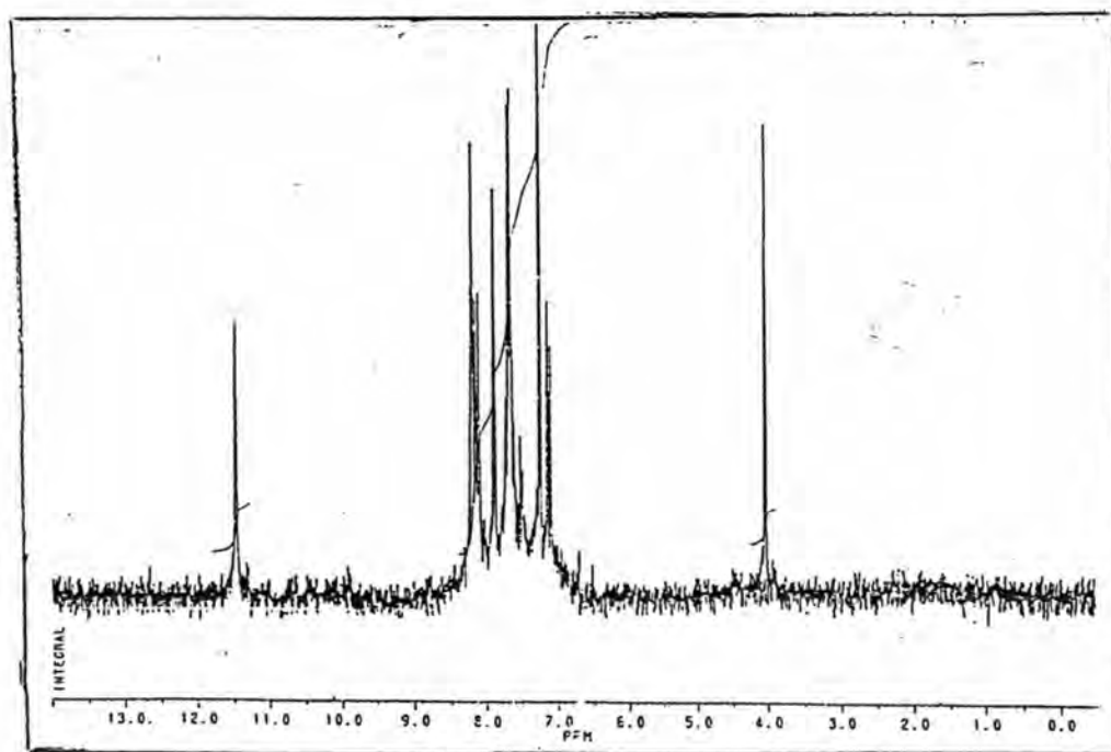
Fig. 23a: 1 H NMR spectrum of Dye 3
