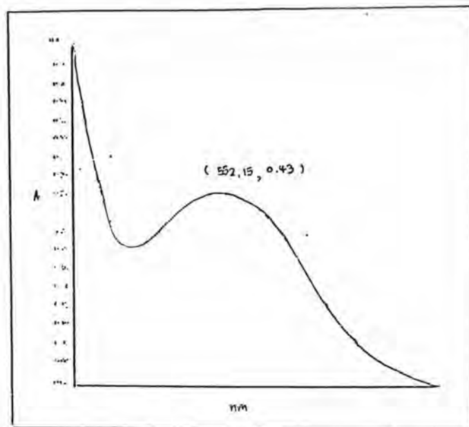
Fig. 56a: UV/VIS spectrum of Dye 8
