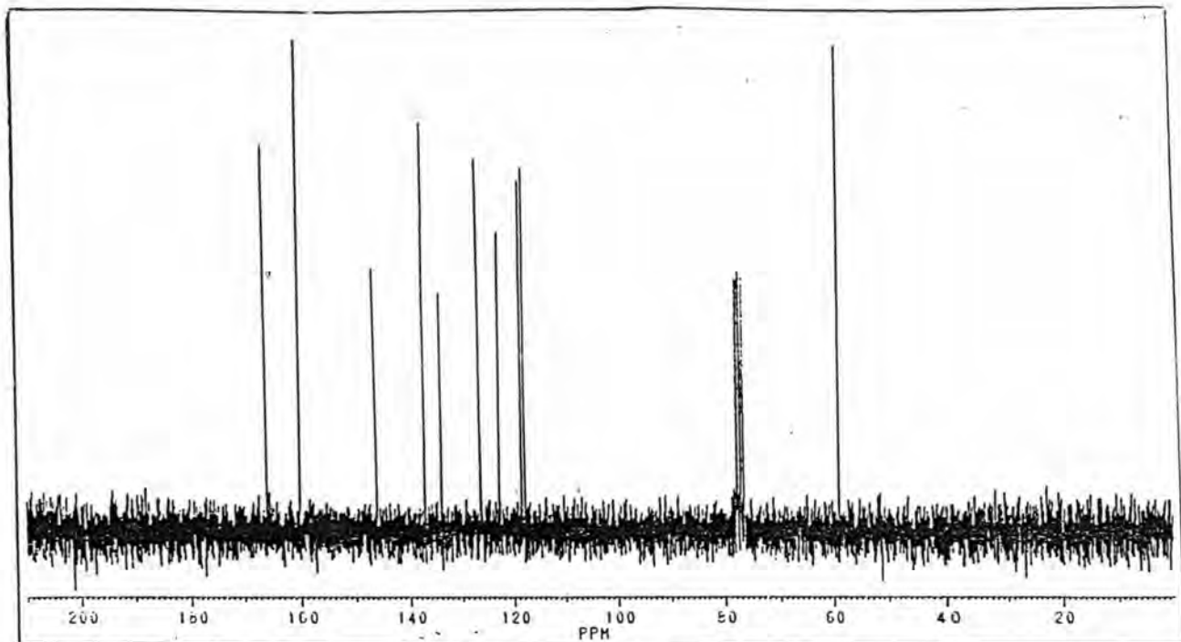
Fig. 18a: ^{13}\text{C} NMR spectrum of Dye 2
