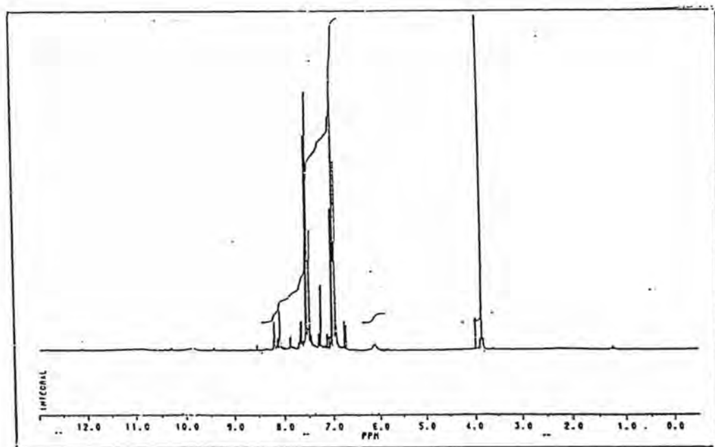
Fig. 71a: 1 H NMR spectrum of Dye 11
