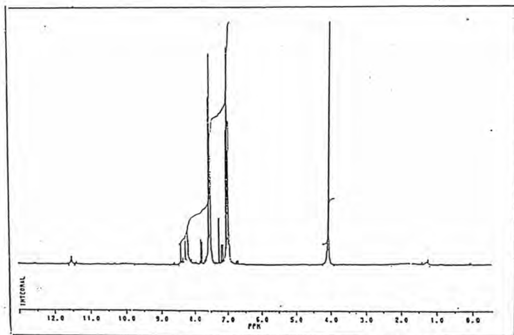
Fig. 65a: 1 H NMR spectrum of Dye 10
