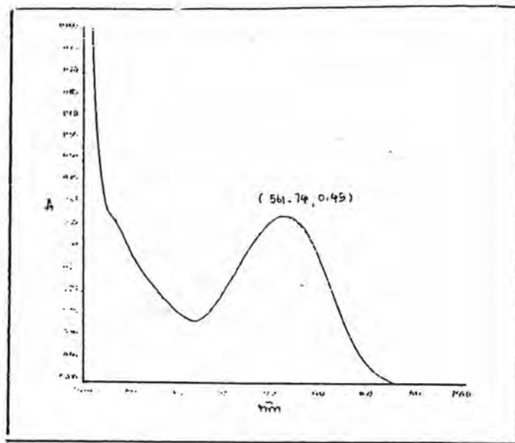
Fig. 80a: UV/VIS spectrum of Dye 12
