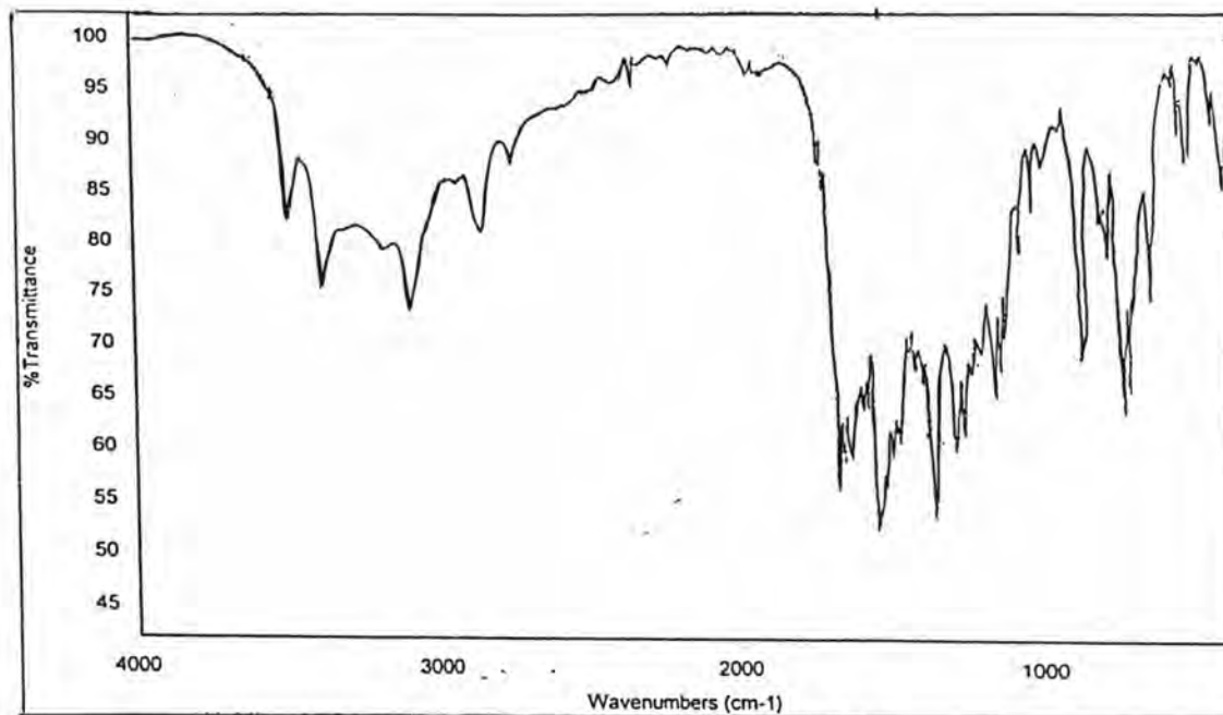
Fig.70a: IR spectrum of Dye 11
