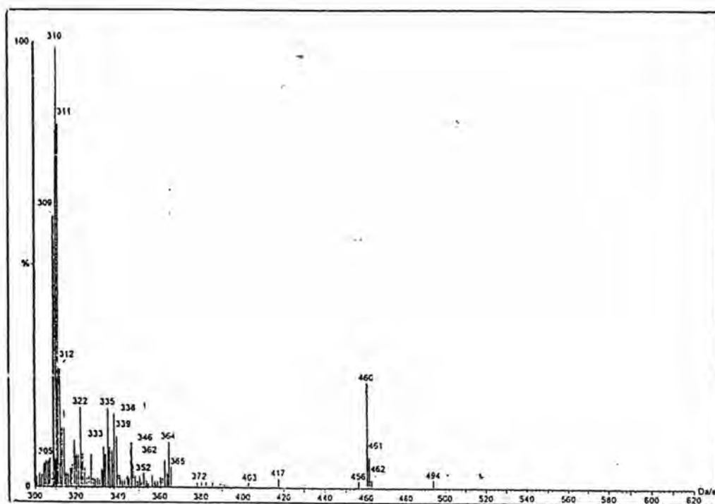
Fig. 37a: Mass spectrum of Dye 5
