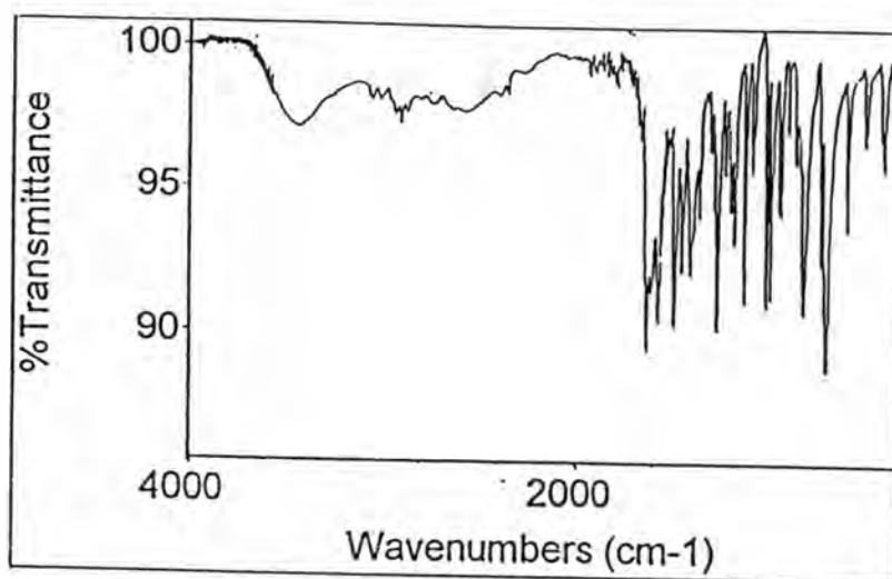
Fig. 7a: IR spectrum of Compound 3
