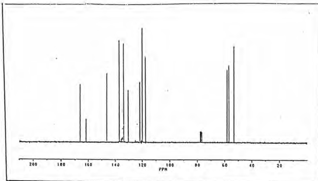
Fig. 72a: ^{13}\text{C} NMR spectrum of Dye 11
