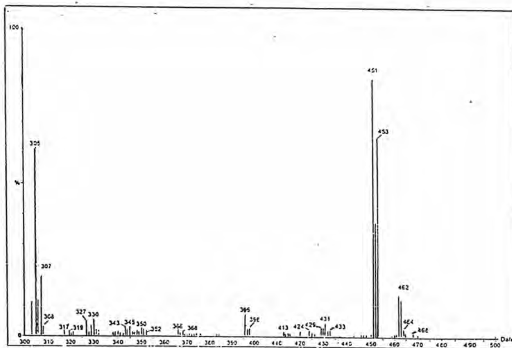
Fig. 19a: Mass spectrum of Dye 2
