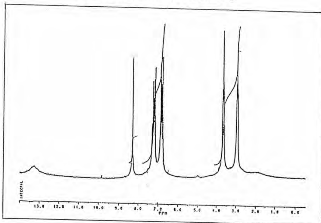
Fig. 5a: 1 H NMR spectrum of Compound 2
