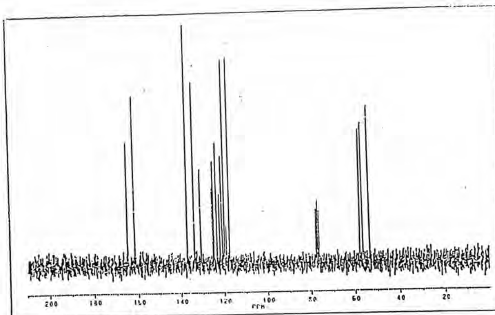
Fig. 60a: ^{13}\text{C} NMR spectrum of Dye 2
