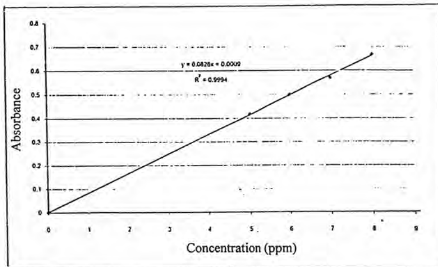
Fig. 27a: Calibration curve of Dye 3
