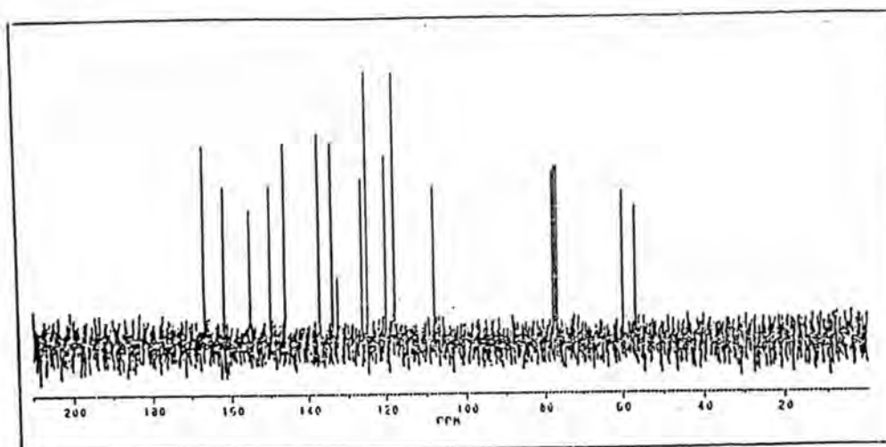
Fig. 30a: ^{13}\text{C} NMR spectrum of Dye 4
