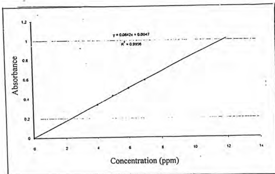
Fig. 57a: Calibration curve of Dye 8
