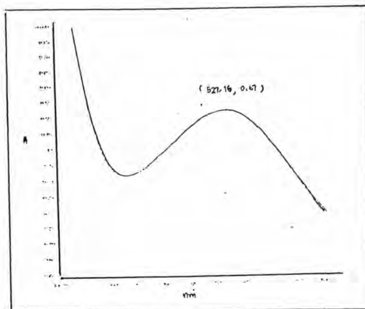
Fig. 62a: UV/VIS spectrum of Dye 2
