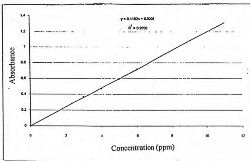
Fig. 39a: Calibration curve of Dye 5
