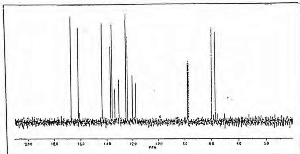
Fig. 48a: ^{13}\text{C} NMR spectrum of Dye 7
