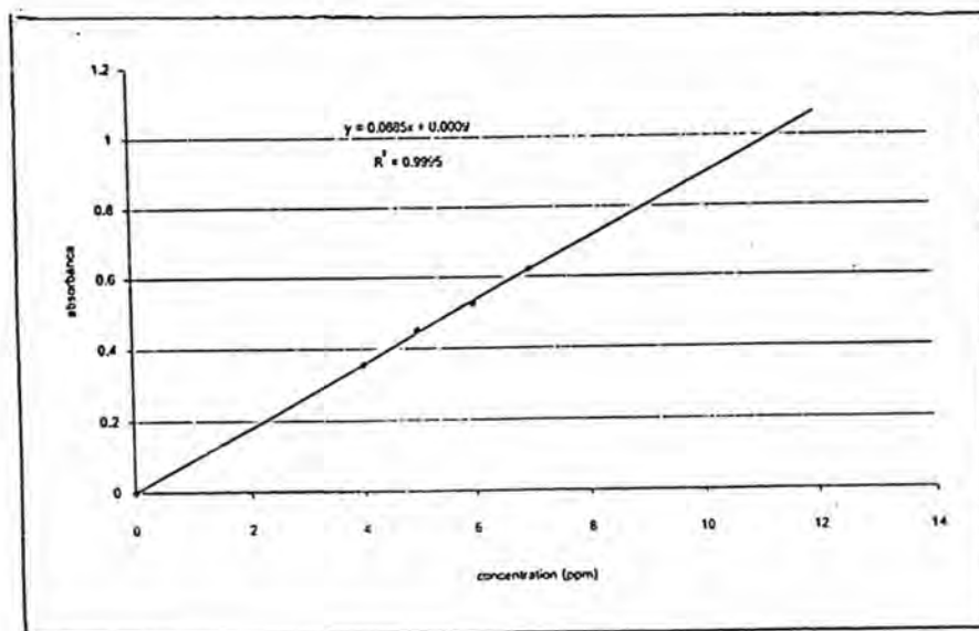
Fig. 81a: Calibration curve of Dye 12
