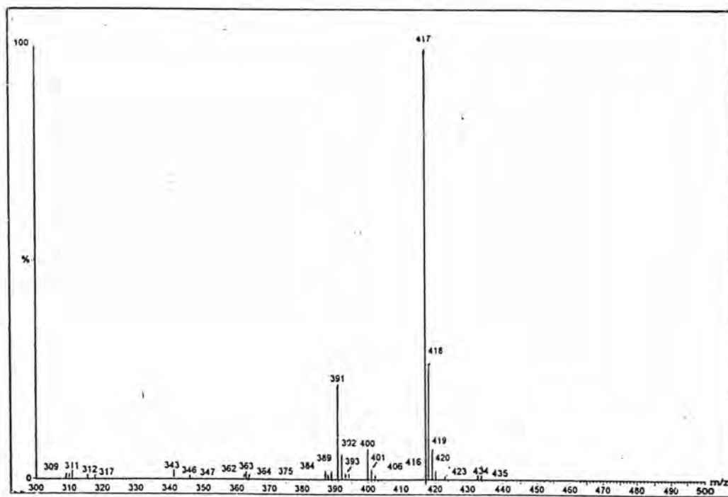
Fig. 13a: Mass spectrum of Dye 1
