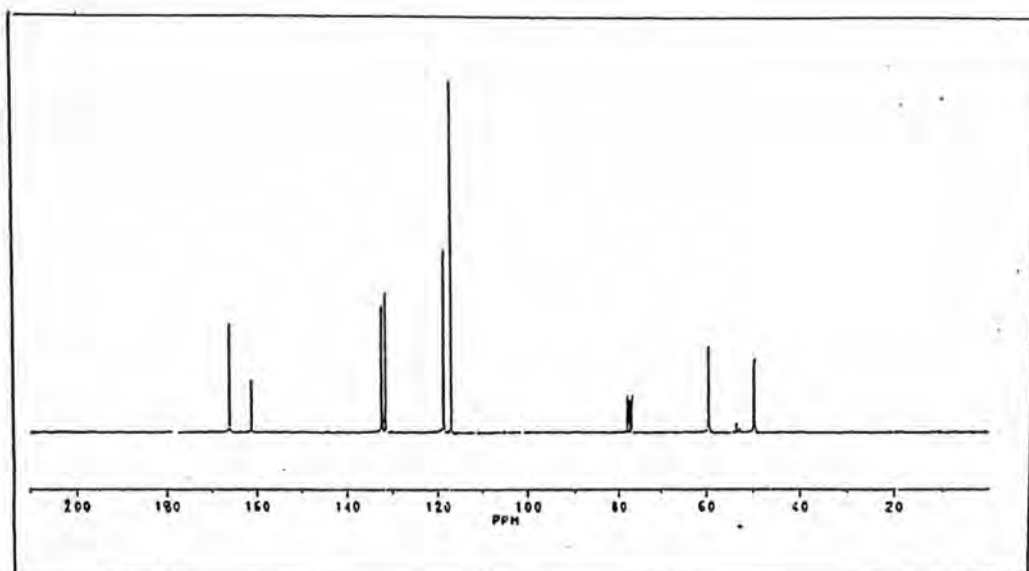
Fig. 6a: ^{13}\text{C} NMR spectrum of Compound 2
