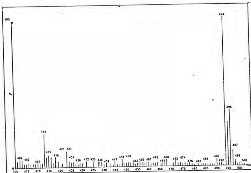
Fig. 43a: Mass spectrum of Dye 6
