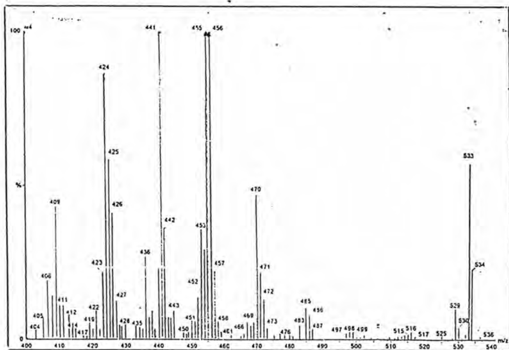
Fig. 79a: Mass spectrum of Dye 12
