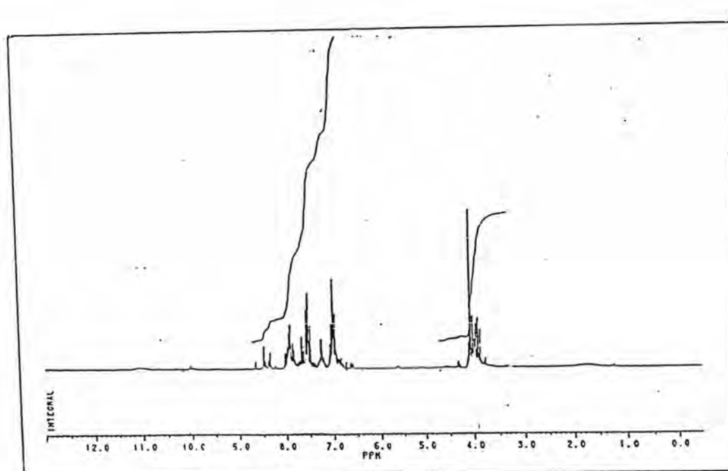
Fig. 29a: 1 H NMR spectrum of Dye 4
