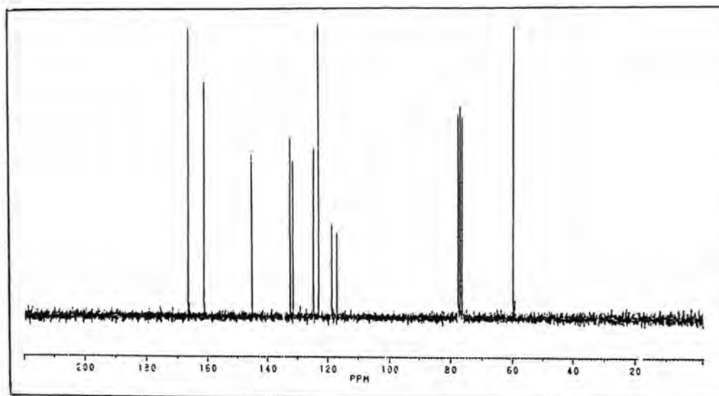
Fig. 12a: ^{13}\text{C} NMR spectrum of Dye 1
