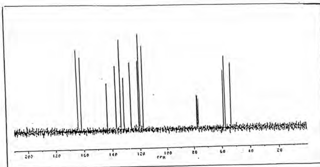
Fig. 66a: ^{13}\text{C} NMR spectrum of Dye 10
