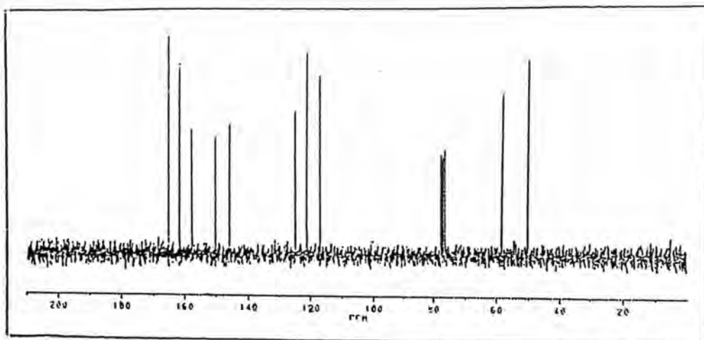
Fig. 36a: ^{13}\text{C} NMR spectrum of Dye 5
