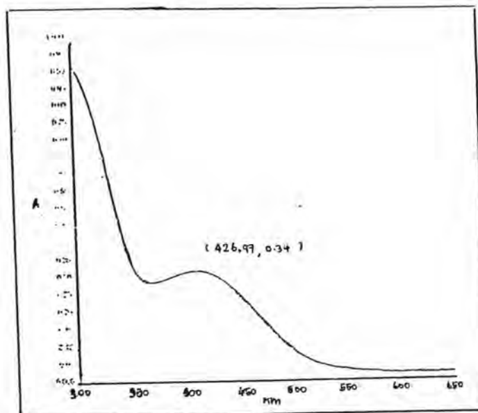
Fig. 50a: UV/VIS spectrum of Dye 7
