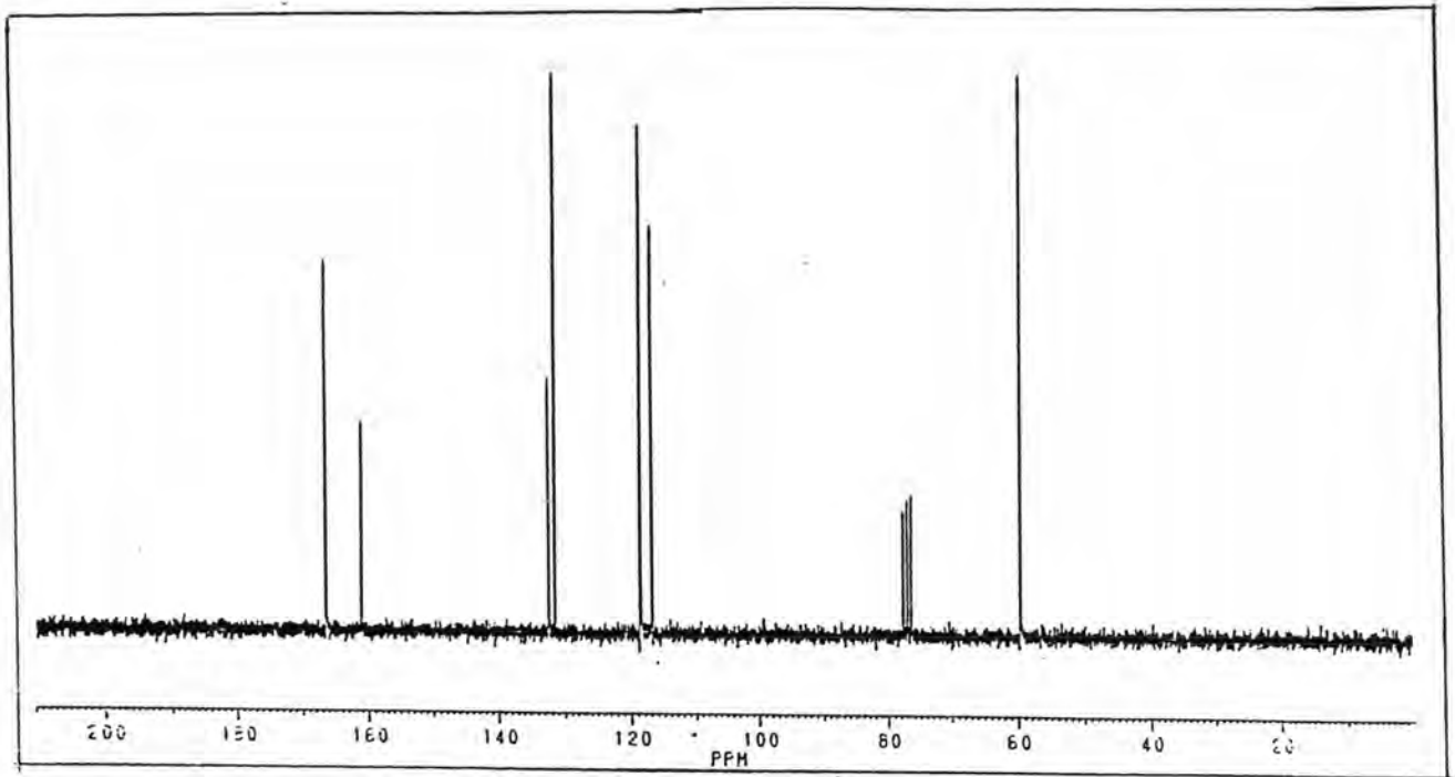
Fig. 3a: ^{13}\text{C} NMR spectrum of Compound 1
