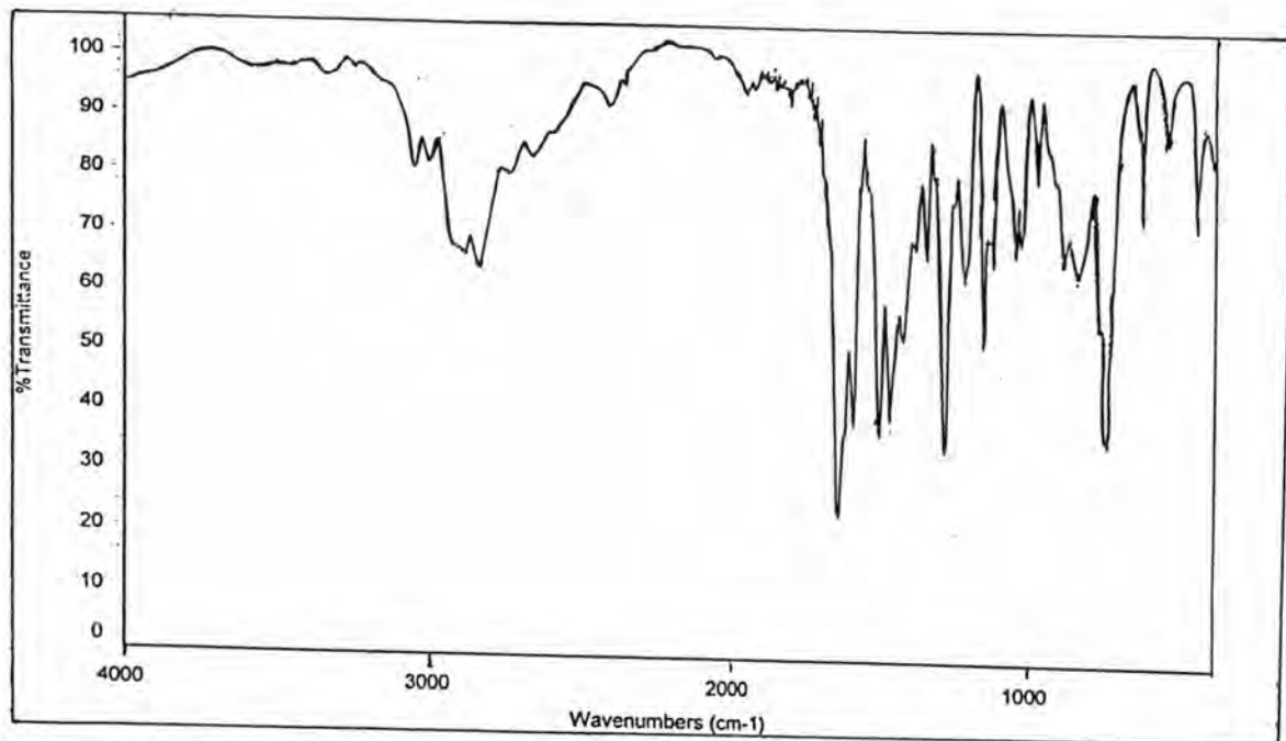
Fig. 4a: IR spectrum of Compound 2
