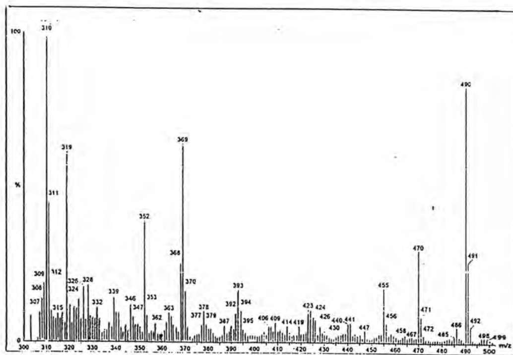
Fig. 55a: Mass spectrum of Dye 8
