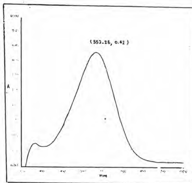
Fig. 20a: UV/VIS spectrum of Dye 2
