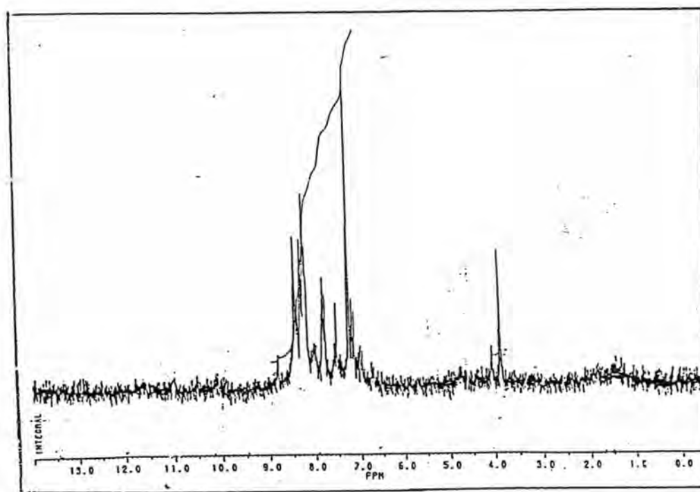
Fig. 41a: 1 H NMR spectrum of Dye 6
