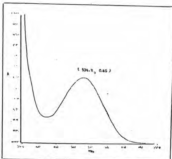
Fig. 32a: UV/VIS spectrum of Dye 4
