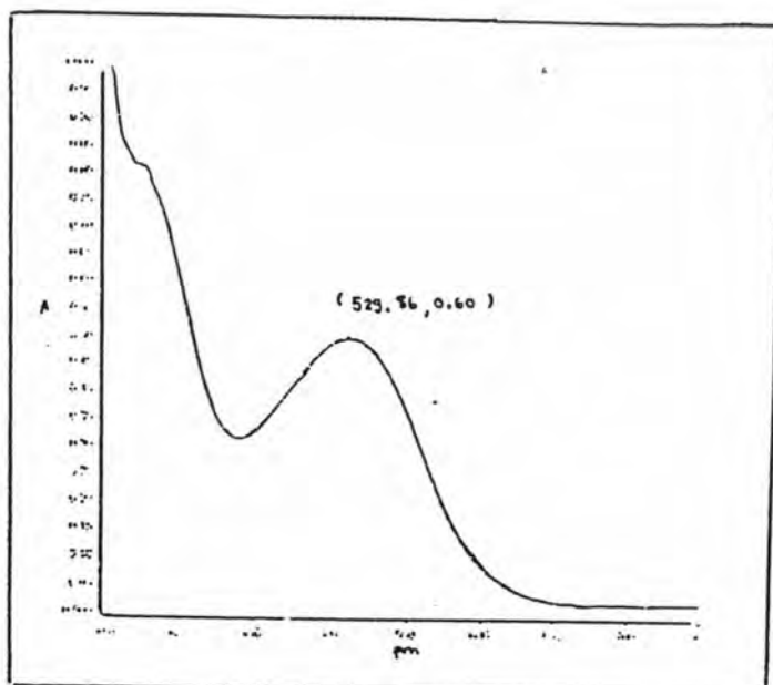
Fig. 38a: UV/VIS spectrum of Dye 5
