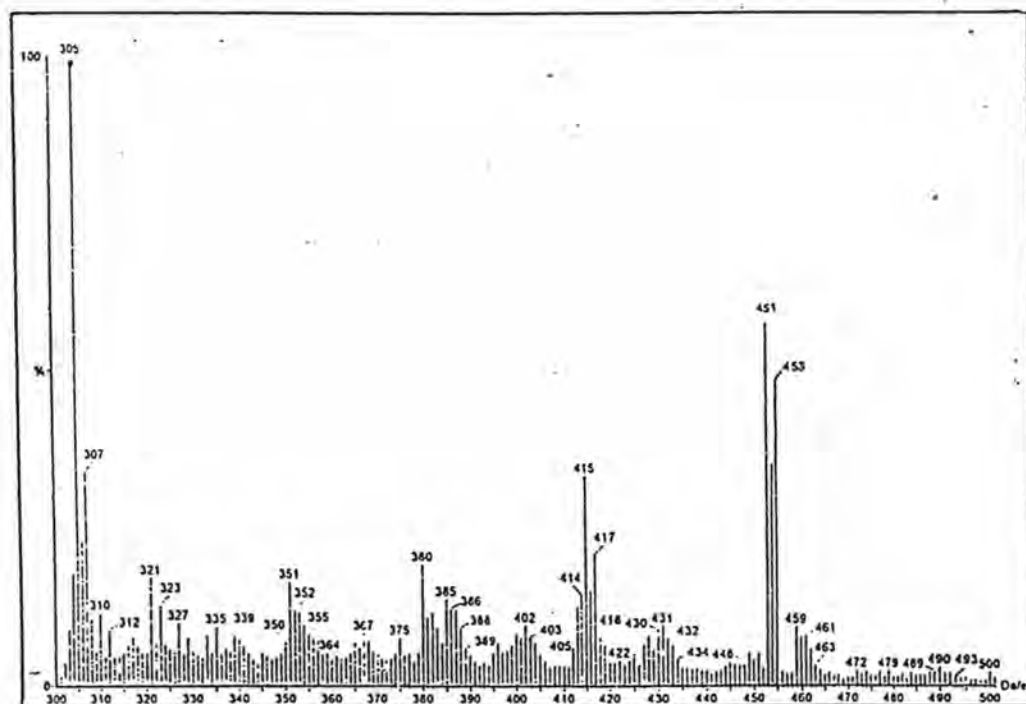
Fig. 25a: Mass spectrum of Dye 3
