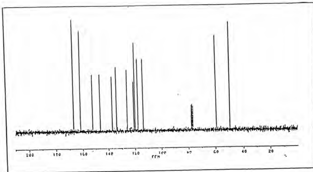
Fig. 42a: ^{13}\text{C} NMR spectrum of Dye 6
