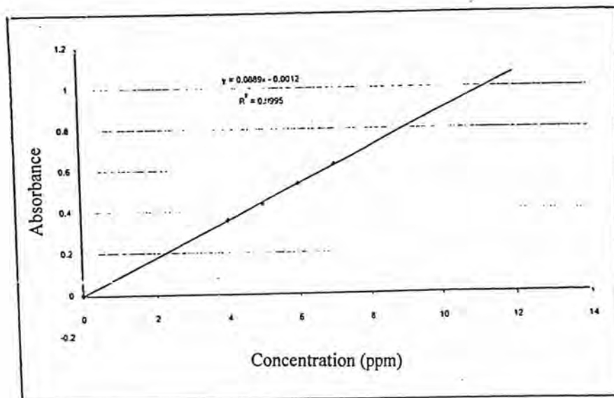
Fig. 45a: Calibration curve of Dye 6
