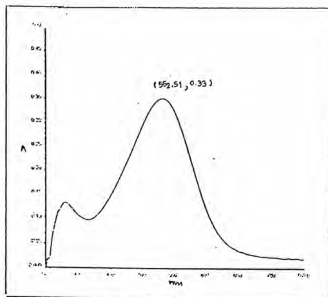
Fig. 68a: UV/VIS spectrum of Dye 10
