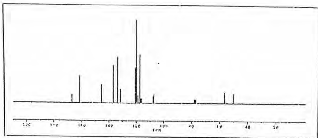
Fig. 54a: ^{13}\text{C} NMR spectrum of Dye 8
