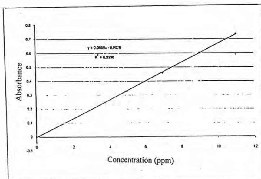
Fig. 69a: Calibration curve of Dye 10
