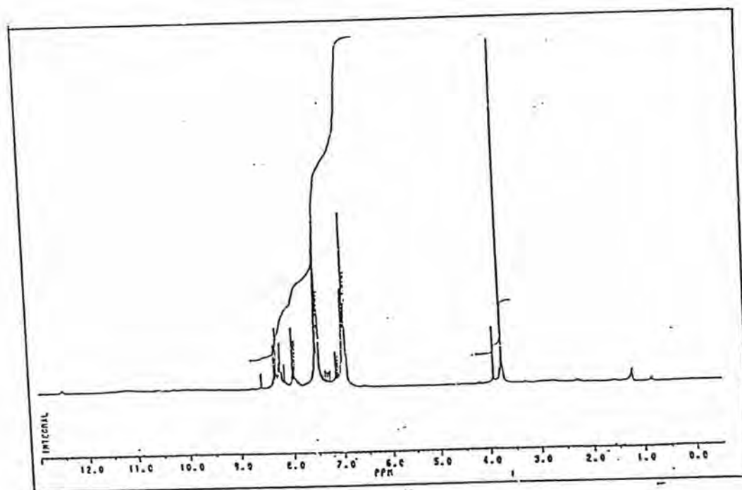
Fig. 59a: 1 H NMR spectrum of Dye 2
