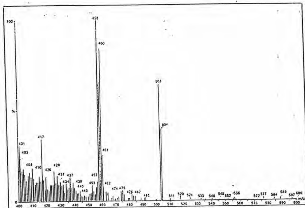
Fig. 61a: Mass spectrum of Dye 2
