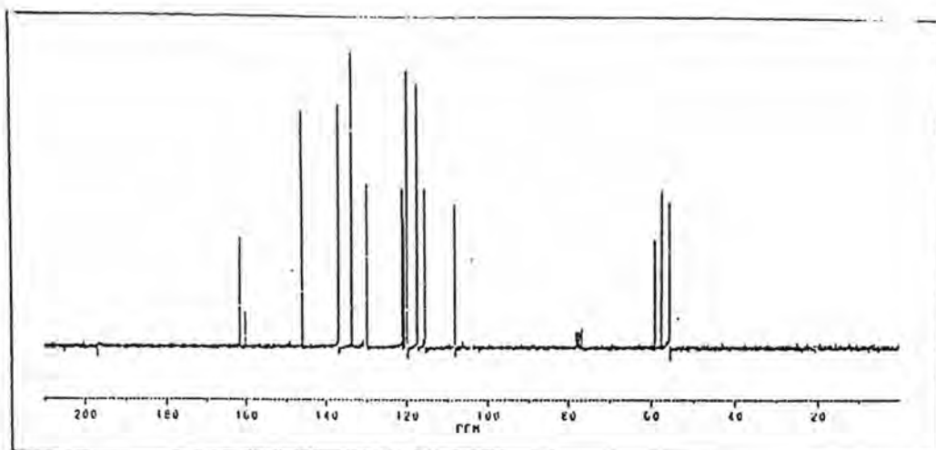
Fig. 78a: ^{13}\text{C} NMR spectrum of Dye 12
