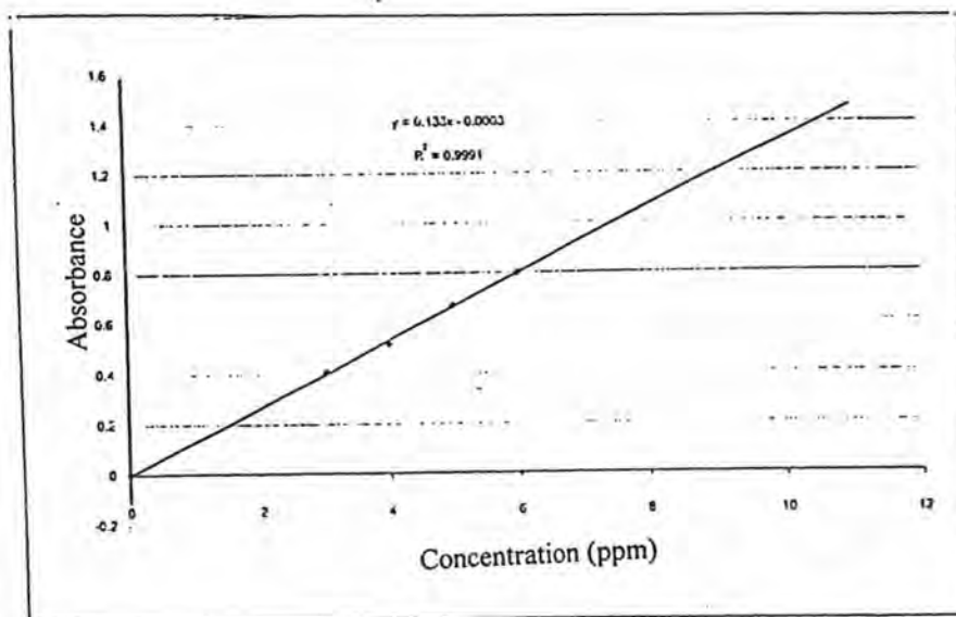
Fig. 63a: Calibration curve of Dye 2
