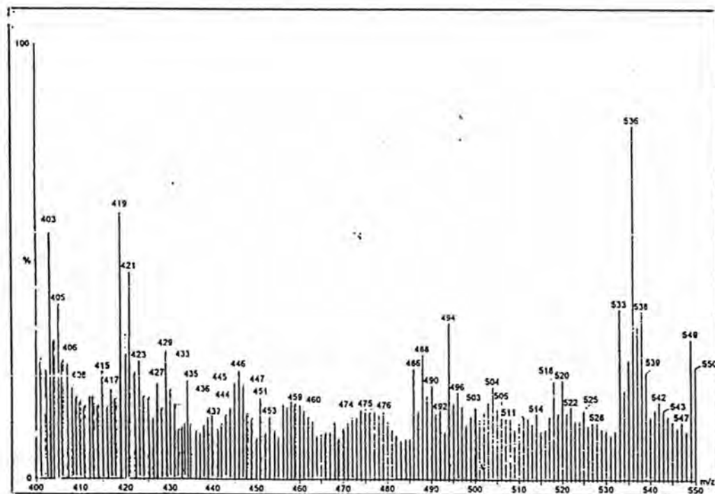
Fig. 73a: Mass spectrum of Dye 11
