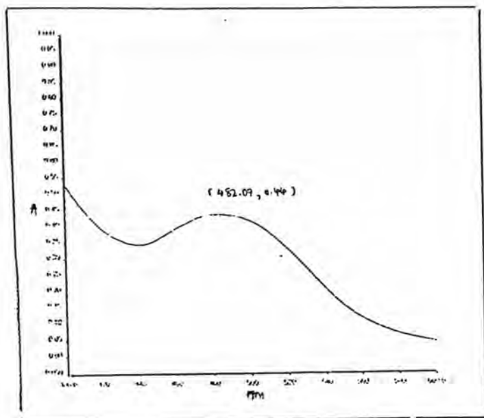
Fig. 74a: UV/VIS spectrum of Dye 11
