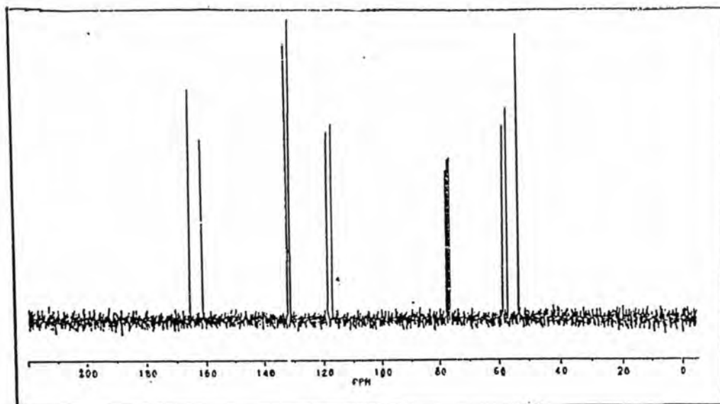
Fig. 9a: ^{13}\text{C} NMR spectrum of Compound 3
