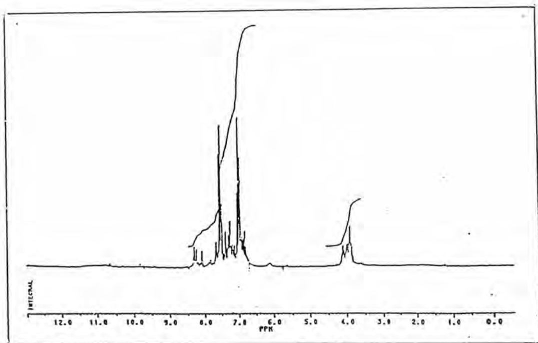
Fig. 47a: 1 H NMR spectrum of Dye 7
