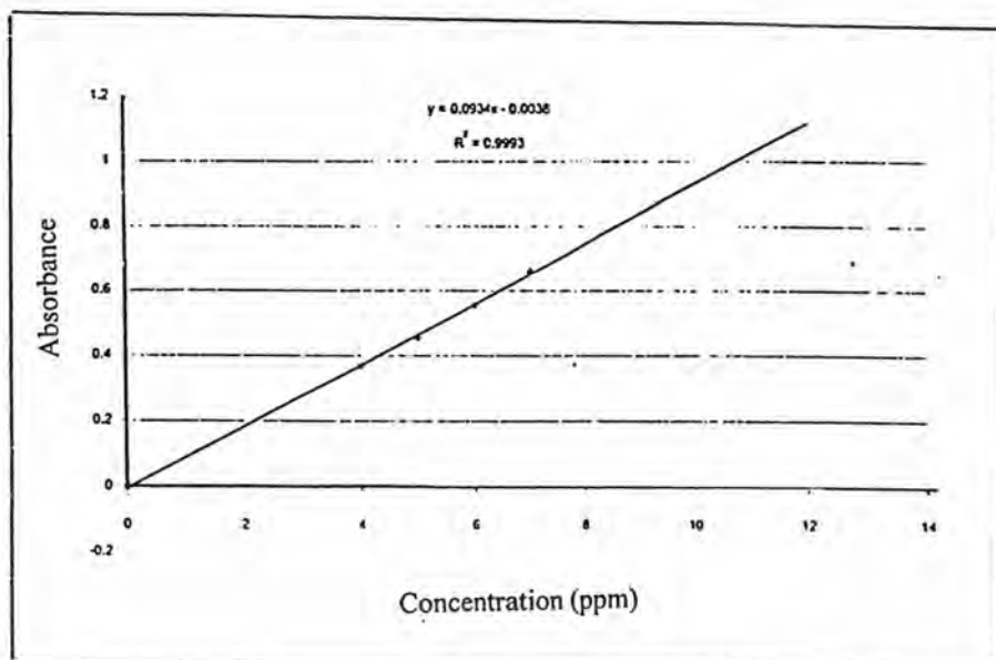
Fig. 33a: Calibration curve of Dye 4
