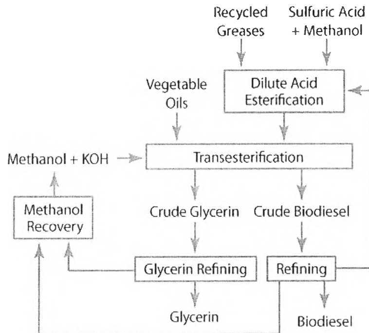
Figure 2.10 Biodiesel production process (AFDC, 2010).
