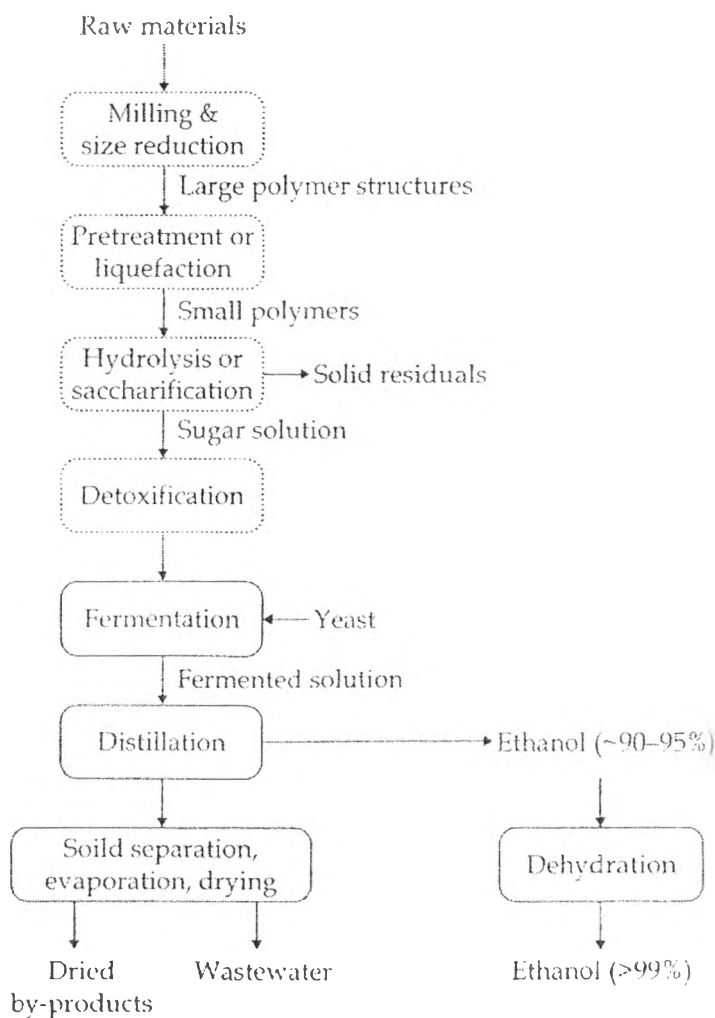
Figure 2.9 Overview of the ethanol production process (Nag, 2008).
