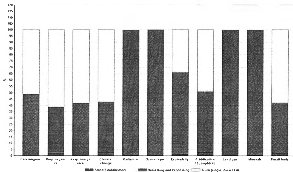
Figure 2.20 The characterized impact factor for natural regeneration scenario (Neupane et al. , 2011).
