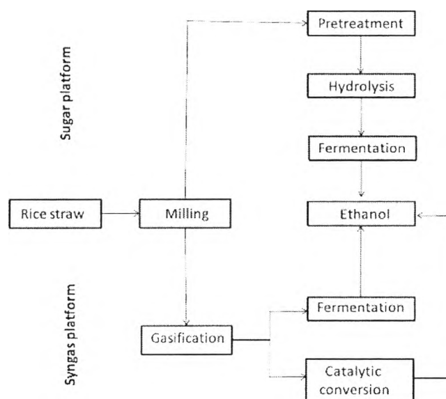
Figure 2.14 Basic concept of ethanol production from rice straw (Binod et.al. , 2010).
