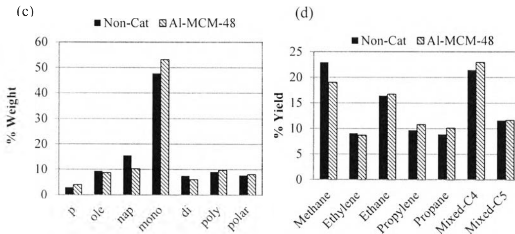
Figure 4.3 (a) Product distribution, (b) Petroleum cuts, (c) Concentration of each group of components in maltene, and (d) Gas composition.
