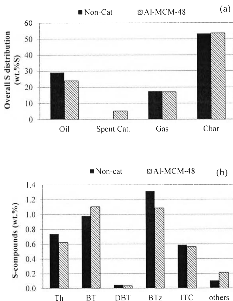
Figure 4.4 (a) Overall sulfur distribution in pyrolytic products, and (b) Sulfur – containing compounds in maltenes.
