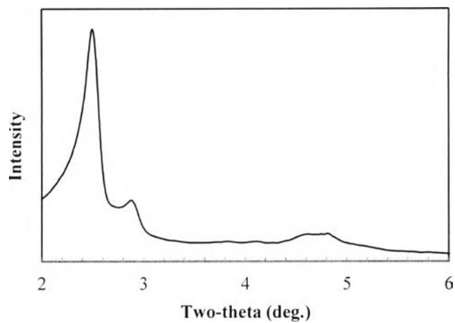
Figure 4.1 SAXS pattern of Al-MCM-48.
