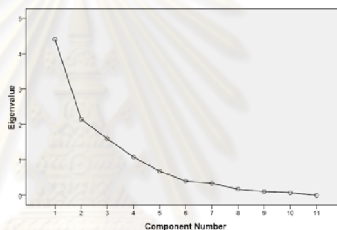
Scree Plot
