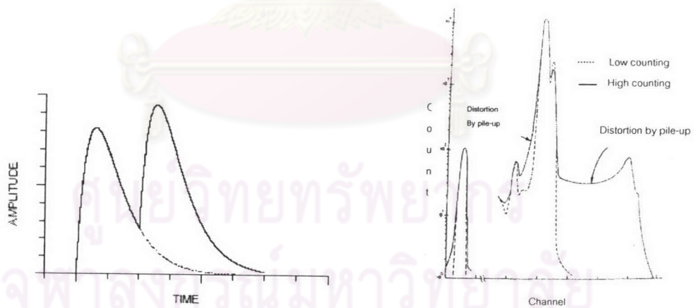
a) Pulse pile up
