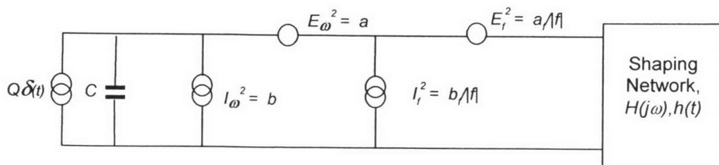
Fig. 2.9 Detector amplifiers modeled with noise sources.
