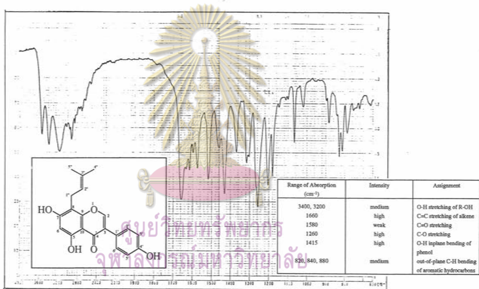
Figure 36 Infrared absorption spectrum of DR-4
