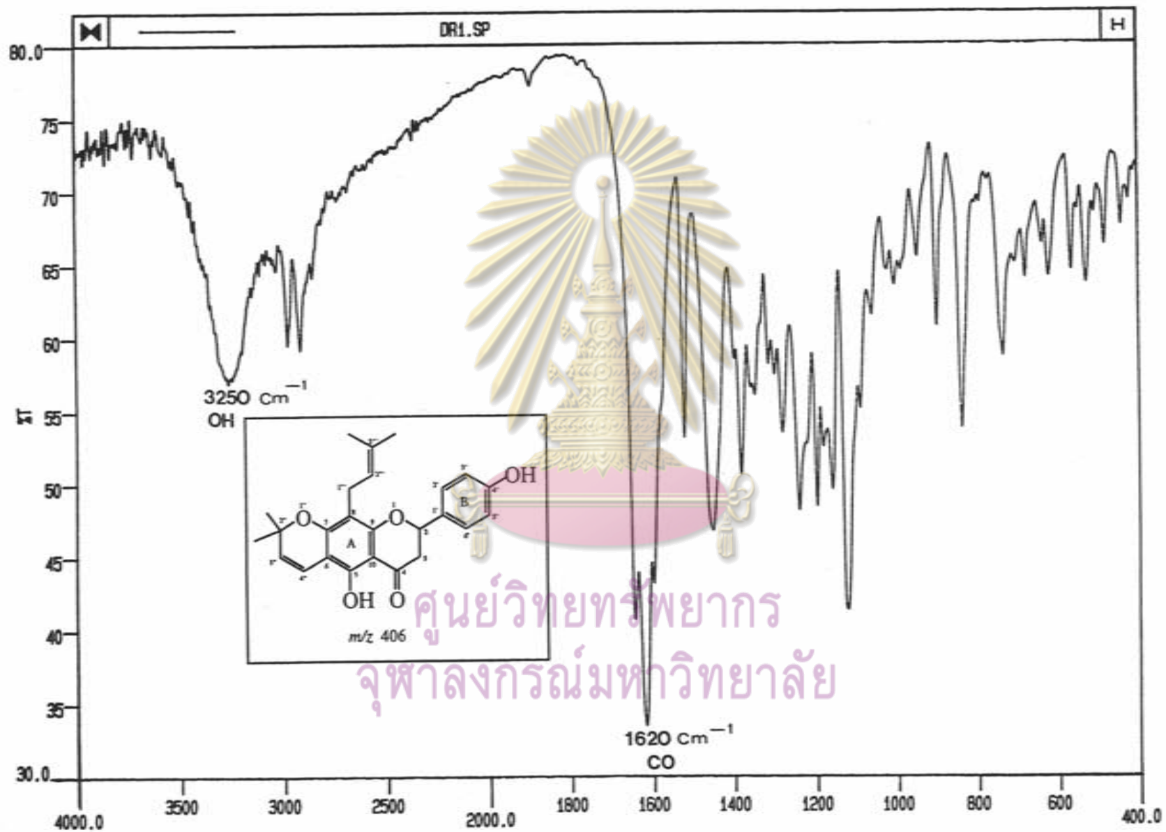
Figure 28 IR spectrum of DR-1
