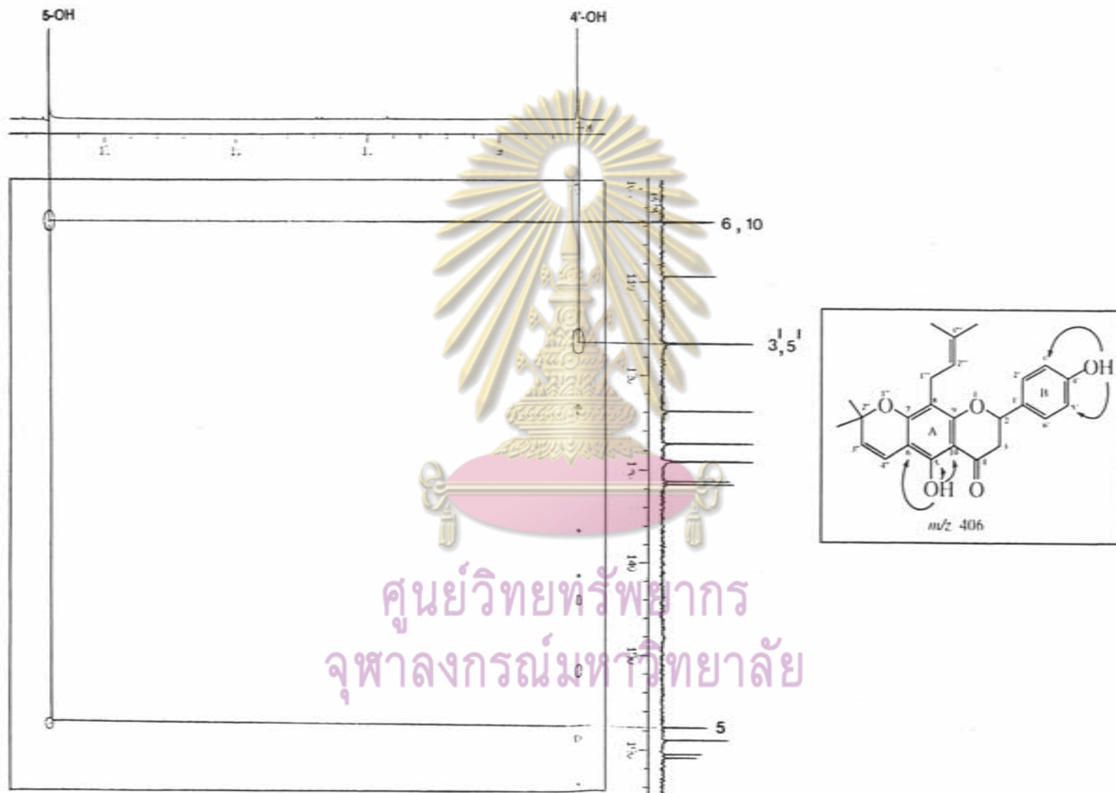
Figure 34.1 HMBC spectrum of DR-1 in acetone - d 6
