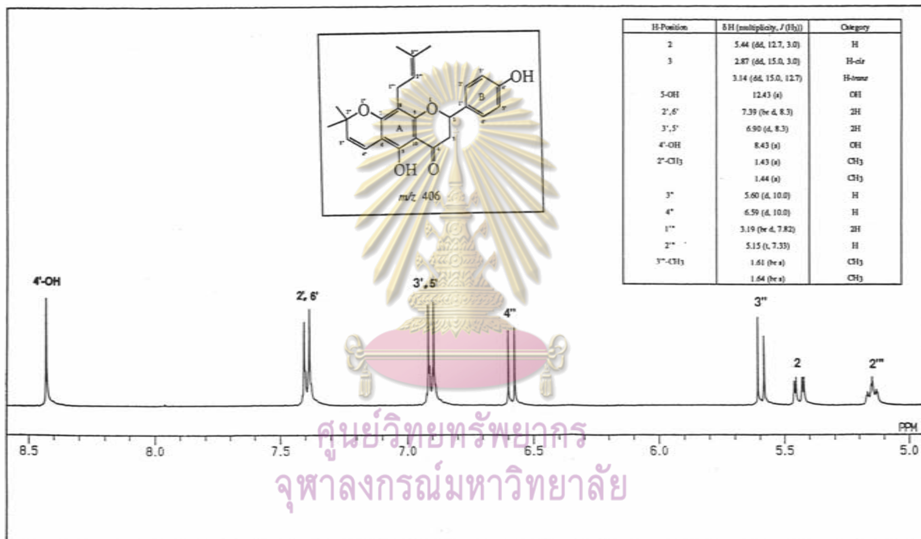
Figure 30.2 ^1\text{H-NMR} spectrum of DR-1 in acetone- d_6
