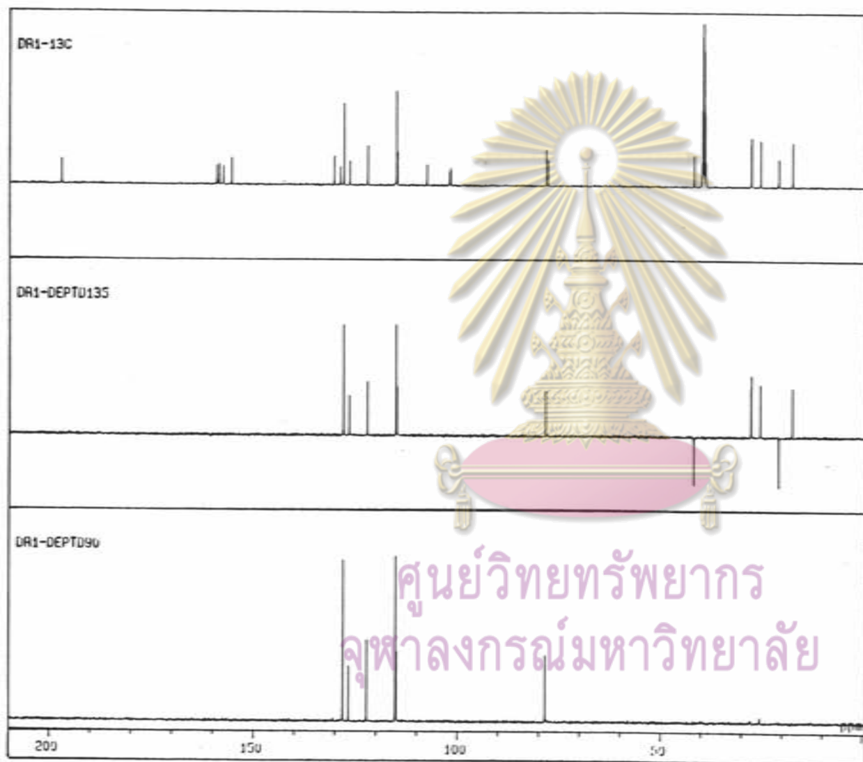
Figure 32.1 ^{13}\text{C} -NMR spectrum of DR-1 (DEPT)
