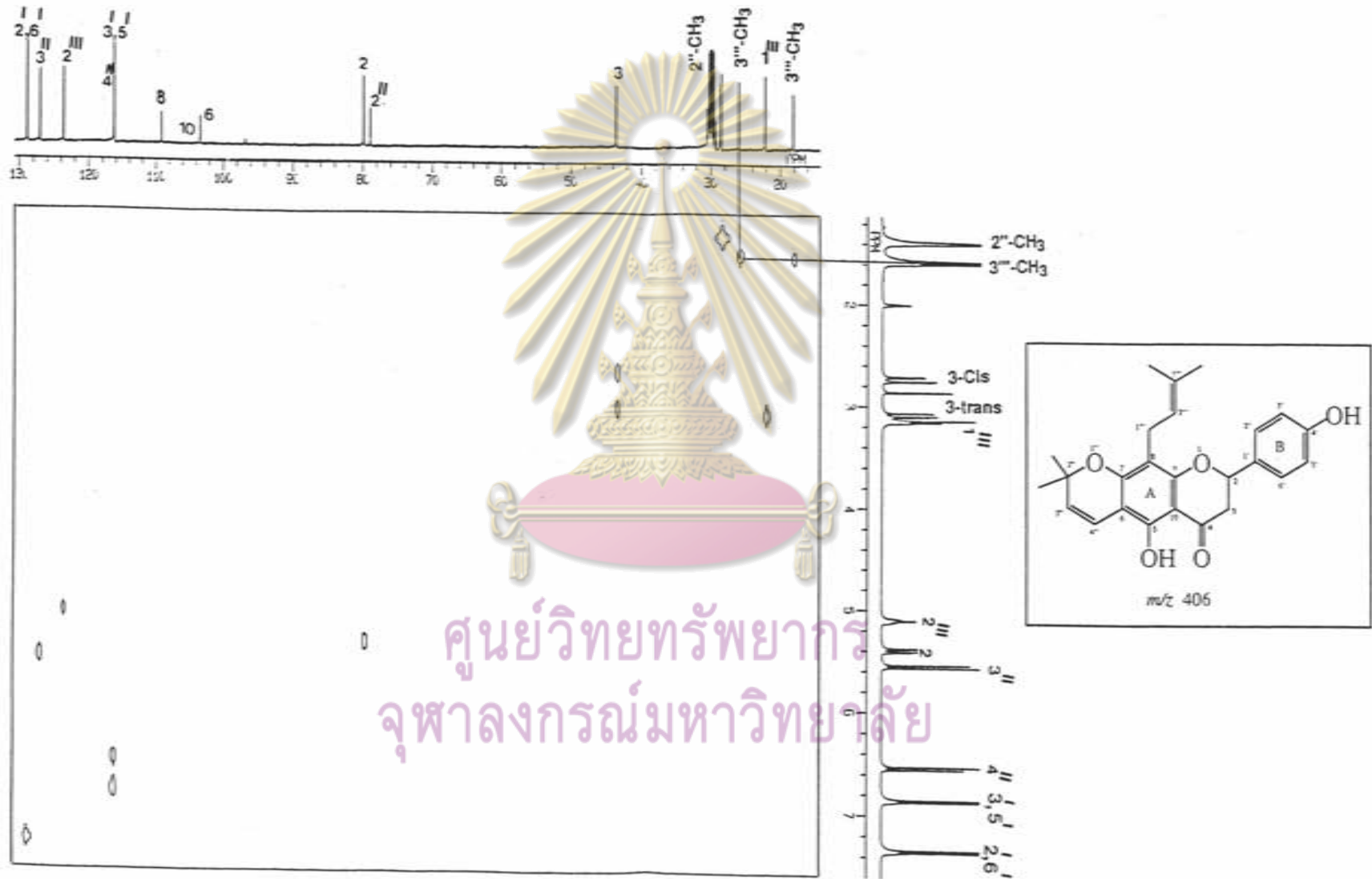
Figure 33.1 HETCOR spectrum of DR-1 in acetone- d_6
