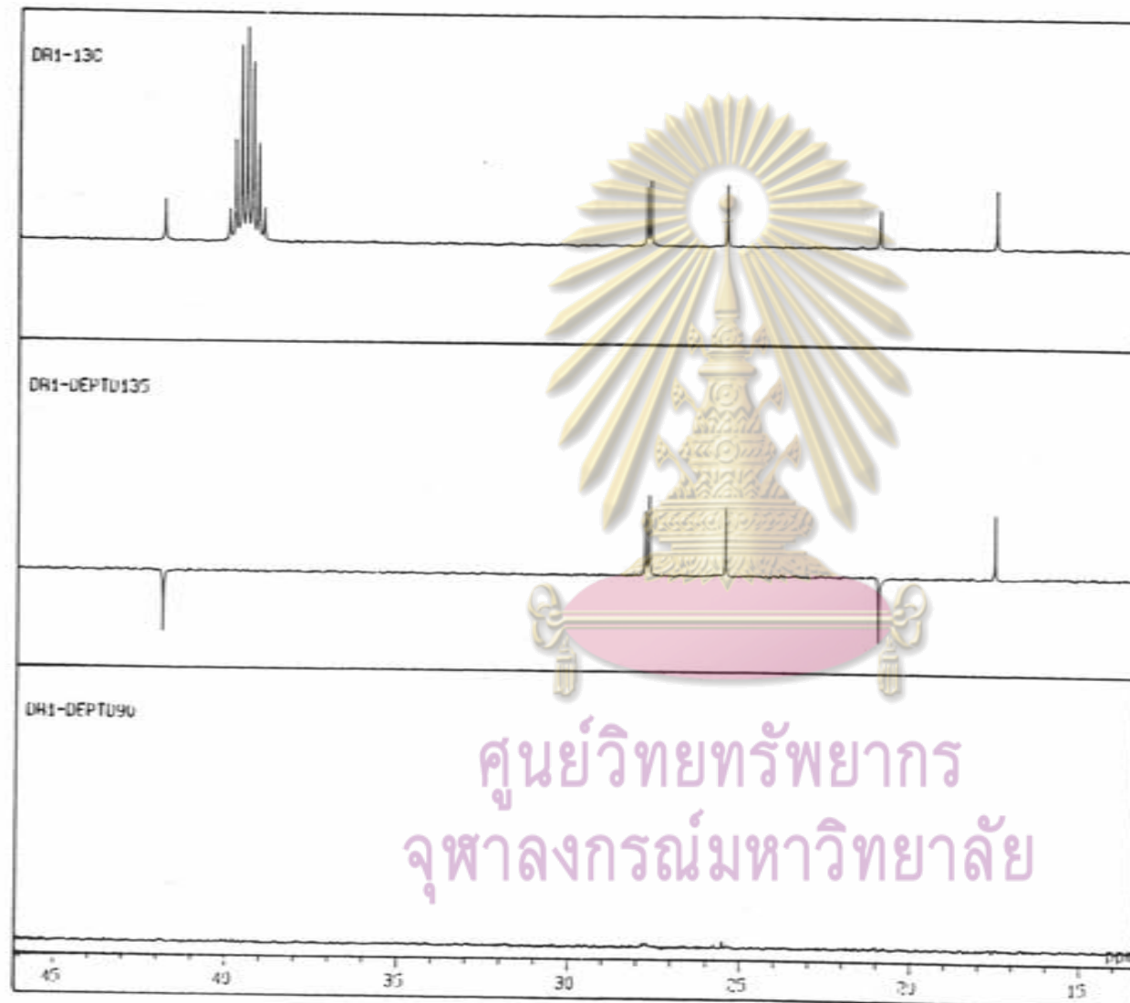
Figure 32 ^{13}\text{C} -NMR spectrum of DR-1 (DEPT)
