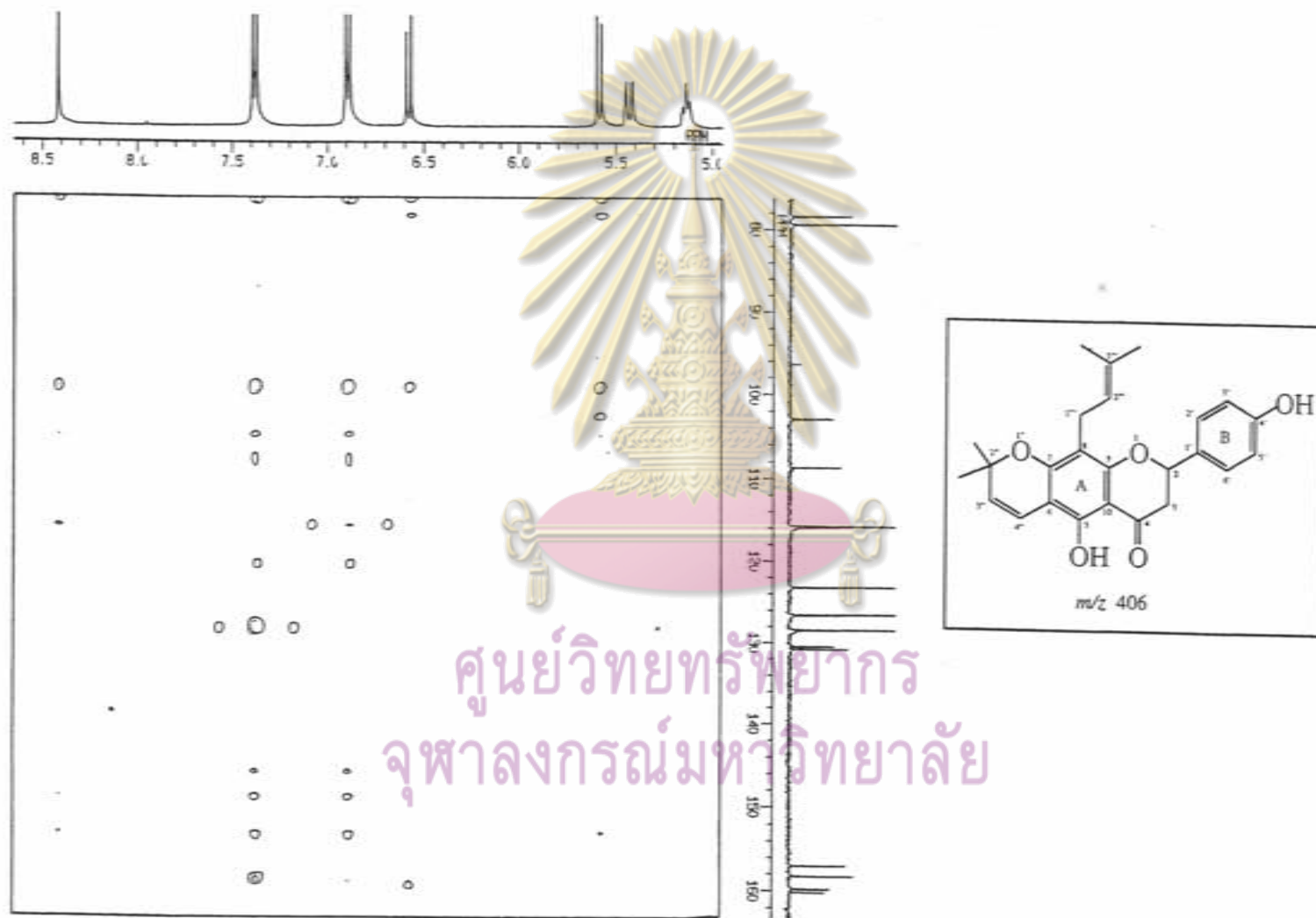
Figure 34.4 HMBC spectrum of DR-1 in acetone- d_6
