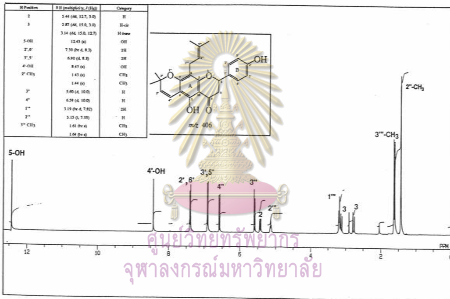
Figure 30 ^1\text{H-NMR} spectrum of DR-1 in acetone - d_6
