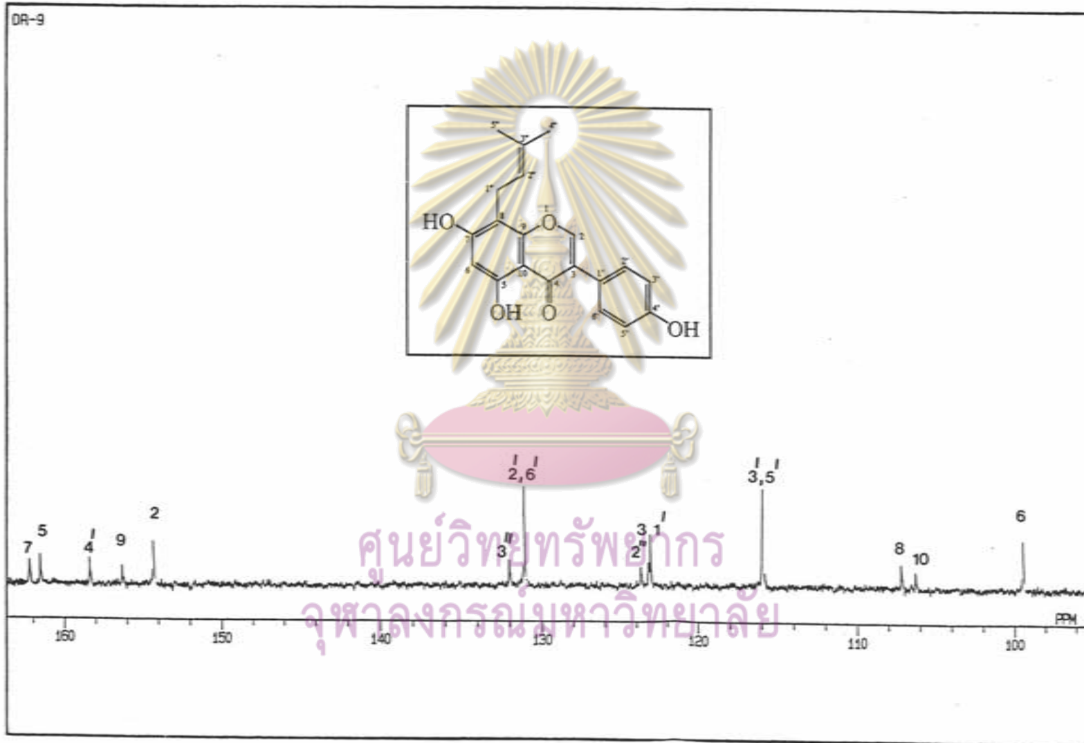
Figure 38 ^{13}\text{C} -NMR spectrum of DR-4 in acetone- d_6
