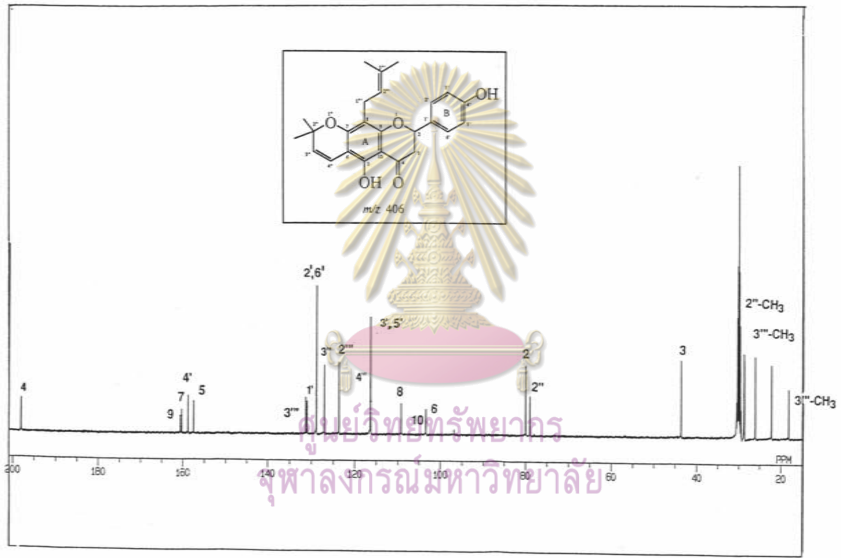
Figure 31 ^{13}\text{C} -NMR spectrum of DR-1 in acetone- d_6
