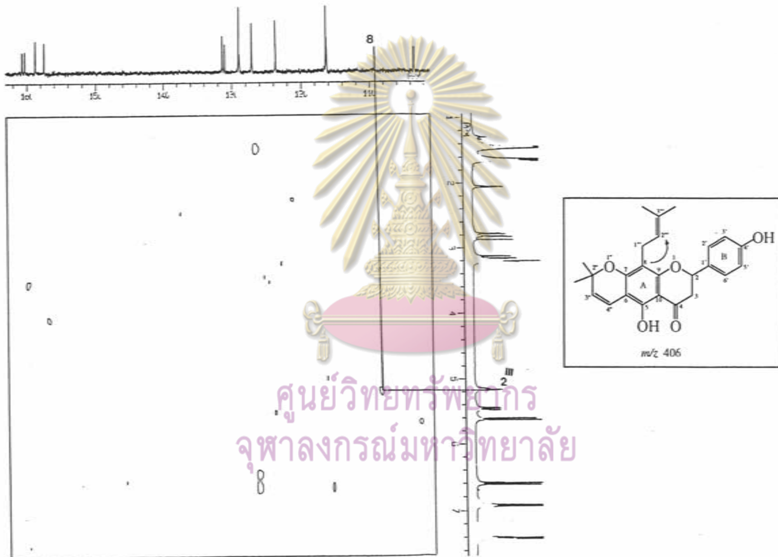
Figure 34.7 COLOC spectrum of DR-1 in acetone- d_6
