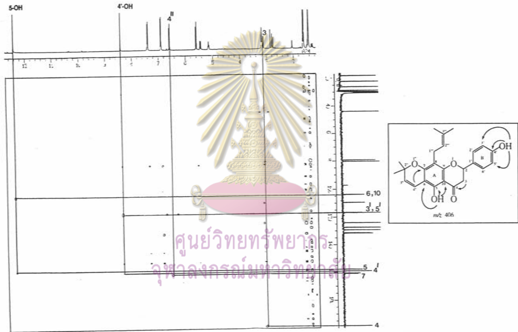
Figure 34.2 HMBC spectrum of DR-1 in acetone- d_6
