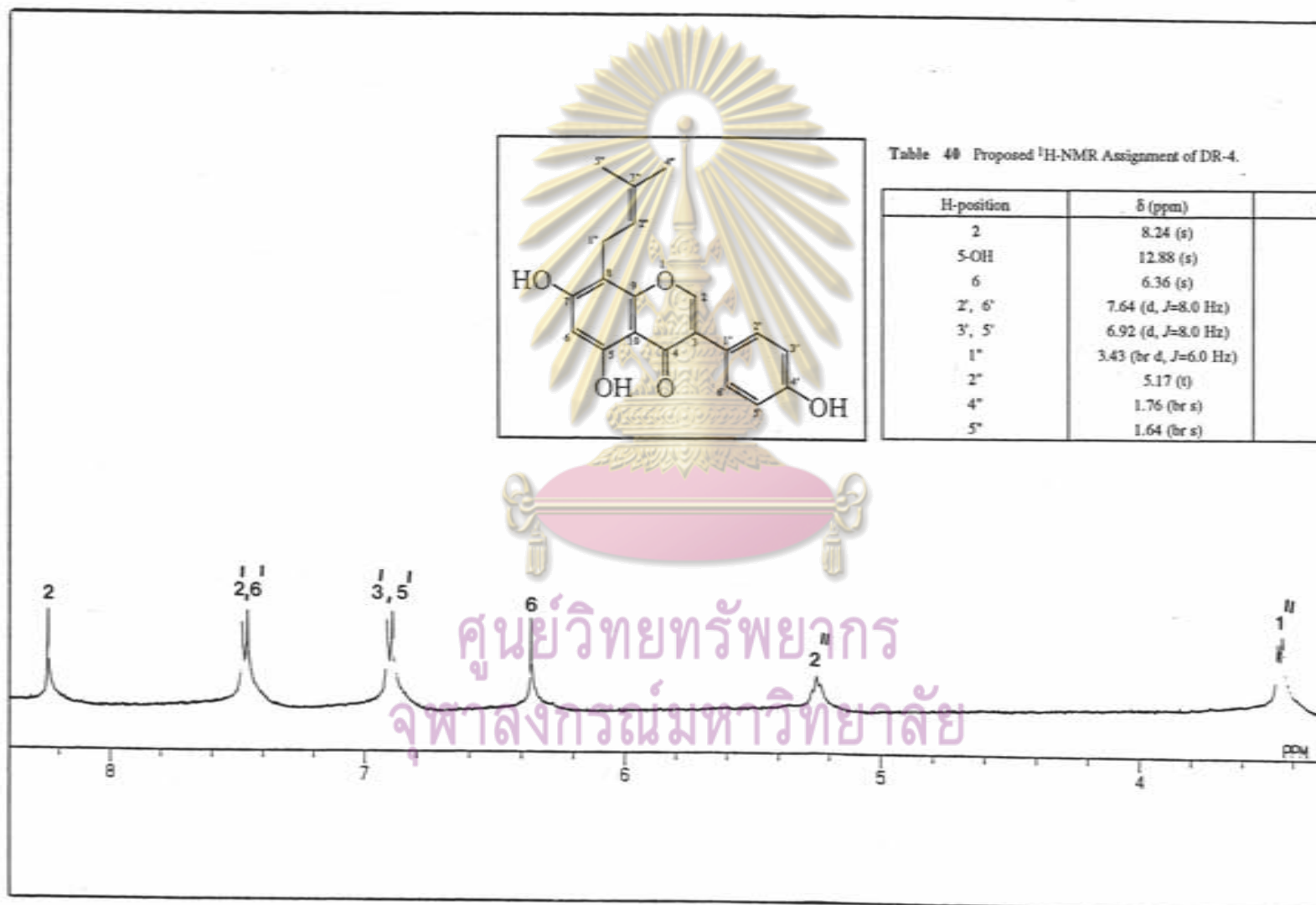
Figure 37.1 ^1\text{H-NMR} spectrum of DR-4 in acetone -d_6
