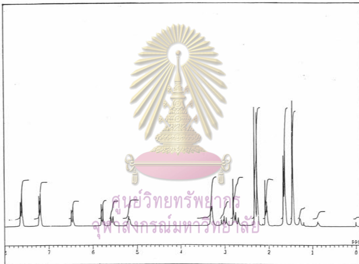
Figure 30.3 ^1\text{H-NMR} spectrum of DR-1 (acetylated DR-1)
