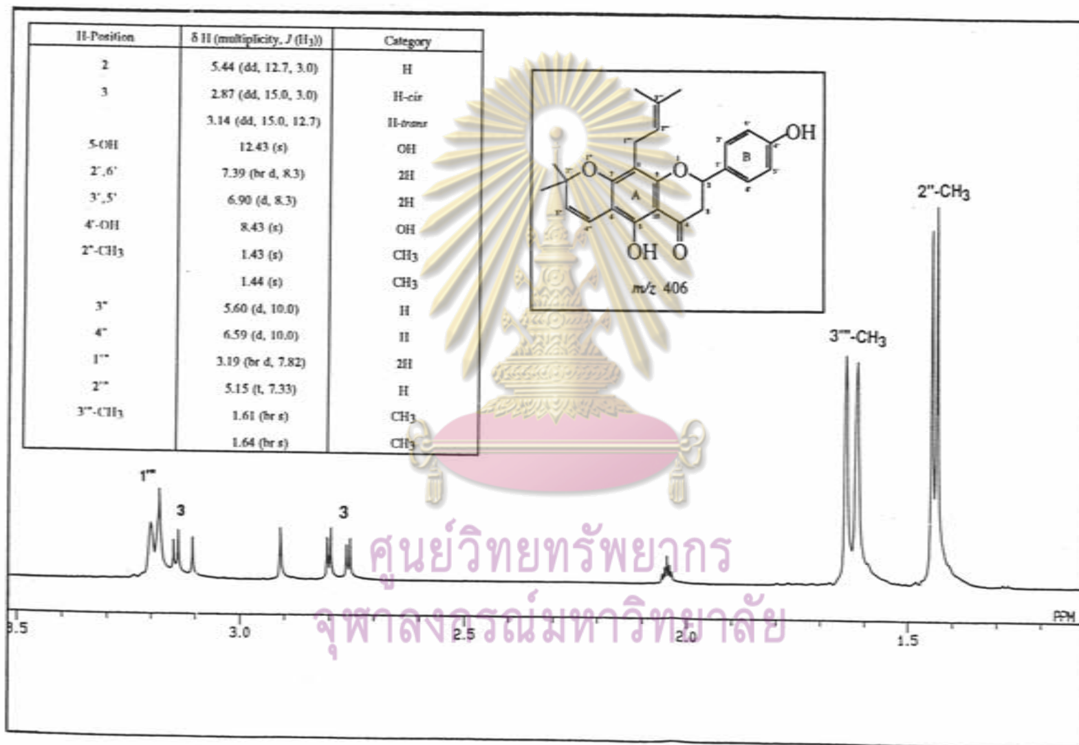
Figure 30.1 1 H-NMR spectrum of DR-1 in acetone - d 6
