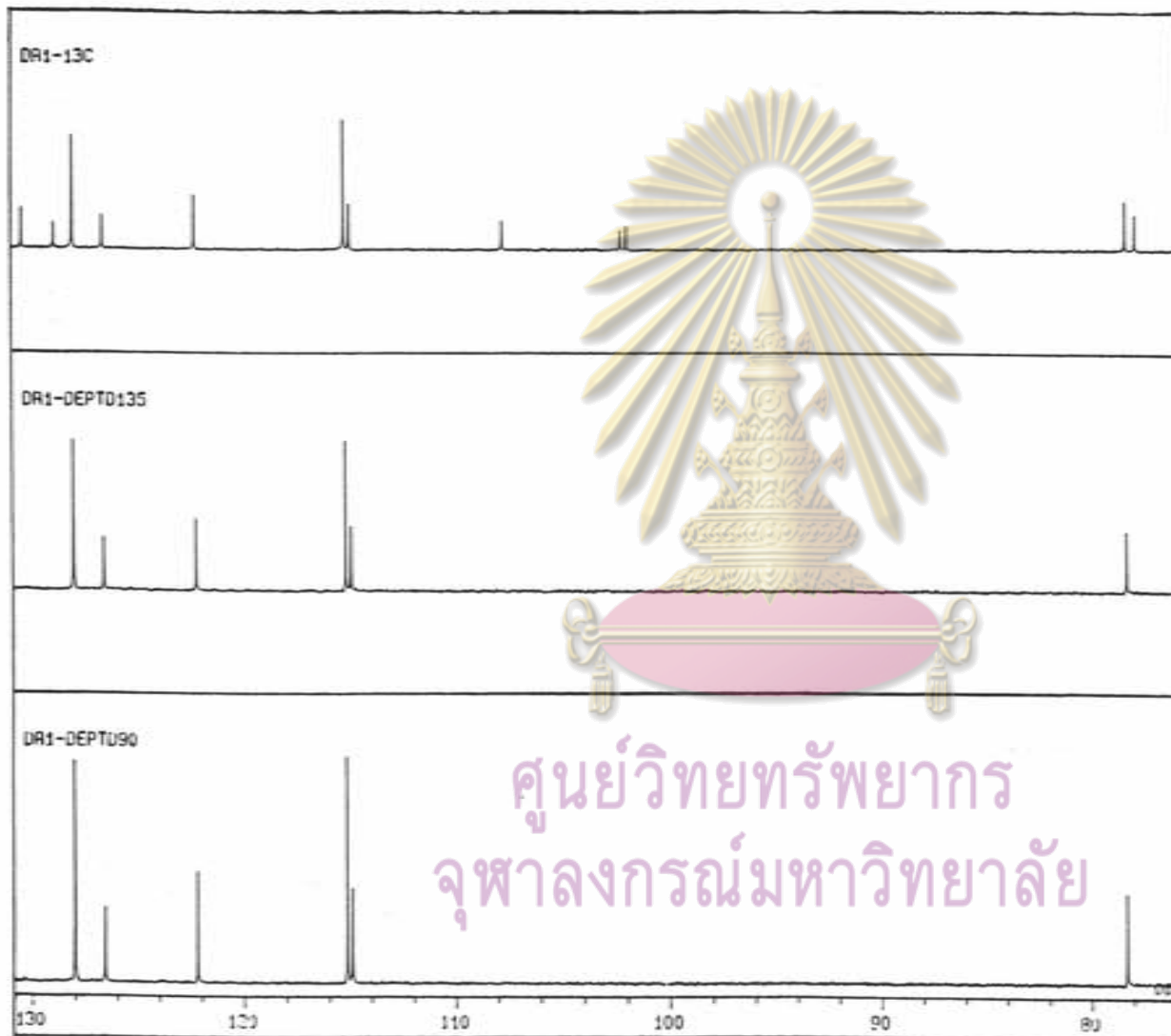
Figure 32.2 ^{13}\text{C} -NMR spectrum of DR-1 (DEPT)
