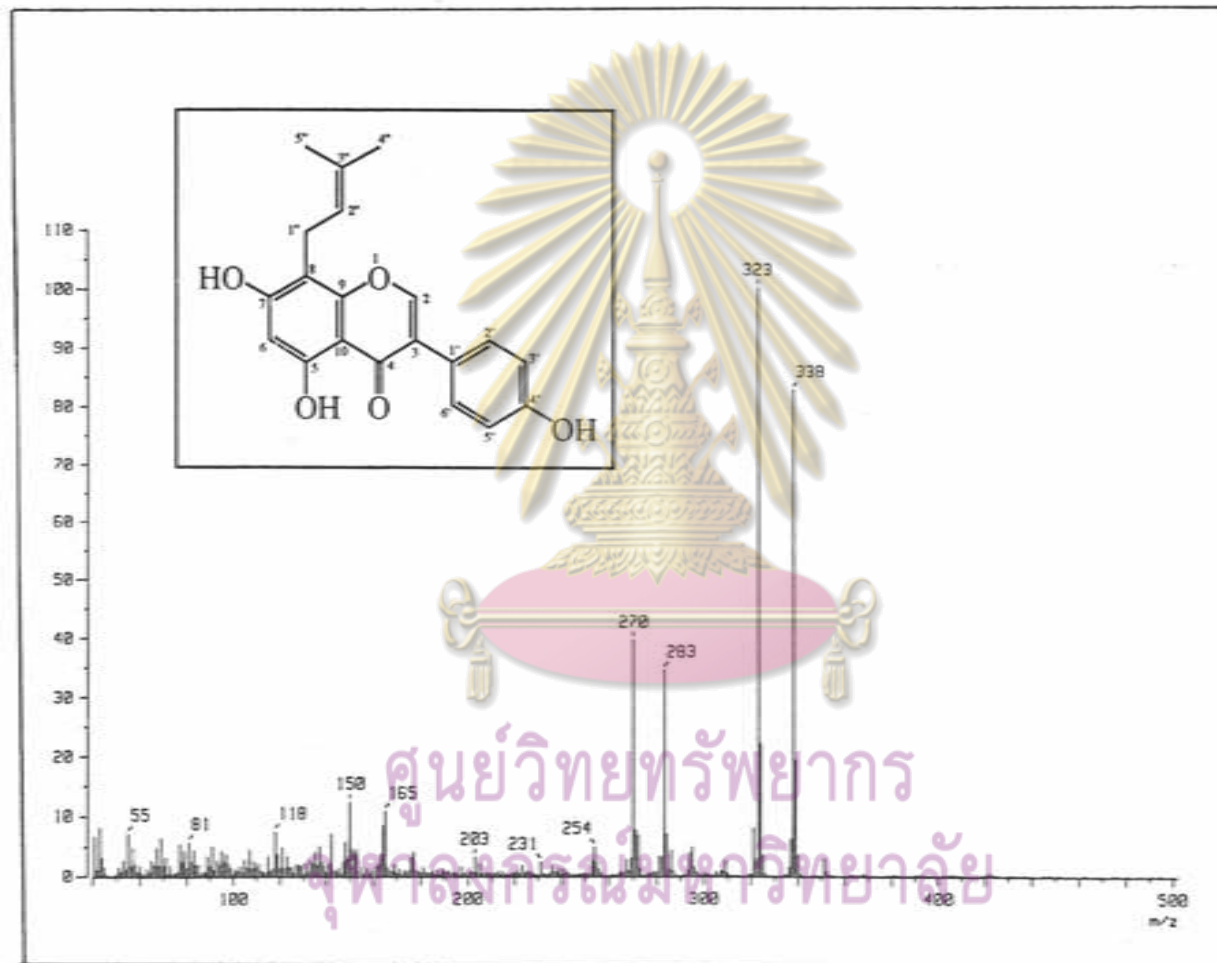
Figure 35 EI mass spectrum of DR-4
