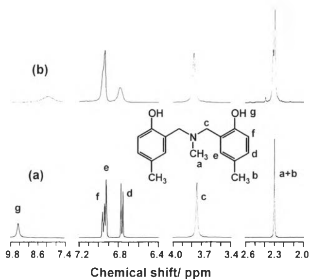
Figure 9. ^1\text{H} NMR (400 MHz) spectra of (a) 1 and (b) 1 - \text{CuCl}_2 in \text{CDCl}_3 .
