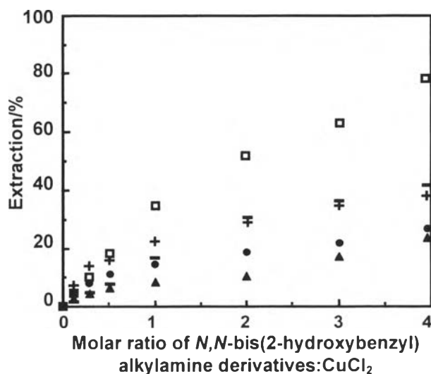
Figure 4. Extraction percentages of (□) 1, (+) 2, (●) 3, (-) 4, and (▲) 5 as a function of molar ratio to CuCl 2 .
