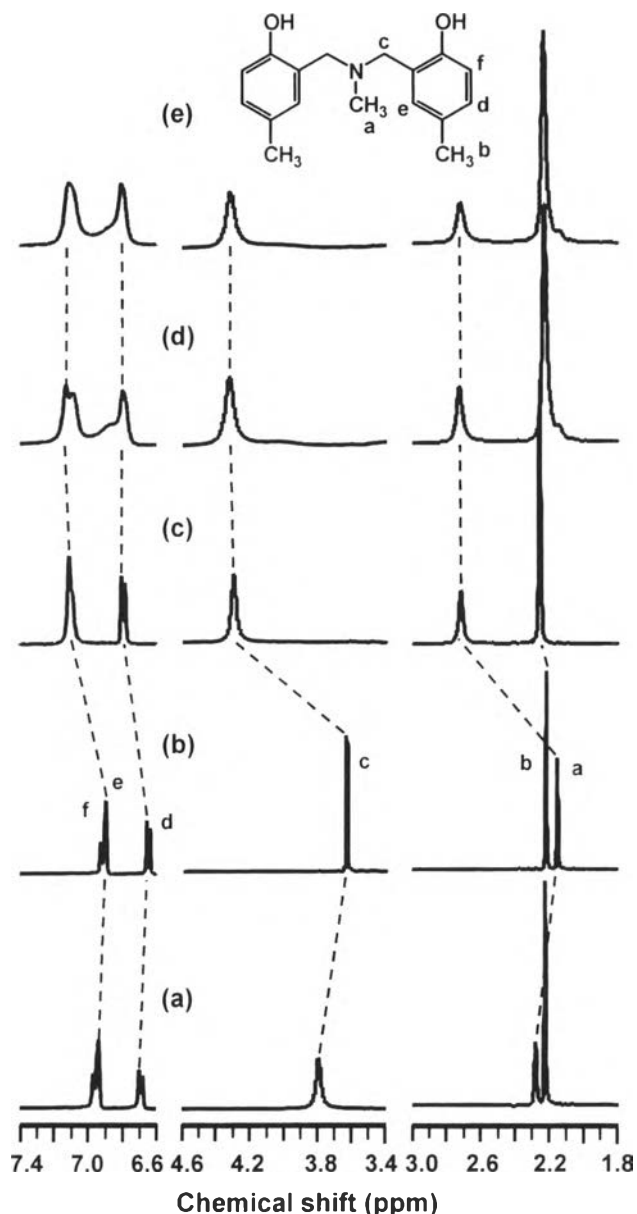
Figure 12. ^1\text{H} NMR (400 MHz) spectra of (a) 1 - \text{CdCl}_2 , (b) 1 , and 1 - \text{ZnCl}_2 at the ratios of (c) 1:1, (d) 1:8, and (e) 1:15 in methanol- d_4 .
