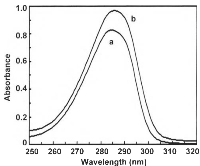
Figure 13. UV Spectra of (a) 1.65 \times 10^{-4} M solution of 1 and (b) 1 -CdCl 2 (1:8).
