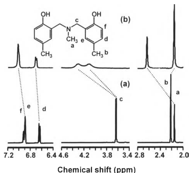
Figure 2. ^1\text{H} NMR (400 MHz) spectra of (a) 1 and (b) 1 - \text{CuCl}_2 in methanol- d_4 with a 1:1 host-guest ratio.
