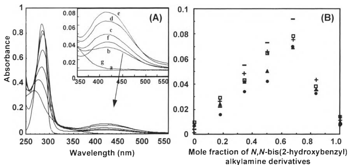
Figure 1. (A) UV-Vis spectra of 1 - \text{CuCl}_2 in methanol at various volumetric ratios; a) 0:6, b) 1:5, c) 2:4, d) 3:3, e) 4:2, f) 5:1, and g) 6:0. (B) Job's Plot as a function of mole fraction of ( \square ) 1 , ( + ) 2 , ( \bullet ) 3 , ( - ) 4 at 415 nm, and ( \blacktriangle ) 5 at 435 nm.
