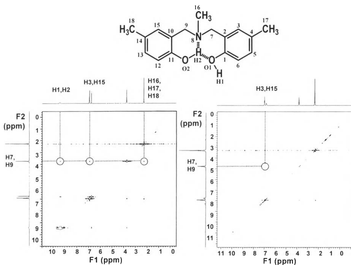
Figure 10. ^1\text{H} - ^1\text{H} NOESY (400 MHz) spectra of (a) 1 and (b) 1 - \text{CuCl}_2 in \text{CDCl}_3 .
