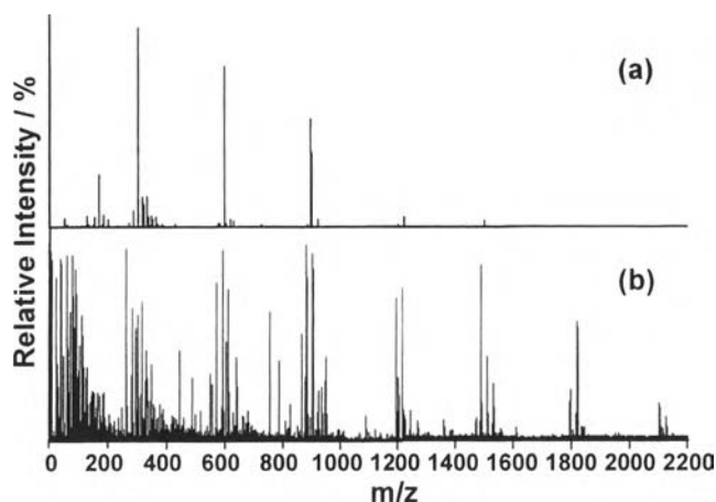
Figure 3. ESIMS spectra of (a) 4 and (b) 4 -CuCl 2 with an orifice of 35V.
