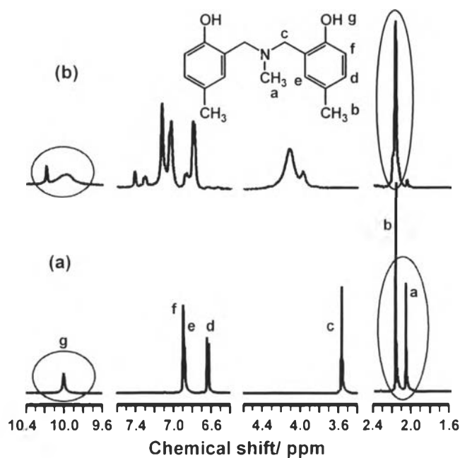
Figure 8. ^1\text{H} NMR (400 MHz) spectra of (a) 1 and (b) 1 - \text{CuCl}_2 in \text{DMSO-}d_6 .
