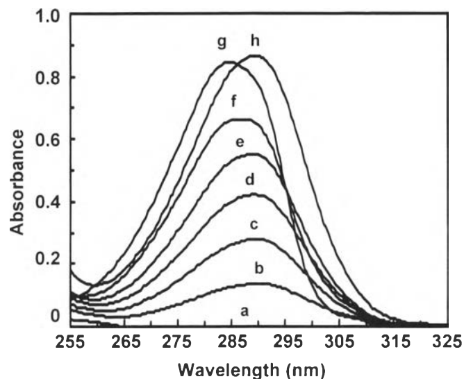
Figure 11. UV Spectra of 1 ( 1.65 \times 10^{-4} M) mixing with \text{ZnCl}_2 ( 1.65 \times 10^{-4} M) in methanol at the volumetric ratios of a) 0:6, b) 1:5, c) 2:4, d) 3:3, e) 4:2, f) 5:1, and g) 6:0, and h) 1.65 \times 10^{-4} M solution of 1 mixed with \text{ZnCl}_2 at the molar ratio of 1:8.
