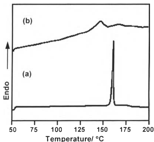
Figure 7. DSC thermograms of (a) 1 and (b) 1 -CuCl 2 .
