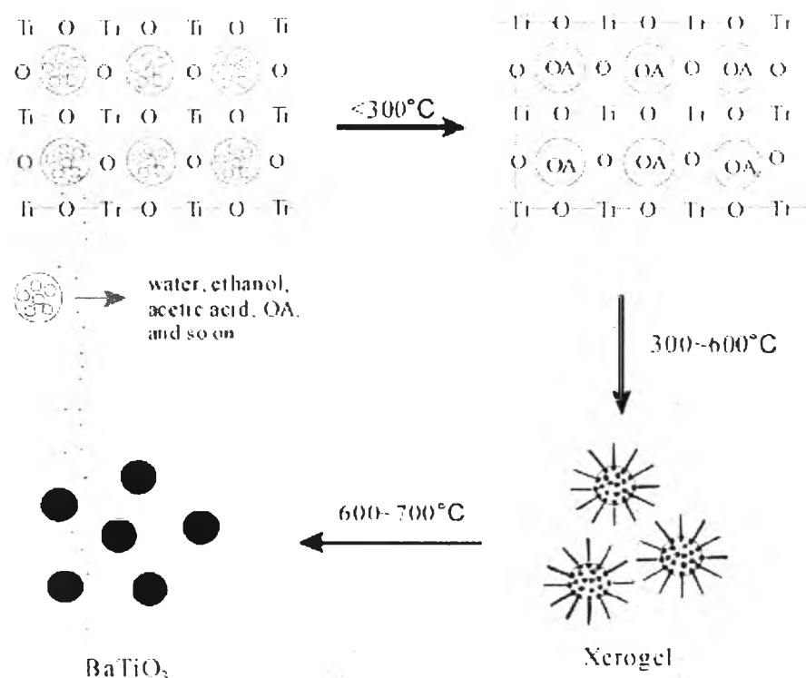
Figure 2.15 A schematic of forming the BaTiO 3 nanoparticles (Yu et al. , 2008).
