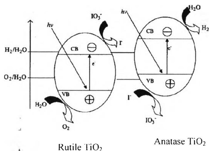
Figure 2.12 Photocatalytic hydrogen production over anatase/rutile \text{TiO}_2 under the mediation of \text{I}^-/\text{IO}_3^- .
