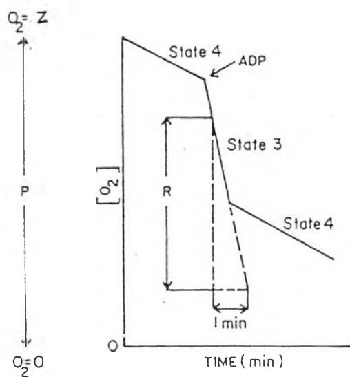
Figure 13. An oxygraph tracing illustrating the measurement of oxygen consumption rates.
