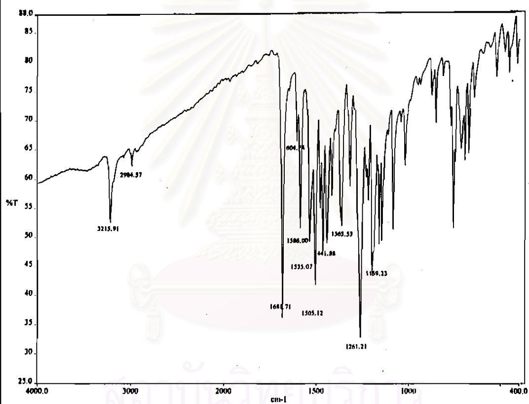
Figure 4-7 FT-IR spectrum of ethyl-2-aminobenzoate-2-nitrophenyl azo
