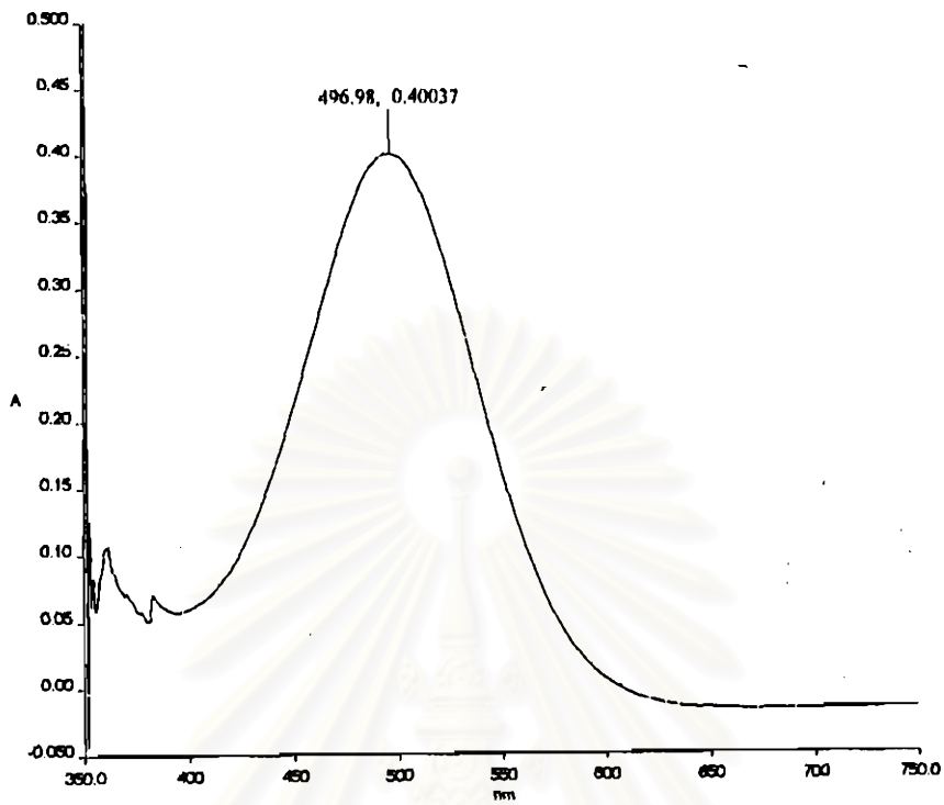
Figure 4-69 Maximum wavelength of ethyl-2-aminobenzoate-4-nitrophenyl azo
