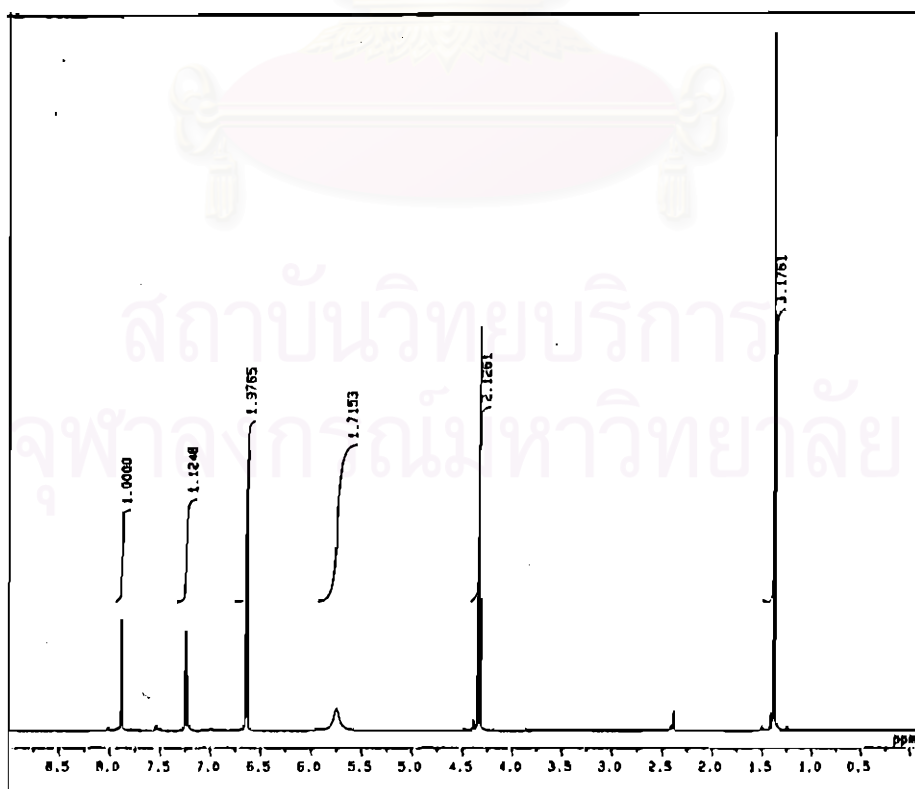
Figure 4-36 ^1\text{H-NMR} spectrum of ethyl-2-aminobenzoate-4-methylphenyl azo
