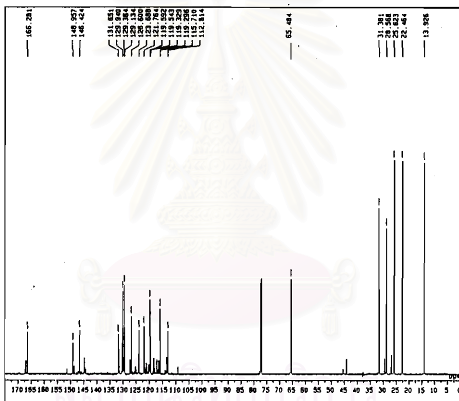
Figure 4-42 ^{13}\text{C} -NMR spectrum of hexyl-3-aminobenzoate-3-nitrophenyl azo
