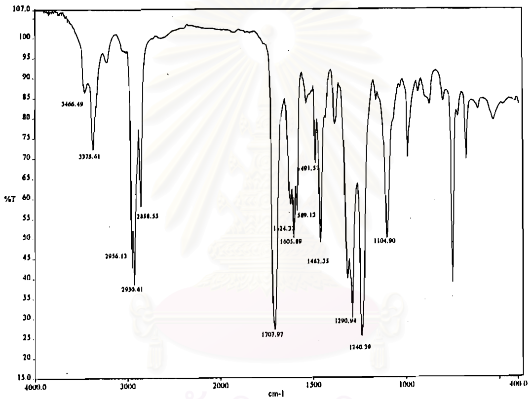
Figure 4-1 FT-IR spectrum of hexyl-3-aminobenzoate
