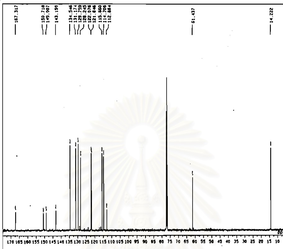
Figure 4-11 ^{13}\text{C} -NMR spectrum of ethyl-2-aminobenzoate-3-nitrophenyl azo
