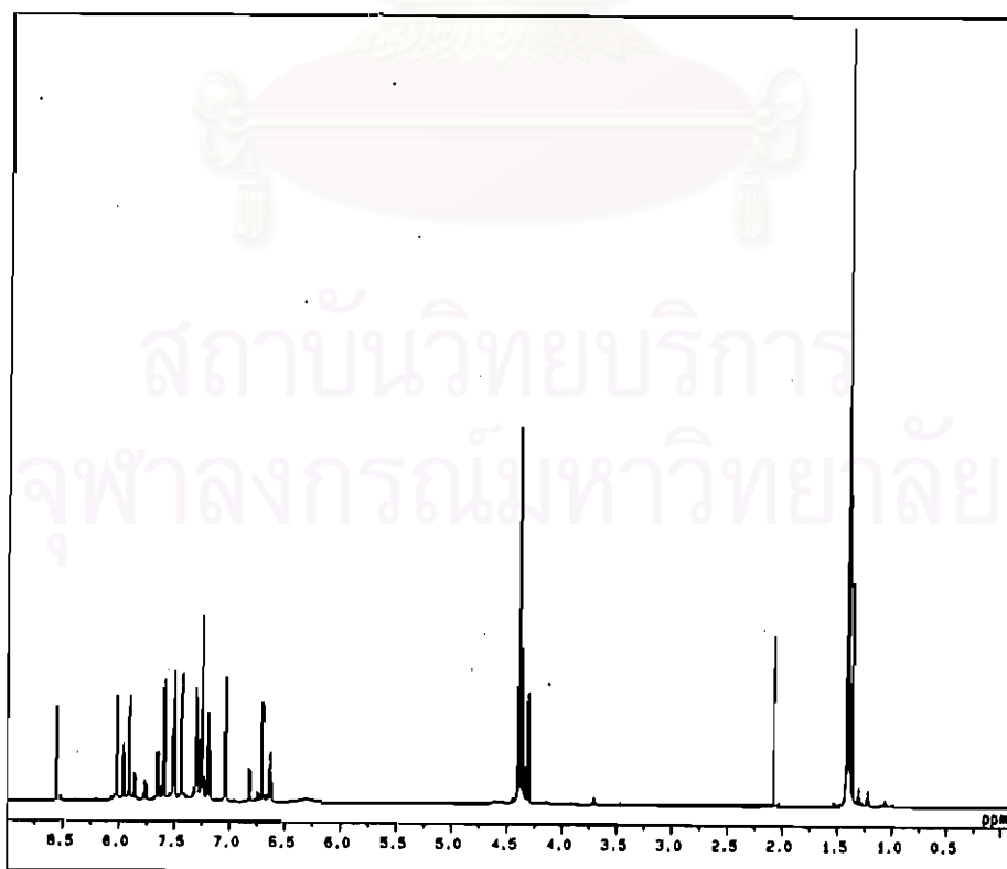
Figure 4-18 ^1\text{H} -NMR spectrum of ethyl-2-aminobenzoate-2-chlorophenyl azo
