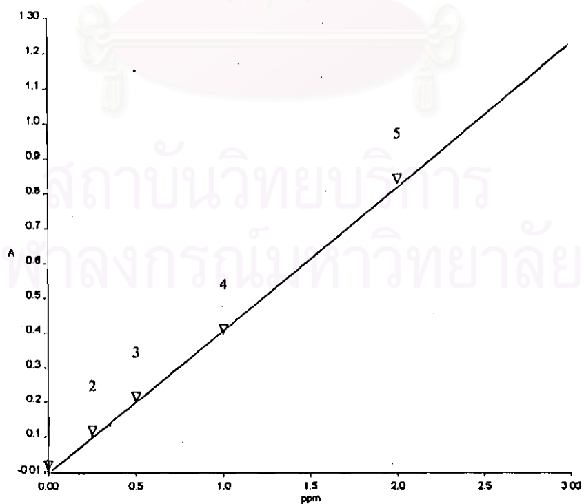
Figure 4-72 Calibration curve of ethyl-2-aminobenzoate-2-chloro-4-nitrophenyl azo
