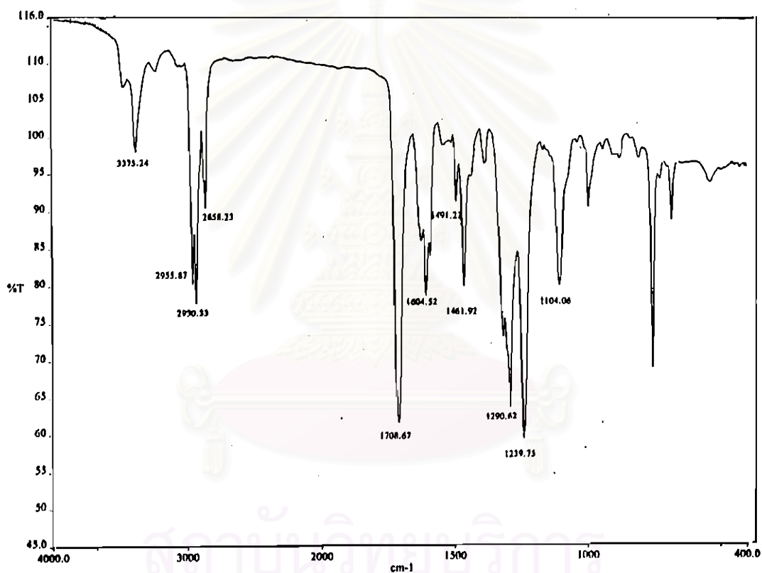
Figure 4-37 FT-IR spectrum of hexyl-3-aminobenzoate phenyl azo
