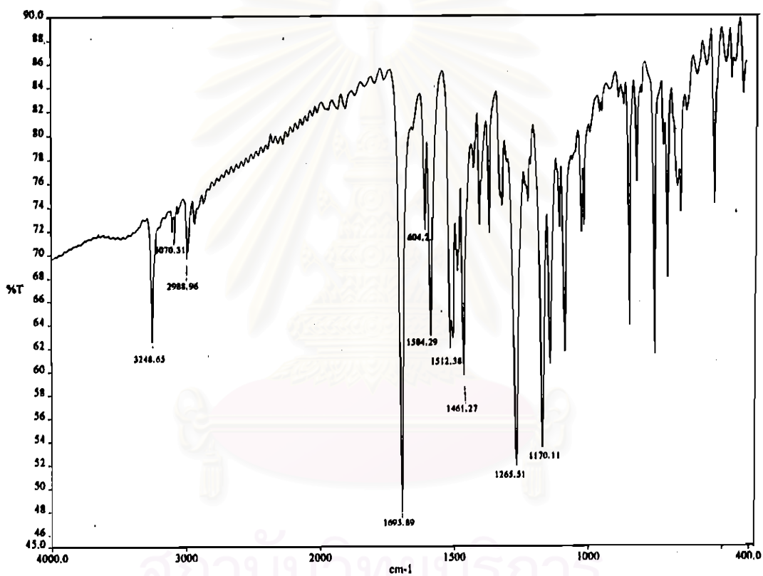
Figure 4-16 FT-IR spectrum of ethyl-2-aminobenzoate-2-chlorophenyl azo
