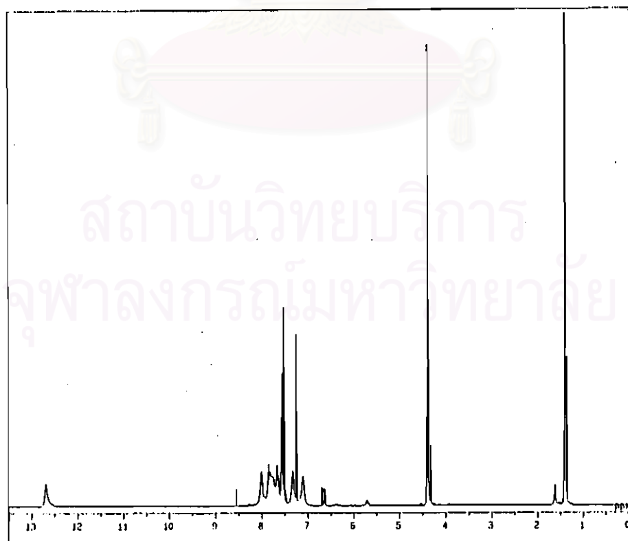
Figure 4-9 ^1\text{H} -NMR spectrum of ethyl-2-aminobenzoate-2-nitrophenyl azo
