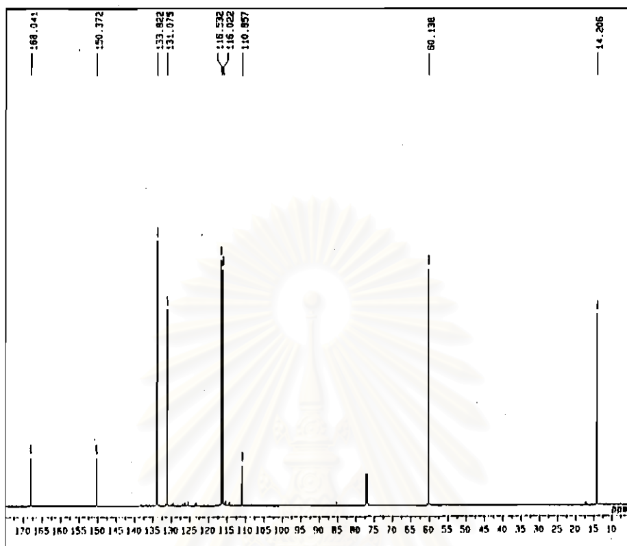
Figure 4-29 ^{13}\text{C} -NMR spectrum of ethyl-2-aminobenzoate-2-methylphenyl azo
