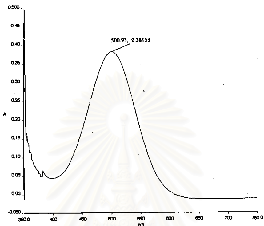
Figure 4-71 Maximum wavelength of ethyl-2-aminobenzoate-2-chloro-4-nitrophenyl azo
