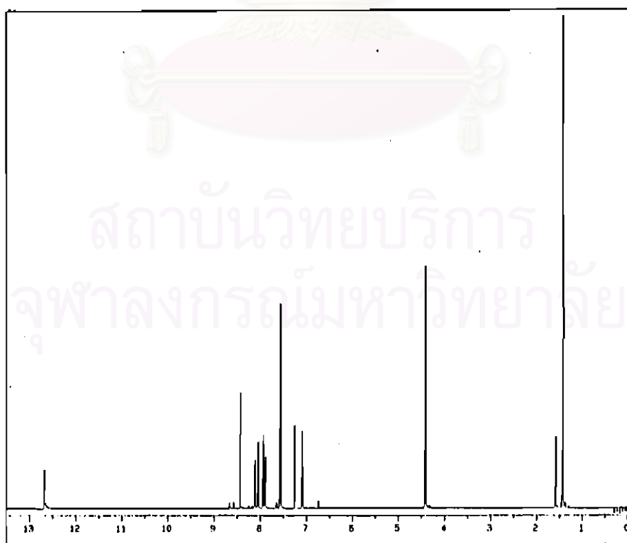
Figure 4-12 ^1\text{H} -NMR spectrum of ethyl-2-aminobenzoate-3-nitrophenyl azo
