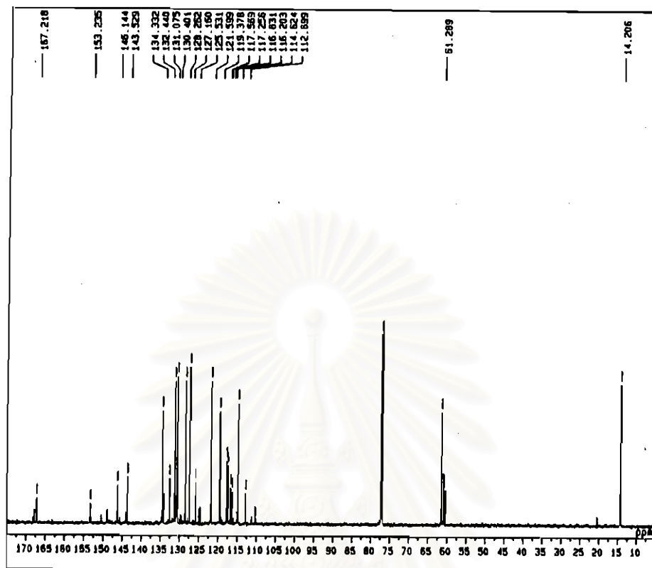
Figure 4-17 ^{13}\text{C} -NMR spectrum of ethyl-2-aminobenzoate-2-chlorophenyl azo
