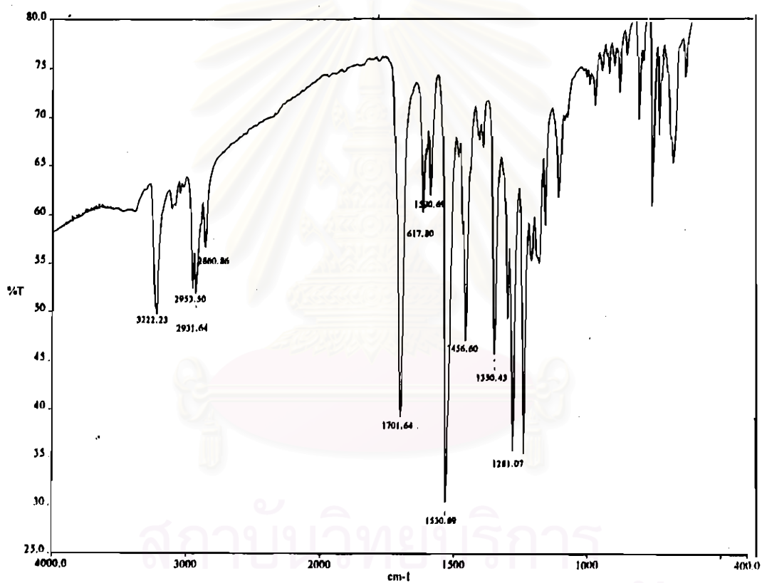
Figure 4-41 FT-IR spectrum of hexyl-3-aminobenzoate-3-nitrophenyl azo
