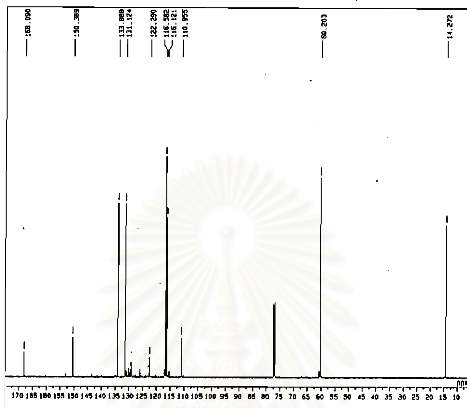
Figure 4-5 ^{13}\text{C} -NMR spectrum of ethyl-2-aminobenzoate phenyl azo
