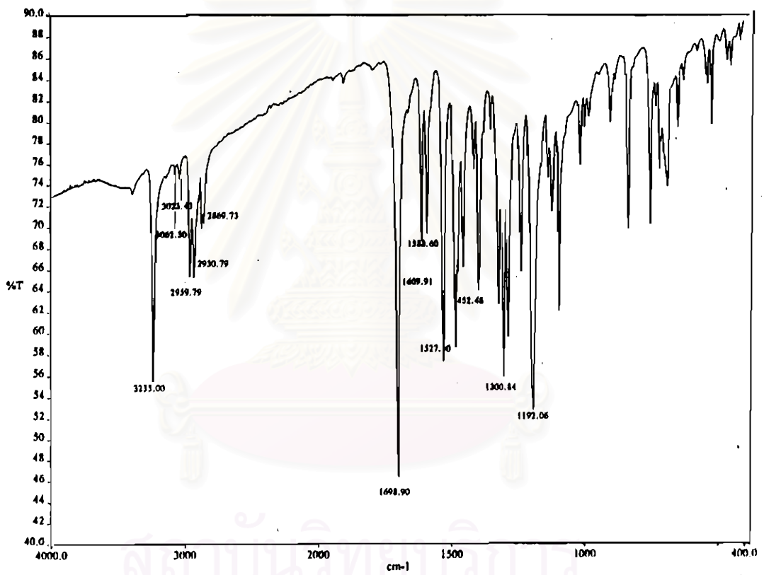
Figure 4-49 FT-IR spectrum of hexyl-3-aminobenzoate-4-chlorophenyl azo
