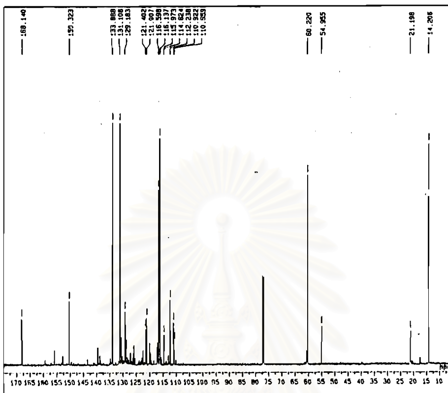
Figure 4-32 ^{13}\text{C} -NMR spectrum of ethyl-2-aminobenzoate-3-methylphenyl azo
