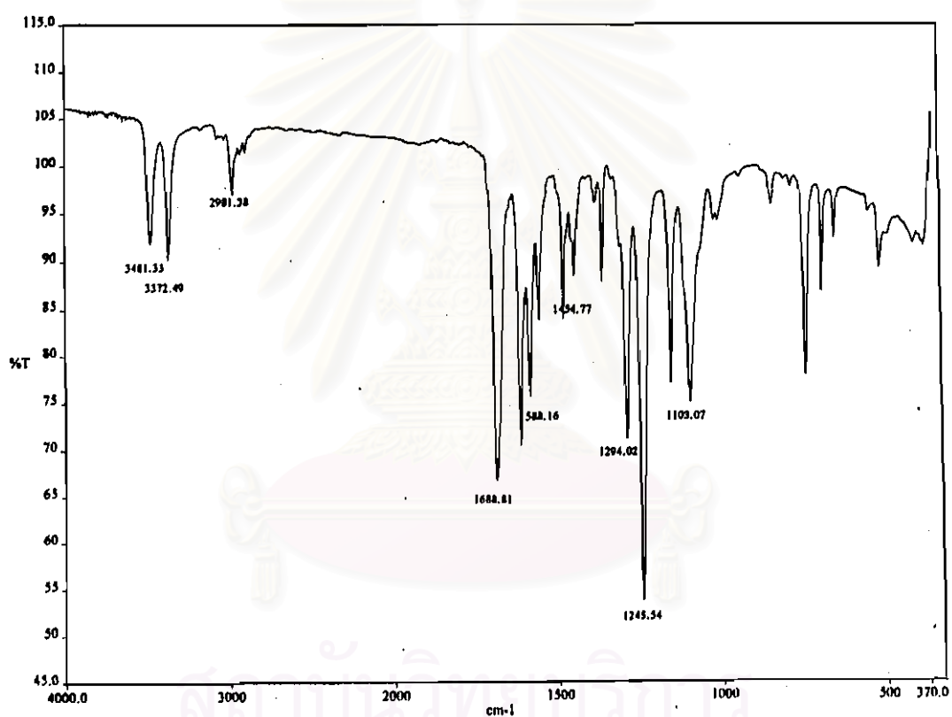
Figure 4-28 FT-IR spectrum of ethyl-2-aminobenzoate-2-methylphenyl azo
