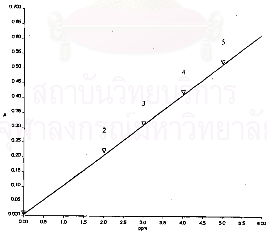
Figure 4-68 Calibration curve of ethyl-2-aminobenzoate-2-nitrophenyl azo
