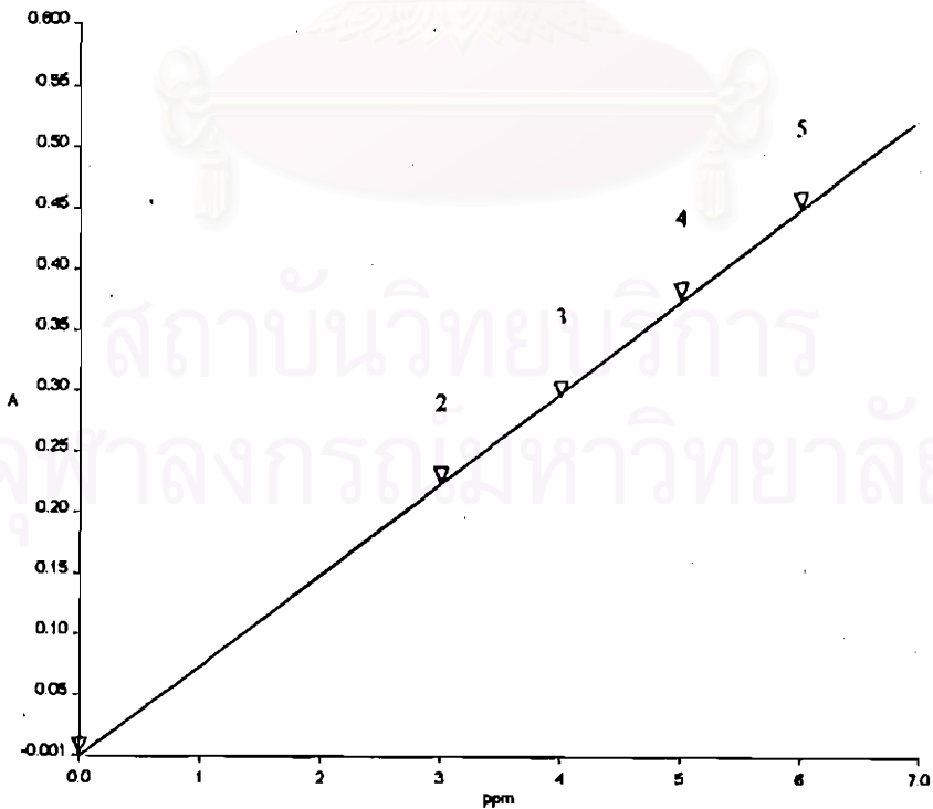
Figure 4-78 Calibration curve of hexyl-3-aminobenzoate-2-chloro-4-nitrophenyl azo
