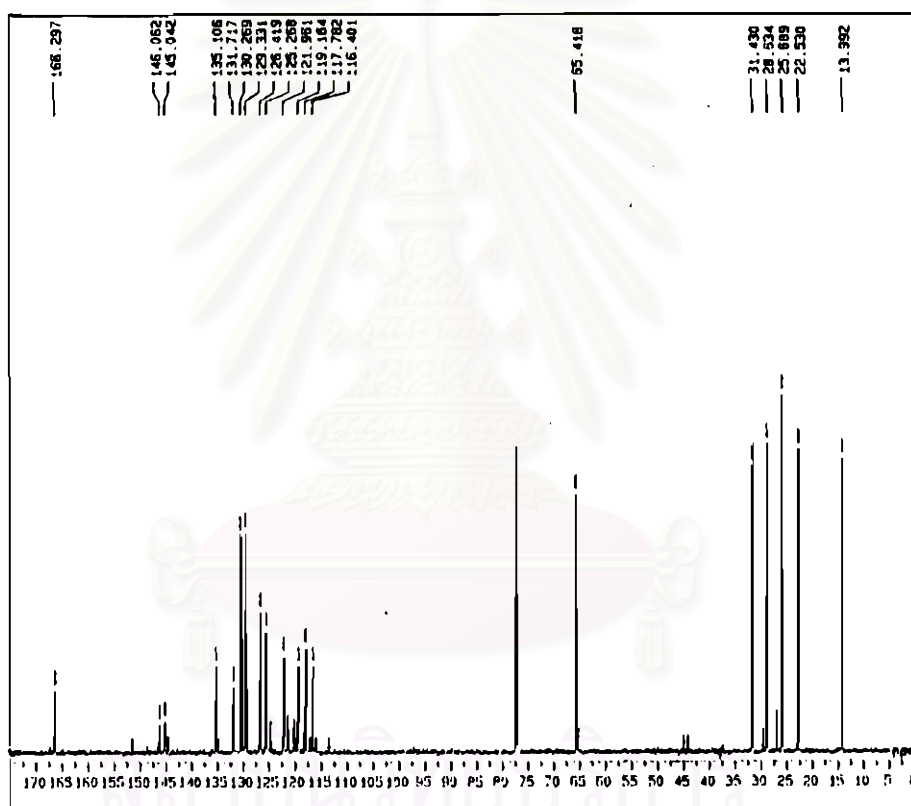
Figure 4-48 ^{13}\text{C} -NMR spectrum of hexyl-3-aminobenzoate-3-chlorophenyl azo
