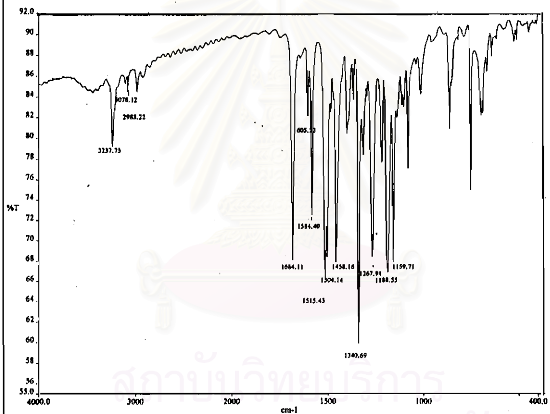
Figure 4-13 FT-IR spectrum of ethyl-2-aminobenzoate-4-nitrophenyl azo
