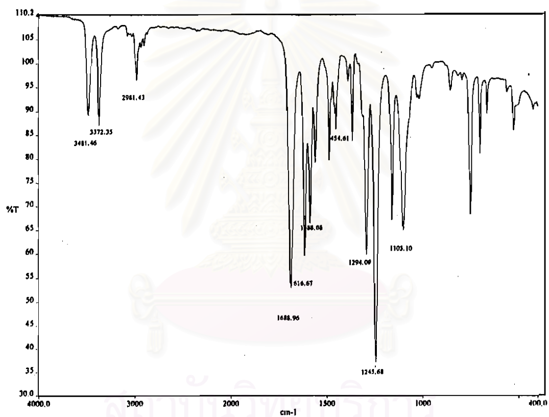
Figure 4-34 FT-IR spectrum of ethyl-2-aminobenzoate-4-methylphenyl azo
