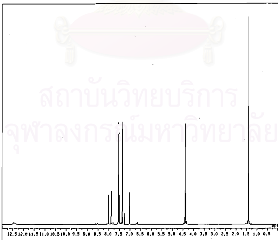
Figure 4-24 ^1\text{H} -NMR spectrum of ethyl-2-aminobenzoate-4-chlorophenyl azo
