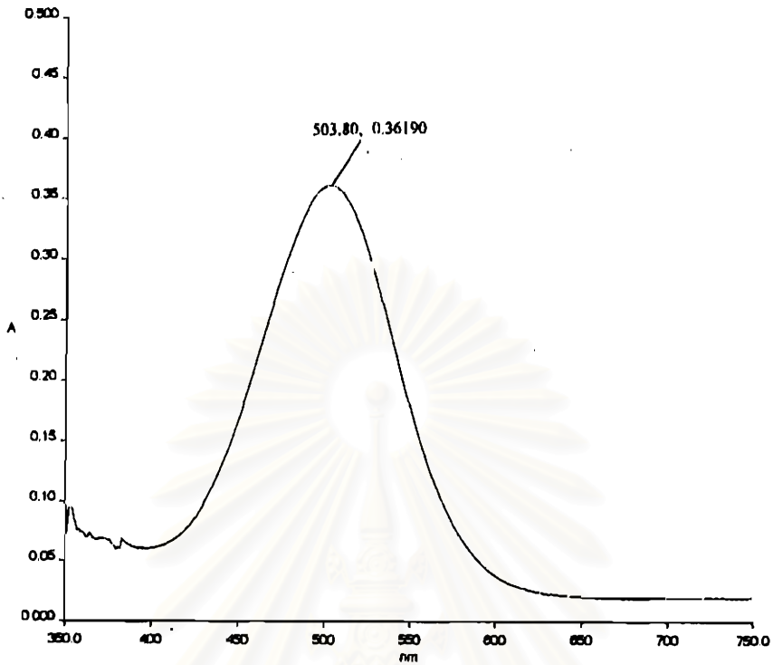
Figure 4-77 Maximum wavelength of hexyl-3-aminobenzoate-2-chloro-4-nitrophenyl azo
