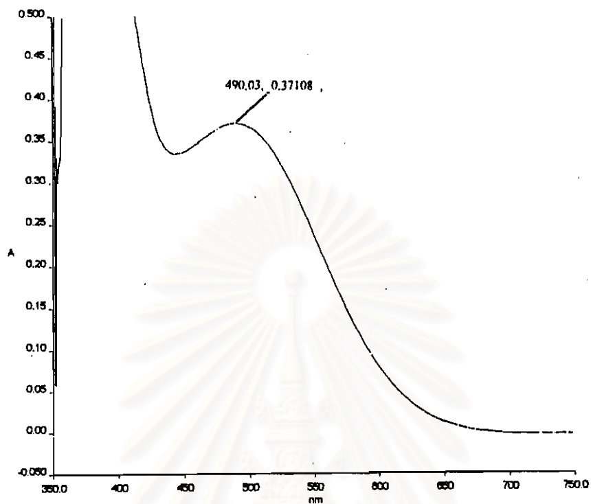
Figure 4-67 Maximum wavelength of ethyl-2-aminobenzoate-2-nitrophenyl azo
