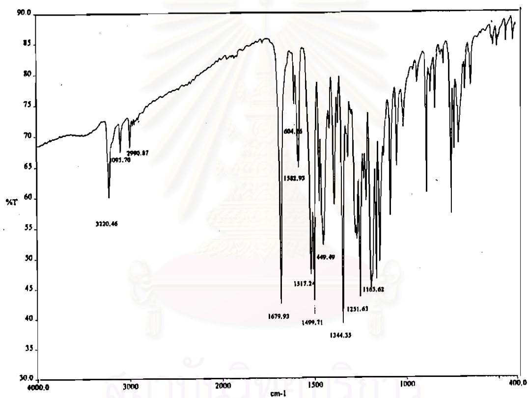
Figure 4-25 FT-IR spectrum of ethyl-2-aminobenzoate-2-chloro-4-nitrophenyl azo
