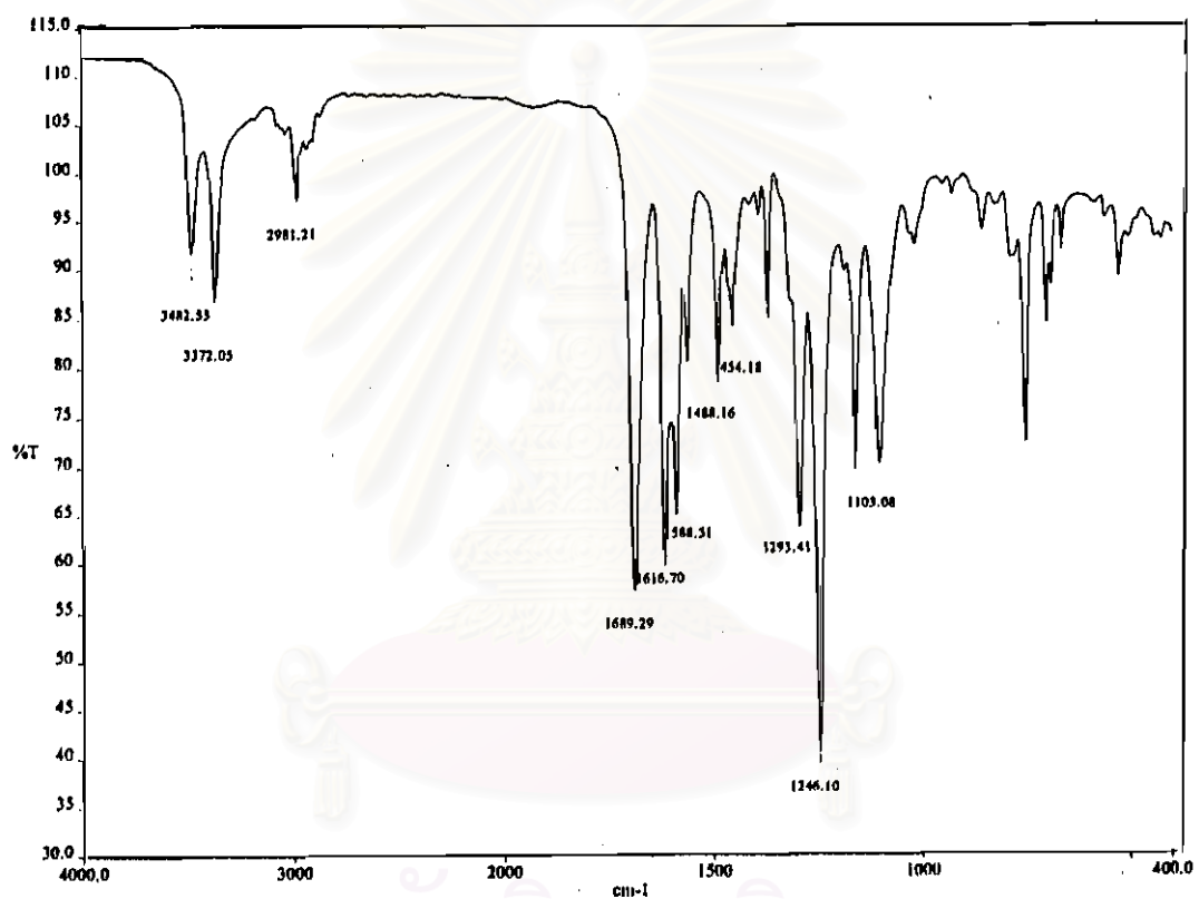
Figure 4-31 FT-IR spectrum of ethyl-2-aminobenzoate-3-methylphenyl azo
