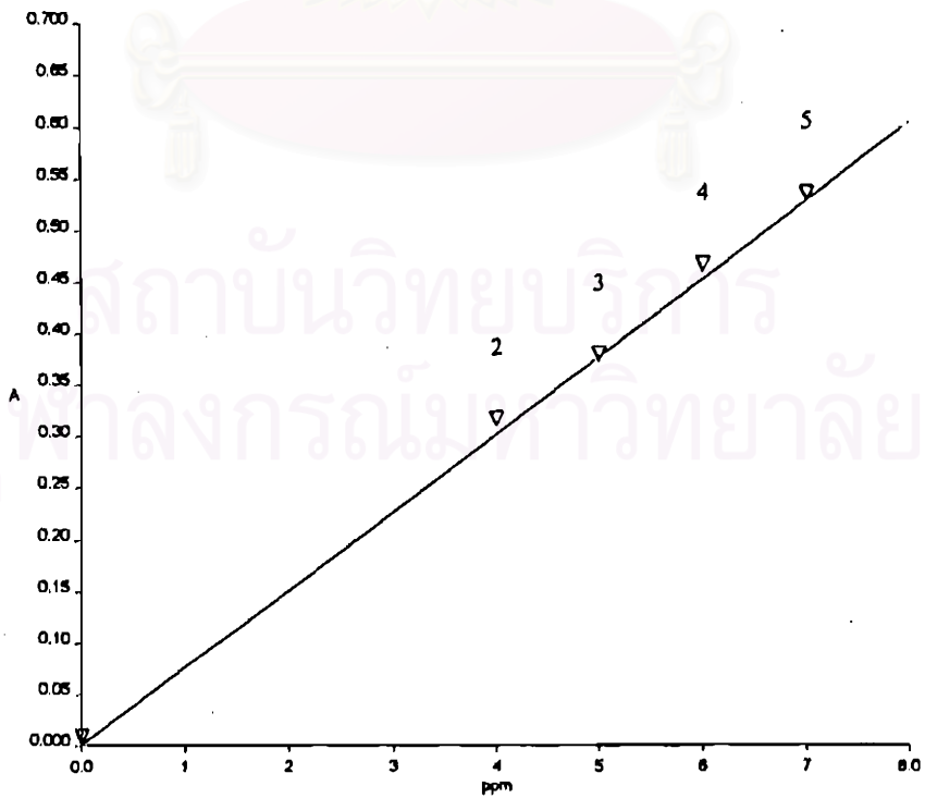
Figure 4-74 Calibration curve of hexyl-3-aminobenzoate-2-nitrophenyl azo
