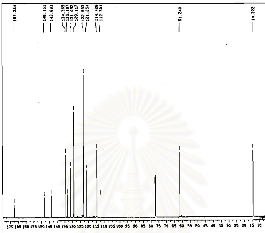
Figure 4-23 ^{13}\text{C} -NMR spectrum of ethyl-2-aminobenzoate-4-chlorophenyl azo
