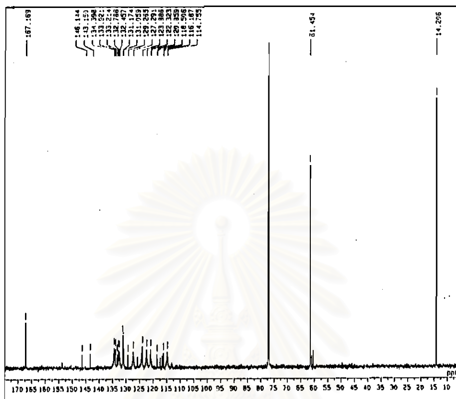
Figure 4-8 ^{13}\text{C} -NMR spectrum of ethyl-2-aminobenzoate-2-nitrophenyl azo
