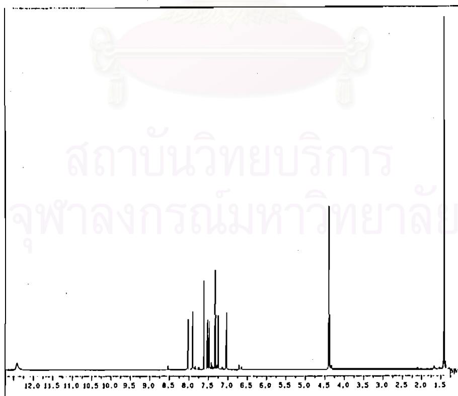
Figure 4-21 ^1\text{H} -NMR spectrum of ethyl-2-aminobenzoate-3-chlorophenyl azo
