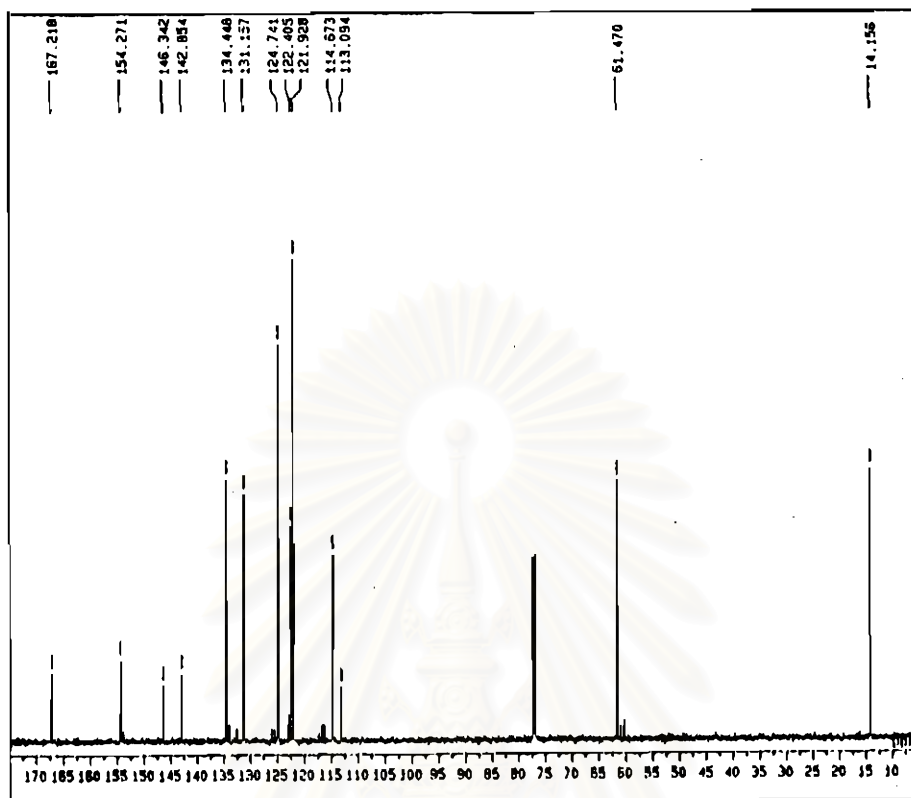
Figure 4-14 ^{13}\text{C} -NMR spectrum of ethyl-2-aminobenzoate-4-nitrophenyl azo
