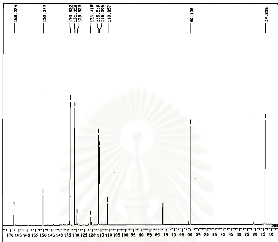
Figure 4-35 ^{13}\text{C-NMR} spectrum of ethyl-2-aminobenzoate-4-methylphenyl azo
