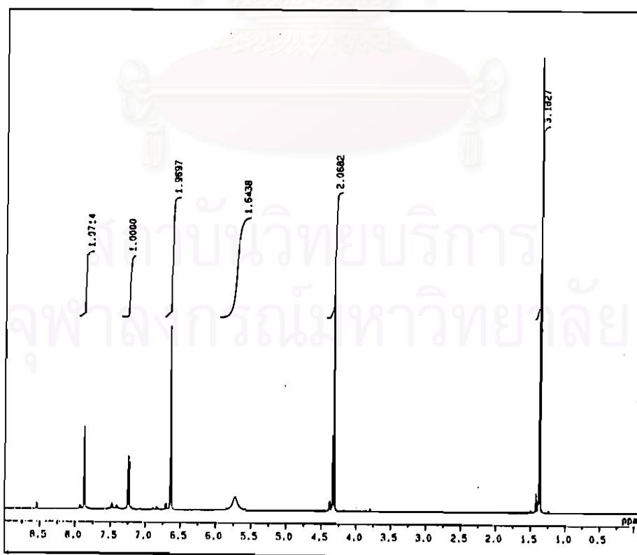
Figure 4-6 ^1\text{H} -NMR spectrum of ethyl-2-aminobenzoate phenyl azo
