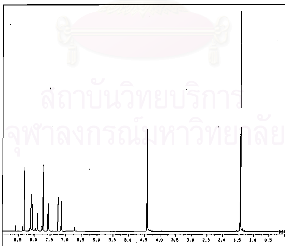
Figure 4-27 ^1\text{H} -NMR spectrum of ethyl-2-aminobenzoate-2-chloro-4-nitrophenyl azo
