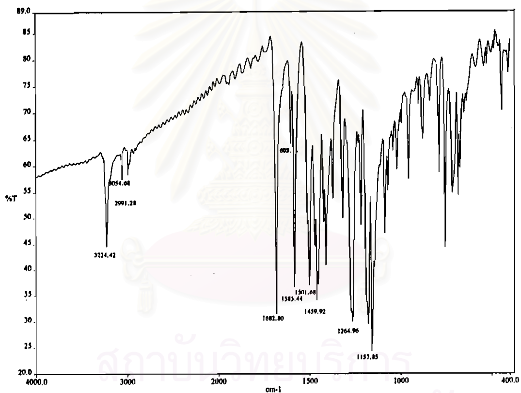
Figure 4-19 FT-IR spectrum of ethyl-2-aminobenzoate-3-chlorophenyl azo
