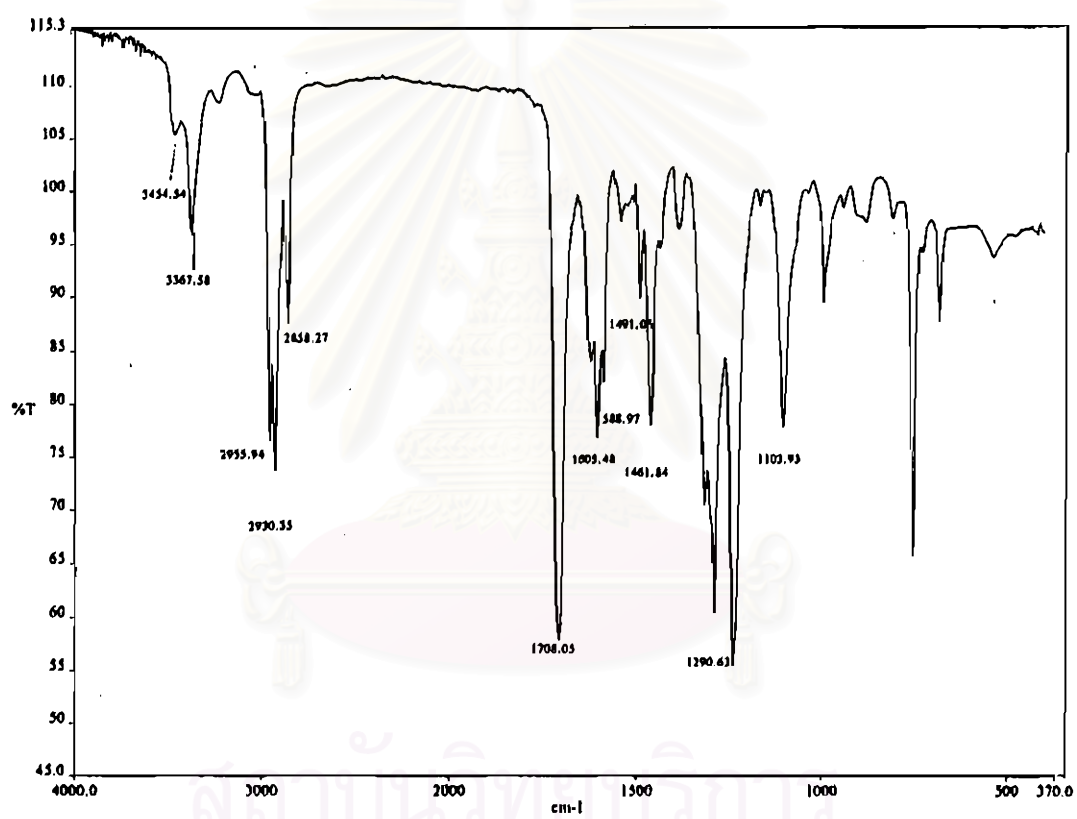
Figure 4-53 FT-IR spectrum of hexyl-3-aminobenzoate-2-methylphenyl azo
