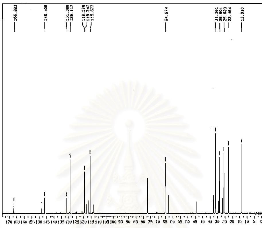
Figure 4-2 ^{13}\text{C} -NMR spectrum of hexyl-3-aminobenzoate
