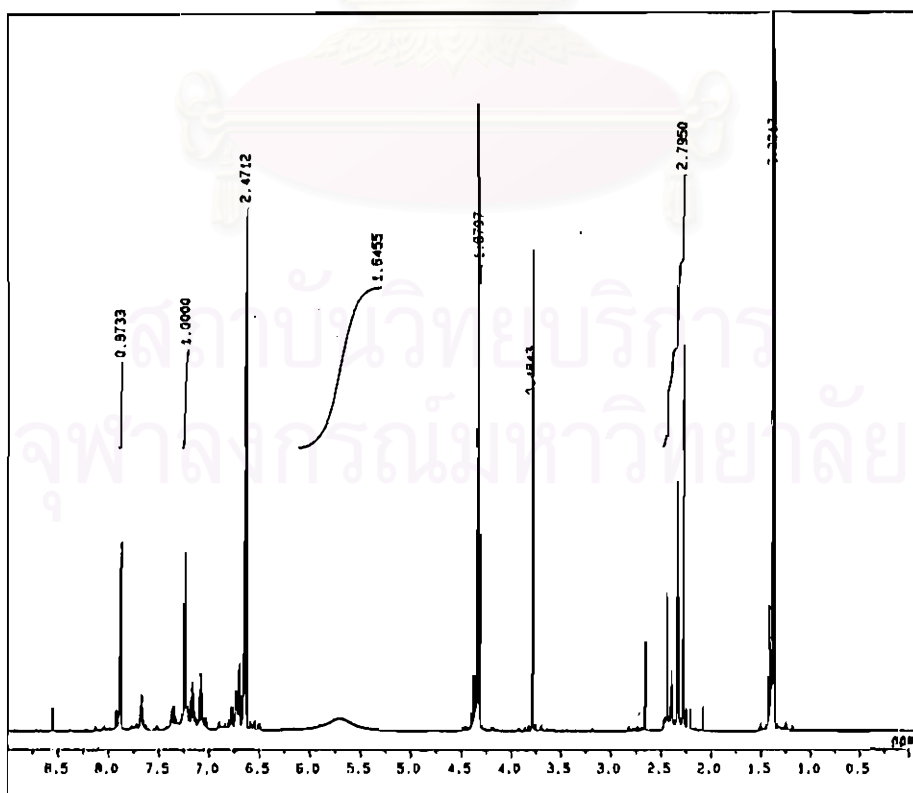
Figure 4-33 ^1\text{H} -NMR spectrum of ethyl-2-aminobenzoate-3-methylphenyl azo
