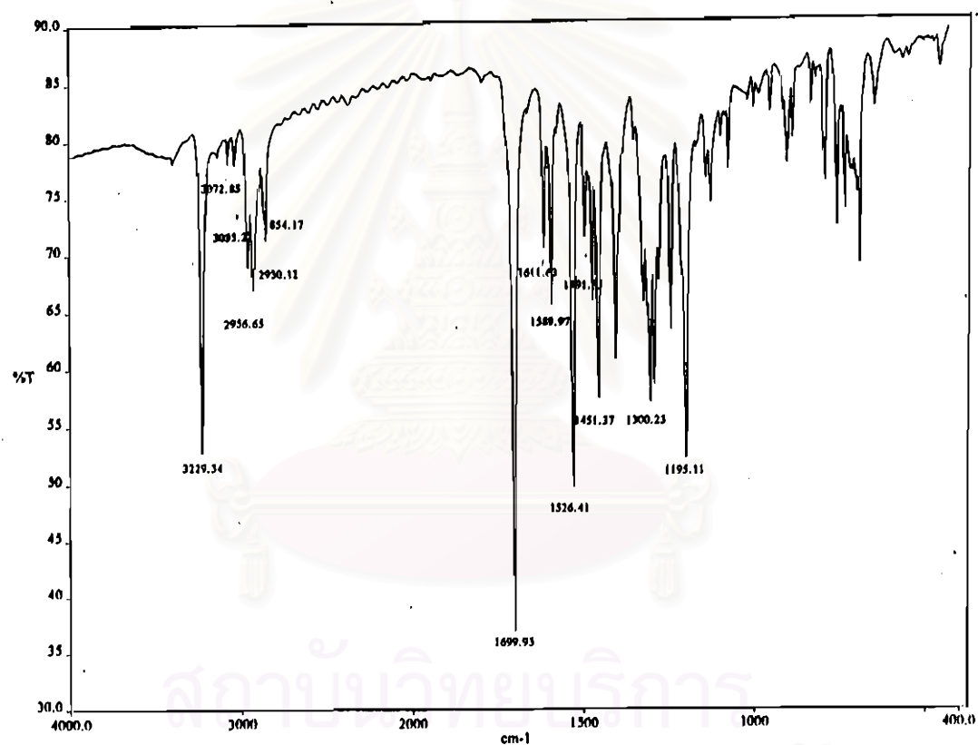
Figure 4-47 FT-IR spectrum of hexyl-3-aminobenzoate-3-chlorophenyl azo
