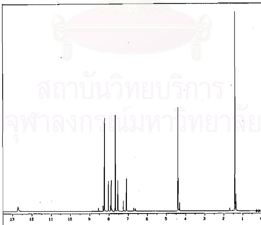
Figure 4-15 ^1\text{H} -NMR spectrum of ethyl-2-aminobenzoate-4-nitrophenyl azo
