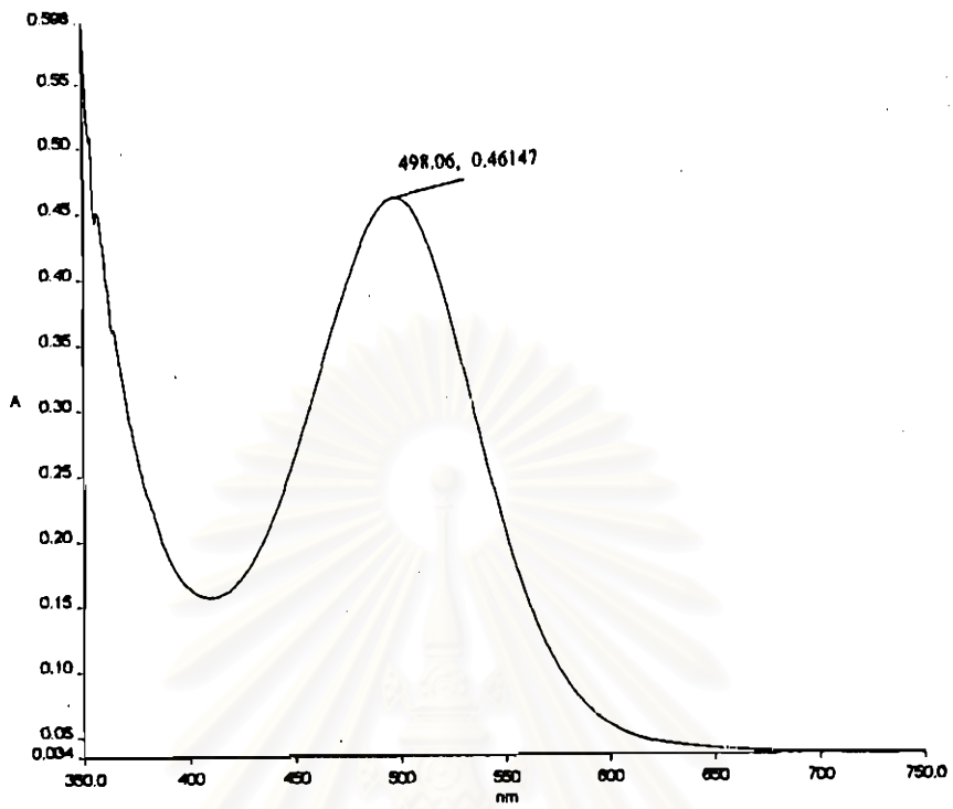
Figure 4-75 Maximum wavelength of hexyl-3-aminobenzoate-4-nitrophenyl azo
