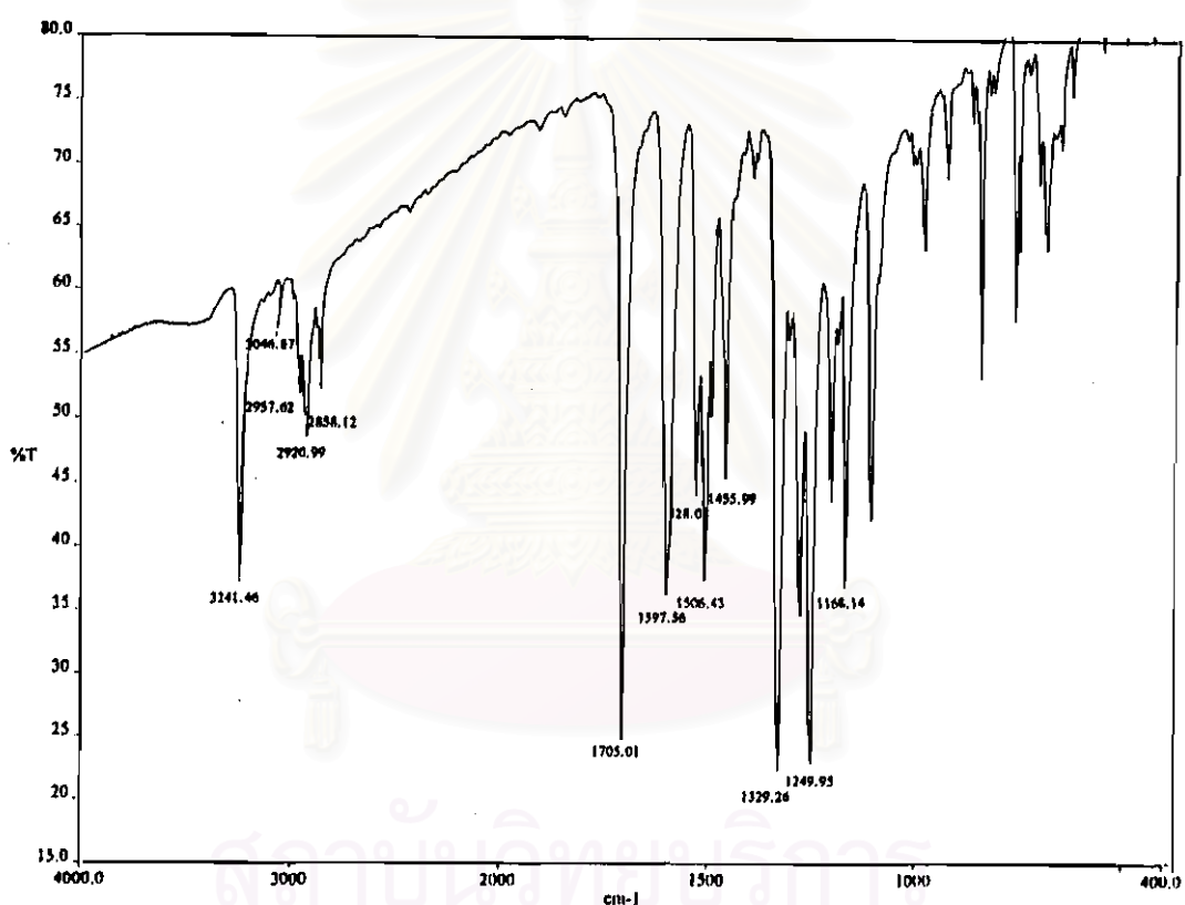
Figure 4-43 FT-IR spectrum of hexyl-3-aminobenzoate-4-nitrophenyl azo
