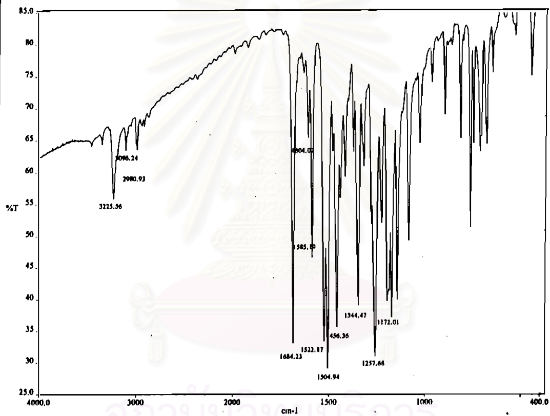
Figure 4-10 FT-IR spectrum of ethyl-2-aminobenzoate-3-nitrophenyl azo
