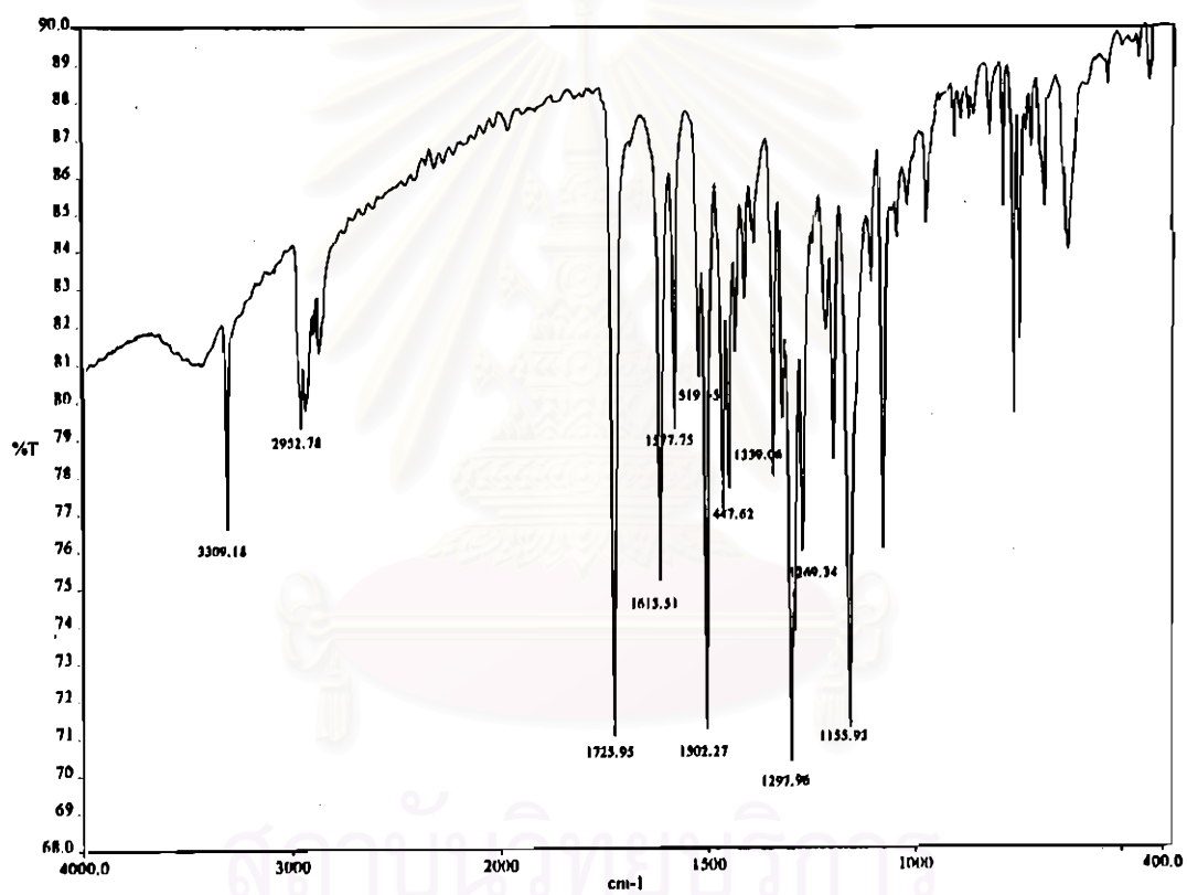
Figure 4-39 FT-IR spectrum of hexyl-3-aminobenzoate-2-nitrophenyl azo
