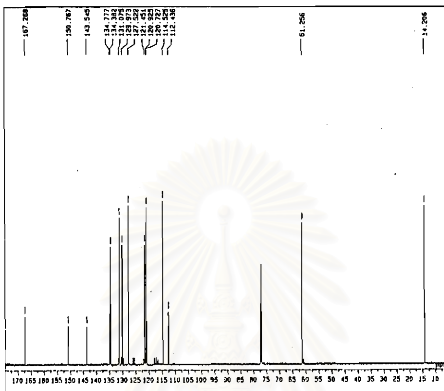
Figure 4-20 ^{13}\text{C} -NMR spectrum of ethyl-2-aminobenzoate-3-chlorophenyl azo
