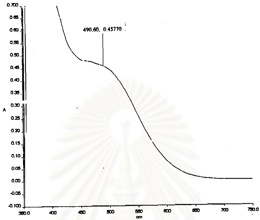
Figure 4-73 Maximum wavelength of hexyl-3-aminobenzoate-2-nitrophenyl azo
