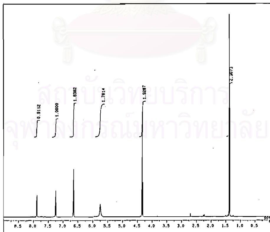
Figure 4-30 ^1\text{H} -NMR spectrum of ethyl-2-aminobenzoate-2-methylphenyl azo
