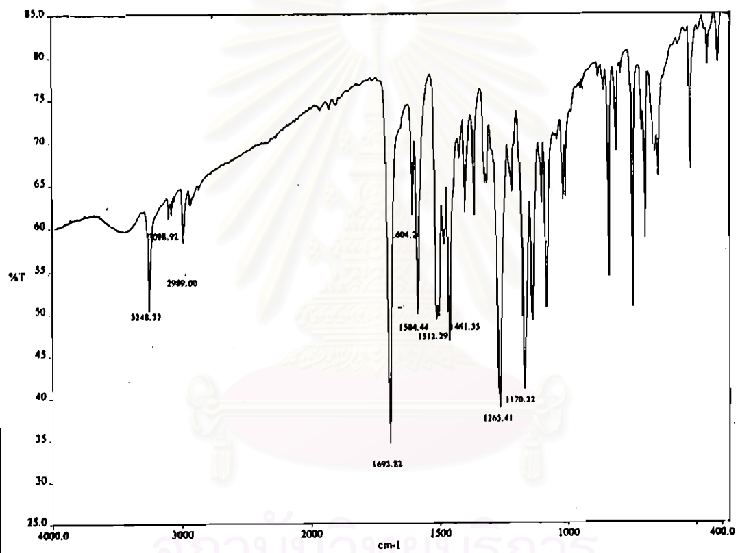
Figure 4-22 FT-IR spectrum of ethyl-2-aminobenzoate-4-chlorophenyl azo
