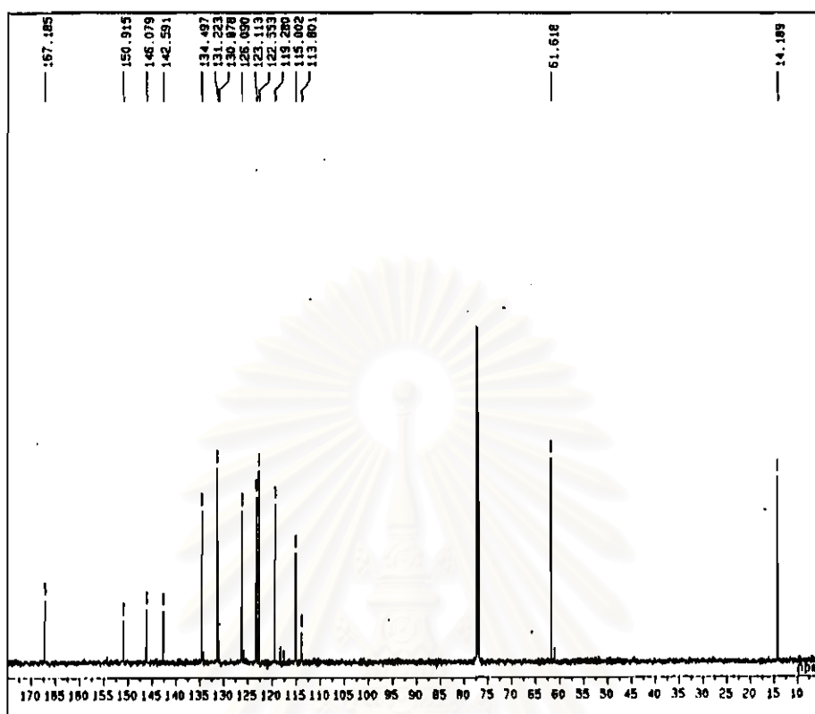
Figure 4-26 ^{13}\text{C} -NMR spectrum of ethyl-2-aminobenzoate-2-chloro-4-nitrophenyl azo
