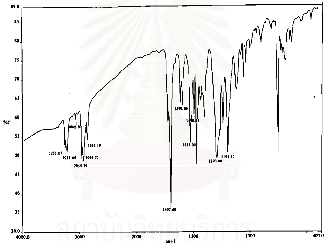
Figure 4-45 FT-IR spectrum of hexyl-3-aminobenzoate-2-chlorophenyl azo
