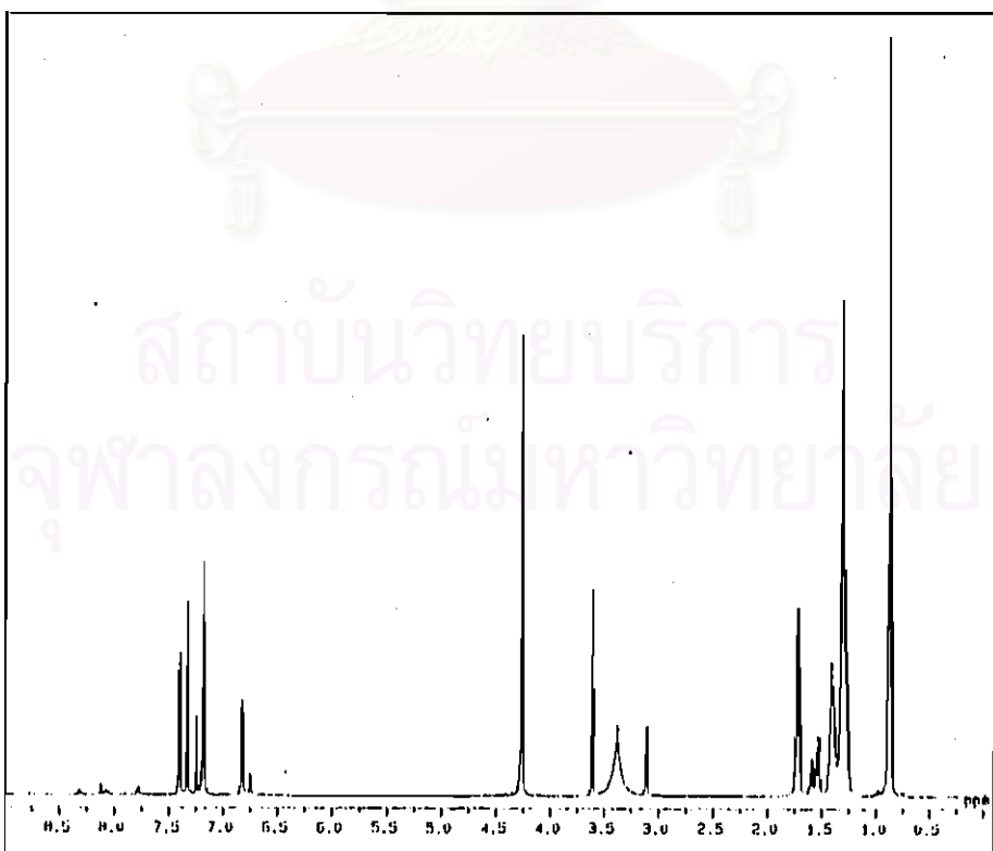
Figure 4-3 ^1\text{H} -NMR spectrum of hexyl-3-aminobenzoate
