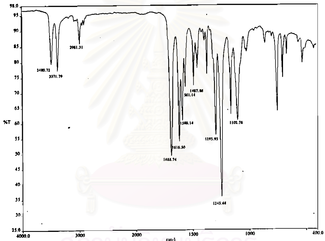
Figure 4-4 FT-IR spectrum of ethyl-2-aminobenzoate phenyl azo
