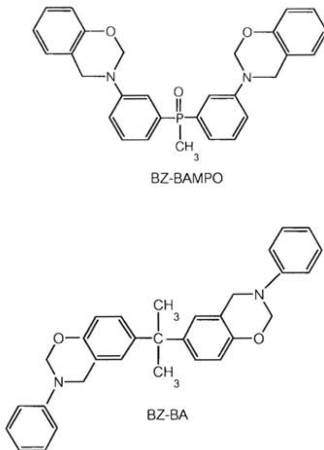
Figure 3.5 The structures of BZ-BAMPO and BZ-BA
