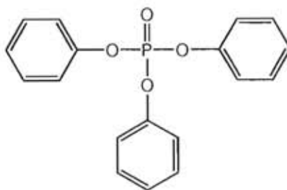
Figure 2.8 Structure of triphenylphosphate flame retardant.
