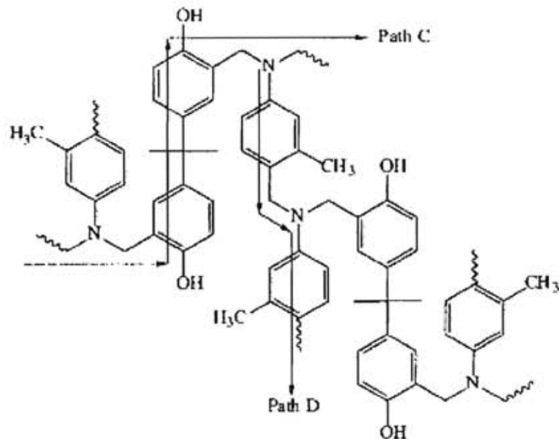
Figure 3.1 The arylamine Mannich bridge network formation
