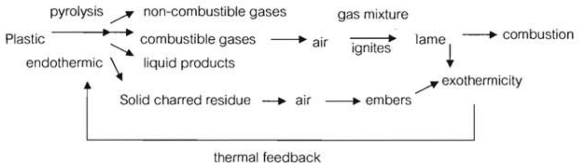
Figure 2.6 Combustion process [14].
