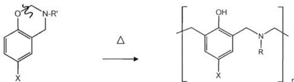
Figure 2.3 Polymerization of monofunctional benzoxazine monomer.
