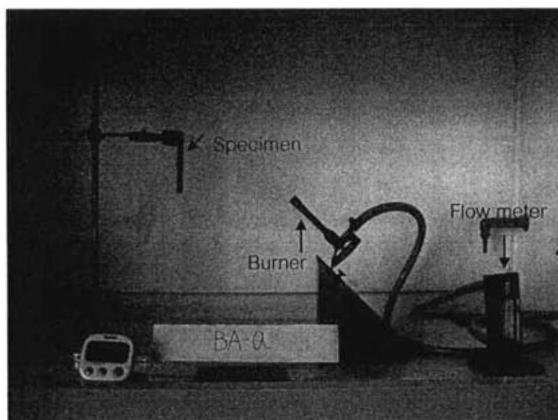
Figure 4.1 Vertical flame test.
