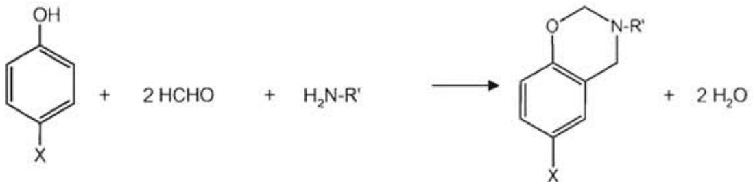
Figure 2.1 Synthesis of monofunctional benzoxazine monomer [11].
