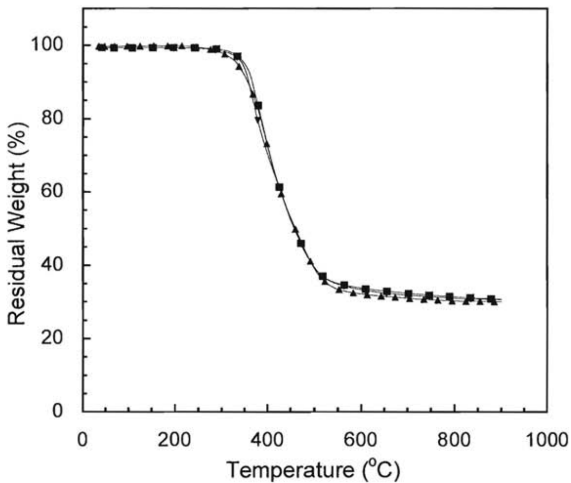
Figure 5.19 TGA thermograms of the neat arylamine-based polybenzoxazines:
