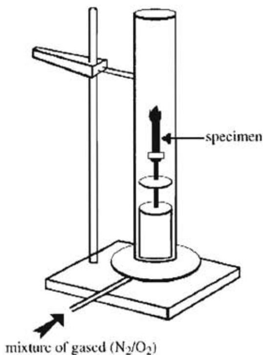
Figure 2.10 Experimental set-up for LOI measurement [9].
