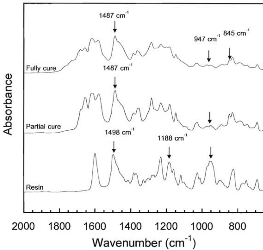
Figure 5.13 FTIR spectra of BA35x/TPP at 90:10 weight ratio.
