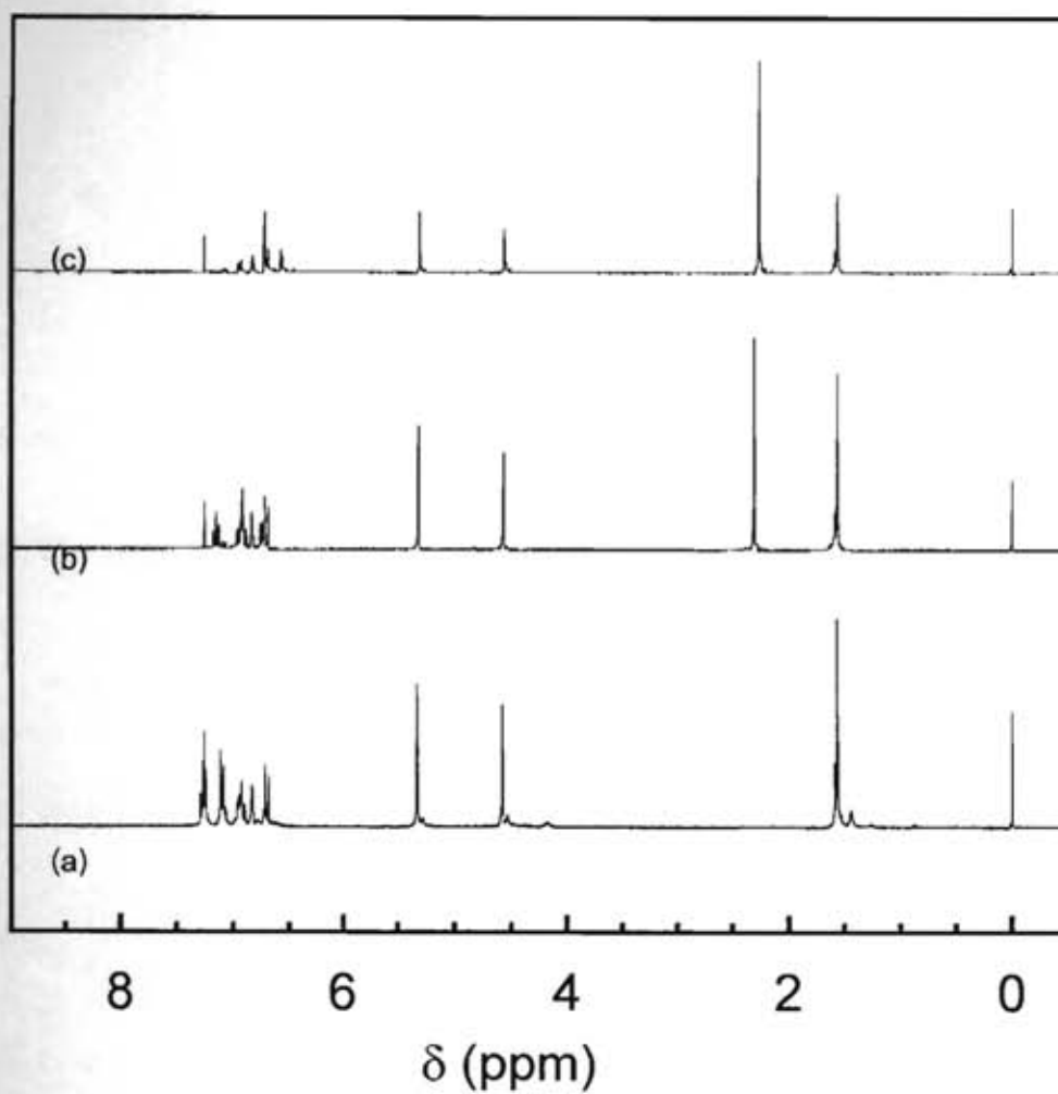
Figure 5.1 ^1\text{H} NMR spectra of the neat arylamine-based benzoxazine resins: (a) BA-a, (b) BA-mt, and (c) BA-35x.
