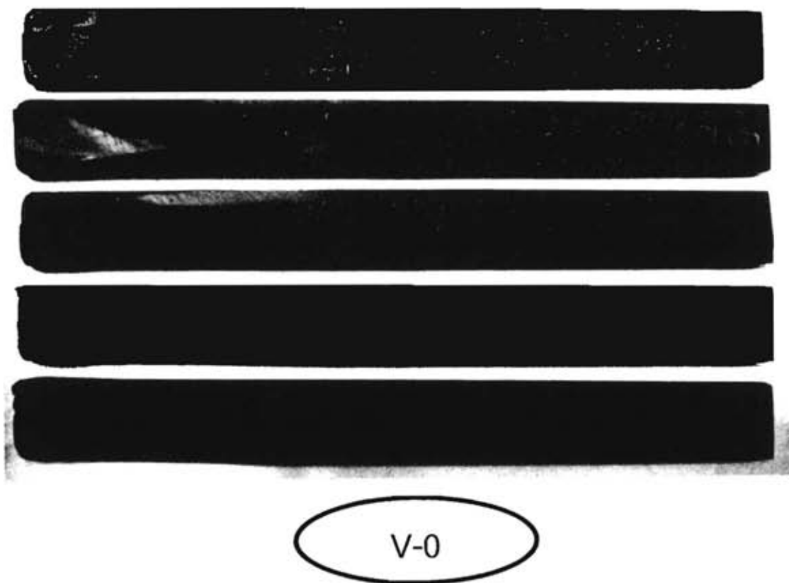
Figure 5.29 UL94 vertical test of BA-mt at 2 wt% TPP flame retardant.
