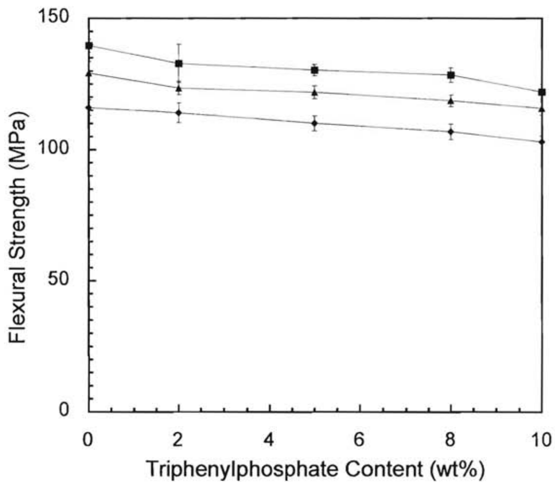
Figure 5.22 Flexural strength of arylamine-based polybenzoxazines at various TPP contents: (■) BA-a, (▲) BA-mt, and (◆) BA-35x.
