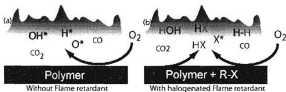
Figure 2.7 Mechanism of action of halogenated flame retardants [16].
