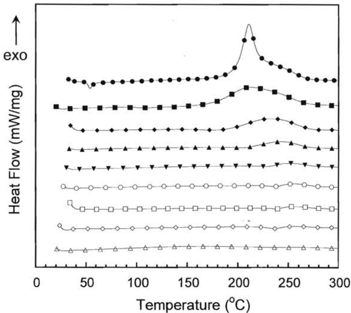
Figure 5.6 DSC thermograms of the neat BA-35x at various curing conditions:
