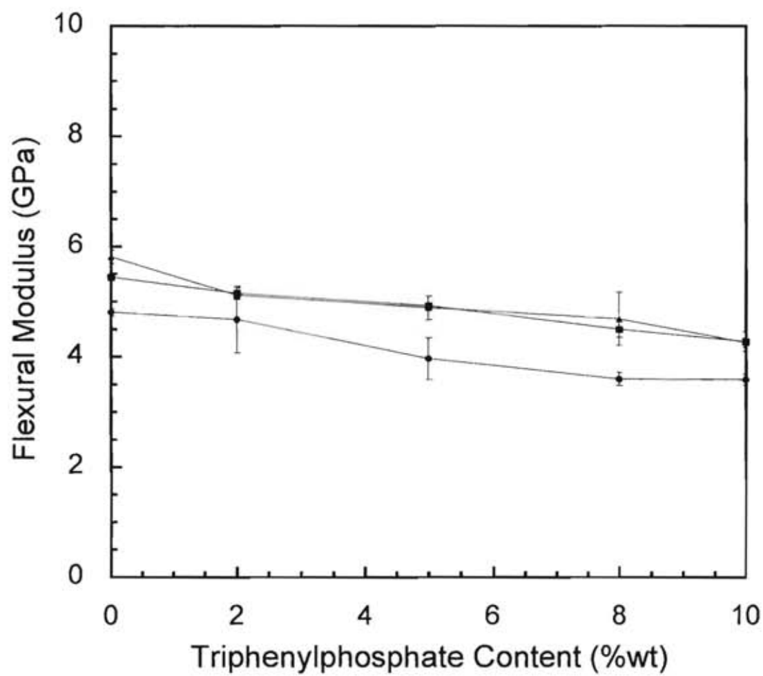
Figure 5.24 Flexural modulus of arylamine-based polybenzoxazines at various TPP contents: (■) BA-a, (▲) BA-mt, and (◆) BA-35x.
