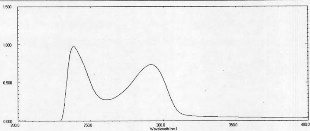
Figure B-3 The spectrum of TOC at 80 µg/ml and blank liposomes 1 mg/ml in chloroform:methanol (1:4)
