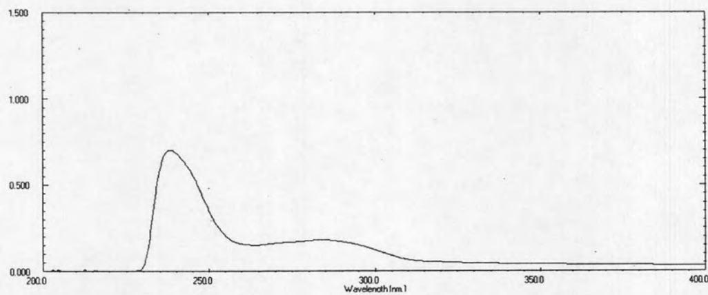
Figure B-2 The spectrum of blank liposomes 1 mg/ml in chloroform:methanol (1:4)
