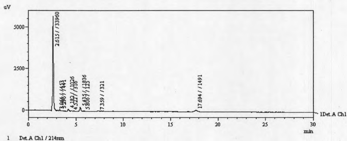
Figure B-6 HPLC chromatogram of blank liposomes 1 mg/ml in 1% Triton-X® 100
