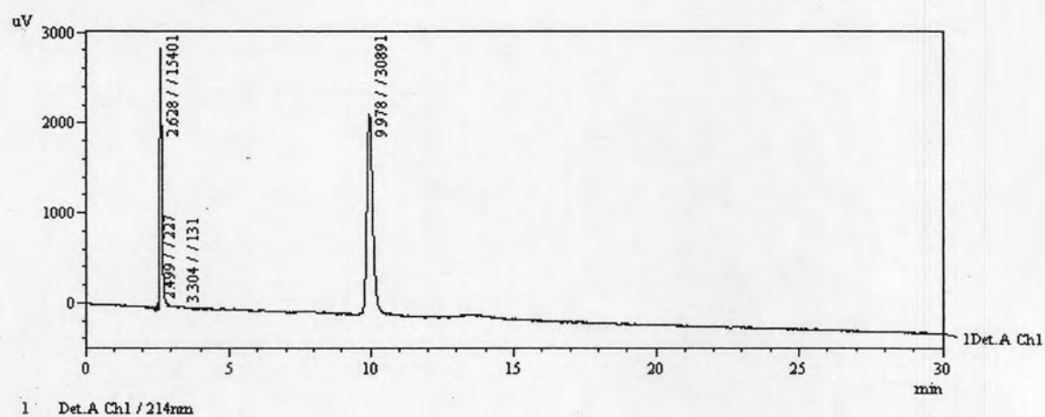
Figure B-5 HPLC chromatogram of NAC solution at 5 µg/ml
