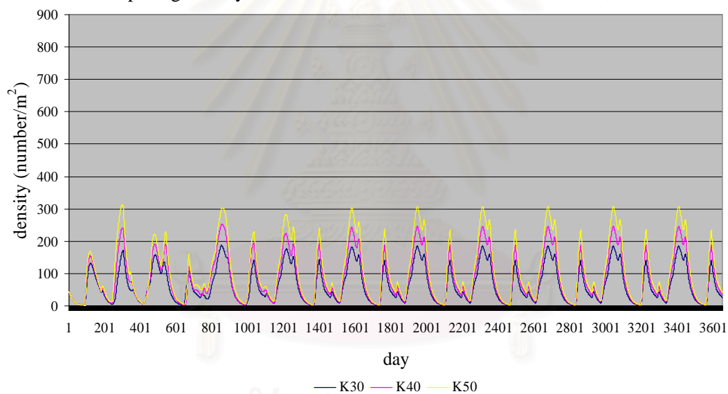
Comparing density of razor clam at M=0.04 , OS=35 , K=30, 40, 50
