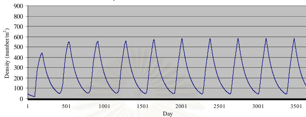
Density of razor clam at K=50 M=0.01 OS=25
