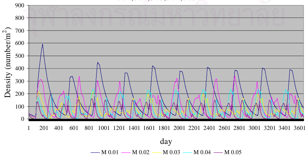
Comparing density of razor clam at K=30 OS=45 M=0.01,0.02,0.03,0.04,0.05
