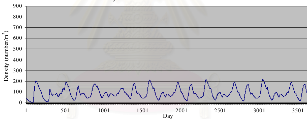
Density of razor clam at K=40 M=0.03 OS=35
