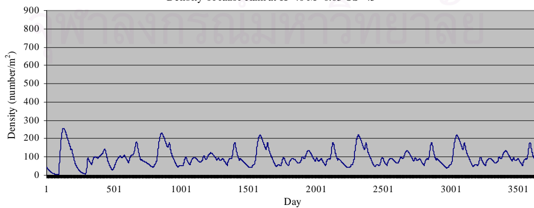
Density of razor clam at K=40 M=0.03 OS=45
