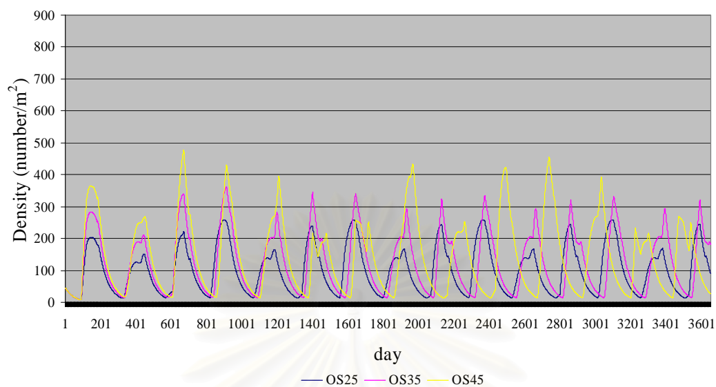
Comparing density of razor clam at K = 40 , M = 0.03 , OS = 25, 35, 45
