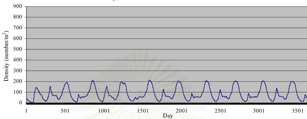
Density of razor clam at K=40 M=0.03 OS=25
