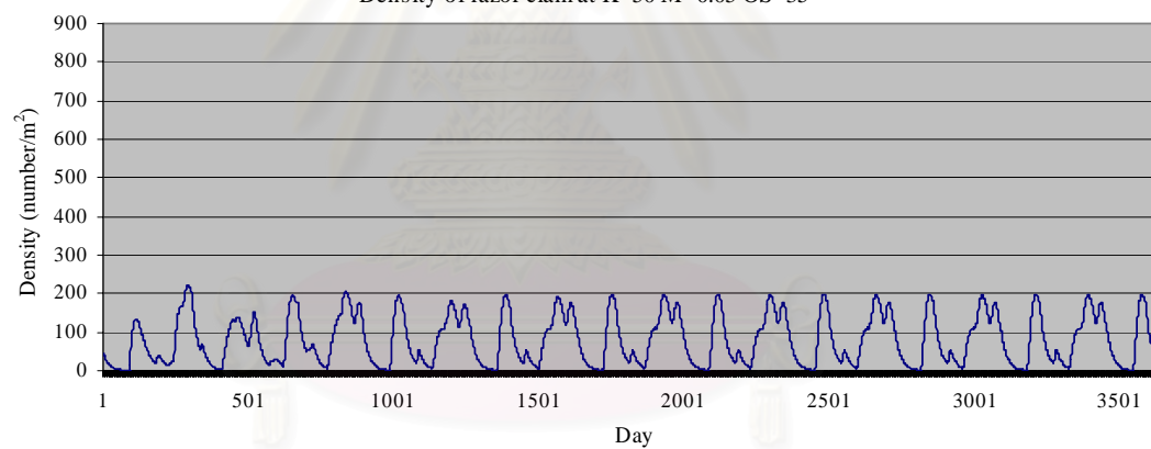
Density of razor clam at K=50 M=0.05 OS=35
