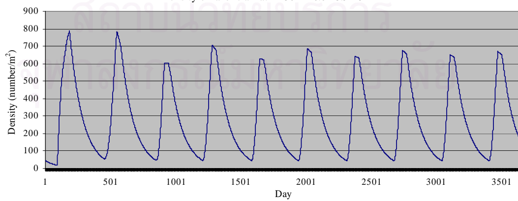
Density of razor clam at K=50 M=0.01 OS=45
