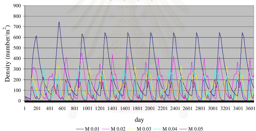
Comparing density of razor clam at K=50 OS=35 M=0.01,0.02,0.03,0.04,0.05
