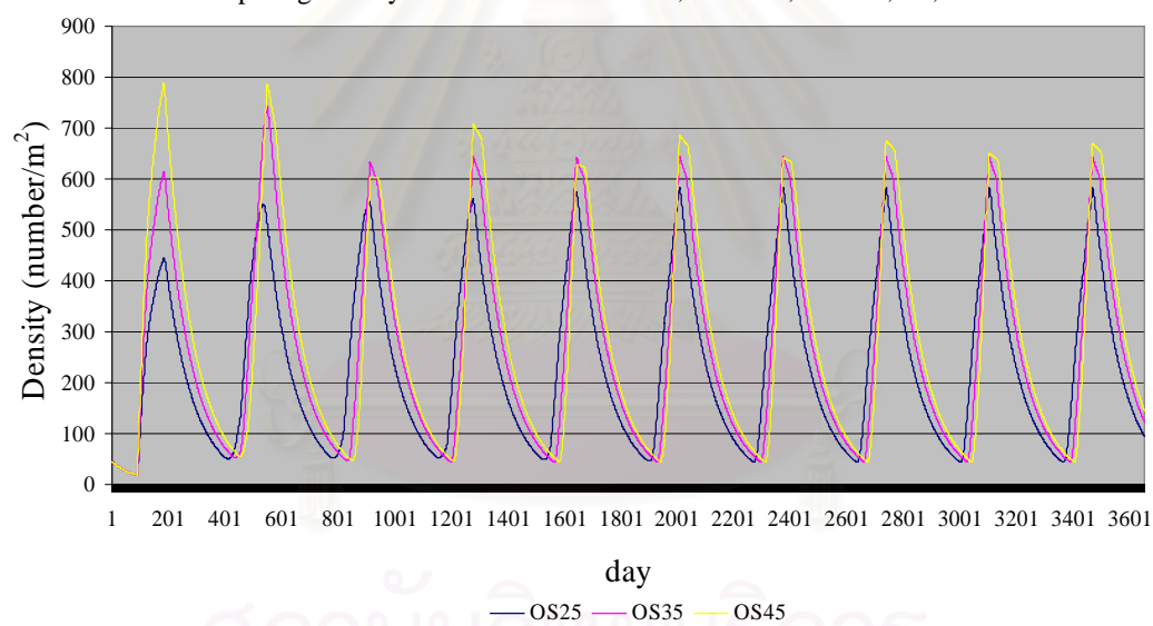
Comparing density of razor clam at K=50 , M=0.01 , OS=25, 35, 45
