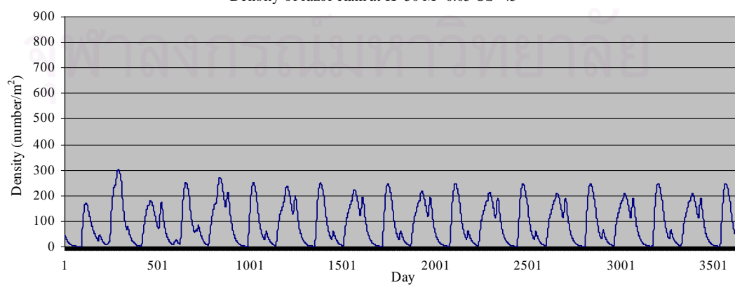
Density of razor clam at K=50 M=0.05 OS=45
