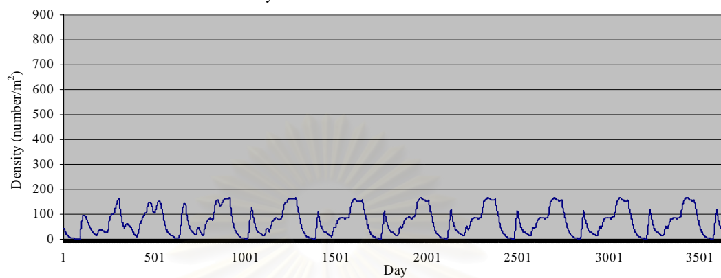
density of razor clam at K=50 M=0.05 OS=25
