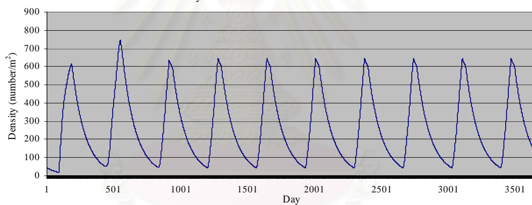
Density of razor clam at K=50 M=0.01 OS=35
