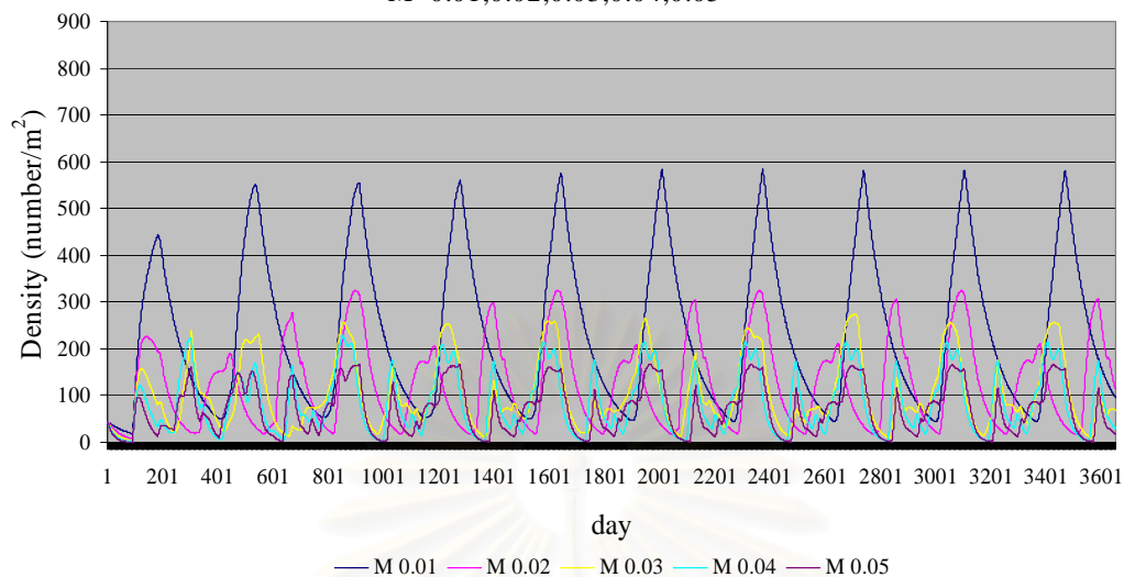
Comparing density of razor clam at K=50 OS=25 M=0.01,0.02,0.03,0.04,0.05
