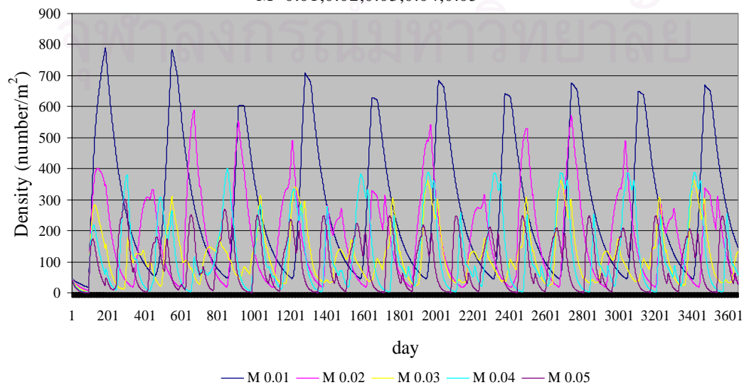
Comparing density of razor clam at K=50 OS=45 M=0.01,0.02,0.03,0.04,0.05
