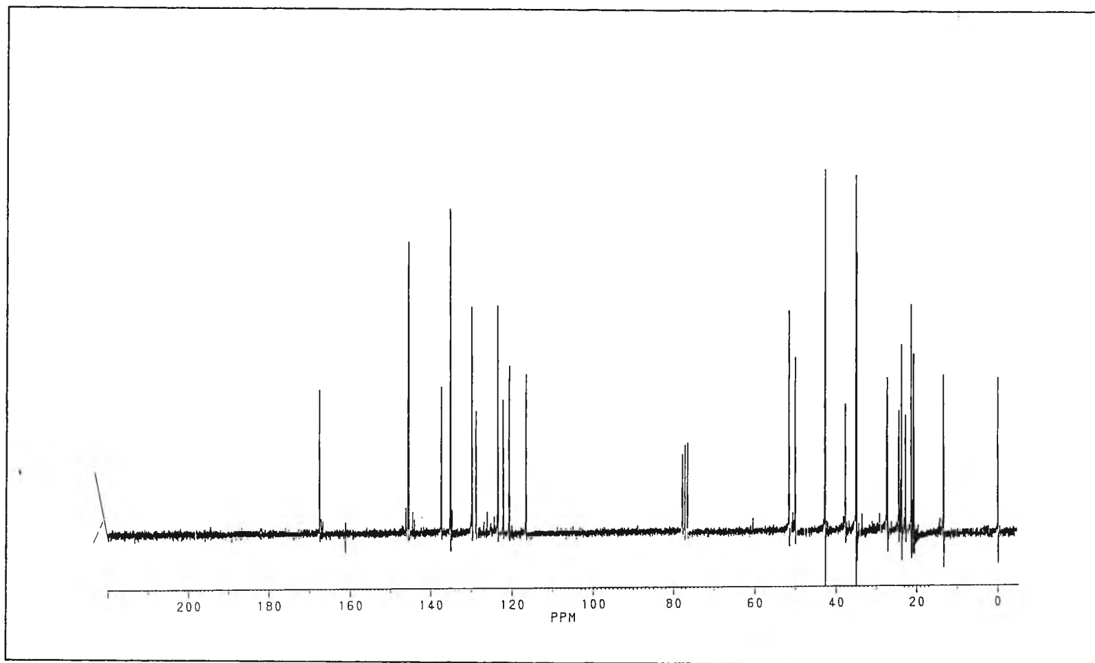
Fig. 31 The ^{13}\text{C} -NMR spectrum of compound 2a
