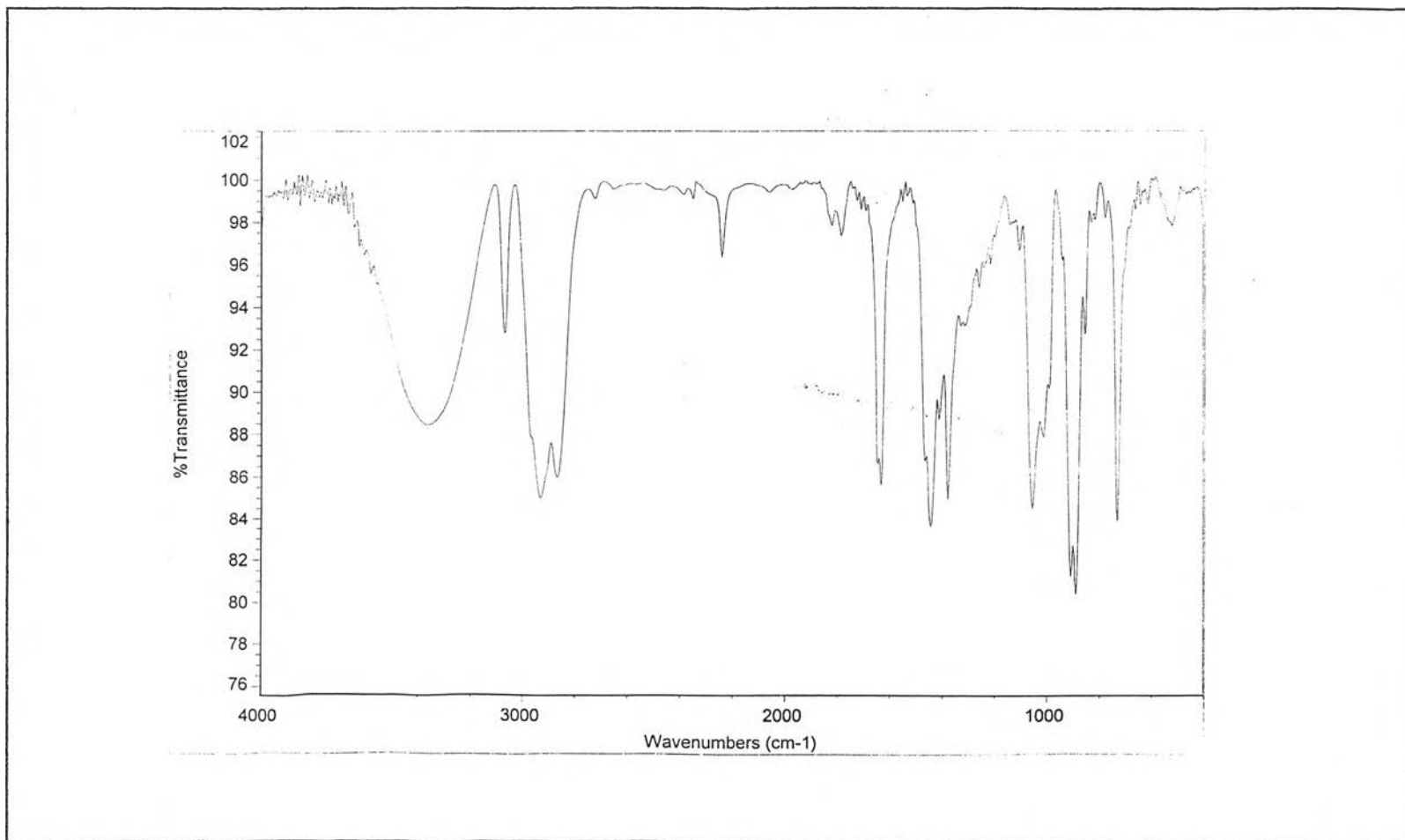
Fig. 15 The IR spectrum of compound 2
