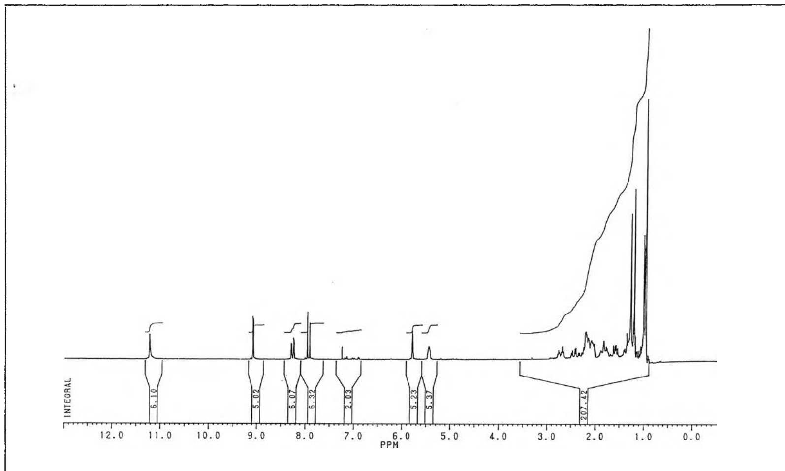
Fig. 30 The ^1\text{H-NMR} spectrum of compound 2a
