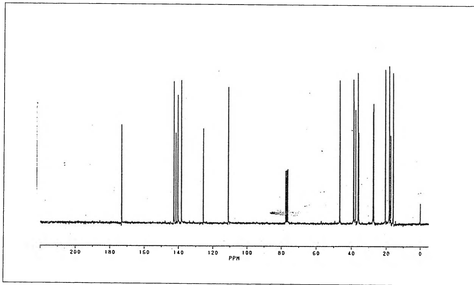
Fig. 12 The ^{13}\text{C} -NMR spectrum of compound 1
