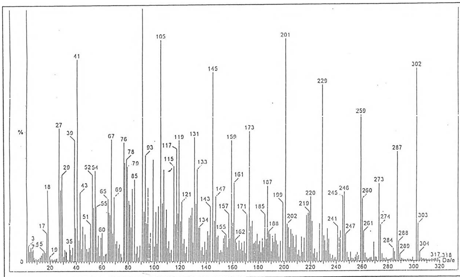
Fig. 28 The EI-MS spectrum of compound 3
