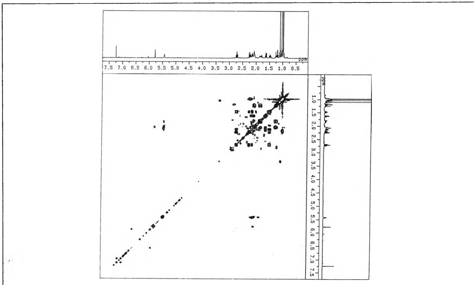
Fig. 21 The COSY-NMR spectrum of compound 2
