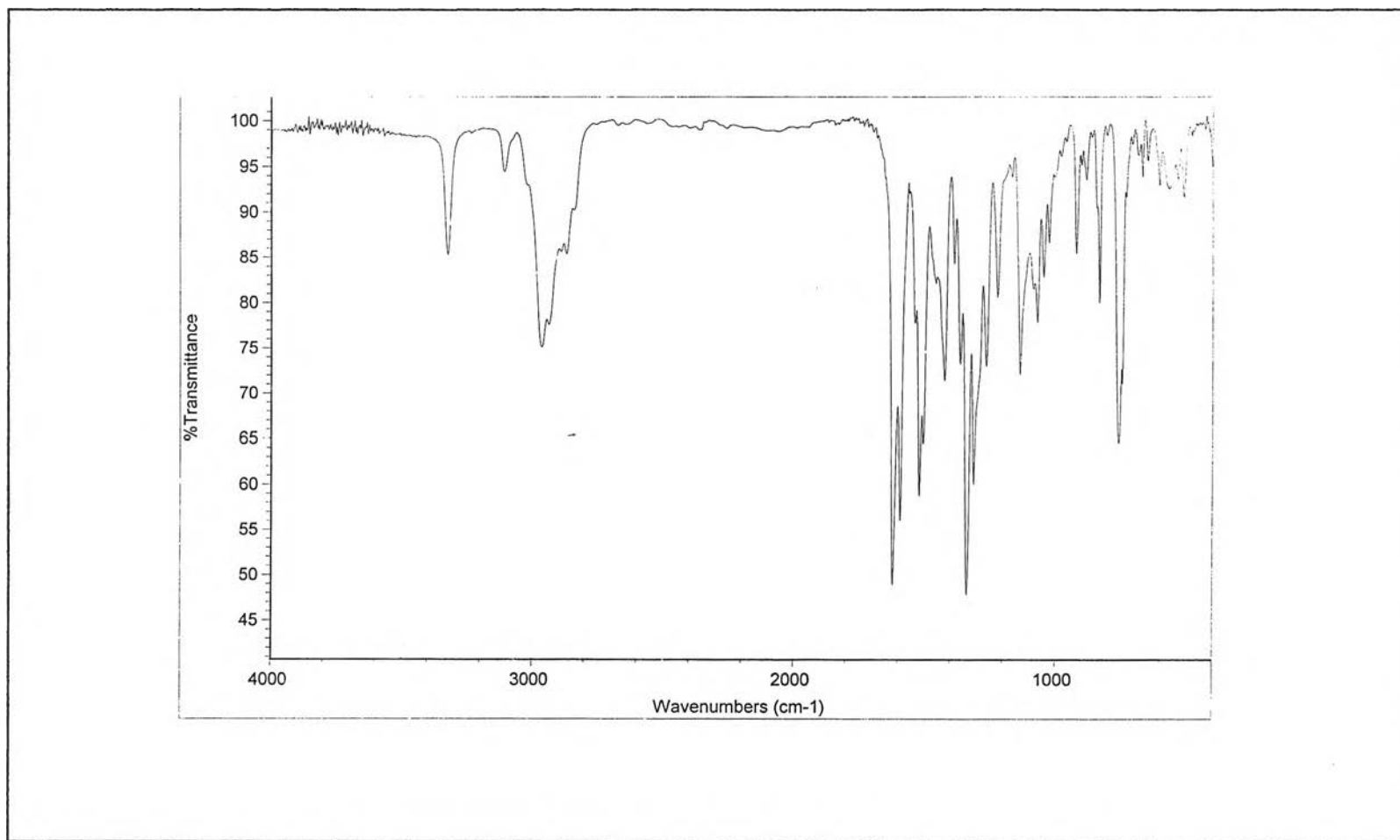
Fig. 29 The IR spectrum of compound 2a
