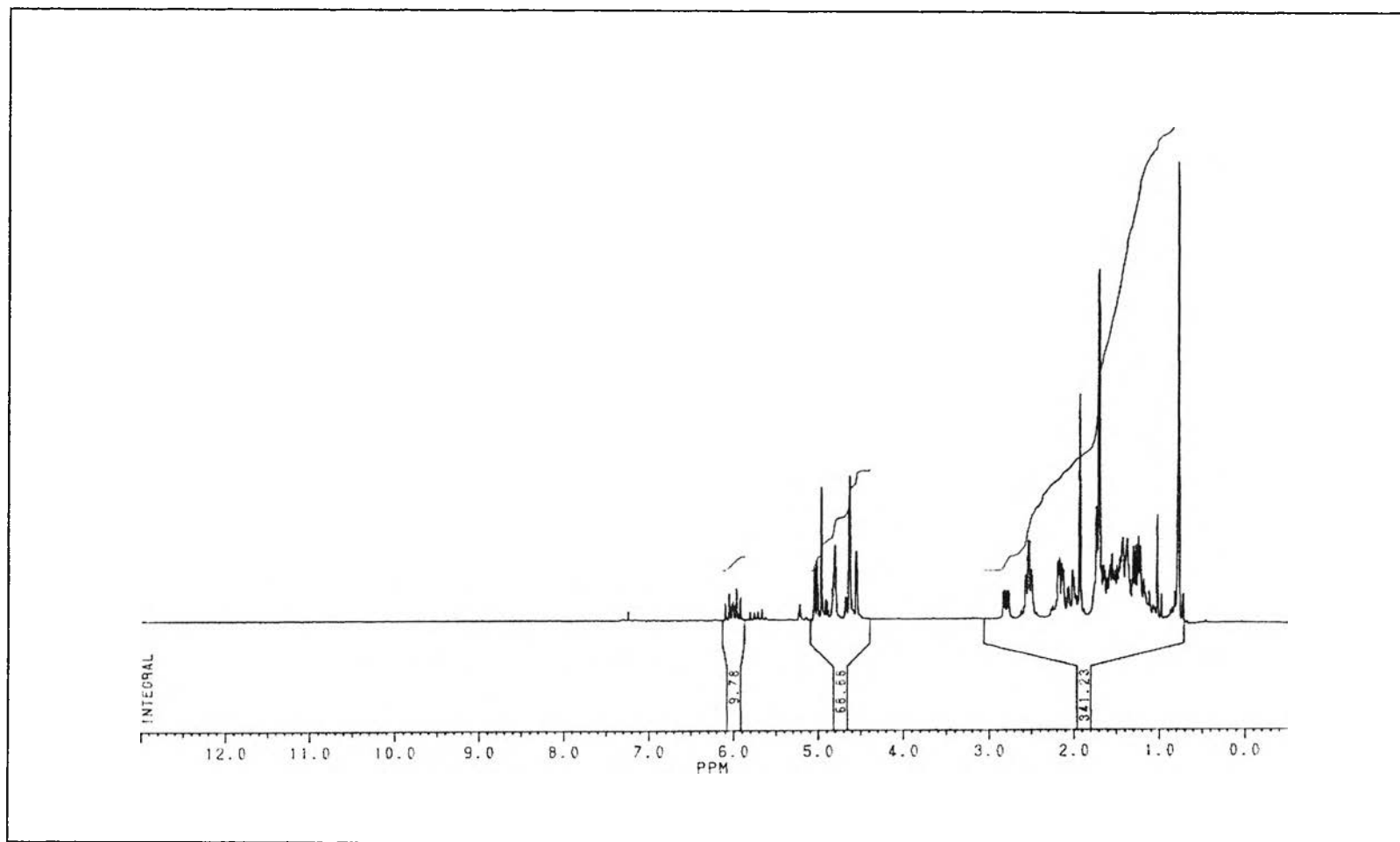
Fig. 25 The ^1\text{H} -NMR spectrum of compound 3
