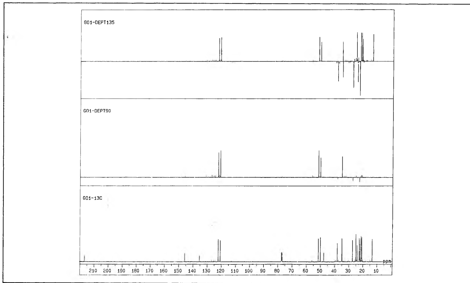
Fig. 18 The DEPT-90, DEPT-135 and ^{13}\text{C} -NMR spectrum of compound 2
