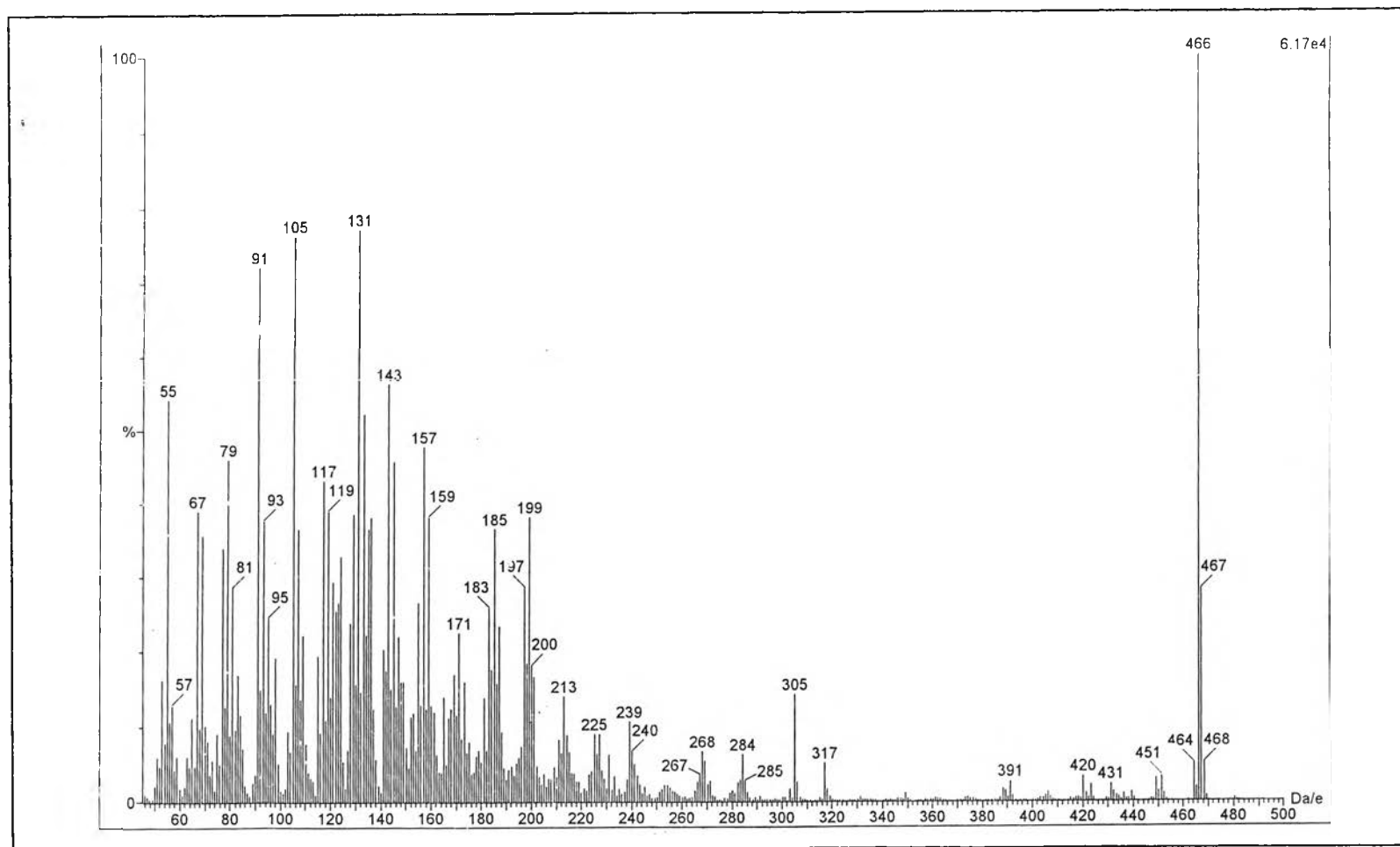
Fig. 33 The EI-MS spectrum of compound 2a
