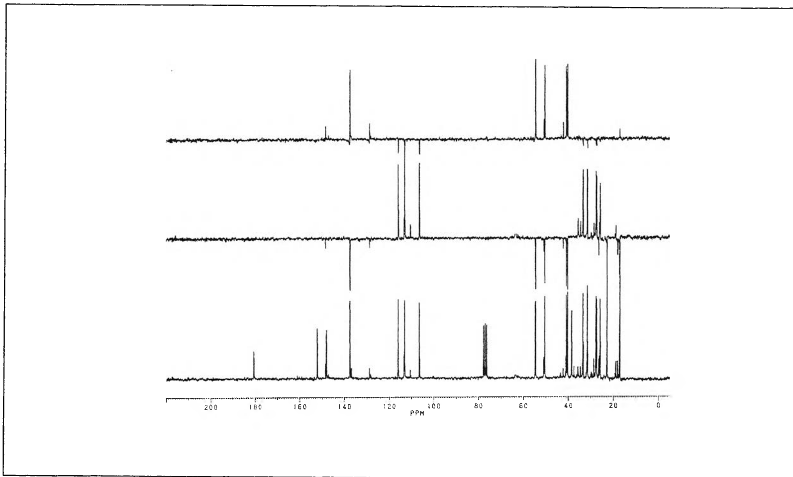
Fig. 27 The DEPT-90, DEPT-135 and ^{13}\text{C} -NMR spectrum of compound 3
