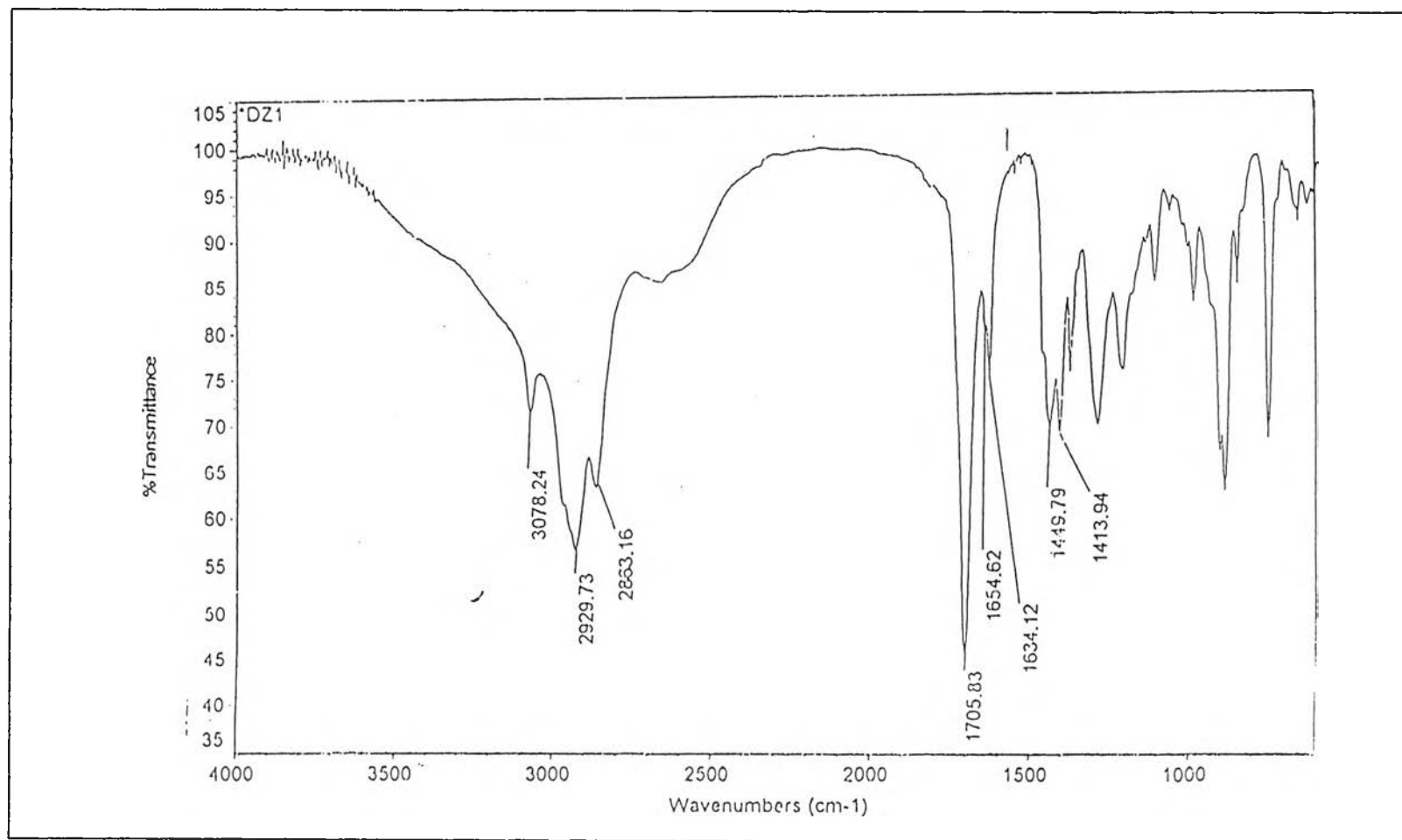
Fig. 24 The IR spectrum of compound 3
