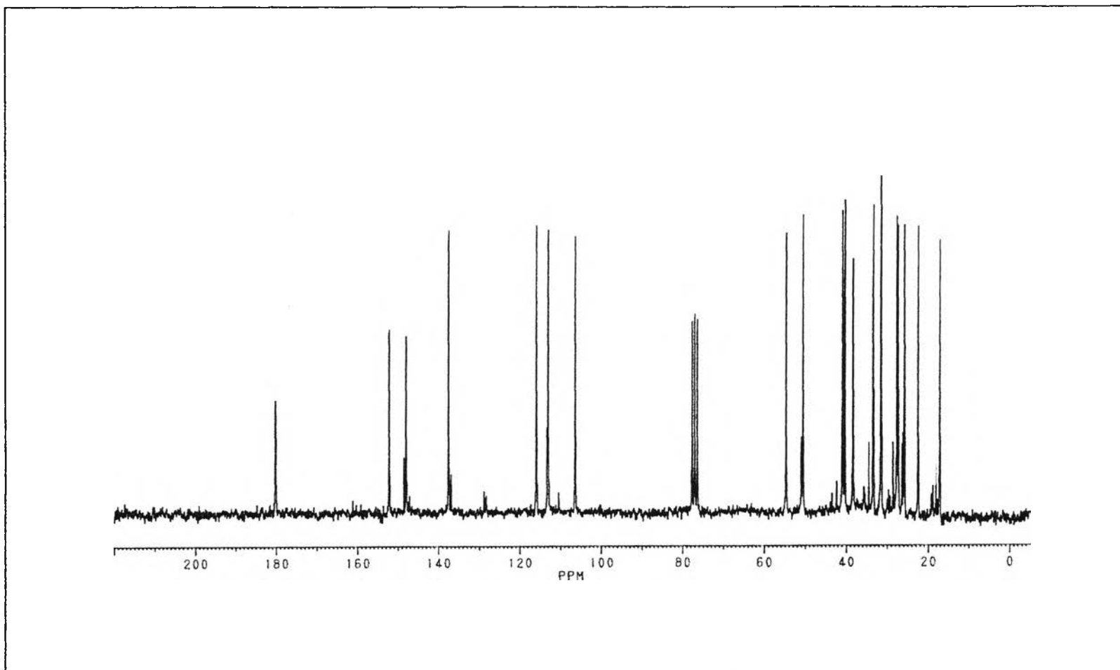
Fig. 26 The ^{13}\text{C} -NMR spectrum of compound 3
