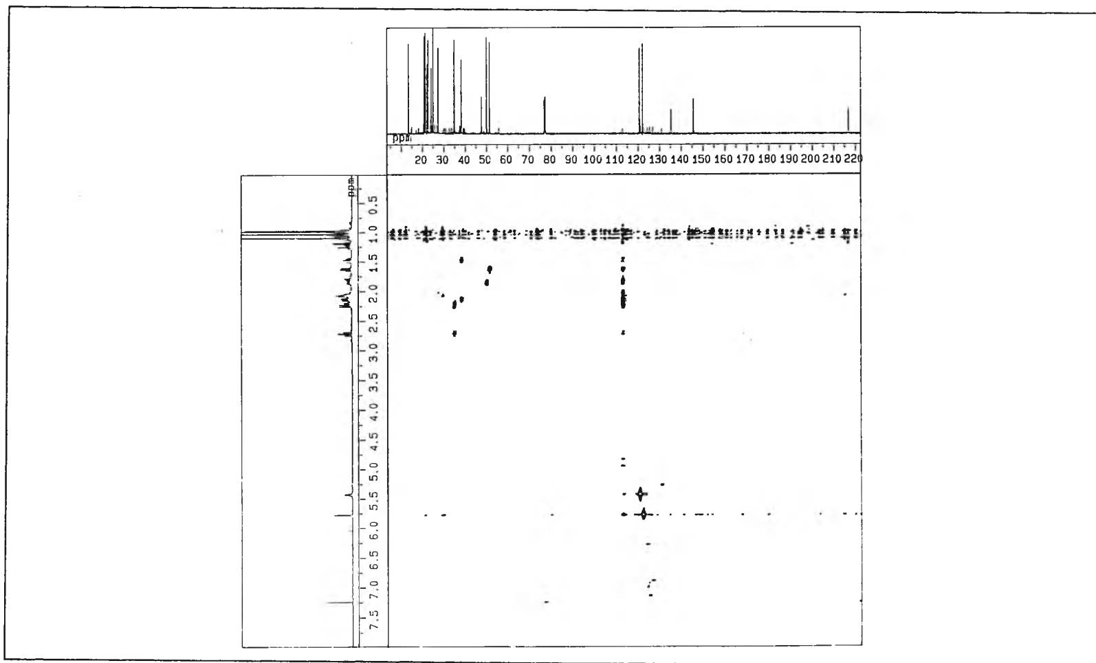
Fig. 20 The HMQC-NMR spectrum of compound 2
