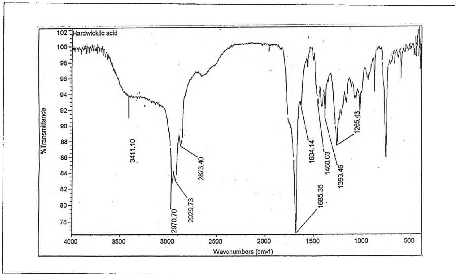
Fig. 10 The IR spectrum of compound 1
