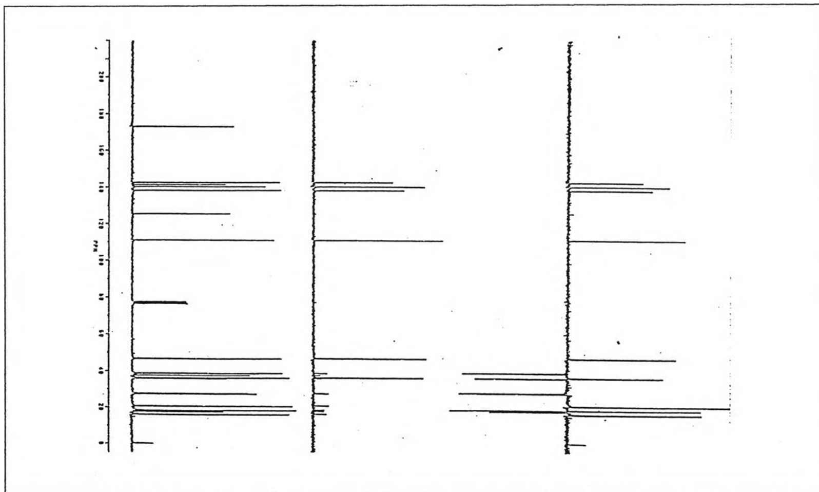
Fig. 13 The DEPT-90, DEPT-135 and ^{13}\text{C} -NMR spectrum of compound 1
