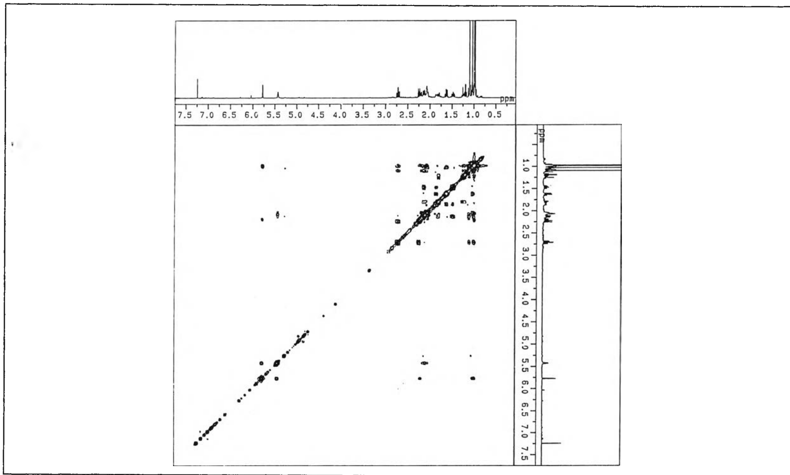
Fig. 23 The NOESY-NMR spectrum of compound 2
