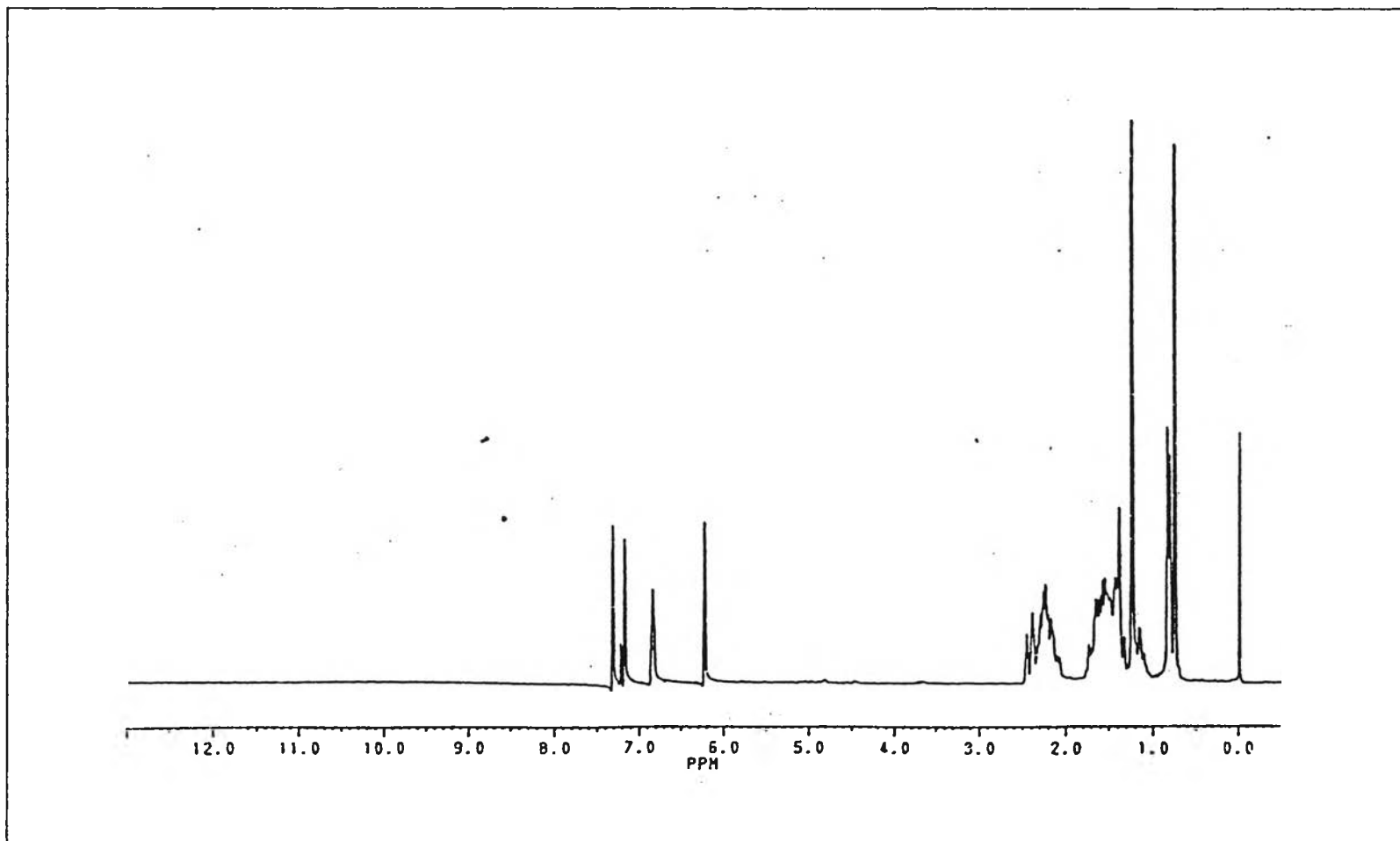
Fig. 11 The ^1\text{H-NMR} spectrum of compound 1
