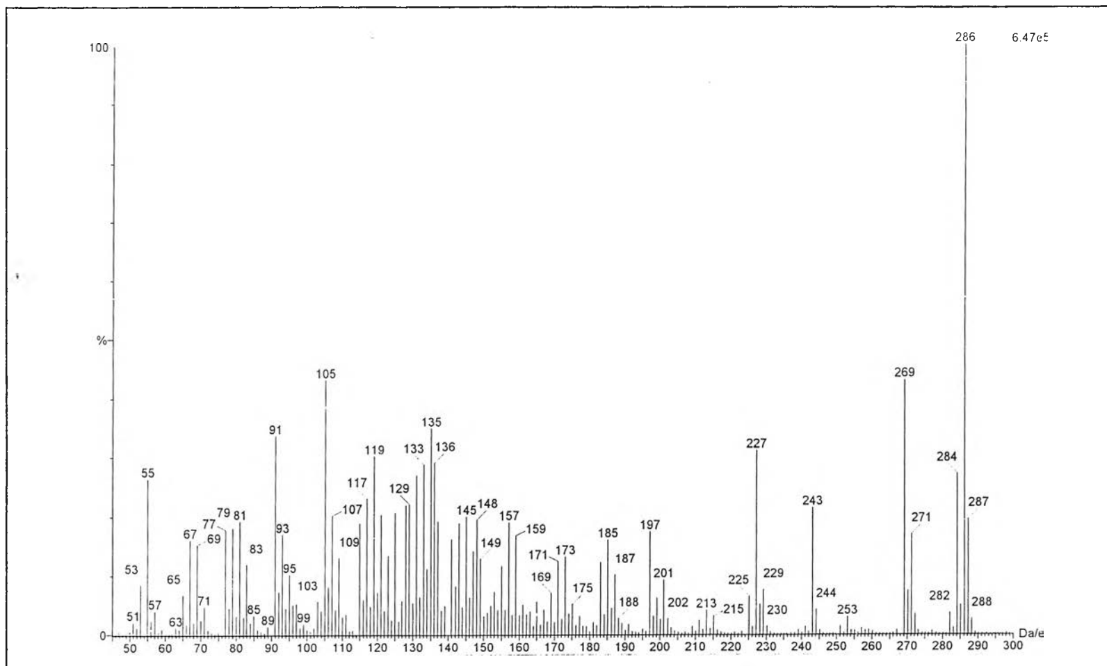
Fig. 19 The EI-MS spectrum of compound 2
