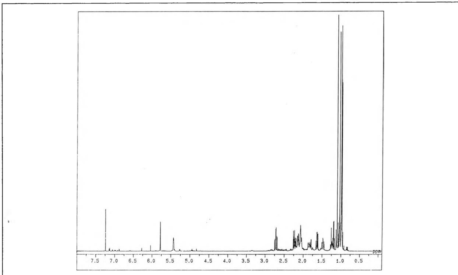
Fig. 16 The ^1\text{H-NMR} spectrum of compound 2
