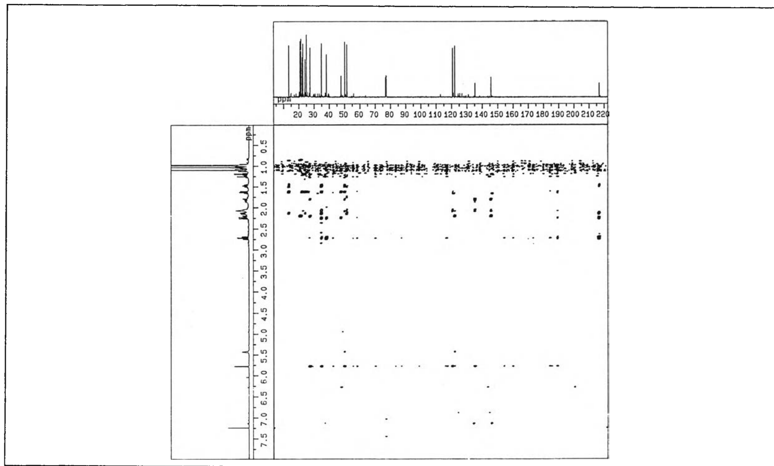
Fig. 22 The HMBC-NMR spectrum of compound 2
