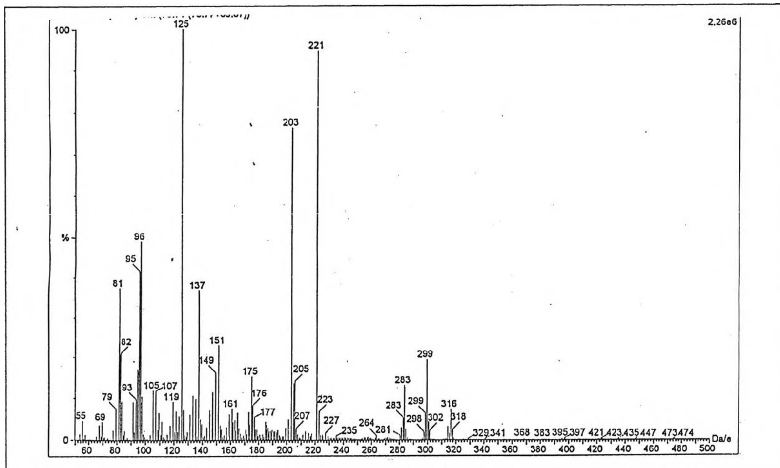
Fig. 14 The EI-MS spectrum of compound 1
