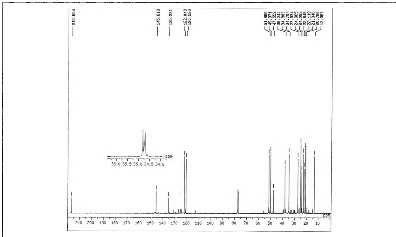
Fig. 17 The ^{13}\text{C} -NMR spectrum of compound 2
