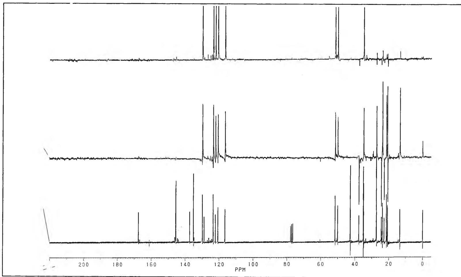
Fig. 32 The DEPT-90, DEPT-135 and ^{13}\text{C} -NMR spectrum of compound 2a
