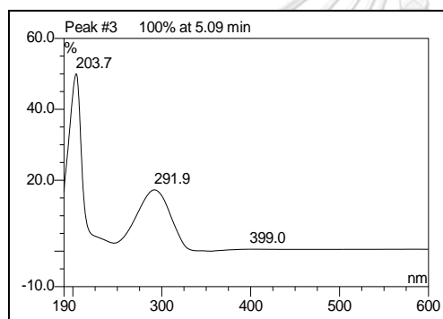
Figure 33. HPLC chromatogram of ethyl acetate crude extract of Streptomyces sp. NE1-12 (A), UV profiles of peak at t_R 5.09 mins (B) t_R 6.21 mins (C) respectively.
