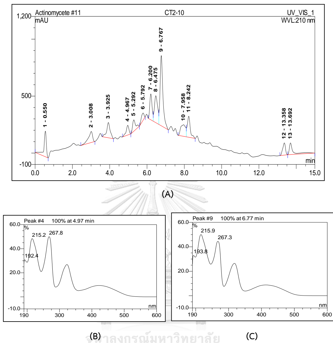
Figure 31. HPLC chromatogram of ethyl acetate crude extract of Streptomyces sp. CT2-10 (A), UV profiles of peak at t_R 4.97 mins (B) t_R 6.77 mins (C) respectively. HPLC condition (Column: Purospher column RP-18 from Merck), (Mobile phase: 0-100% Acetonitrile in water) and (Flow rate: 0.5ml/min)
