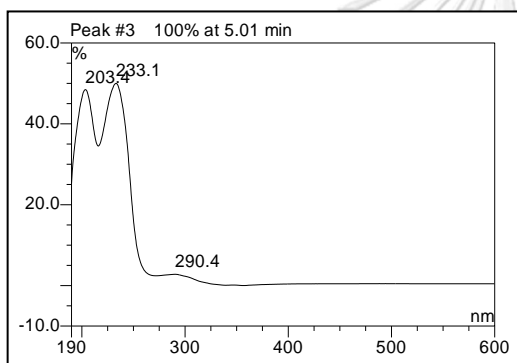
Figure 32. HPLC chromatogram of ethyl acetate crude extract of Streptomyces sp. ET3-23 (A), UV profiles of peak at t_R 5.01 mins (B) t_R 6.21 mins (C) respectively.
