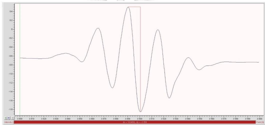
Figure 1.9 The peak-to-peak width ( \Delta BPP ) was 10.049 G of the TC=0.08 msec at the dose of 1000 cGy
