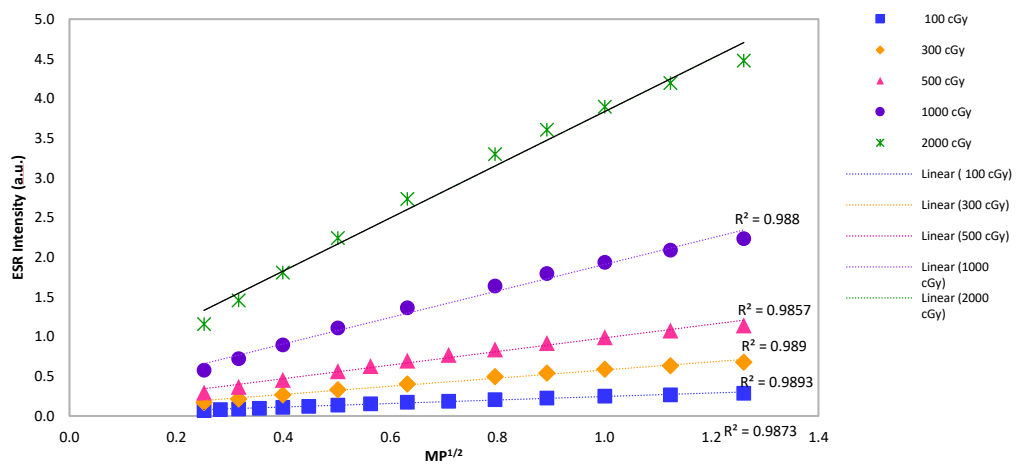
Figure I.2 The MP square of all doses was plotted against the EPR intensity graph. the highest limit of the linear part at MP^{1/2} = 1.26 (MP = 1.589 mW)
