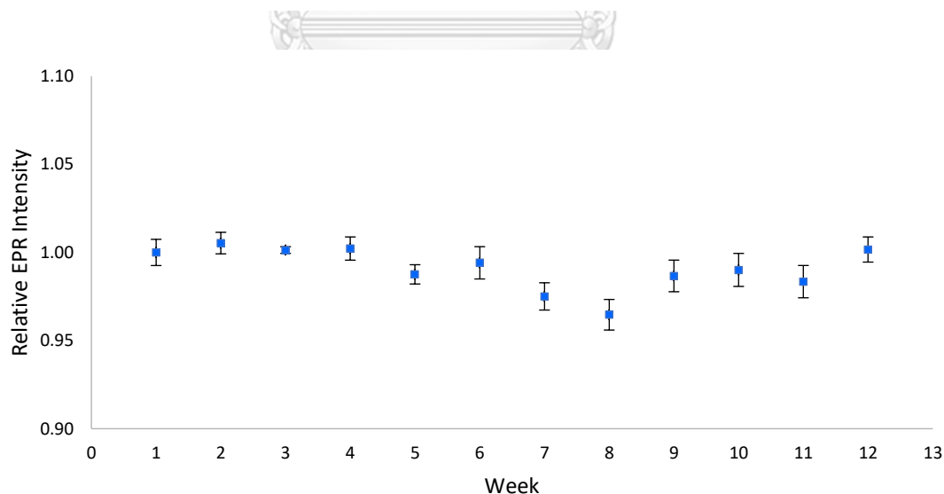
Figure 4.5 Fading of alanine dosimeter over 12 weeks. Error bars represent standard deviation of relative response from 5 alanine dosimeters.
