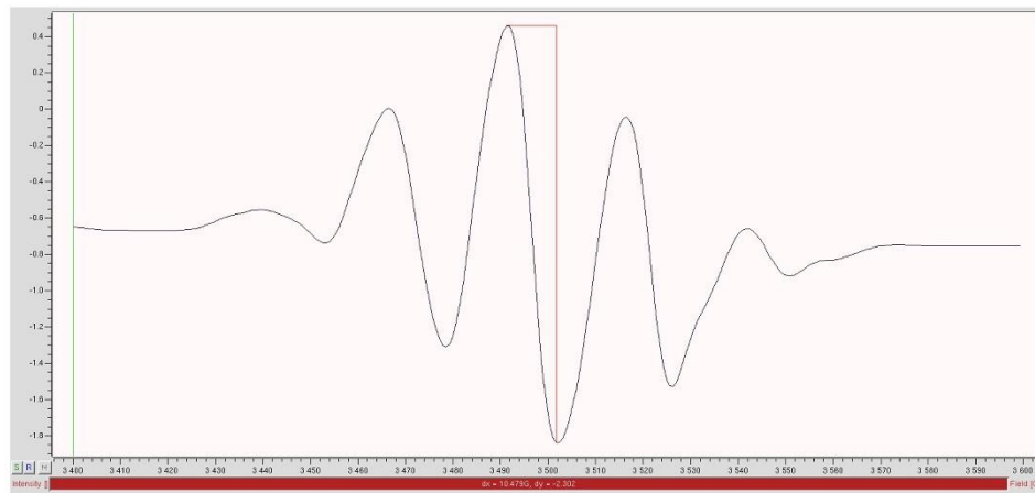
Figure 1.21 The peak-to-peak width ( \Delta BPP ) was 10.479 G of the TC=327.68 msec at the dose of 1000 cGy
