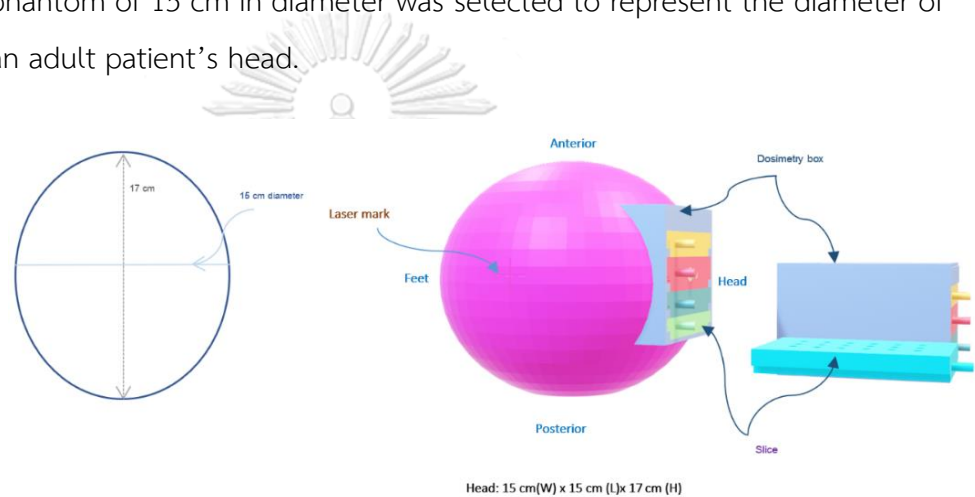
Figure 3.14 Fabricated head phantom
