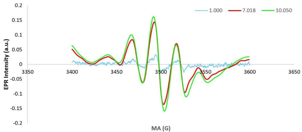
Figure 3.10 Spectrum from EPR signal at dose delivery of 100 cGy was set at 1.000, 7.018, and 10.050 G. Optimal MP was 1.589 mW and TC was fixed at 0.01 ms. Clear spectrum of alanine was present in the red line.
