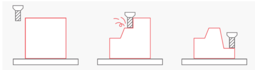
Figure 2.1 subtractive manufacturing
