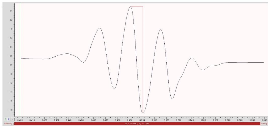
Figure 1.8 The peak-to-peak width ( \Delta BPP ) was 10.049 G of the TC=0.04 msec at the dose of 1000 cGy
