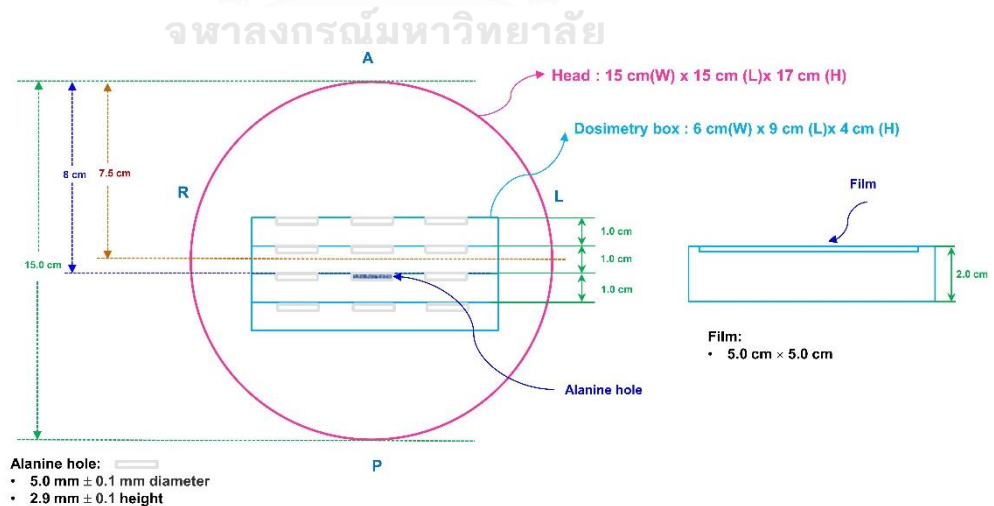
Figure 3.15 Cross-sectional view of the phantom
