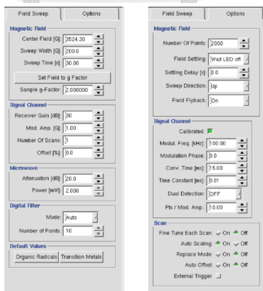
Figure 2.8 Field sweep parameters and options (21)
