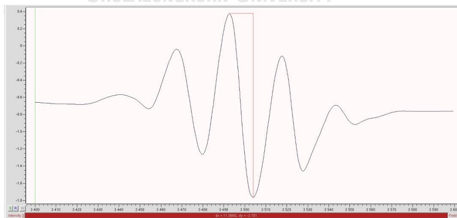
Figure 1.22 The peak-to-peak width ( \Delta BPP ) was 11.388 G of the TC=655.36 msec at the dose of 1000 cGy
