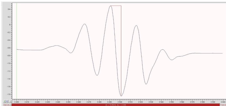
Figure 1.20 The peak-to-peak width ( \Delta BPP ) was 10.052 G of the TC=163.84 msec at the dose of 1000 cGy
