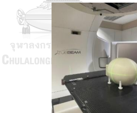
Figure 3.19 Irradiation of fabricated head phantom with a set of alanine dosimeters inside the TrueBeam with 6 MV-FFF linear accelerator.
