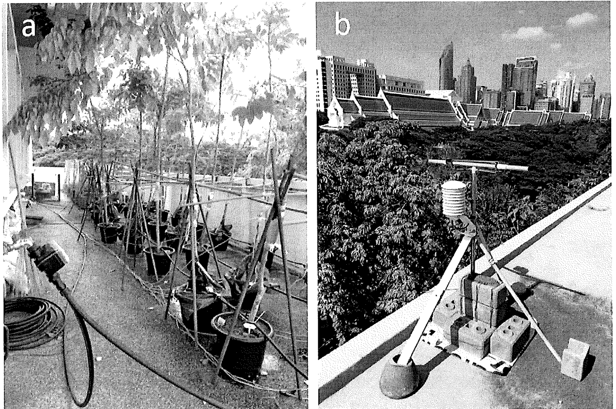
Figure 1: Site establishments (a) settings of the studied potted trees and sap flux measurements (b) measurement setup of meteorological variables
