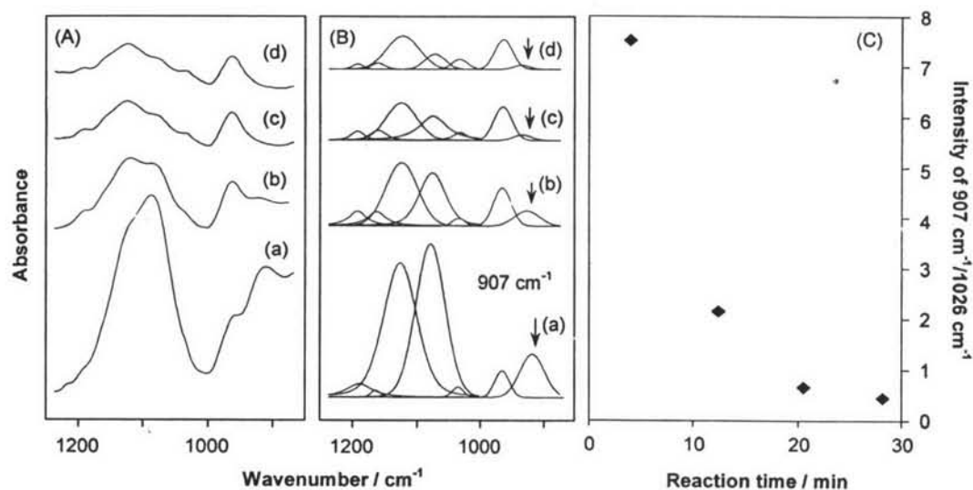
Figure 2. FTIR spectra of (A) before and (B) after curve fitting of 3 reacted with hydrazine 20 moles equivalent to pyranose ring at room temperature: for (a) 4 minutes, (b) 12 minutes, (c) 20 minutes, (d) 28 minutes; and (C) Gelation time of 4 as quantified by the oxirane peak at 907 cm -1 and pyranose ring peak at 1026 cm -1 .
