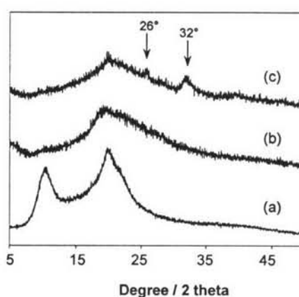
Figure 3. X-ray diffractograms of (a) 1 , (b) 4 , and (c) 4 after alternate soaking in \text{CaCl}_2/\text{Na}_2\text{HPO}_4 for 5 times.
