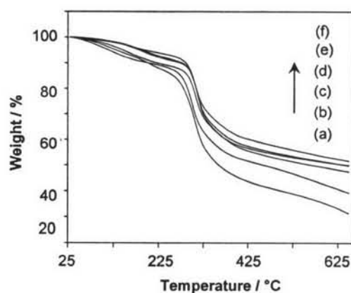
Figure 4. TGA thermograms of (a) 4 , and 4 after alternate soaking in \text{CaCl}_2/\text{Na}_2\text{HPO}_4 for the (b) 1 st cycle, (c) 2 nd cycle, (d) 3 rd cycle, (e) 4 th cycle, and (f) 5 th cycle.
