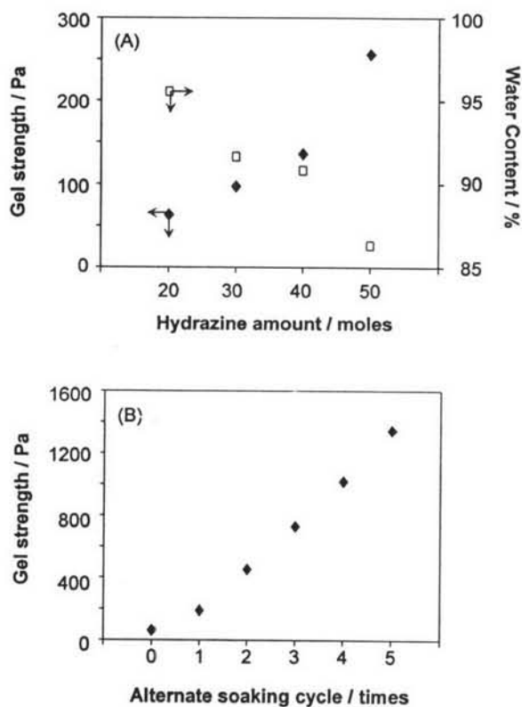
Figure 6. (A) Gel strength and water content of 4 under various hydrazine molar ratios, (B) Gel strength of (a) 4 with 20 times of hydrazine and 4 after alternate soaking in \text{CaCl}_2/\text{Na}_2\text{HPO}_4 for the (b) 1 st cycle, (c) 2 nd cycle, (d) 3 rd cycle, (e) 4 th cycle, and (f) 5 th cycle.
