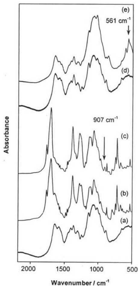
Figure 1. FTIR spectra of (a) 1 , (b) 2 , (c) 3 , (d) 4 , and (e) 4 after alternate soaking in \text{CaCl}_2/\text{Na}_2\text{HPO}_4 for 5 times.
