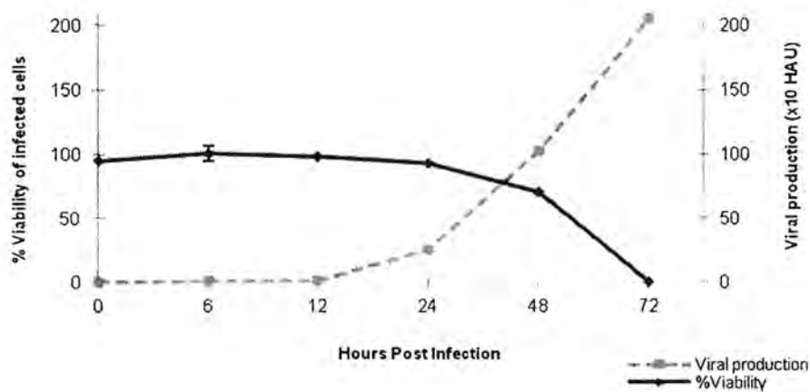
Fig. 3. Virus production and susceptibility of SH-SY5Y cells to H5N1 infection. Confluent monolayers of SH-SY5Y cells were infected with H5N1 virus at MOI of 1. At indicated time points, cell-free supernatants were collected for hemagglutination assay. The viability of mock and infected cells was determined by trypan blue dye exclusion method. All experiments were performed in triplicate. The dashed and solid lines indicate the amount of virus produced and infected cell viability compared with mock infection, respectively.
