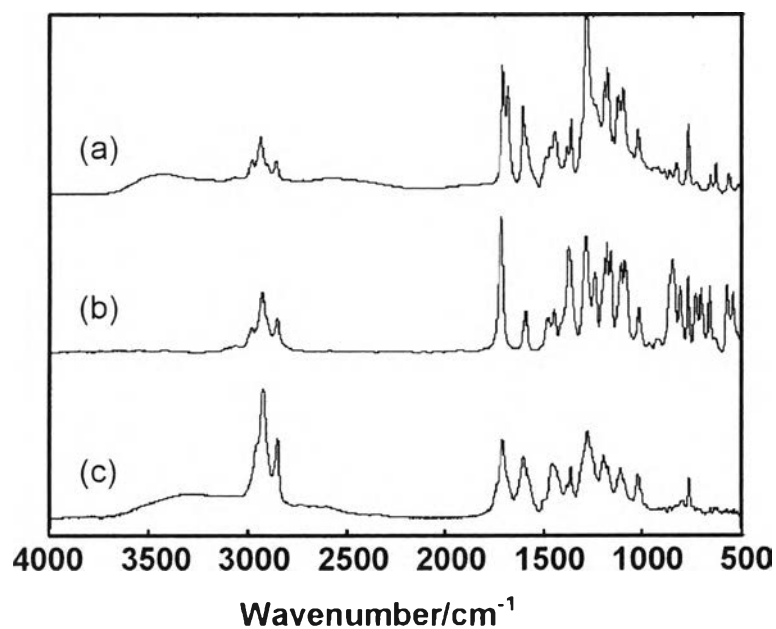
Figure 6.6 FTIR spectra of: (a) 3 , (b) 4 , and (c) 5 .
