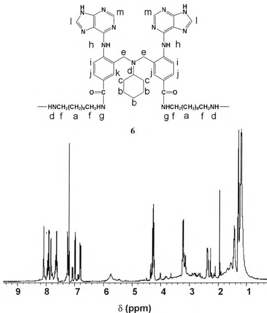
Figure 6.10 ^1\text{H} -NMR spectrum of 6 .
