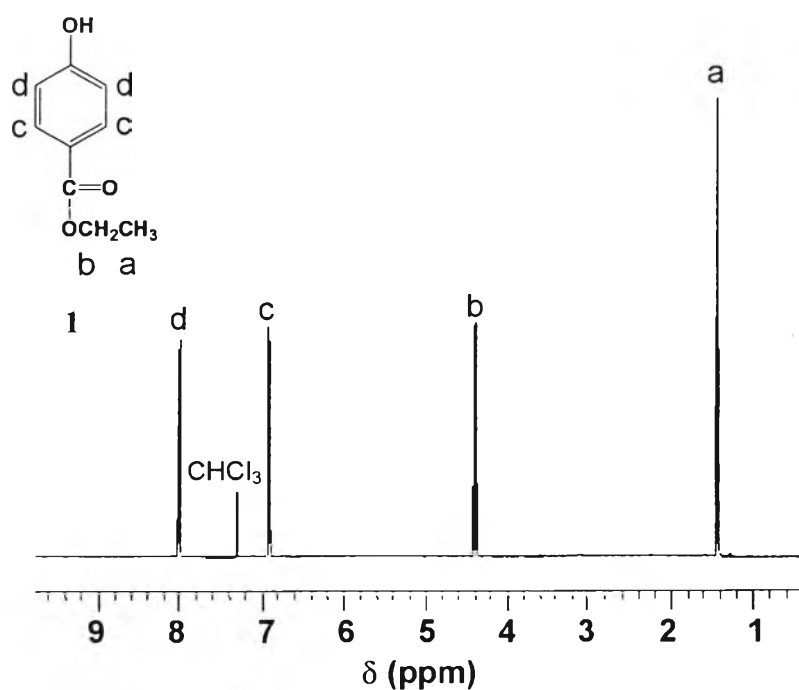
Figure 6.2 ^1\text{H-NMR} spectrum of 1 .
