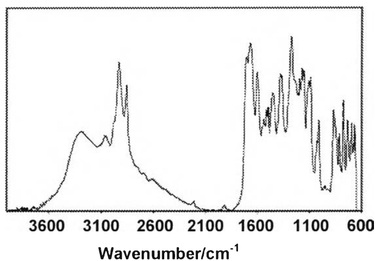
Figure 6.9 FTIR spectra of 6 .
