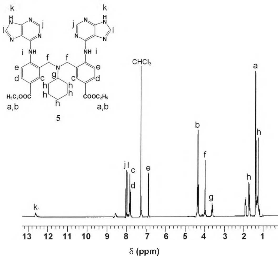
Figure 6.8 ^1\text{H} -NMR spectrum of 5 .
