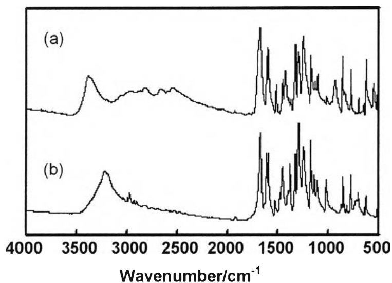
Figure 6.1 FTIR spectra of: (a) 4-hydroxybenzoic acid, and (b) 1 .
