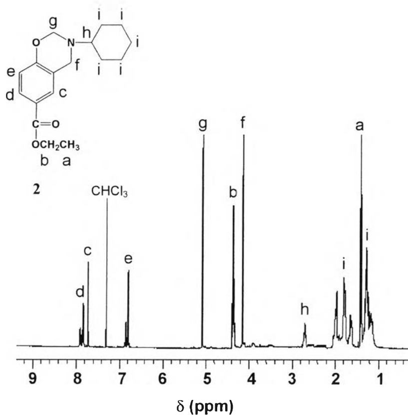
Figure 6.4 ^1\text{H-NMR} spectrum of 2 .
