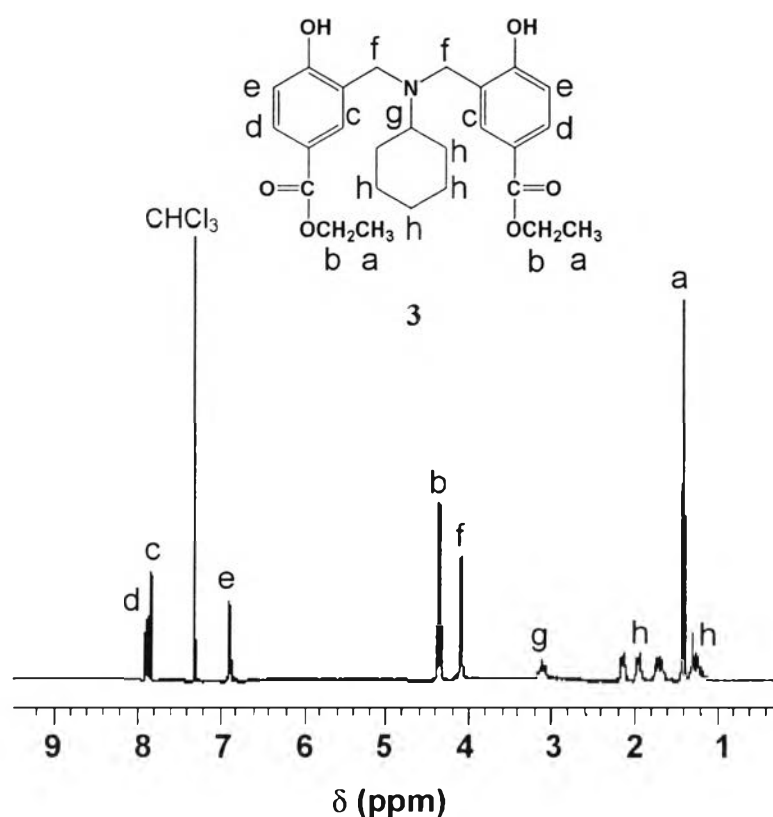
Figure 6.5 ^1\text{H-NMR} spectrum of 3.
