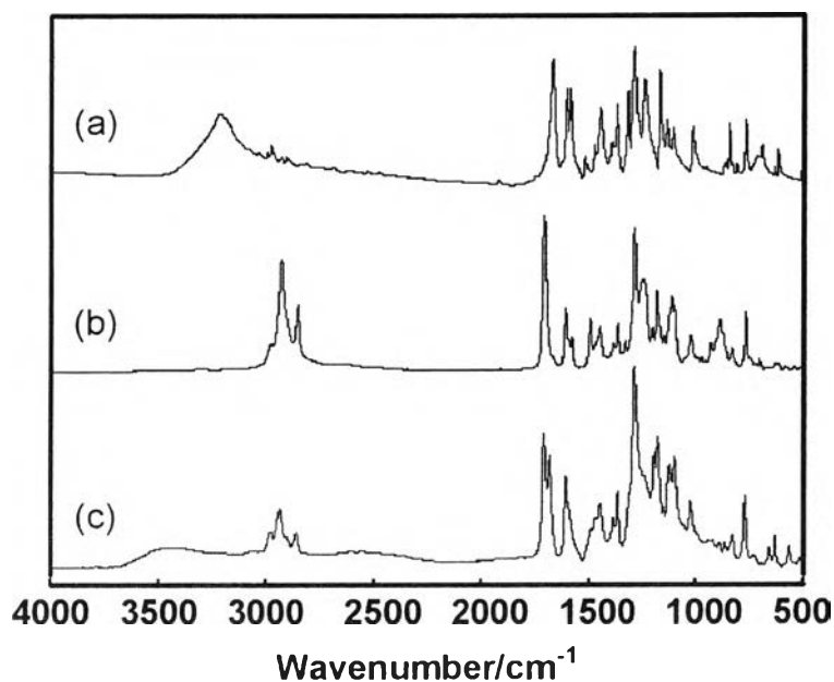
Figure 6.3 FTIR spectra of: (a) 1 , (b) 2 , and (c) 3 .
