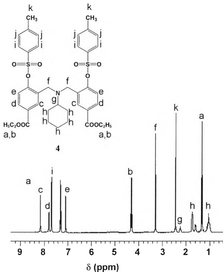
Figure 6.7 ^1\text{H} -NMR spectrum of 4 .
