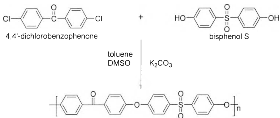
Figure 3.1 Condensation polymerization of the PEKES.
