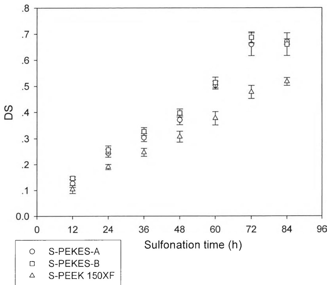
Figure 3.9 Degrees of sulfonation of S-PEKES-A, S-PEKES-B, and S-PEEK 150XF.
