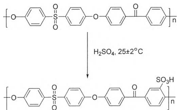
Figure 3.3 Post-sulfonation of PEKES Systems A and B.
