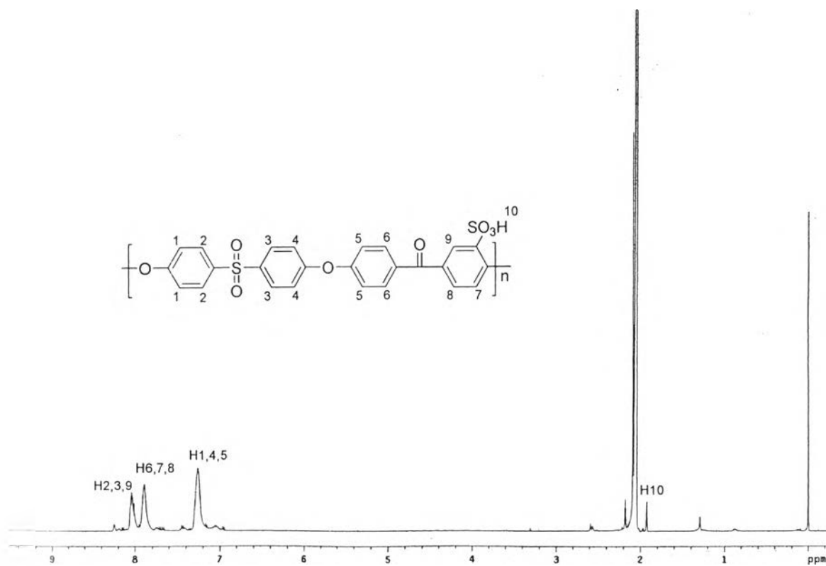
Figure 3.7 1 H-NMR spectra of S-PEKES-A and S-PEKES-B.
