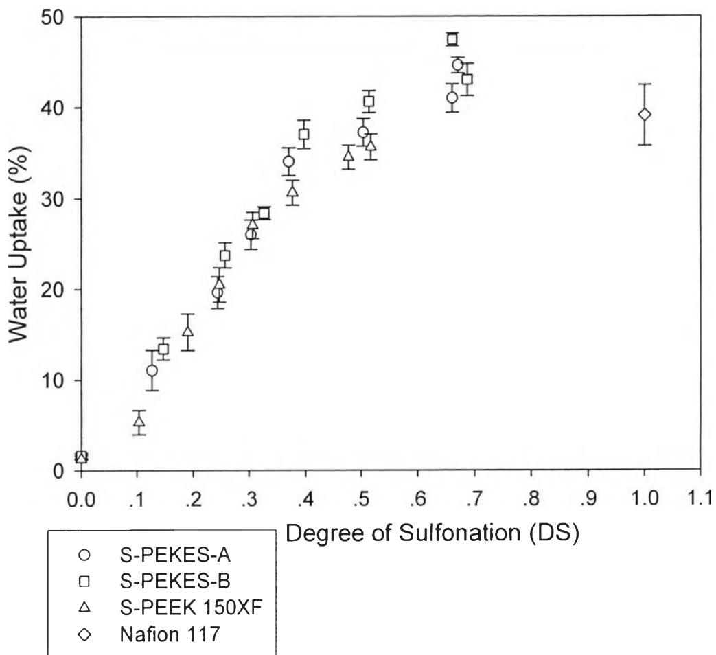
Figure 3.11 Water uptake (%) of S-PEKES-A, S-PEKES-B, and S-PEEK 150XF.
