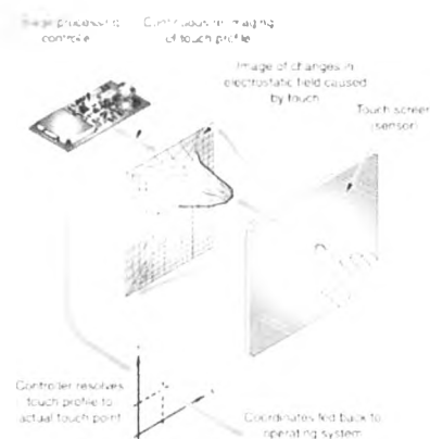
Figure 2.1 The fundamental of capacitive touchscreen.
