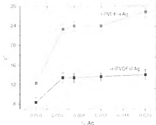
Figure 2.26 Dielectric constant at room temperature for (a) \alpha -PVDF@Ag and (b) \beta -PVDF@Ag at different silver nanoparticle concentrations (Miranda et al. , 2008).
