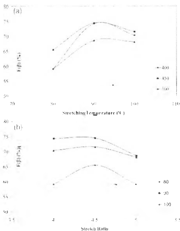
Figure 2.10 Variation of \beta -phase content for Kynar 720 as a function of (a) stretching temperature and (b) stretch ratio ( S.R. = \frac{Length_{final}}{Length_{initial}} ) (Salimi et al. , 2003).
