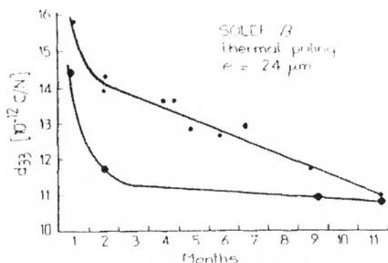
Figure 2.19 Long term behavior after thermal poling (Betz, (1984).
