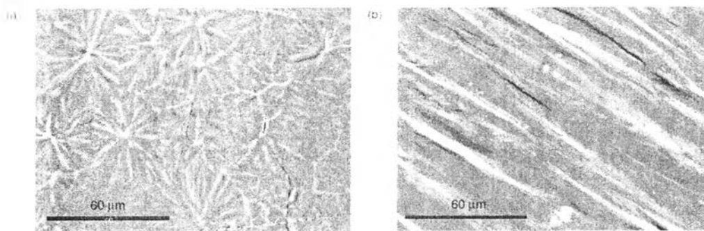
Figure 2.15 SEM images of the PVDF@Ag nanocomposites: (a) with R=1 (b) with R=5 (D. Miranda et al. , 2008).
