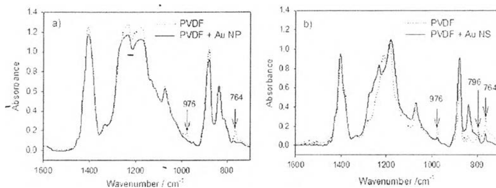
Figure 2.22 FT-IR spectra from dried polymer films of (a) PVDF and Au-NP/PVDF composite, and (b) PVDF and Au-NS/PVDF composite, prepared from mixed solvents of DMF and water. The mass ratio of gold over PVDF in the mixture is 0.5% (Wang et al. , 2011).
