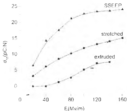
Figure 2.18 Poling field dependence of piezoelectric coefficient d_{33} for extruded, stretched and static electric field poling (SSSEP) (Huan et al. , 2007).
