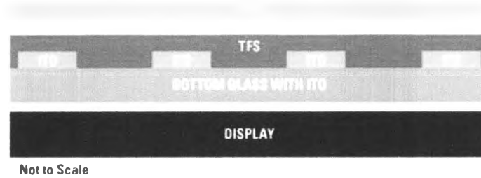
Figure 2.3 Transparent force sensing layer incorporated in a digital resistive multi-touch screen construction.
