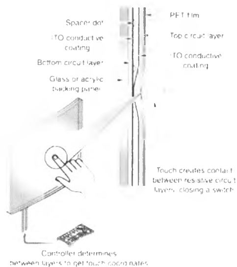
Figure 2.2 The fundamental of resistive touchscreen.
