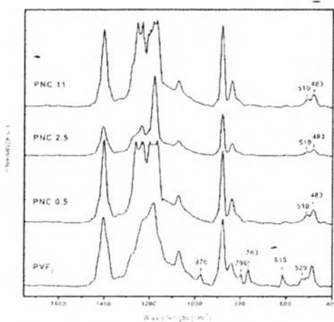
Figure 2.25 FT-IR spectra of PVDF and the nanocomposite films at indicated concentrations (Manna et al. , 2006).
