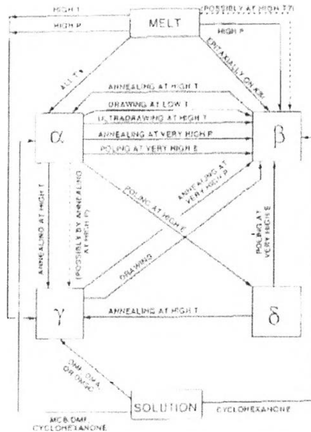
Figure 2.7 The interrelations among the four well-established phase of PVDF by Lovinger. (1982).
