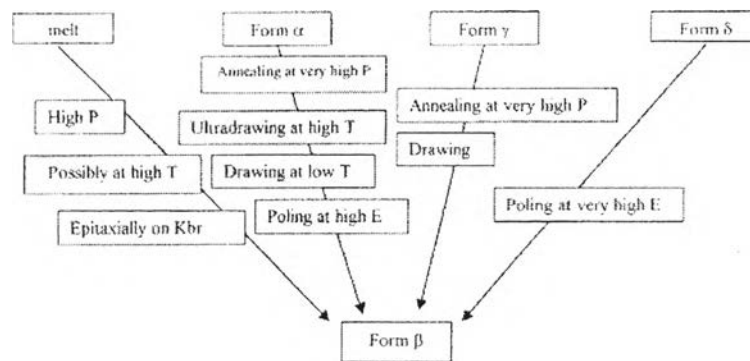
Figure 2.6 Transitions from different conformations of PVDF to \beta -phase (Nalwa et al. , 1995).
