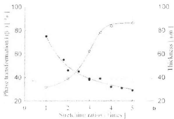
Figure 2.11 The F(\beta) fraction content and thickness variation of PVDF films with different stretching ratios (Chang et al. , 2008).
