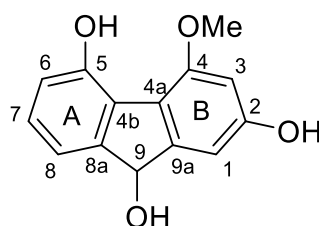
4-methoxy-9H-fluorene-2,5,9-triol [ 312 ]
