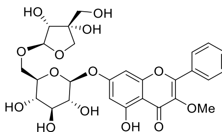
5-Hydroxy-3-methoxyflavone-7-O-[\beta-D-aposyl-(1\to6)]-\beta-D-glucoside [15]
