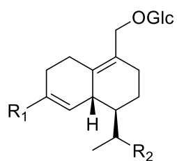
[195] Dendronobiloside C, R 1 = -CH 2 OGlc, R 2 =H
