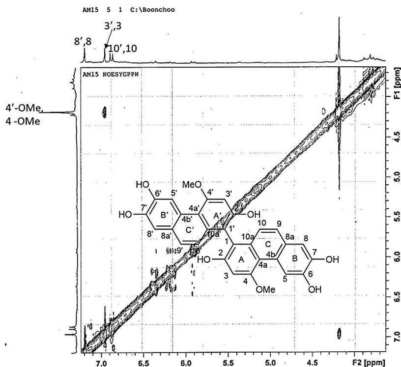
Figure 139 NOESY spectrum of compound AMF3
