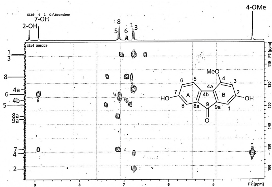
Figure 89 HMBC spectrum of compound DG5
