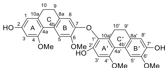
aerimultin A [337]
