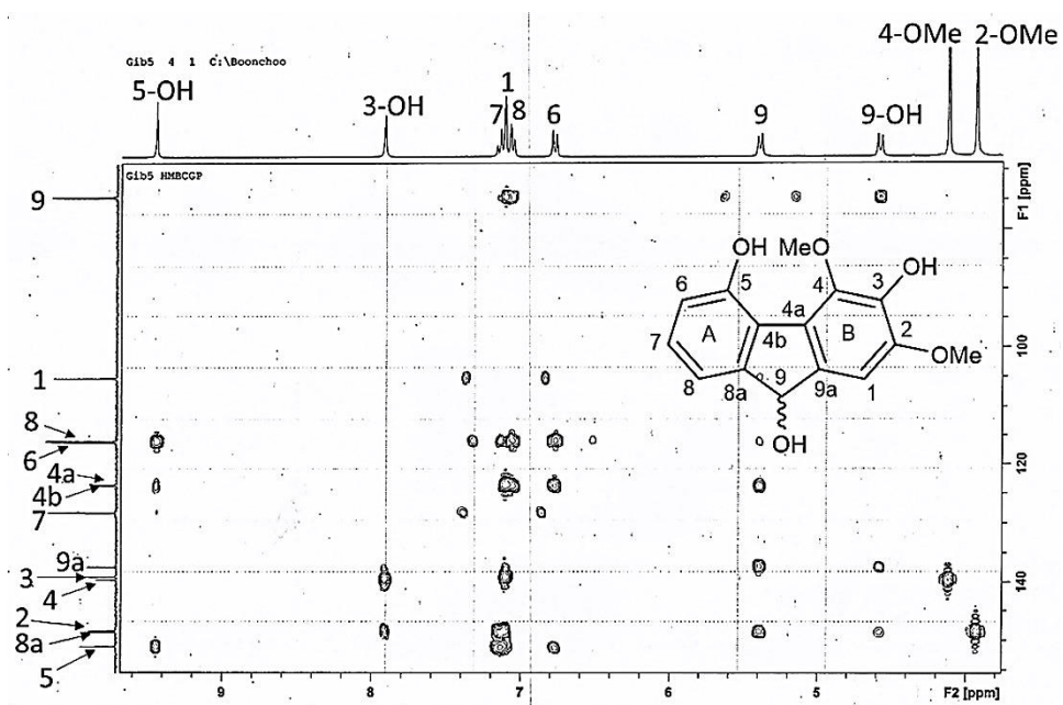
Figure 62 HMBC spectrum of compound DG1
