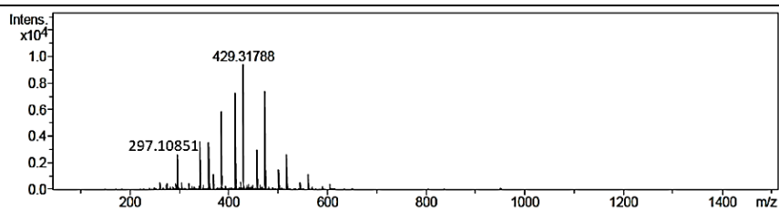
Figure 154 Mass spectrum of compound AMF6
