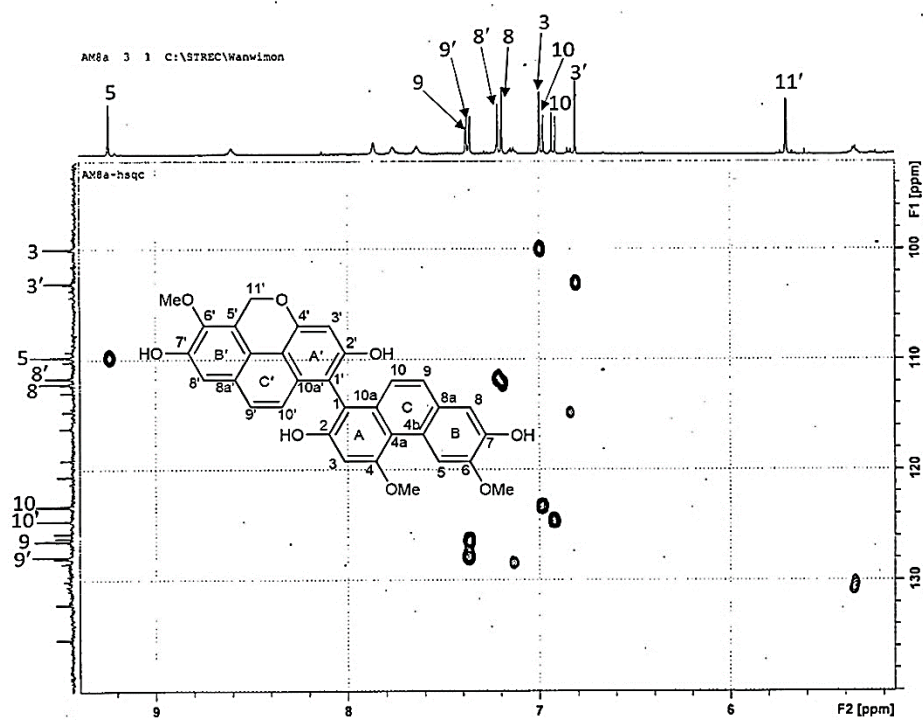
Figure 128 ^{13}\text{C} -NMR (125 MHz) spectrum of compound AMF2
