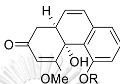
[140] 9,10-Dihydro-aphyllone A-5-O- \beta -D-glucopyranoside: R = Glc
