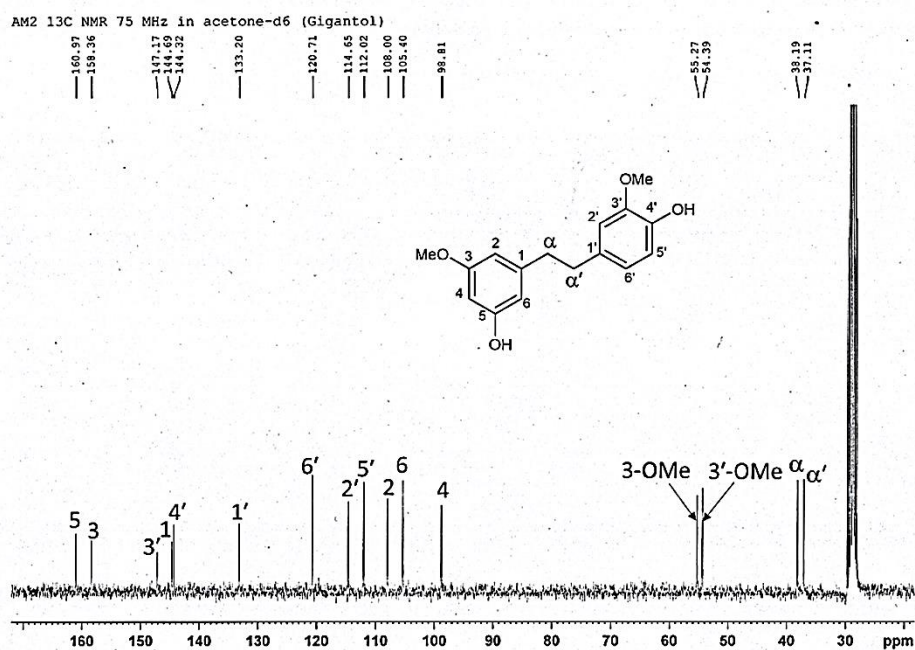
Figure 156 13 C-NMR (75 MHz) spectrum of compound AMF6
