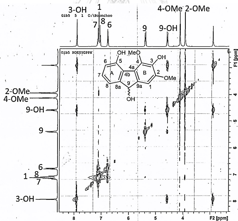
Figure 63 NOESY spectrum of compound DG1
