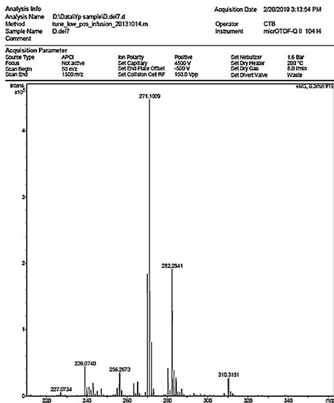
Figure 24 Mass spectrum of compound DD5
