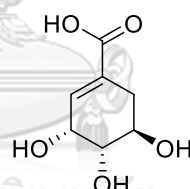
[240] (-)-Shikimic acid
