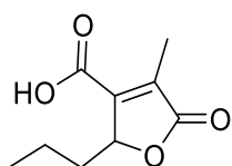
[236] Decumbic acid
