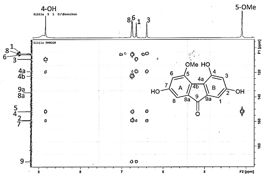
Figure 106 HMBC spectrum of compound DG8
