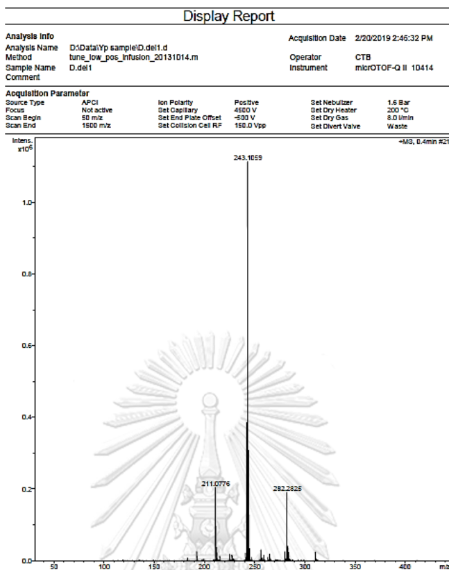
Figure 8 Mass spectrum of compound DD1
