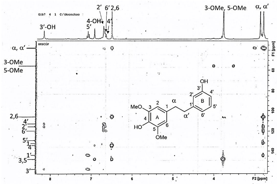
Figure 95 HMBC spectrum of compound DG6
