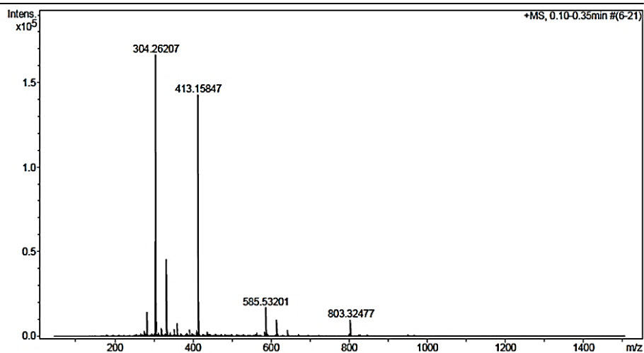
Figure 140 Mass spectrum of compound AMF4
