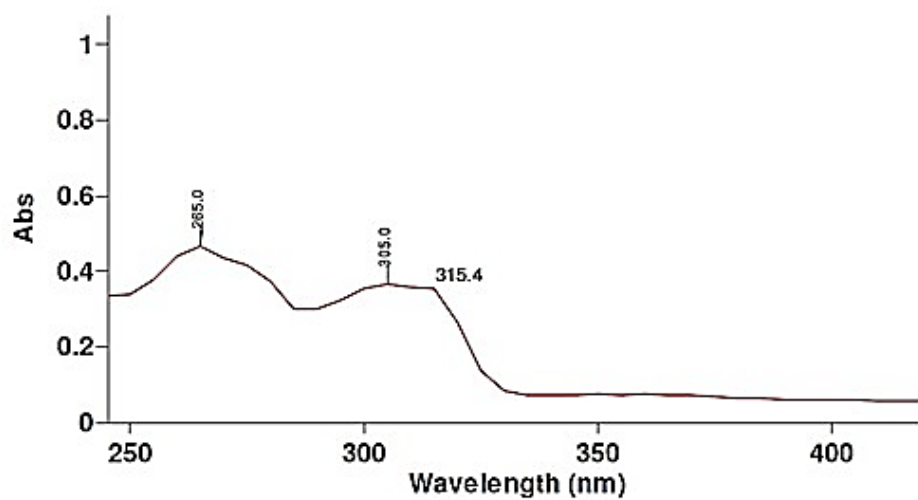
Figure 116 UV spectrum of compound AMF1
