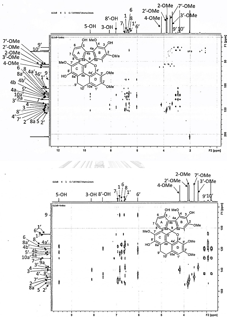
Figure 70 HMBC spectrum of compound DG2 (full and expanded spectrum)
