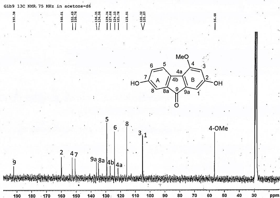
Figure 87 13 C-NMR (75 MHz) spectrum of compound DG5
