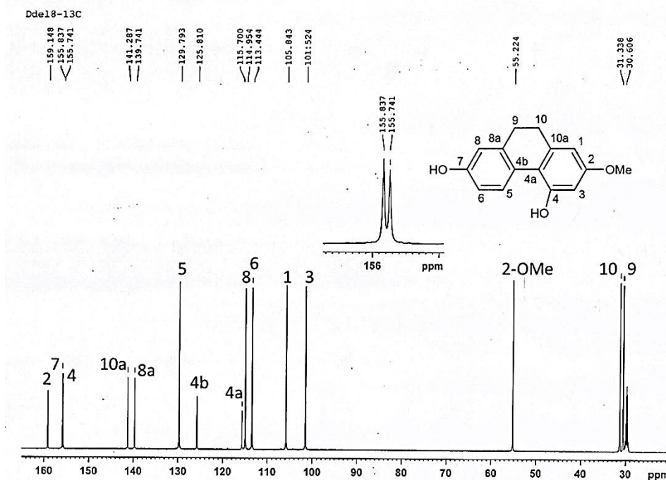
Figure 36 ^{13}\text{C} -NMR (125 MHz) spectrum of compound DD8
