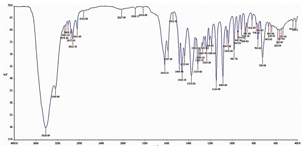
Figure 58 IR spectrum of compound DG1
