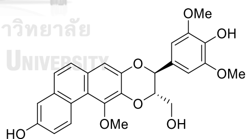
[137] Dendrocandin P1
