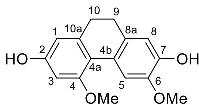
6-methoxycoelonin [ 332 ]
