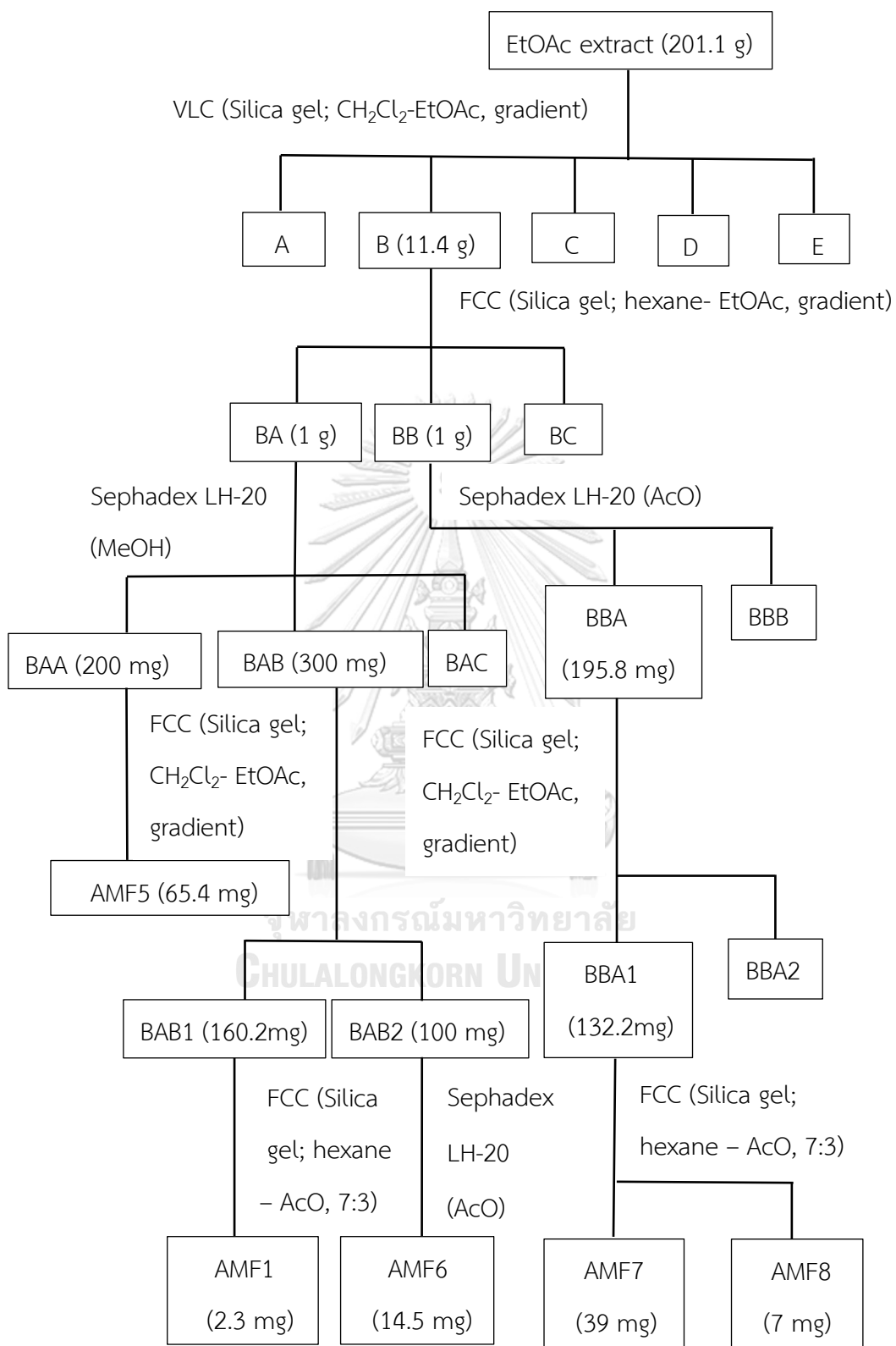
Scheme 6 Separation and isolation of compounds from Aerides multiflora
