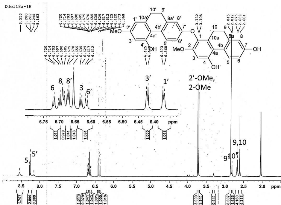
Figure 44 ^1\text{H-NMR} (500 MHz) spectrum of compound DD10
