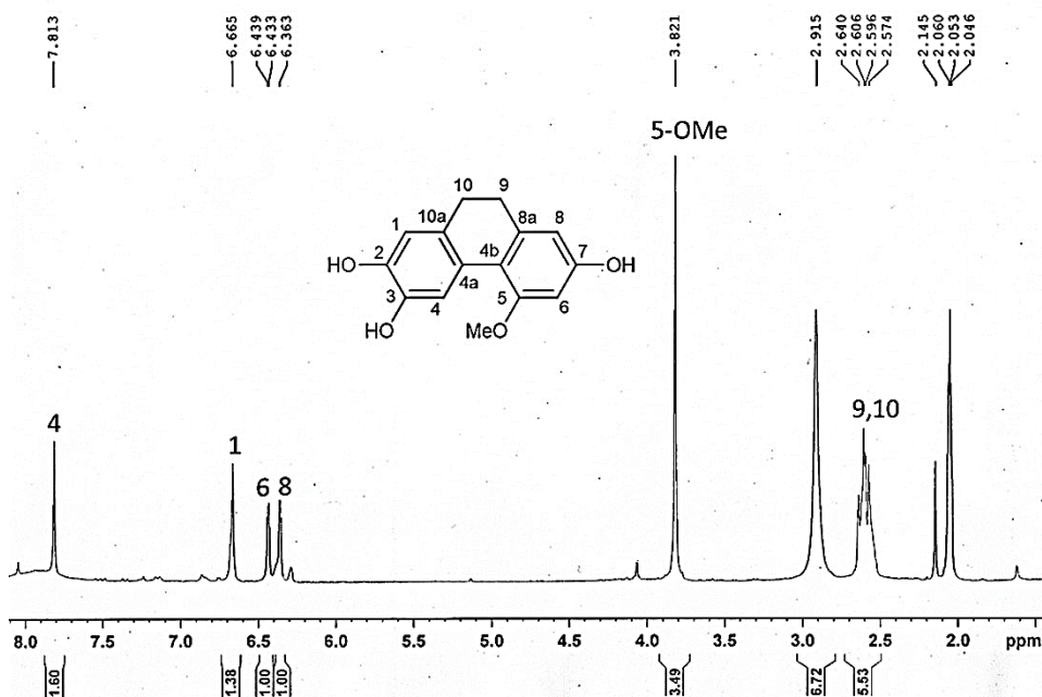
Figure 177 1 H-NMR (300 MHz) spectrum of compound AMF10
