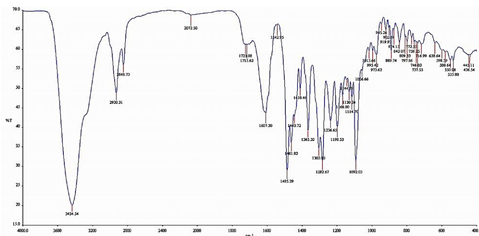
Figure 66 IR spectrum of compound DG2
