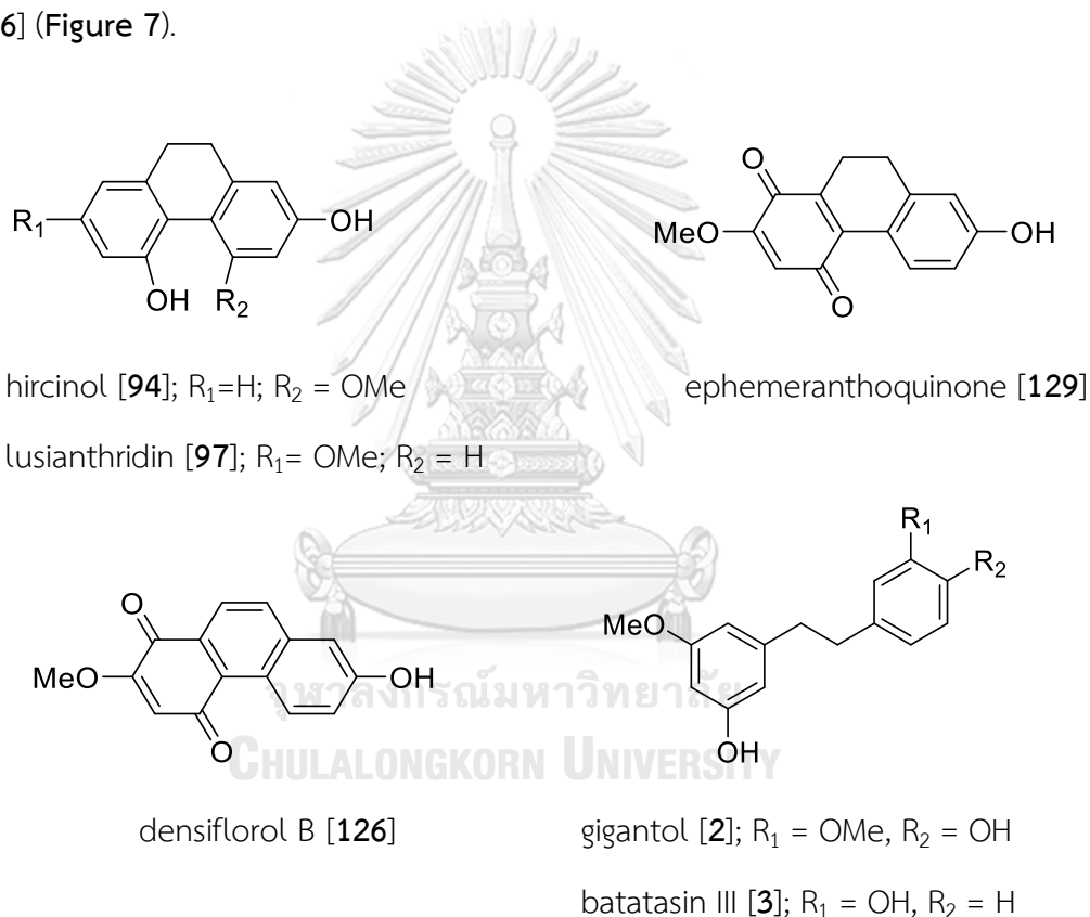
Figure 7 Structures of compounds isolated from Dendrobium delacourii
