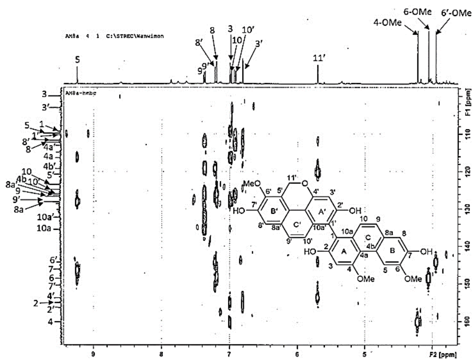
Figure 130 HMBC spectrum of compound AMF2
