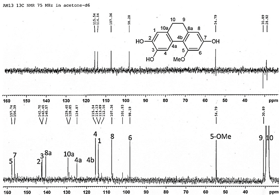
Figure 178 ^{13}\text{C} -NMR (75 MHz) spectrum of compound AMF10
