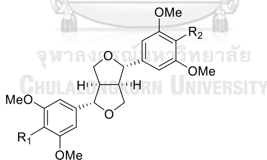
[291] Balanophonin,: R 1 =OH, R 2 =CHO
