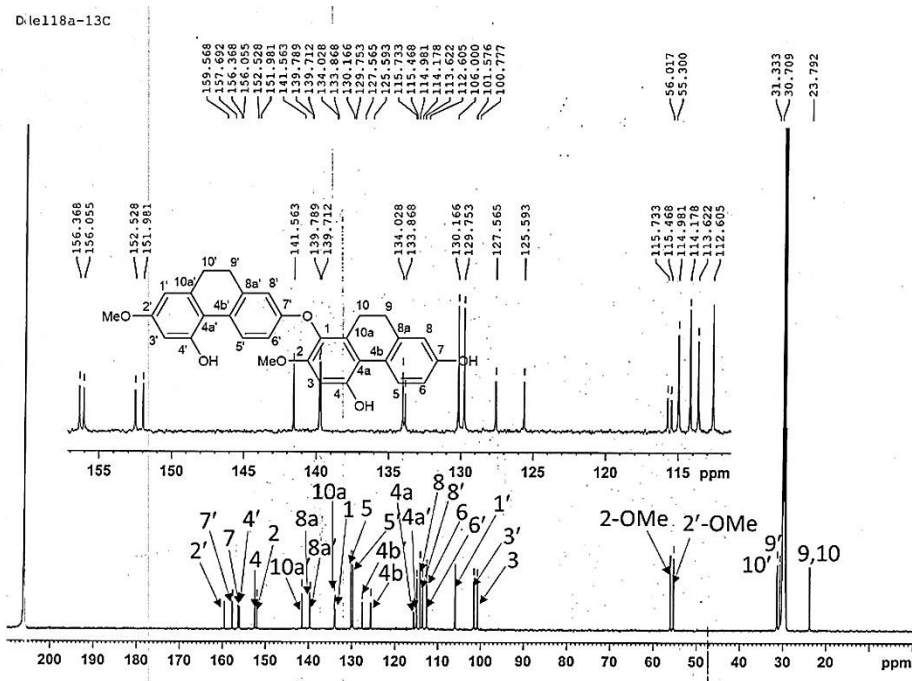
Figure 46 ^{13}\text{C} -NMR (125 MHz) spectrum of compound DD10
