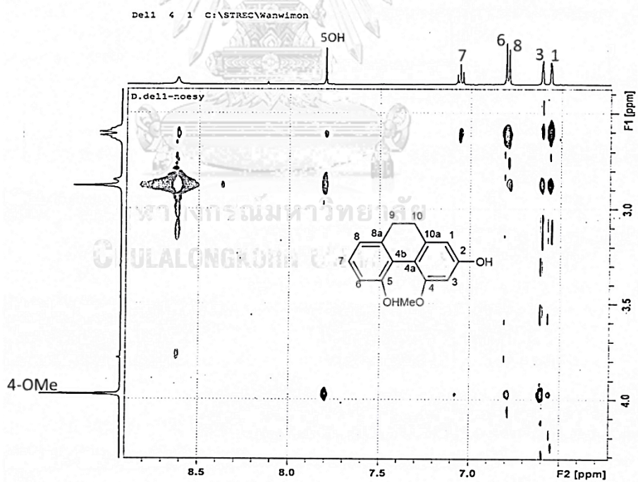
Figure 11 NOESY spectrum of compound DD1
