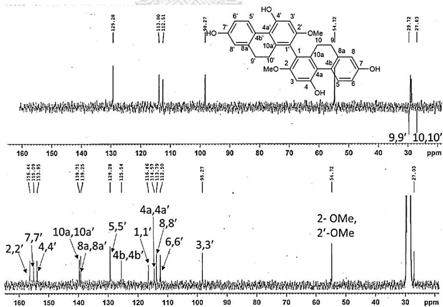
Figure 40 ^{13}\text{C} -NMR (75 MHz) spectrum of compound DD9
