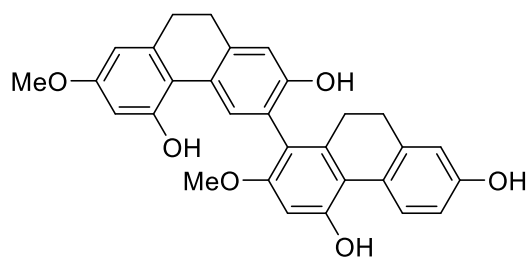
[156] Phoyunnanin C
