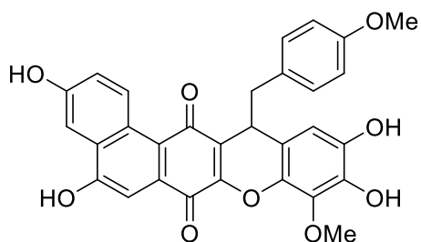
[160] Dendrocandin H
