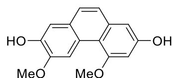
[328] 3,5-Dimethoxyphenanthrene-2,7-diol
