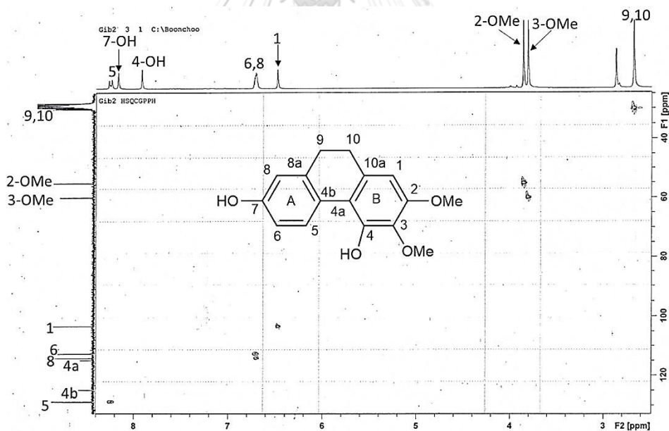
Figure 75 ^{13}\text{C} -NMR (75 MHz) spectrum of compound DG3
