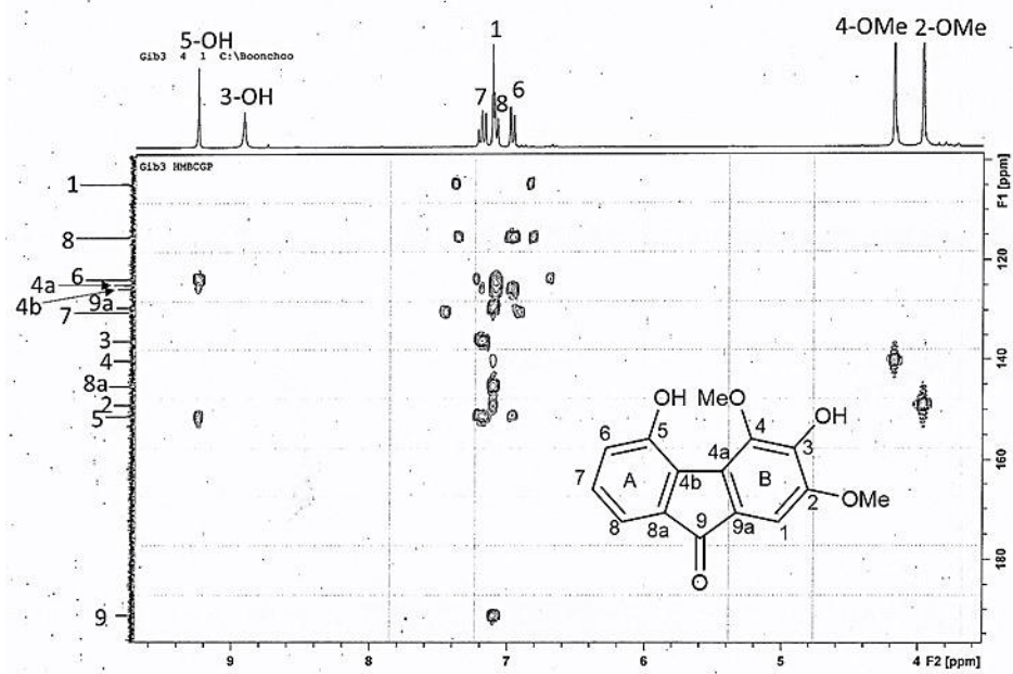
Figure 83 HMBC spectrum of compound DG4
