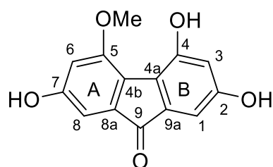
denchrysan A [305]
