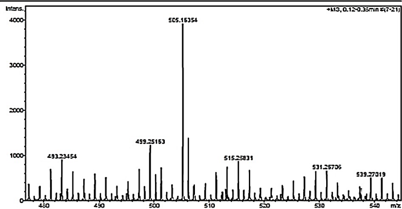
Figure 49 Mass spectrum of compound DD11
