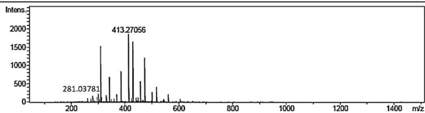
Figure 102 Mass spectrum of compound DG8
