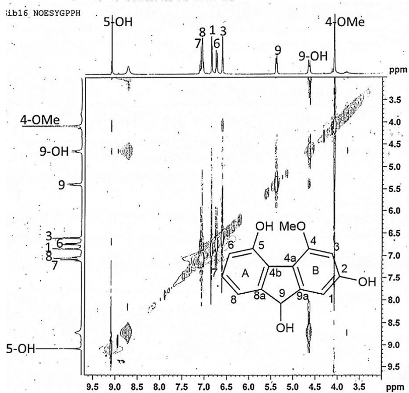
Figure 112 HMBC spectrum of compound DG9
