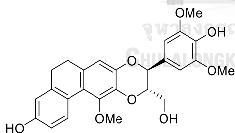
[136] Dendrocandin P2
