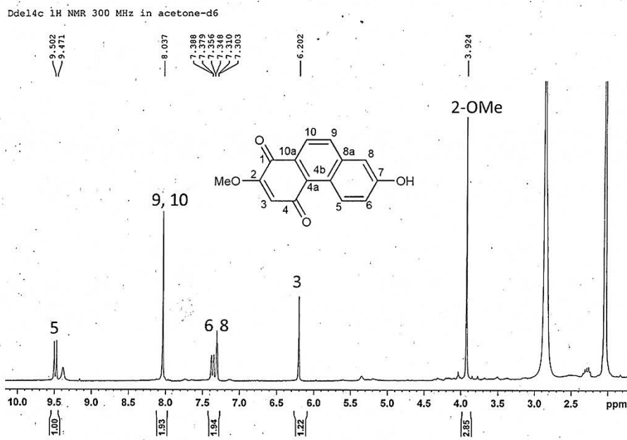
Figure 17 ^1\text{H-NMR} (300 MHz) spectrum of compound DD3
