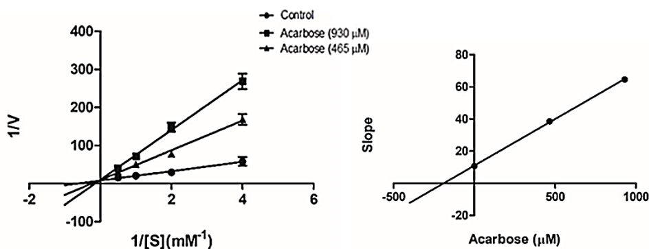
Figure 184 Lineweaver–Burk plot and secondary plot of acarbose
