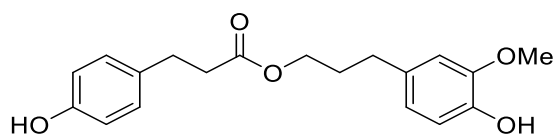
[275] Dihydroconiferyl dihydro- p -coumarate
