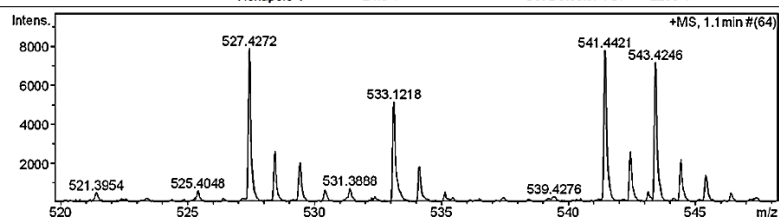
Figure 132 Mass spectrum of compound AMF3
