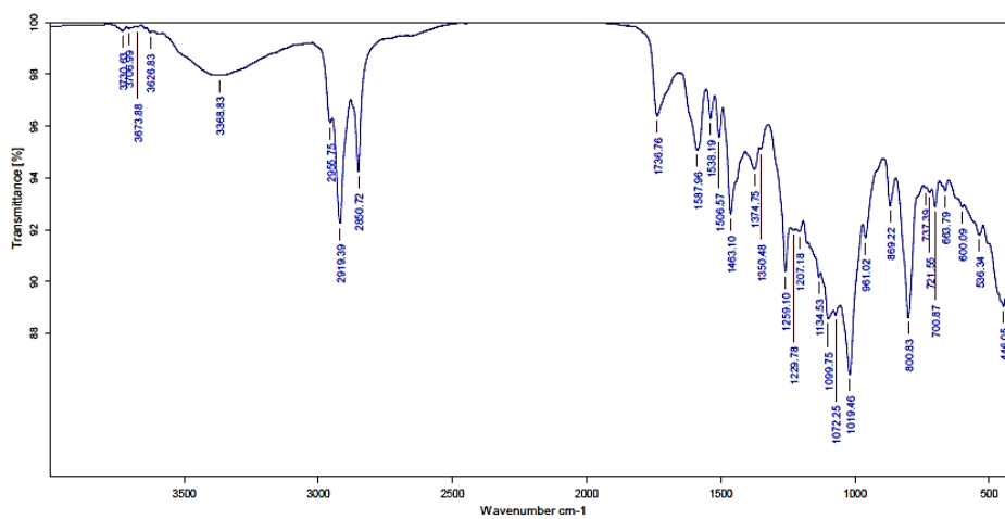
Figure 126 FT-IR spectrum of compound AMF2
