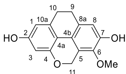
imbricatin [330]
