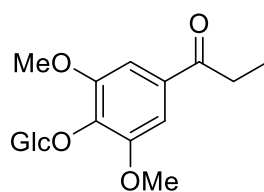
[276] 1-[4-( \beta -D-glucopyranosyloxy)-3,5-dimethoxyphenyl]-1-propanone
