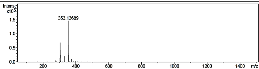
Figure 170 Mass spectrum of compound AMF9
