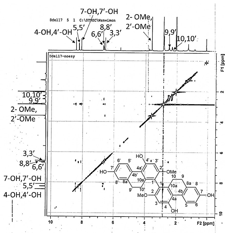
Figure 39 NOESY spectrum of compound DD9
