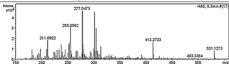
Figure 16 Mass spectrum of compound DD3
