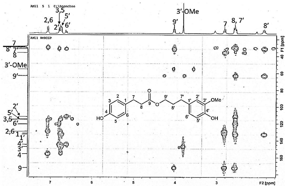
Figure 174 HMBC spectrum of compound AMF9
