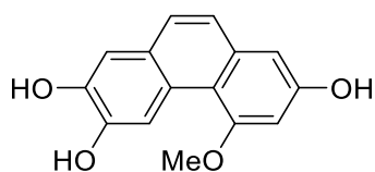
[325] Aerosanthrene
