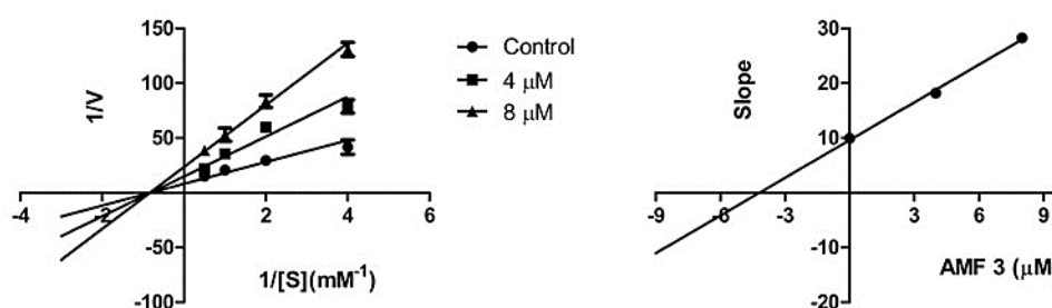
Figure 186 Lineweaver–Burk plot and secondary plot of compound AMF3 [339]
