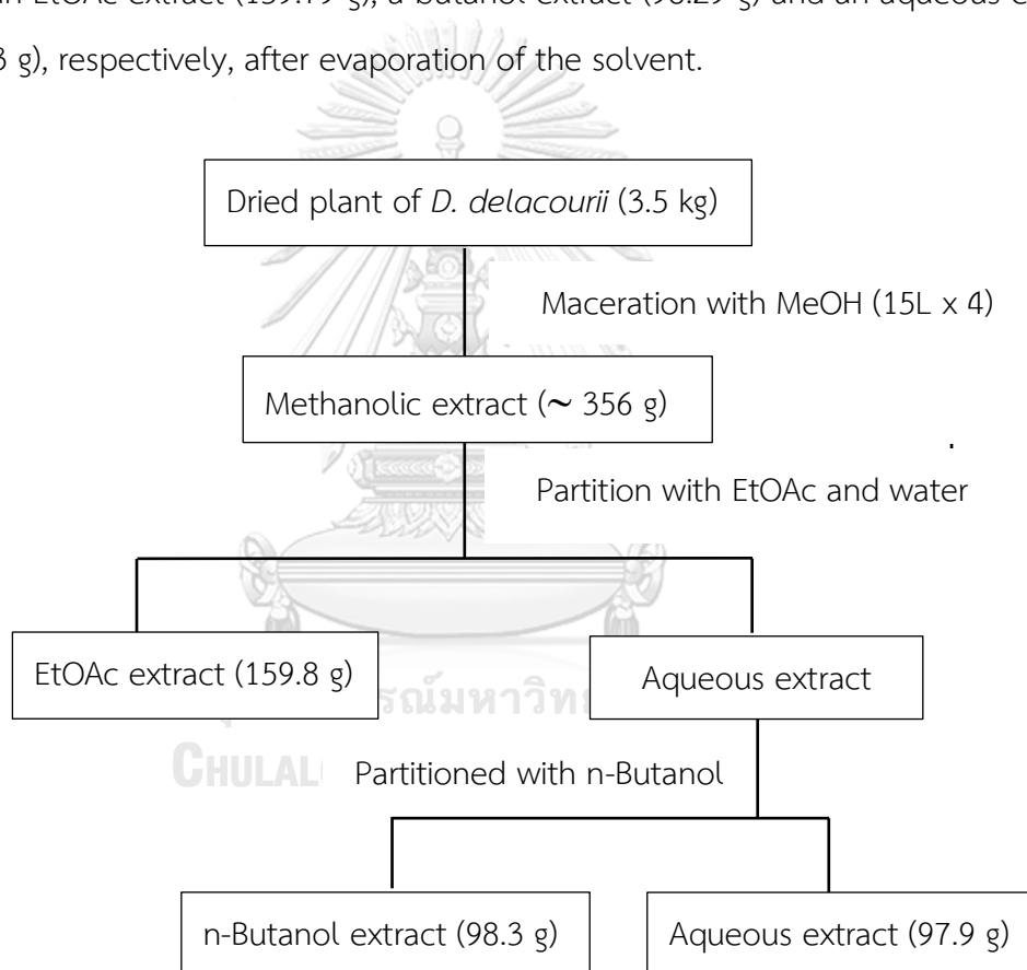
Scheme 1 Extraction steps of Dendrobium delacourii
