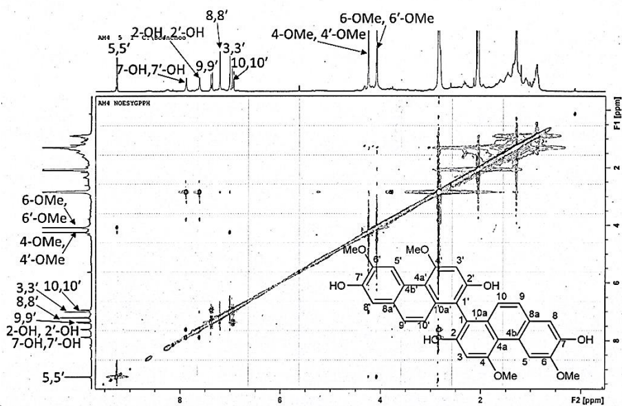
Figure 168 HMBC spectrum of compound AMF8
