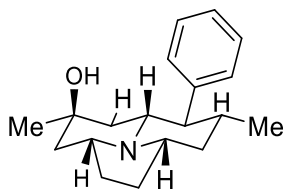
[315] Crepidatumine A
