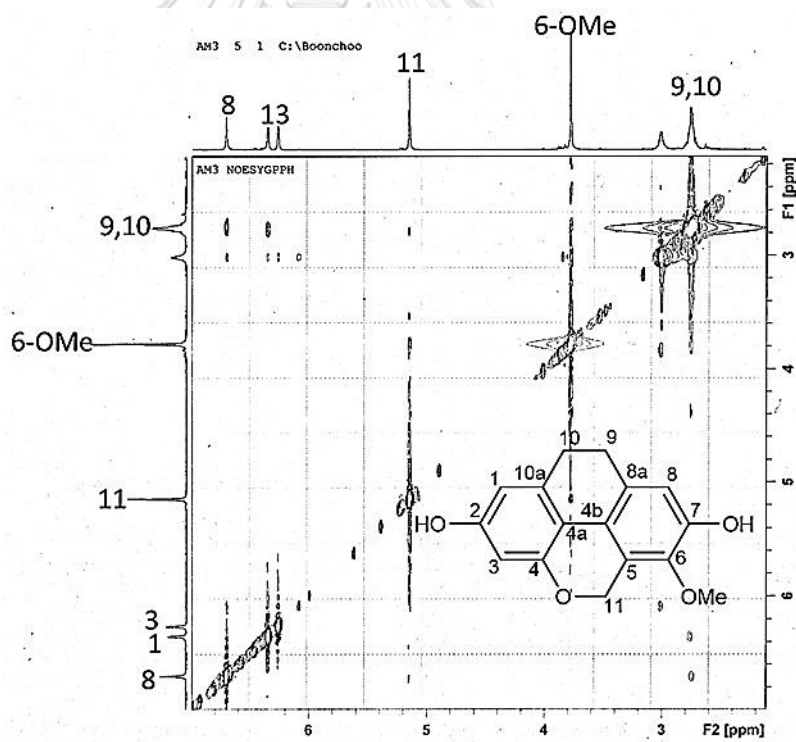
Figure 162 HMBC spectrum of compound AMF7
