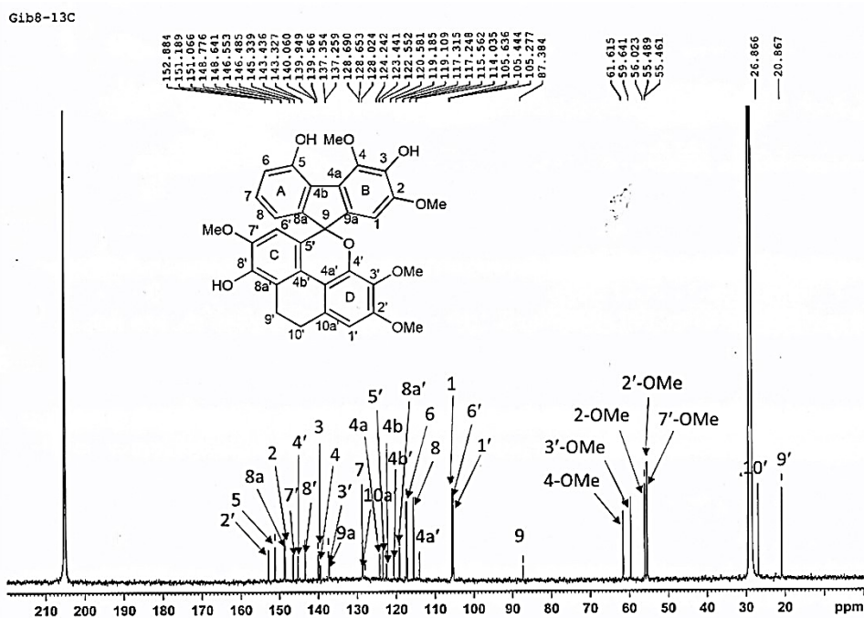
Figure 68 ^{13}\text{C} -NMR (125 MHz) of compound DG2
