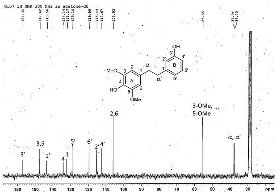
Figure 93 ^{13}\text{C} -NMR (75 MHz) spectrum of compound DG6
