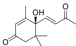
[321] Dehydrovomifoliol
