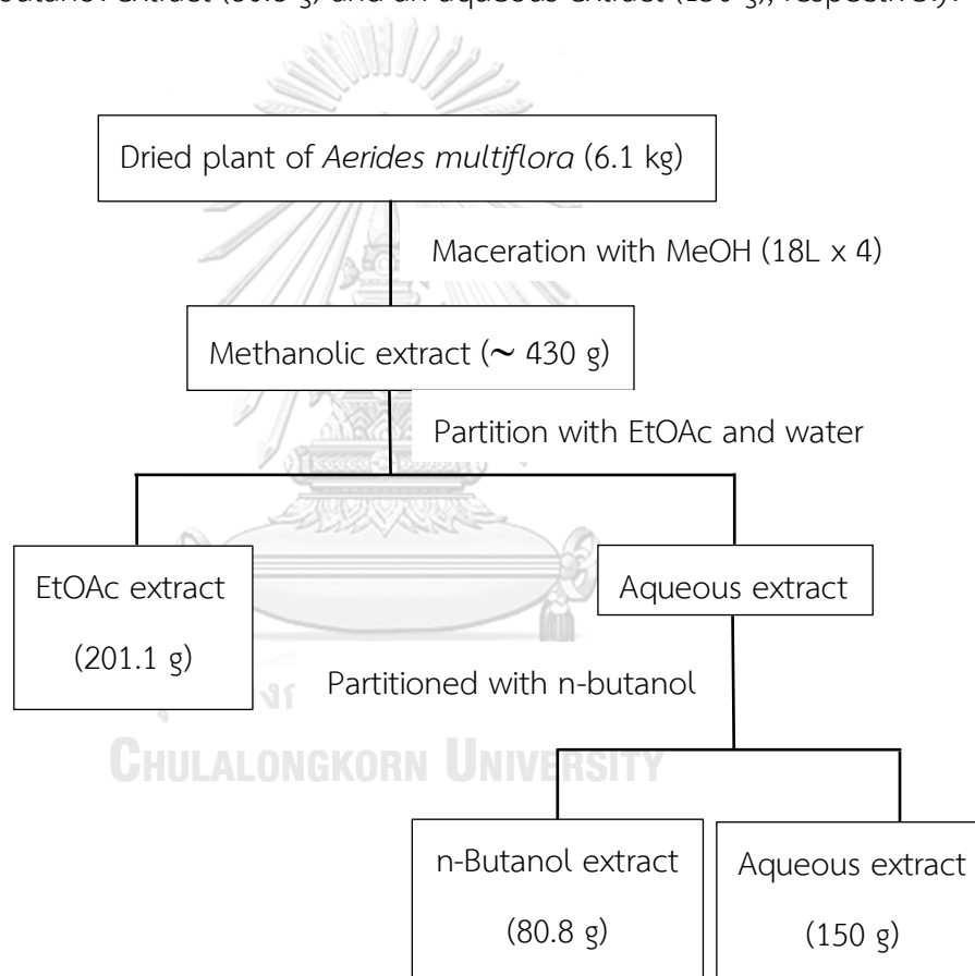
Scheme 5 Extraction steps of Aerides multiflora
