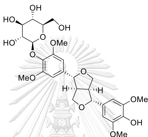
Syringaresinol-4'-O-D-glucopyranoside [17]
