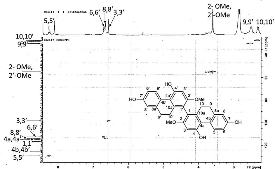
Figure 41 HSQC spectrum of compound DD9
