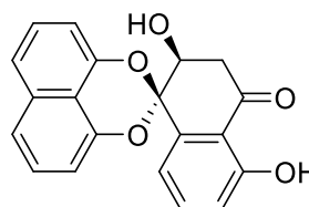
[320] Palmarumycin JC2
