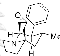
[316] Crepidatumine B
