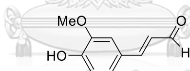
Coniferyl aldehyde [18]
