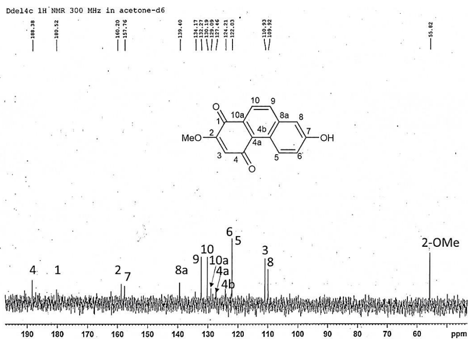
Figure 18 ^{13}\text{C} -NMR (75 MHz) spectrum of compound DD3
