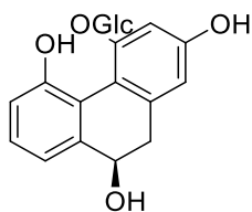
[141] 2,4,5,9S-Tetrahydroxy-9,10-dihydro-phenanthrene-4-O- \beta -D-glucopyranoside
