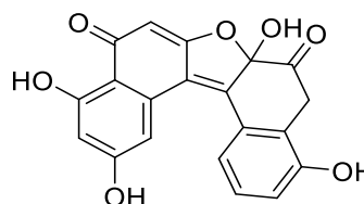
[324] RF-3192C
