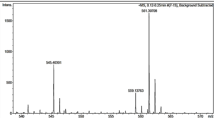
Figure 124 Mass spectrum of compound AMF2
