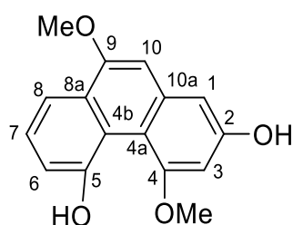
4,9-dimethoxy-2,5-phenanthrenediol [105]
