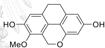
[330] Imbricatin
