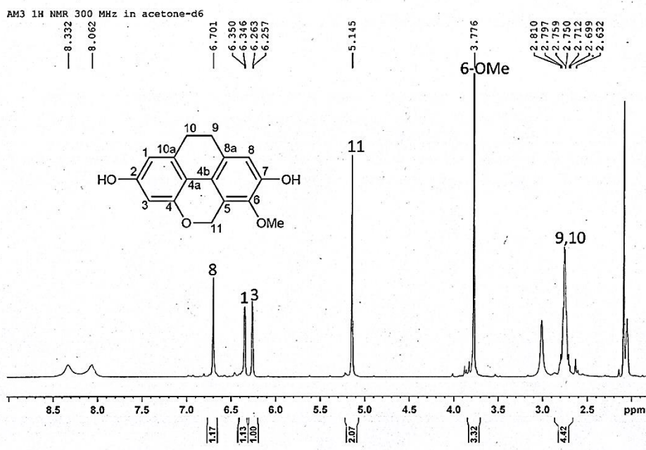
Figure 159 1 H-NMR (300 MHz) spectrum of compound AMF7
