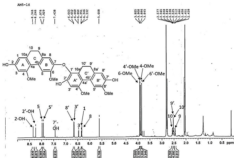
Figure 118 ^1\text{H-NMR} (500 MHz) spectrum of compound AMF1
