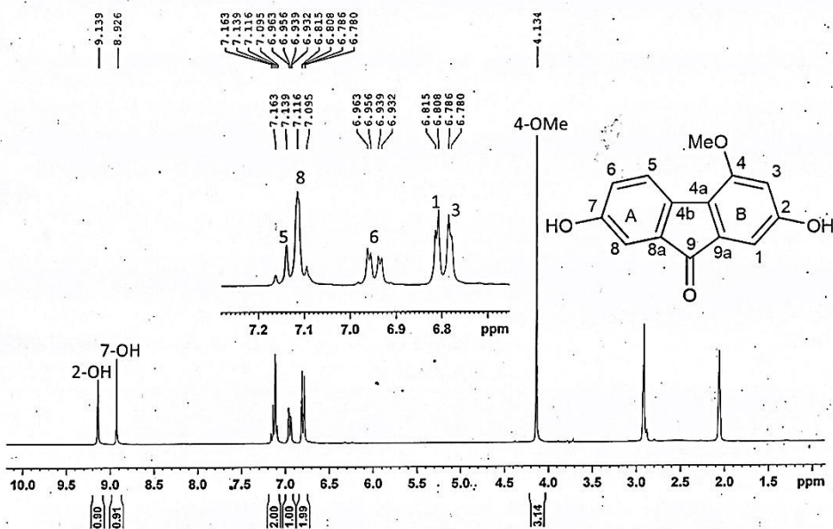
Figure 86 ^1\text{H-NMR} (300 MHz) spectrum of compound DG5
