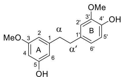
gigantol [2]
