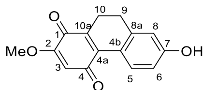
ephemeranthoquinone [ 129 ]
