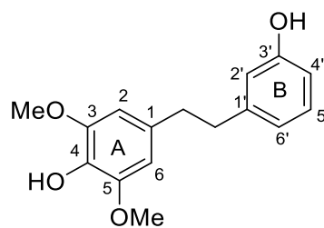
aloifol I [20]
