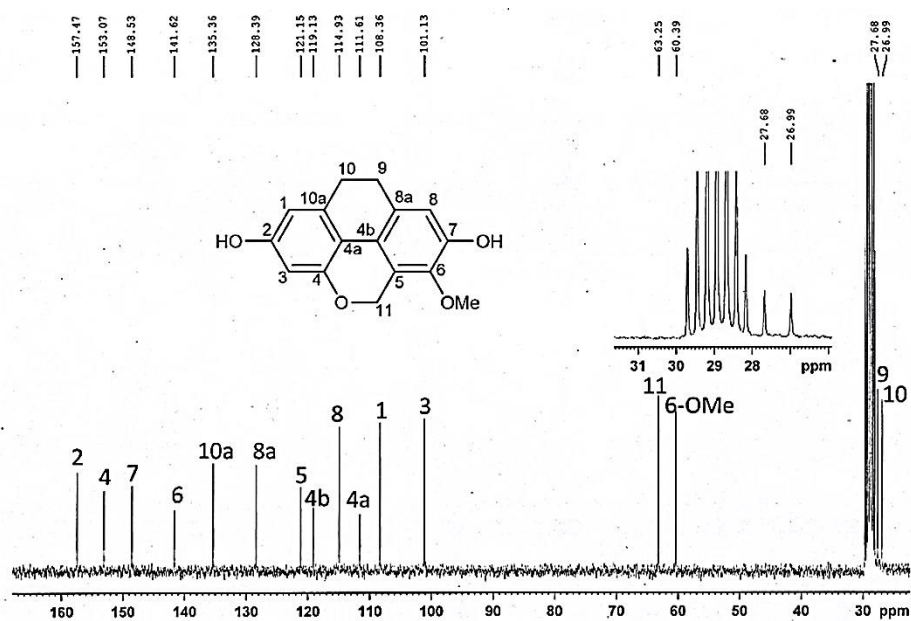
Figure 160 ^{13}\text{C} -NMR (75 MHz) spectrum of compound AMF7
