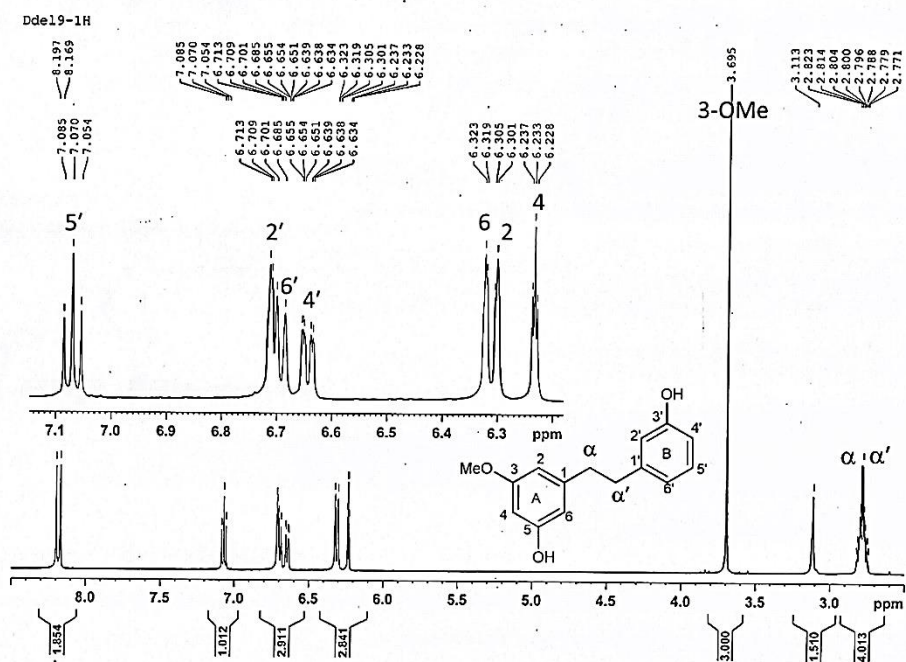
Figure 32 ^1\text{H-NMR} (500 MHz) spectrum of compound DD7
