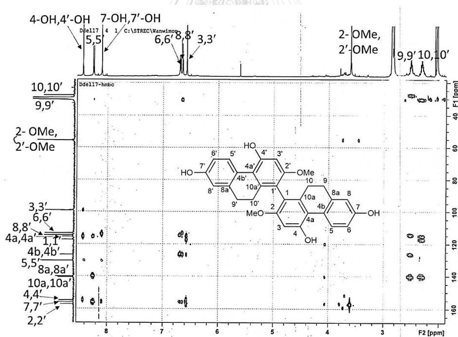
Figure 42 HMBC spectrum of compound DD9
