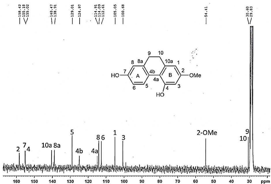
Figure 98 ^{13}\text{C} -NMR (75 MHz) spectrum of compound DG7
