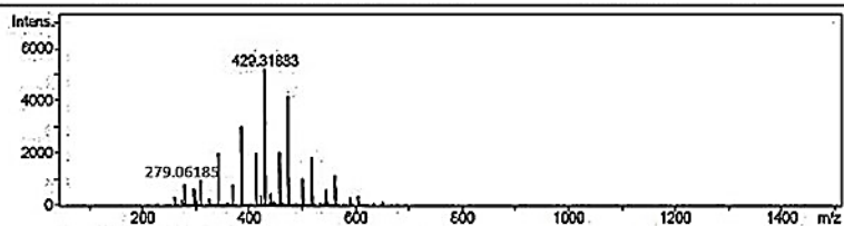
Figure 12 Mass spectrum of compound DD2
