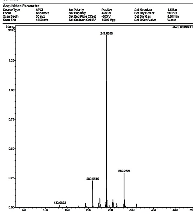
Figure 20 Mass spectrum of compound DD4
