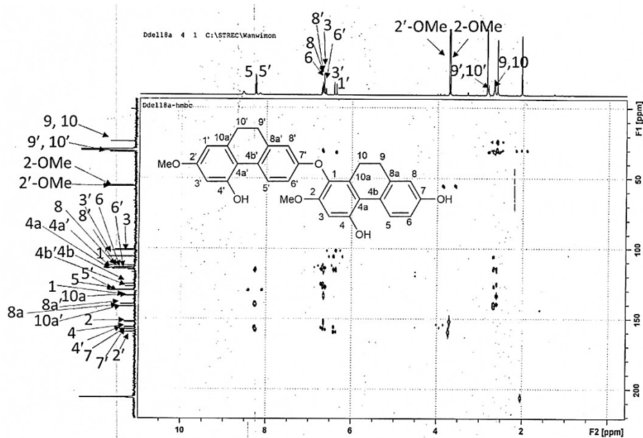
Figure 48 HMBC spectrum of compound DD10
