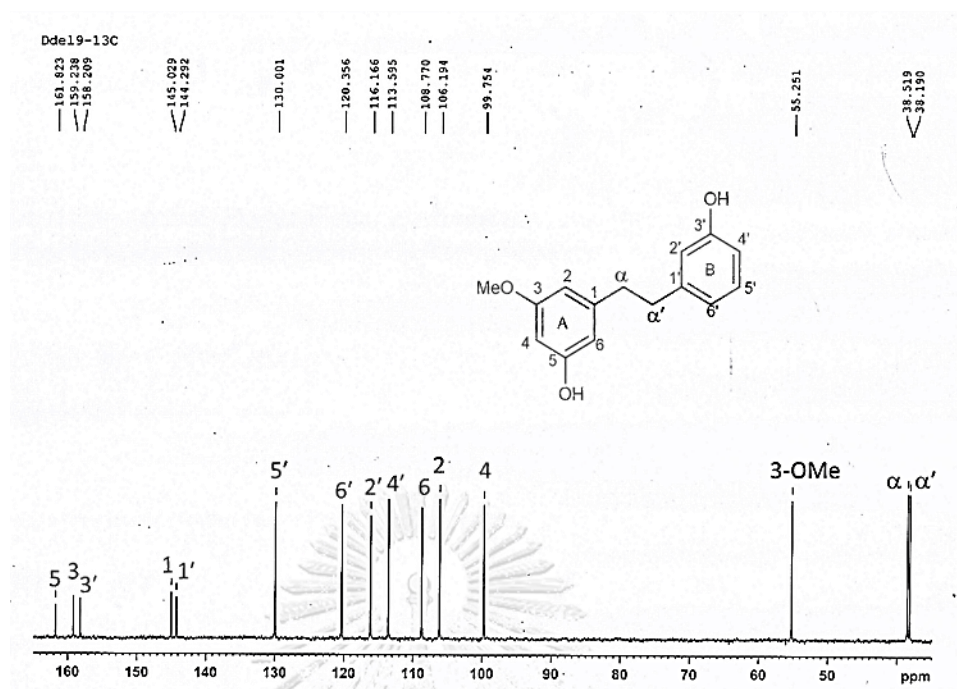
Figure 33 ^{13}\text{C} -NMR (125 MHz) spectrum of compound DD7
