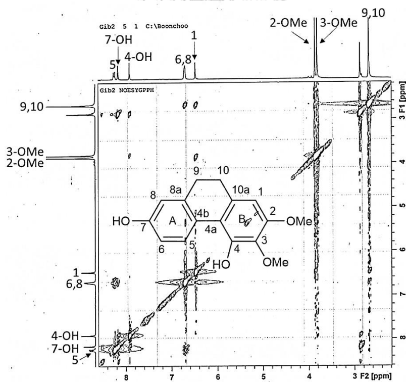
Figure 78 NOESY spectrum of compound DG3
