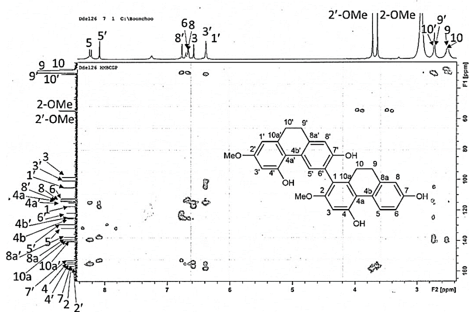
Figure 53 HMBC spectrum of compound DD11
