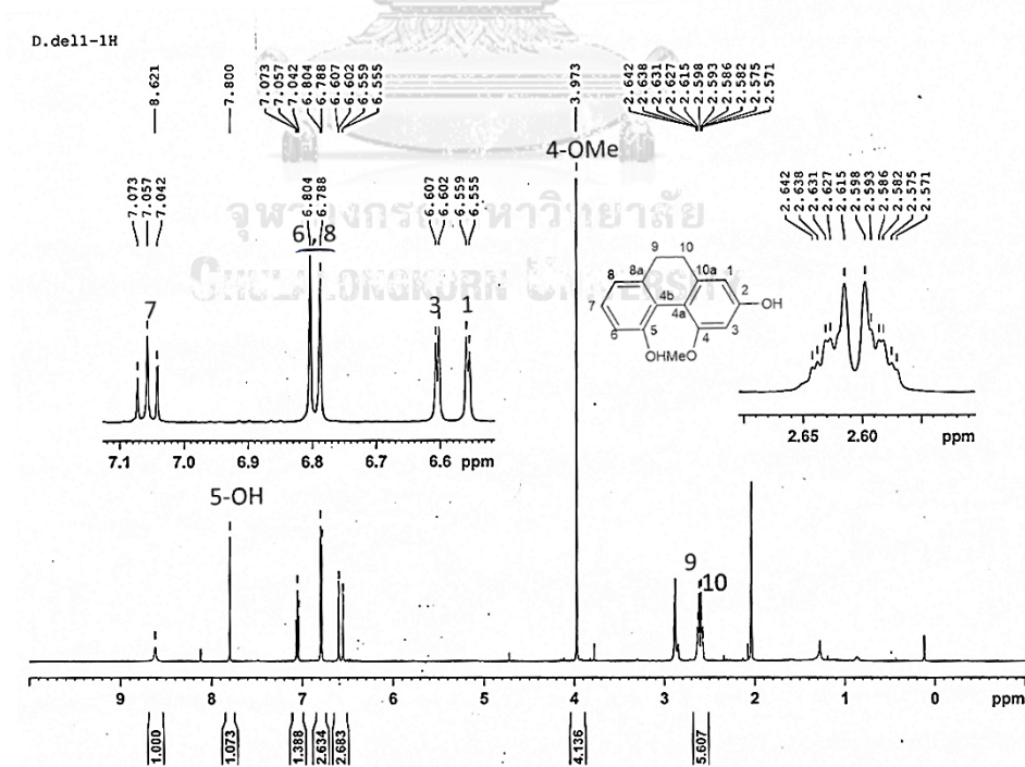
Figure 9 ^1\text{H-NMR} (500 MHz) spectrum of compound DD1
