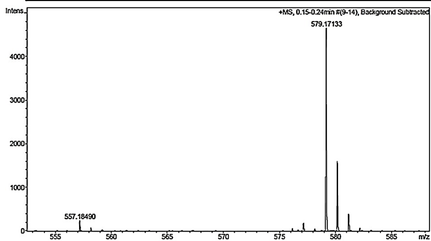
Figure 64 Mass spectrum of compound DG2
