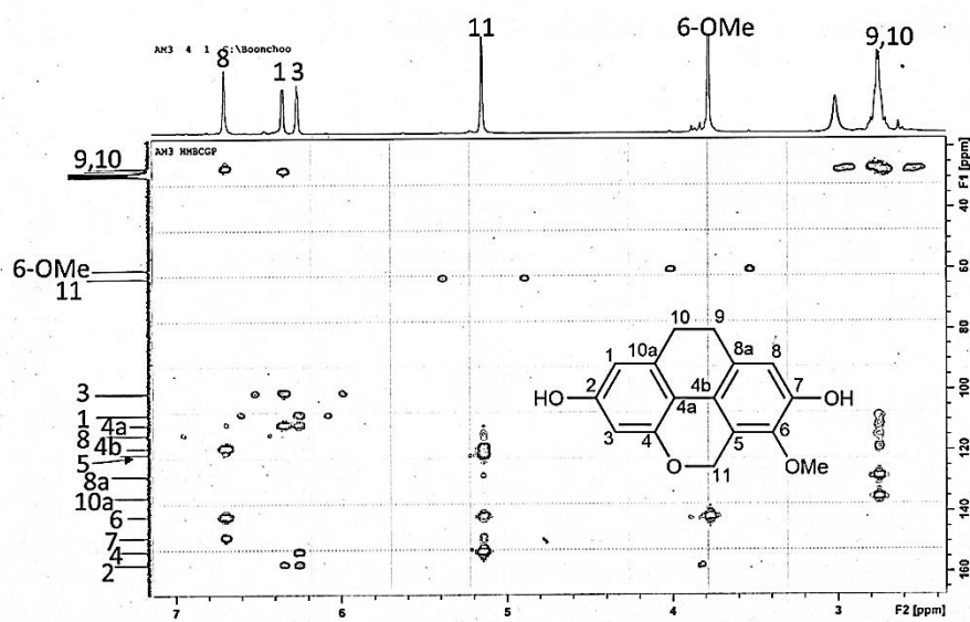
Figure 162 HMBC spectrum of compound AMF7
