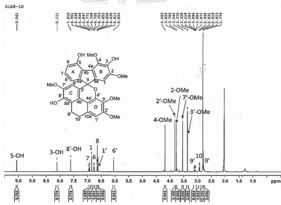
Figure 67 ^1\text{H-NMR} (500 MHz) spectrum of compound DG2
