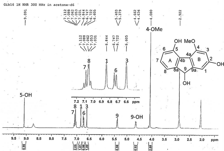
Figure 109 1 H-NMR (300 MHz) spectrum of compound DG9
