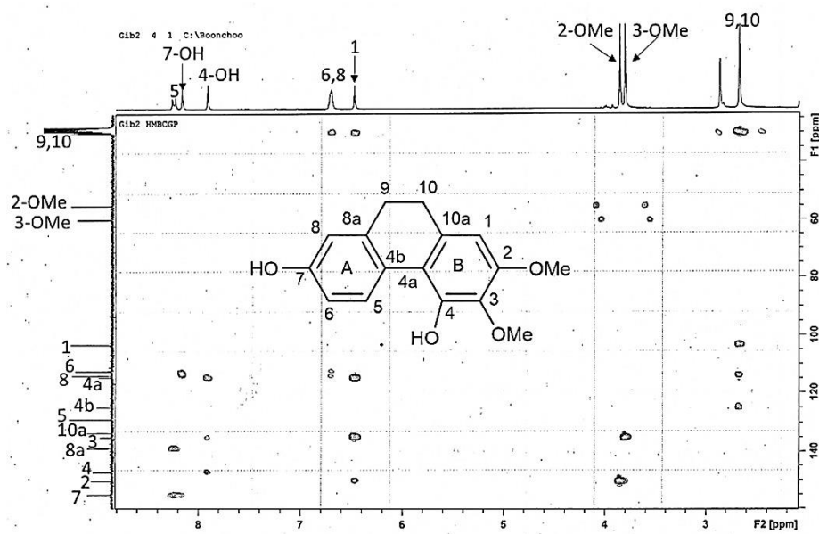
Figure 77 HMBC spectrum of compound DG3
