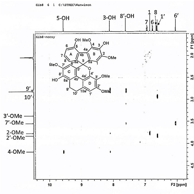
Figure 71 NOESY spectrum of compound DG2
