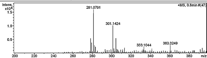
Figure 176 Mass spectrum of compound AMF10
