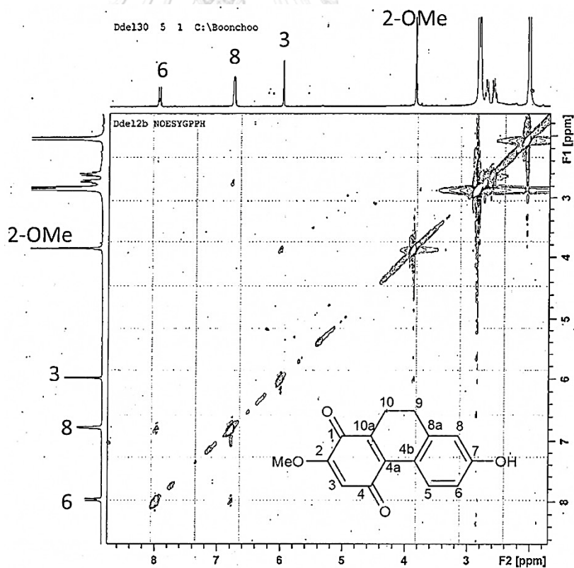
Figure 15 NOESY spectrum of compound DD2
