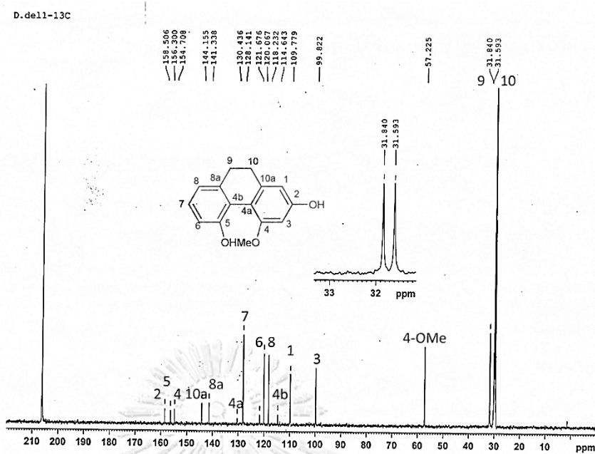
Figure 10 ^{13}\text{C} -NMR (125 MHz) spectrum of compound DD1
