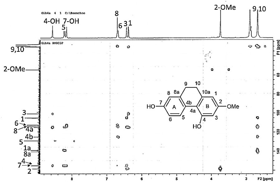
Figure 100 HMBC spectrum of compound DG7
