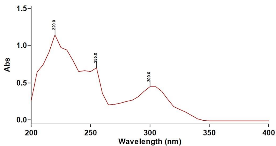
Figure 57 UV spectrum of compound DG1
