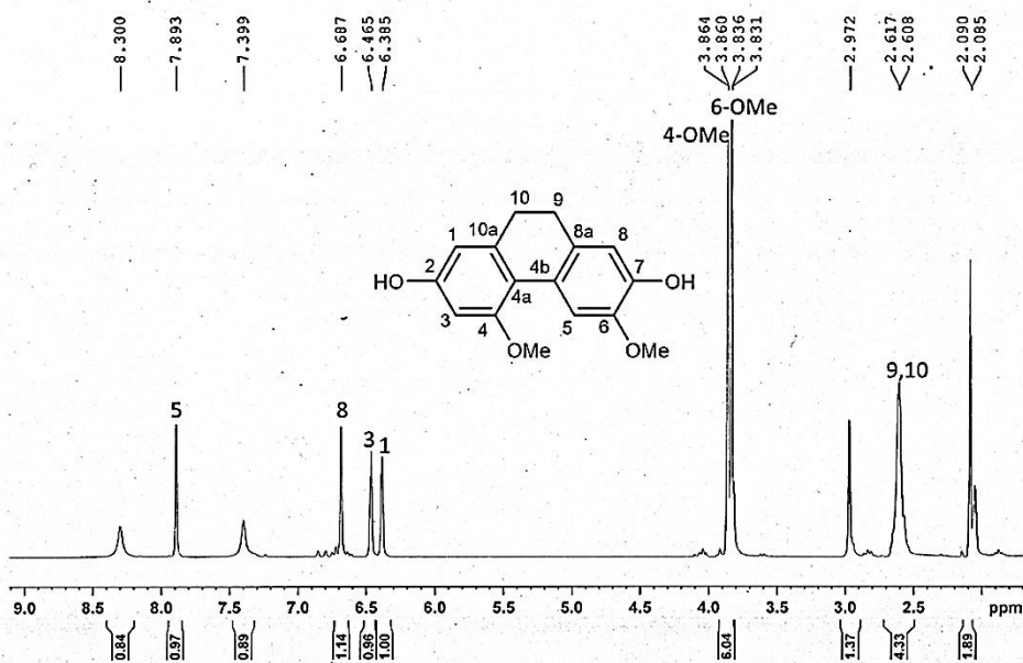
Figure 149 1 H-NMR (300 MHz) spectrum of compound AMF5
