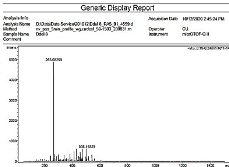
Figure 34 Mass spectrum of compound DD8
