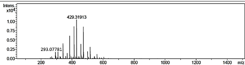
Figure 158 Mass spectrum of compound AMF7
