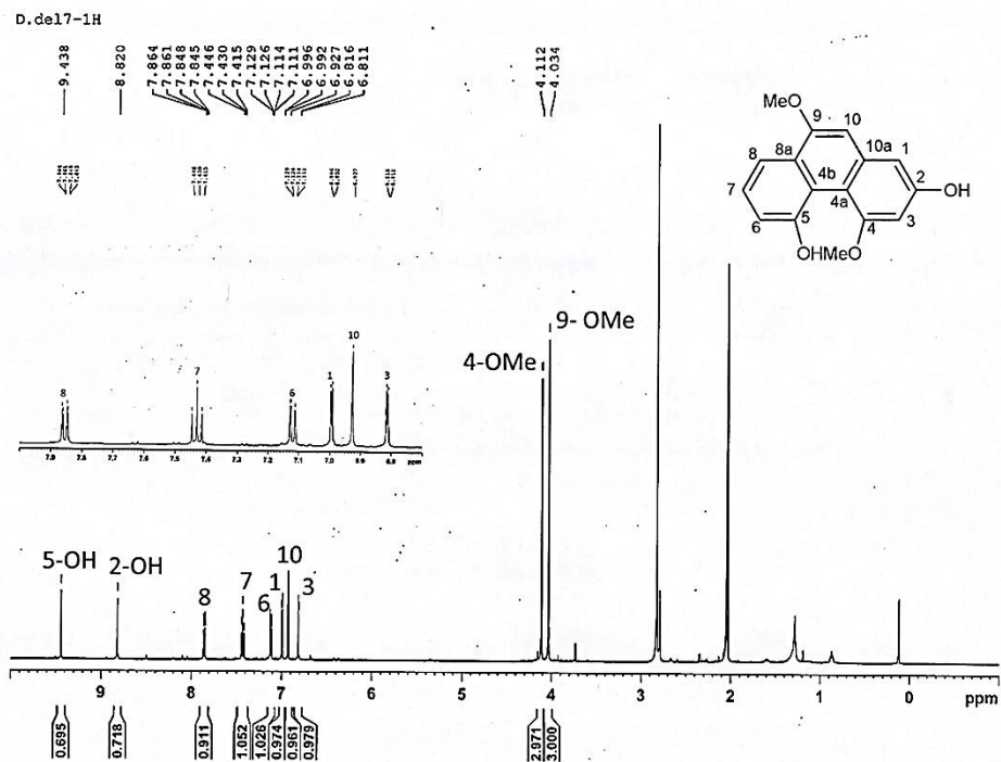
Figure 25 ^1\text{H-NMR} (500 MHz) spectrum of compound DD5
