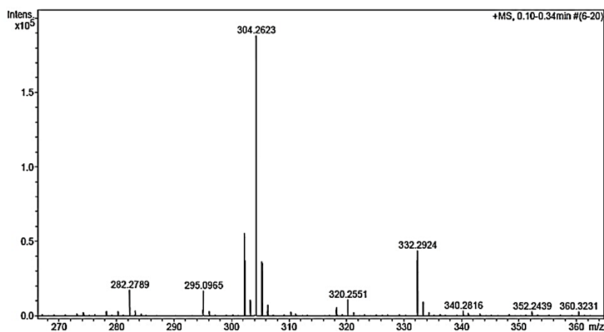
Figure 73 Mass spectrum of compound DG3
