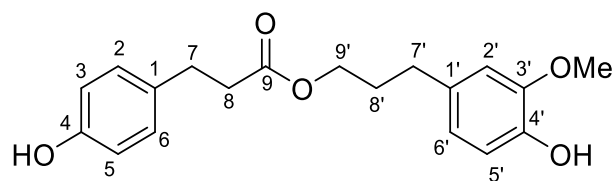
dihydrocorniferyldihydro- p -coumarate [275]
