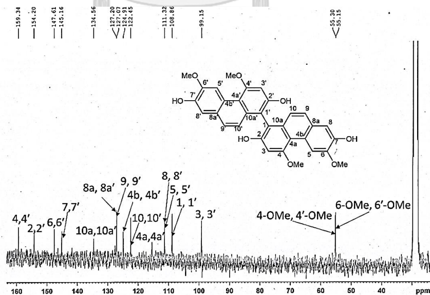
Figure 165 ^{13}\text{C} -NMR (75 MHz) spectrum of compound AMF8
