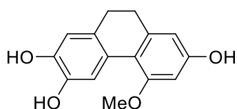
[327] 5-Methoxy-9,10-dihydro- 2,3,7-phenanthrenetriol
