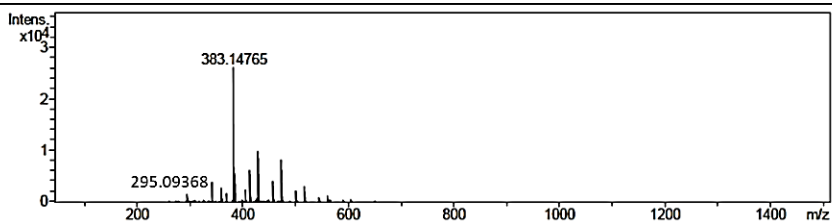
Figure 148 Mass spectrum of compound AMF5
