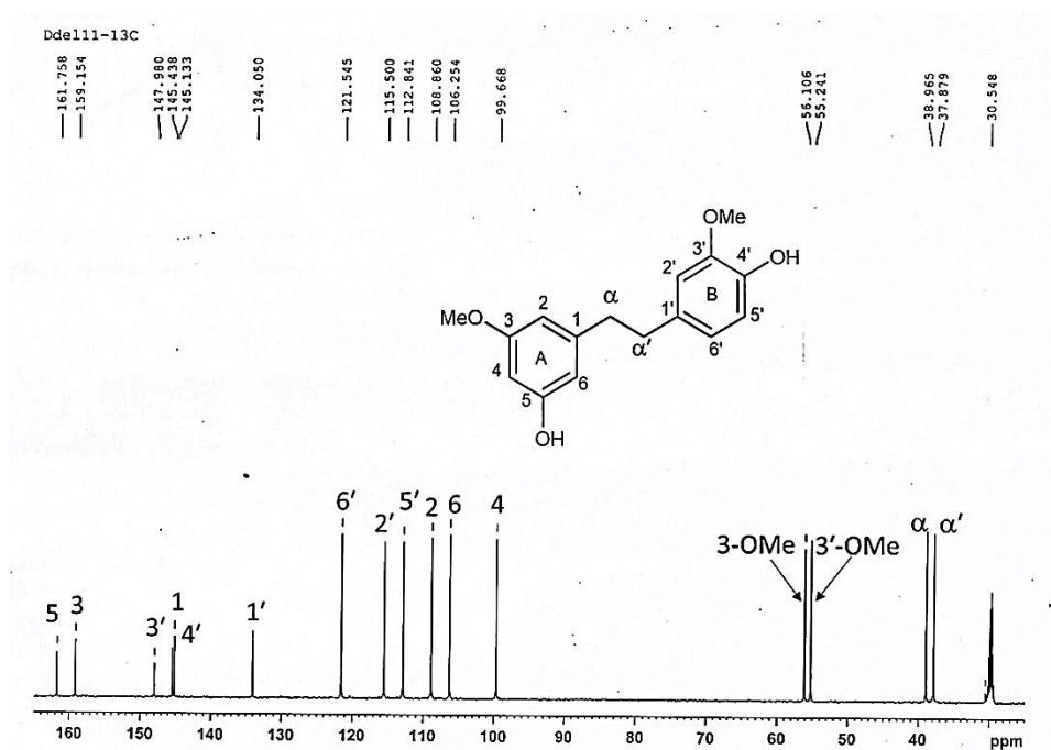
Figure 30 ^{13}\text{C} -NMR (125 MHz) spectrum of compound DD6
