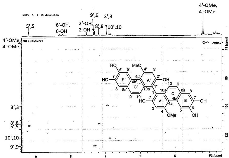
Figure 137 HSQC spectrum of compound AMF3
