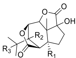
[222] Amotin: R 1 = R 3 = H, R 2 = OH
