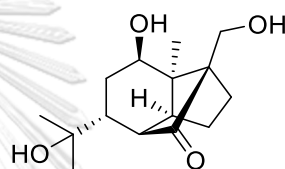
[208] Dendronobilin K
