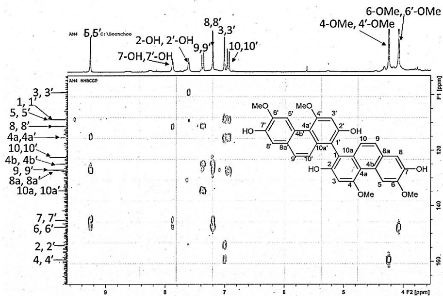
Figure 168 HMBC spectrum of compound AMF8
