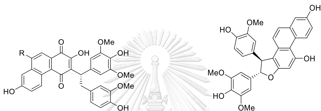
[161] Loddigesiinol G: R = H
