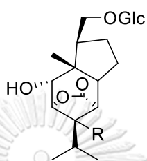
[217] Dendroside F; R = H
