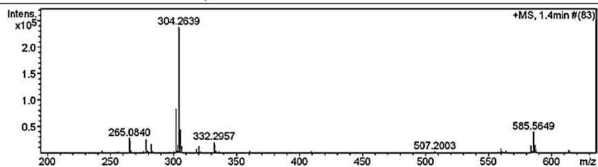
Figure 96 Mass spectrum of compound DG7
