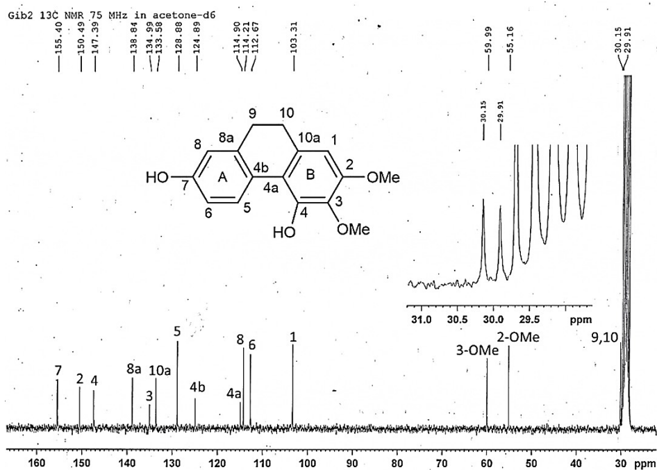
Figure 75 ^{13}\text{C} -NMR (75 MHz) spectrum of compound DG3
