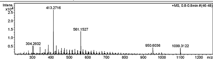
Figure 164 Mass spectrum of compound AMF8
