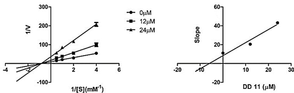
Figure 183 Lineweaver-Burk plot and secondary plot of compound DD11 [ 156 ]
