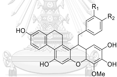
[158] Dendrosignatol: R 1 = H, R 2 = OMe
