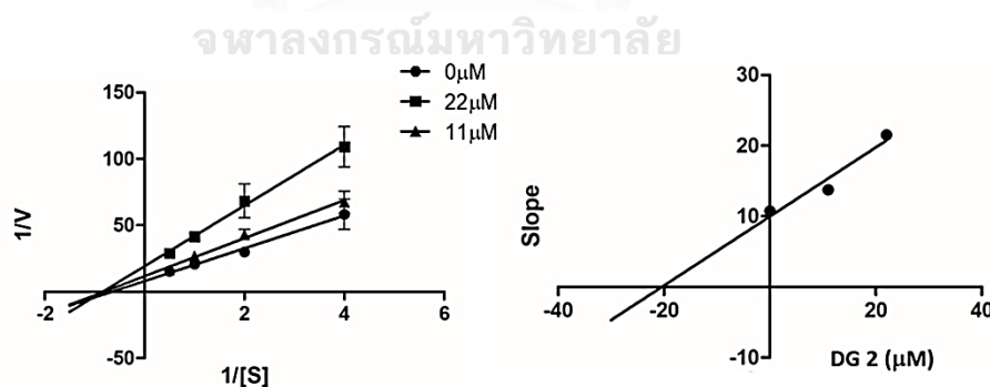
Figure 185 Lineweaver–Burk plot and secondary plot of compound DG2 [336]
