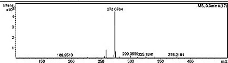
Figure 56 Mass spectrum of compound DG1
