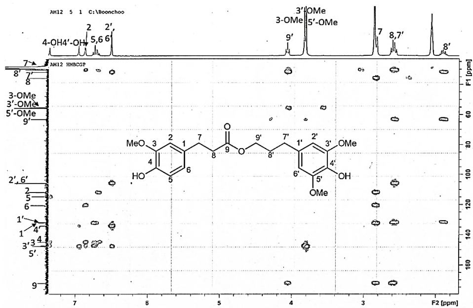
Figure 146 HMBC spectrum of compound AMF4
