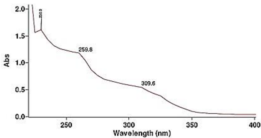
Figure 65 UV spectrum of compound DG2
