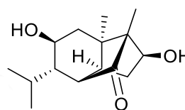
[198] Dendronobilin A
