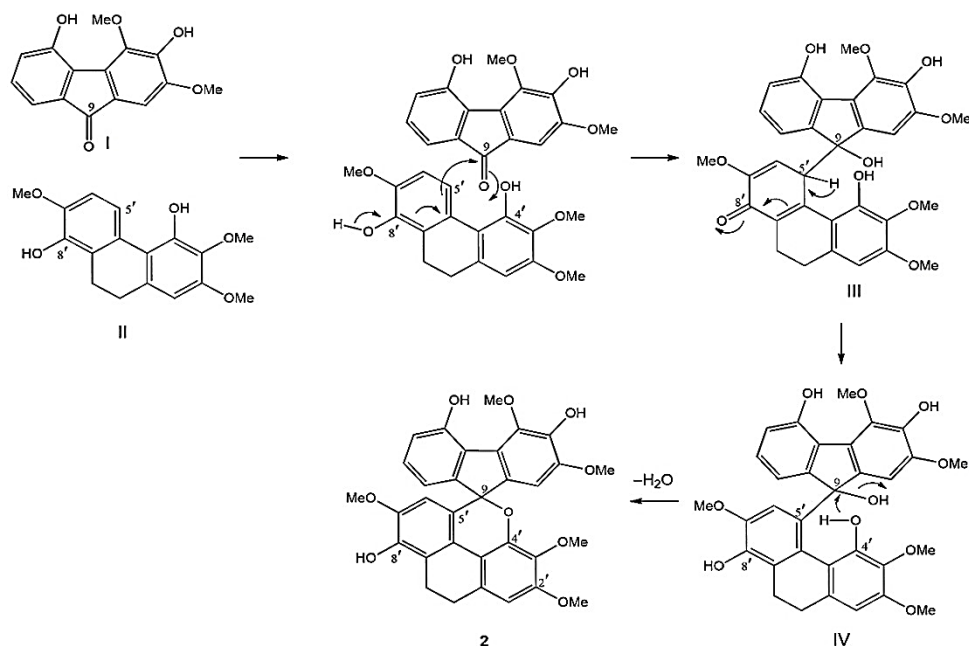
Figure 72 Possible biogenesis of dendrogibsol
