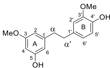
gigantol [2]
