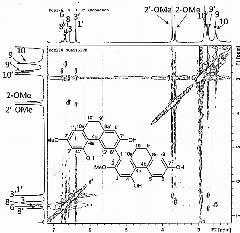
Figure 54 NOESY spectrum of compound DD11
