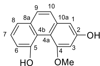
Moscatin [110]
