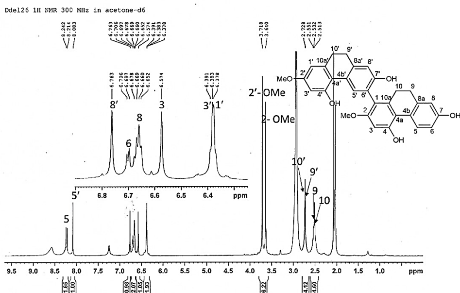
Figure 50 1 H-NMR (300 MHz) spectrum of compound DD11
