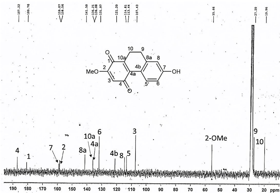
Figure 14 ^{13}\text{C} -NMR (75 MHz) spectrum of compound DD2
