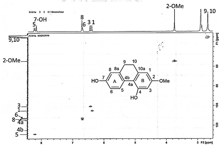
Figure 98 ^{13}\text{C} -NMR (75 MHz) spectrum of compound DG7
