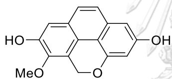
[329] 3-Methoxy-2,7-dihydroxy- 5H-phenanthro[4,5-bcd]pyran
