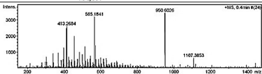
Figure 115 Mass spectrum of compound AMF1
