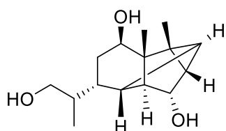
[191] Dendrobane A
