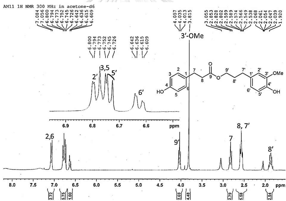
Figure 171 1 H-NMR (300 MHz) spectrum of compound AMF9
