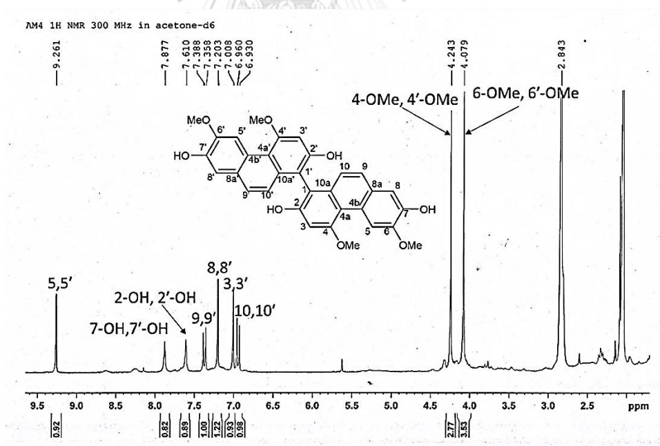
Figure 167 ^1\text{H-NMR} (300 MHz) spectrum of compound AMF8
