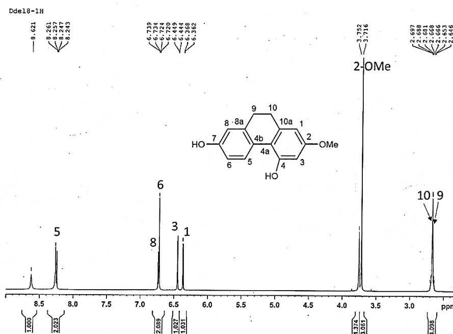
Figure 35 ^1\text{H-NMR} (500 MHz) spectrum of compound DD8
