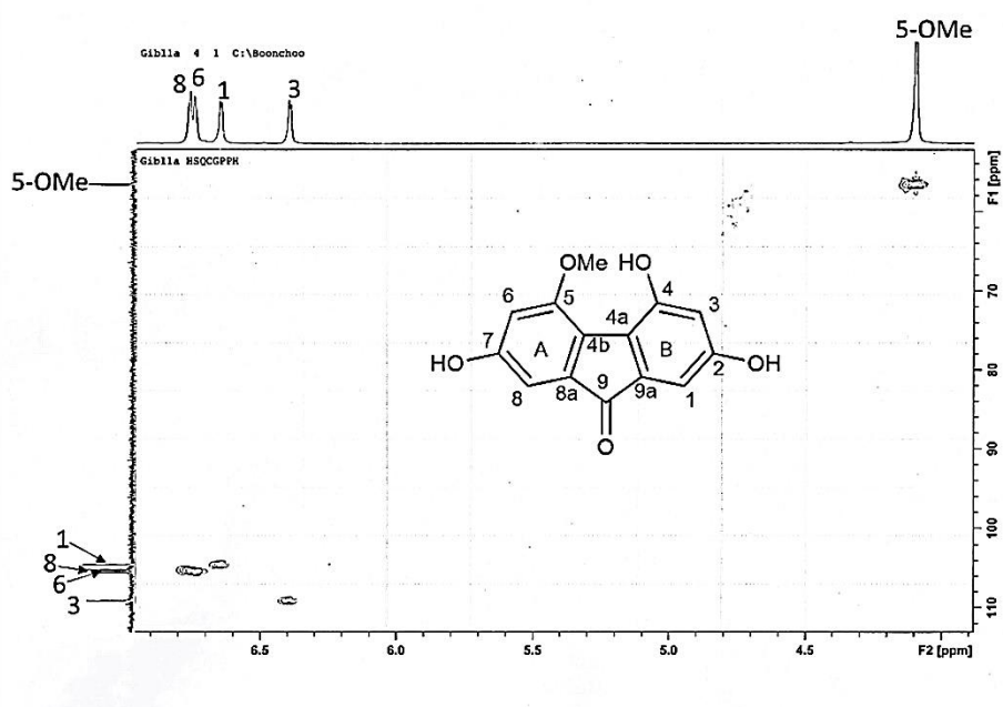
Figure 105 HSQC spectrum of compound DG8
