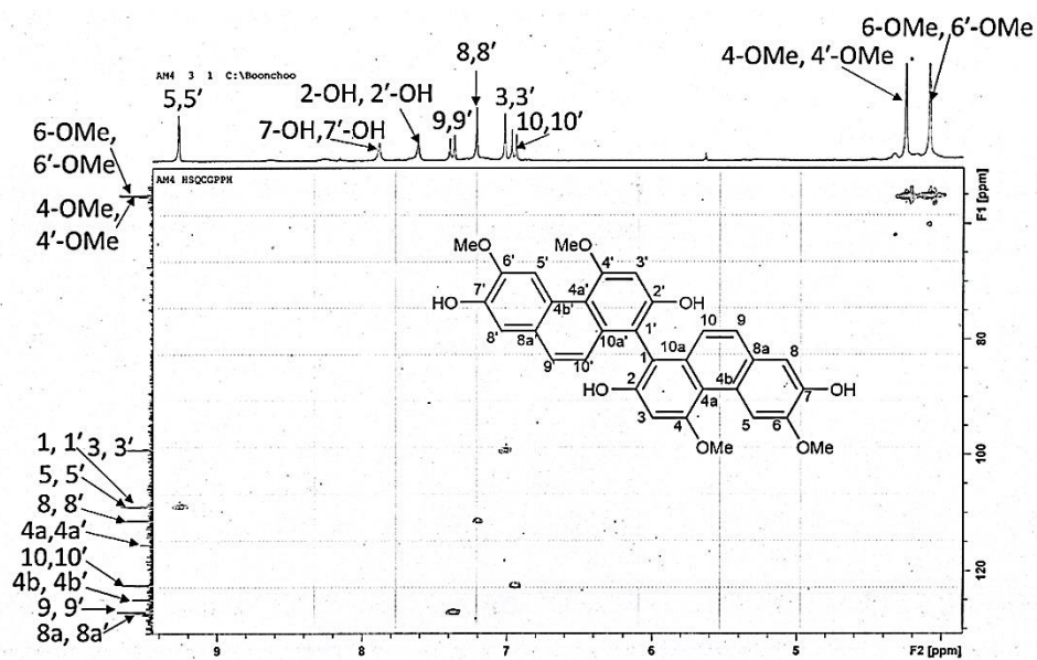
Figure 166 HSQC spectrum of compound AMF8
