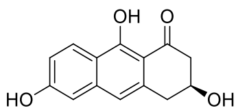
[319] 3,6,9-Trihydroxy-3,4-dihydroanthracen-1(2 H )-one
