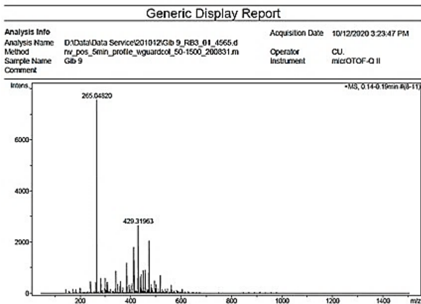
Figure 85 Mass spectrum of compound DG5
