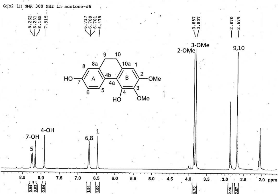
Figure 74 1 H-NMR (300 MHz) spectrum of compound DG3
