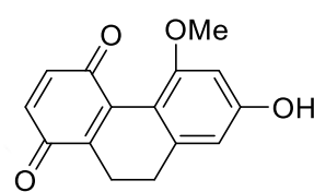
5-Methoxy-7-hydroxy-9,10-dihydro- 1,4-phenanthrenequinone [12]
