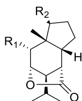
[192] Dendromonilide B, R_1 = \text{OGlc} , R_2 = \text{COOH}
