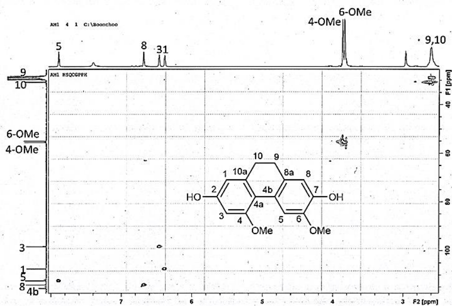
Figure 150 ^{13}\text{C} -NMR (75 MHz) spectrum of compound AMF5
