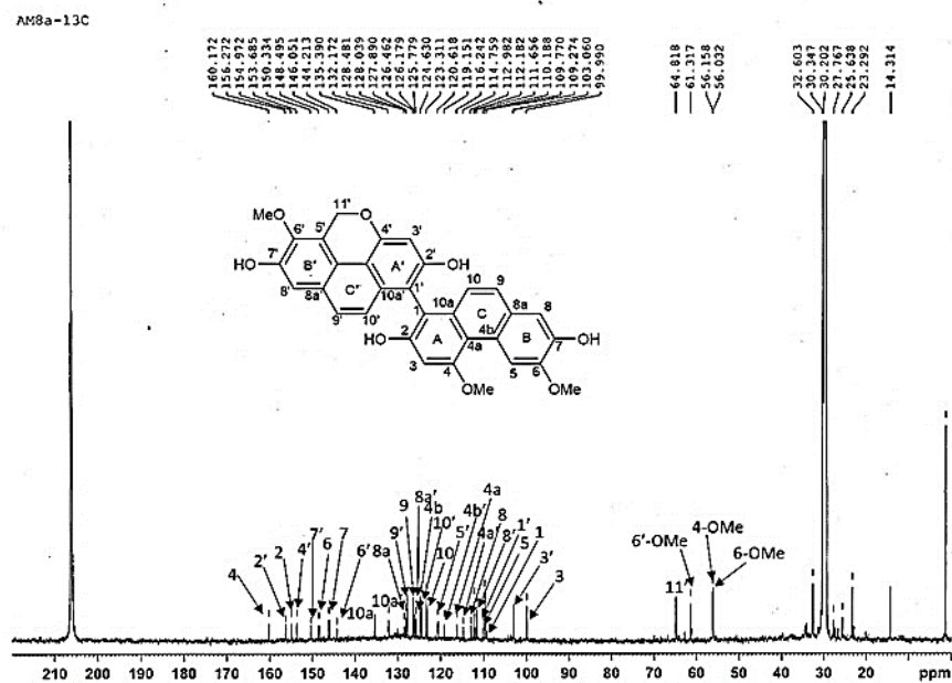
Figure 128 ^{13}\text{C} -NMR (125 MHz) spectrum of compound AMF2
