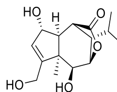
[190] Crystallinin
