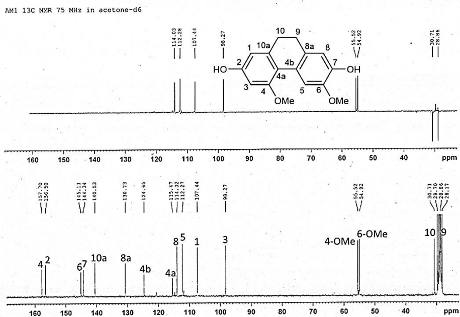
Figure 150 ^{13}\text{C} -NMR (75 MHz) spectrum of compound AMF5
