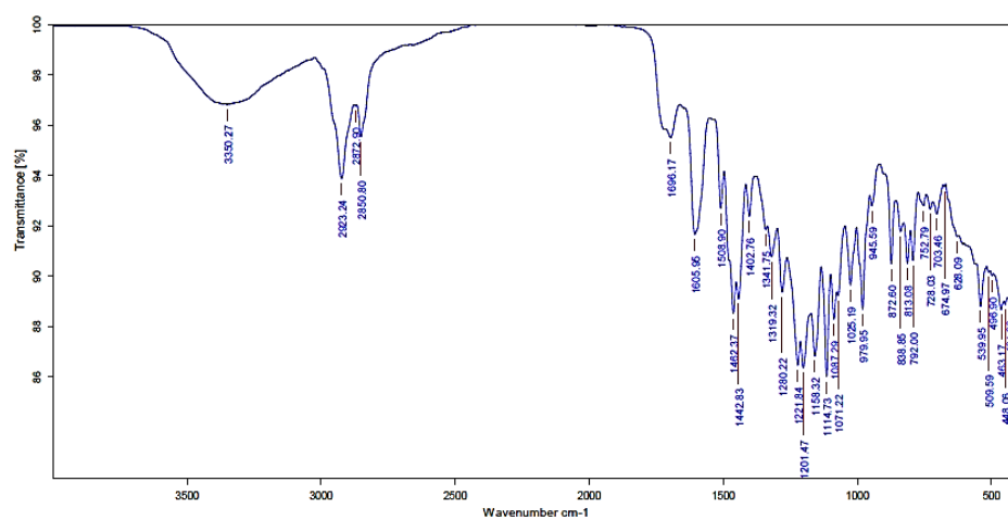
Figure 117 FT-IR spectrum of compound AMF1
