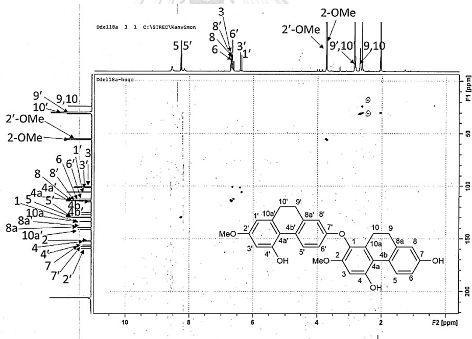
Figure 46 ^{13}\text{C} -NMR (125 MHz) spectrum of compound DD10
