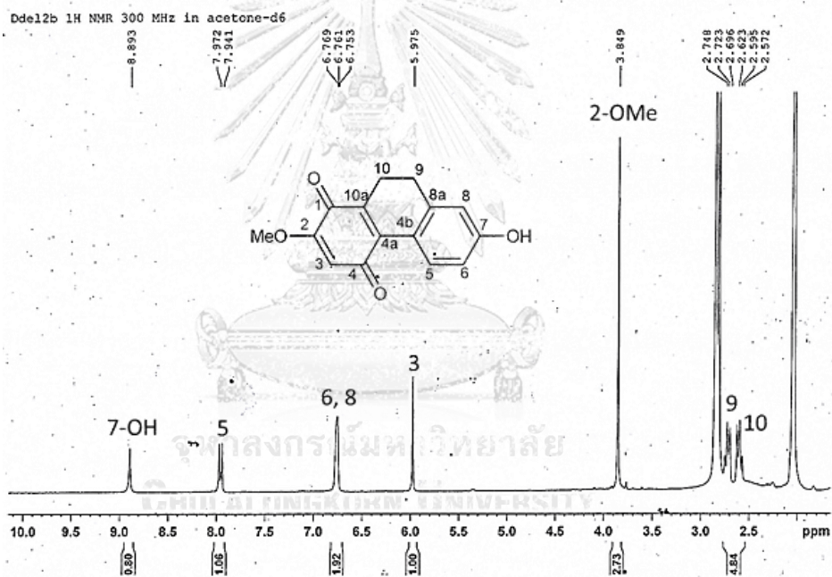
Figure 13 ^1\text{H-NMR} (300 MHz) spectrum of compound DD2
