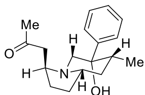
[317] Crepidatumine C
