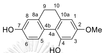
lusianthridin [97]
