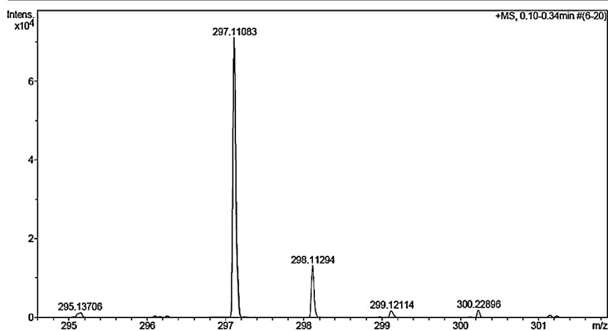
Figure 91 Mass spectrum of compound DG6
