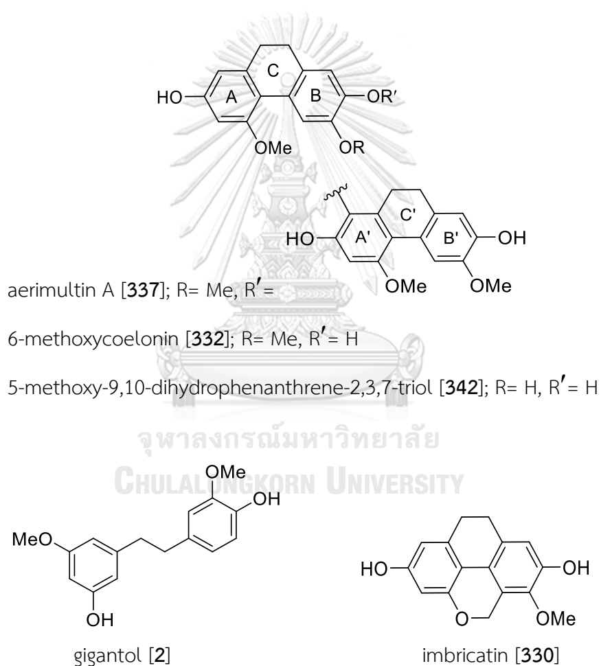
Figure 114 Structures of compounds isolated from Aerides multiflora
