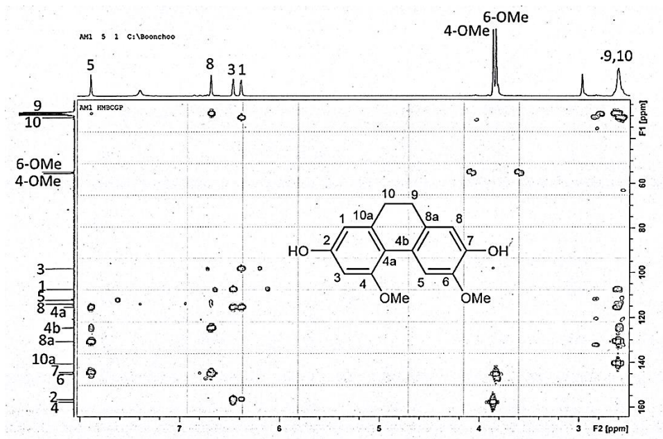
Figure 152 HMBC spectrum of compound AMF5
