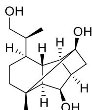
[221] Dendrowardol C
