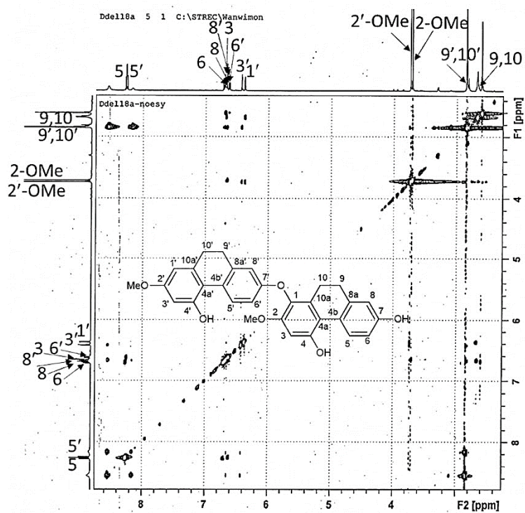
Figure 45 NOESY spectrum of compound DD10
