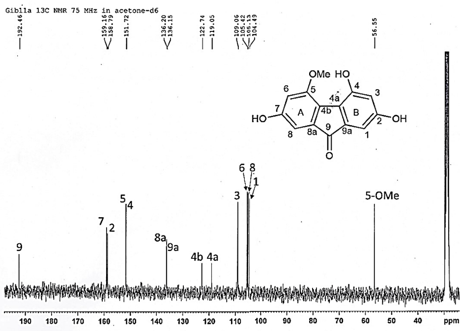
Figure 104 ^{13}\text{C} -NMR (75 MHz) spectrum of compound DG8
