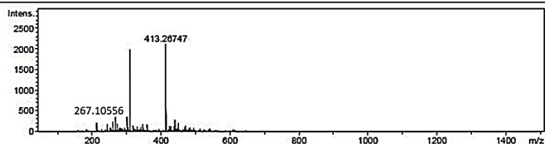
Figure 31 Mass spectrum of compound DD7
