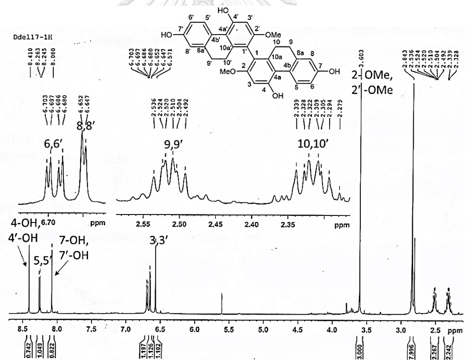
Figure 38 ^1\text{H-NMR} (300 MHz) spectrum of compound DD9
