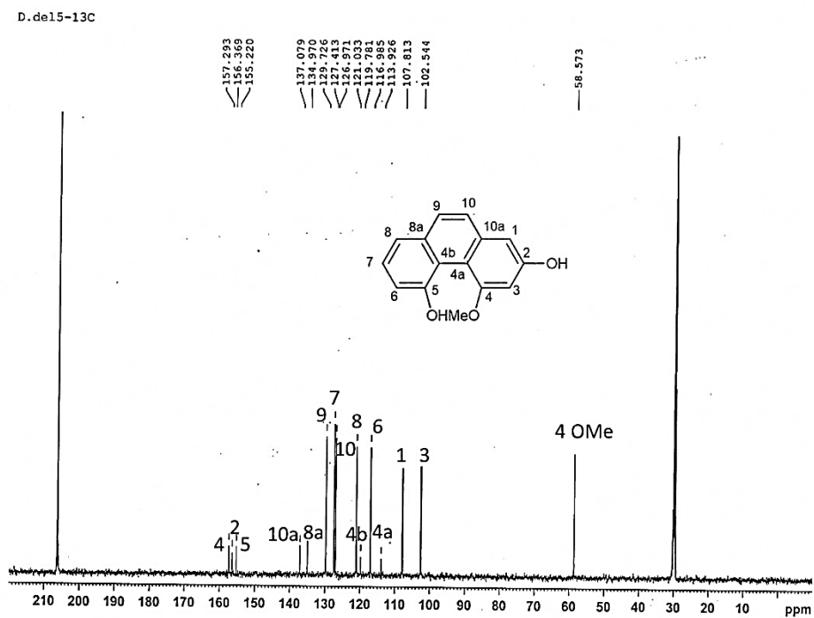
Figure 22 ^{13}\text{C} -NMR (125 MHz) spectrum of compound DD4
