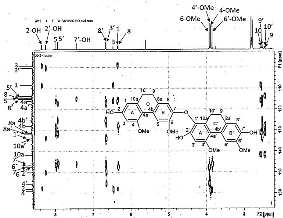
Figure 120 HSQC spectrum of compound AMF1
