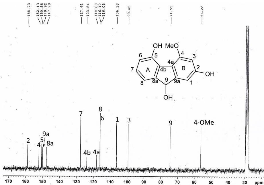
Figure 110 ^{13}\text{C} -NMR (75 MHz) spectrum of compound DG9
