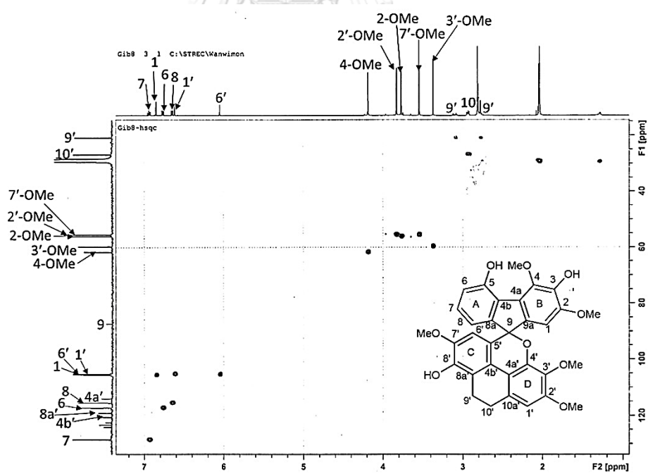
Figure 69 HSQC spectrum of compound DG2
