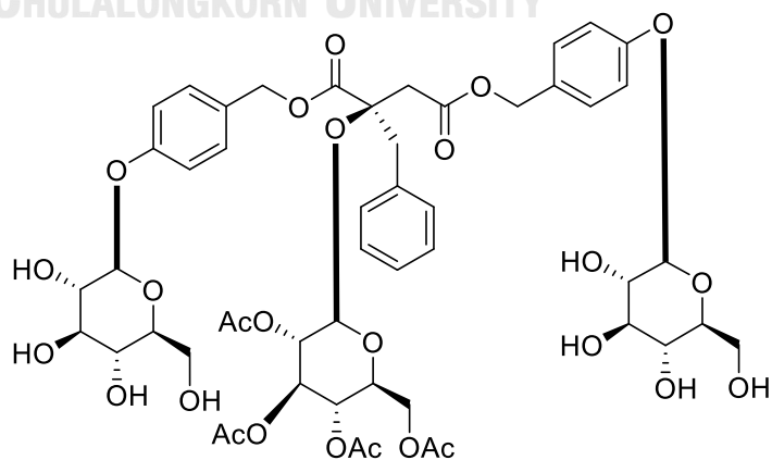
Arundinoside D [19]
