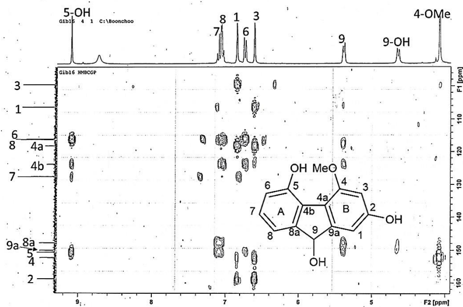
Figure 112 HMBC spectrum of compound DG9
