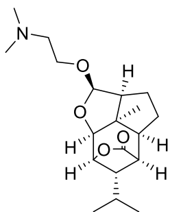
[233] Wardianumine A
