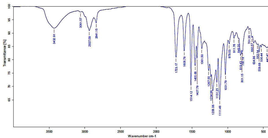
Figure 142 FT-IR spectrum of compound AMF4
