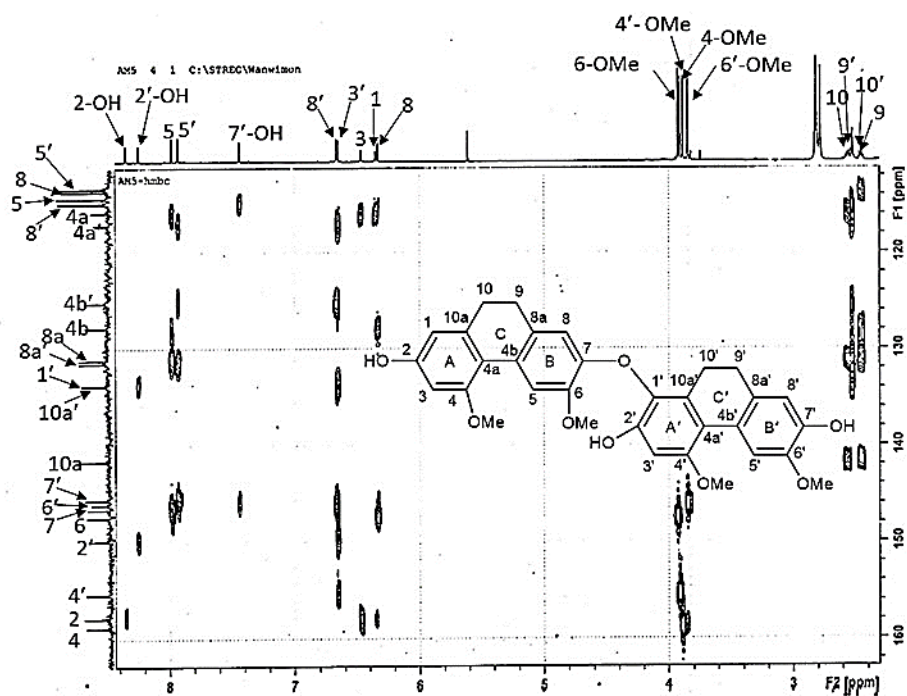
Figure 122 HMBC (expanded) spectrum of compound AMF1
