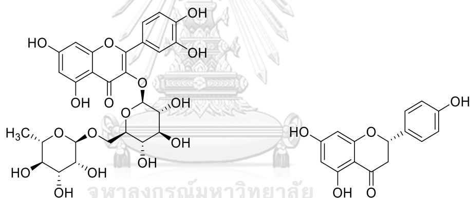
Rutin [13]
