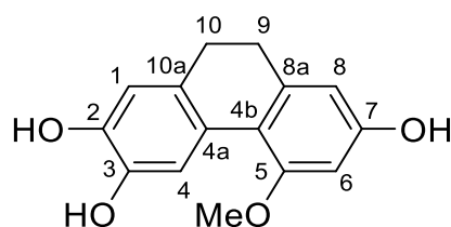
5-methoxy-9,10-dihydrophenanthrene-2,3,7-triol [342]
