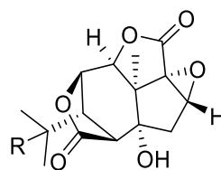
[225] \alpha -Dihydropicrotoxinin: R = H
