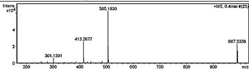
Figure 37 Mass spectrum of compound DD9
