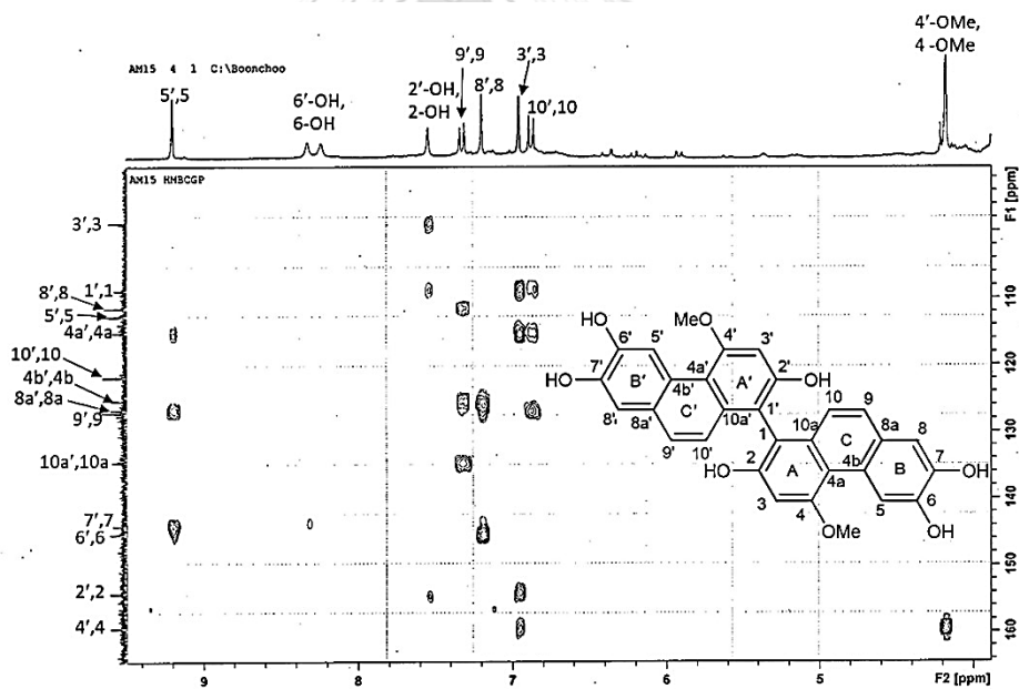
Figure 137 HSQC spectrum of compound AMF3
