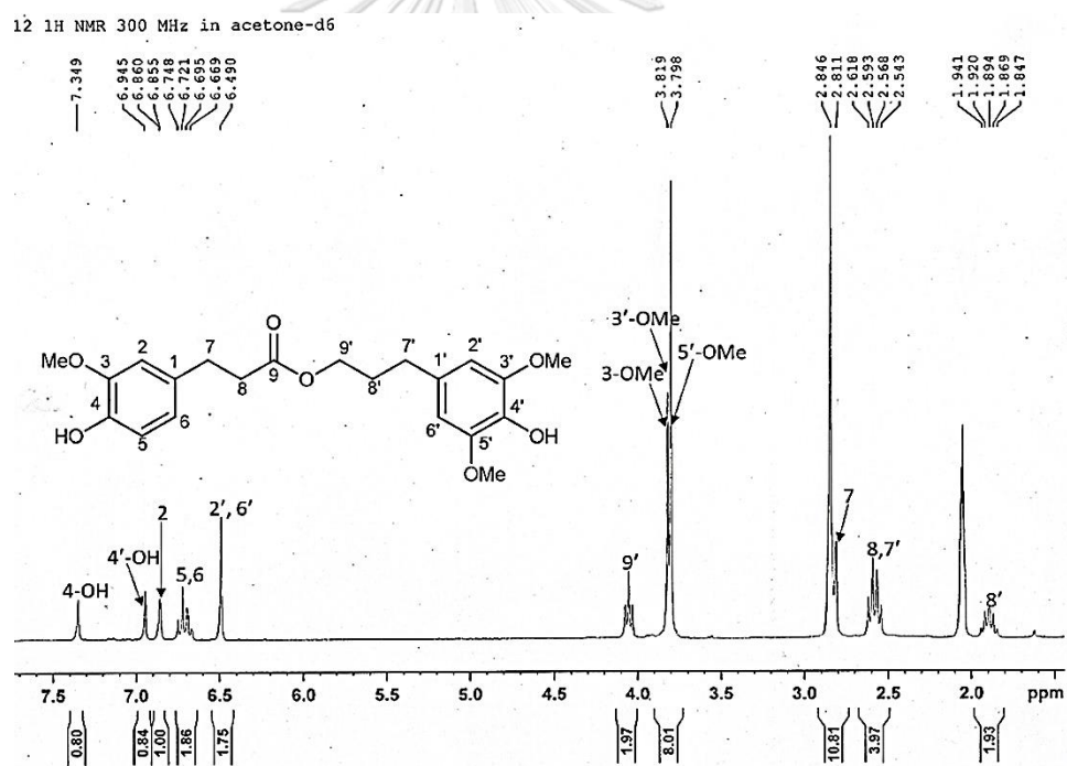
Figure 143 1 H-NMR (300 MHz) spectrum of compound AMF4
