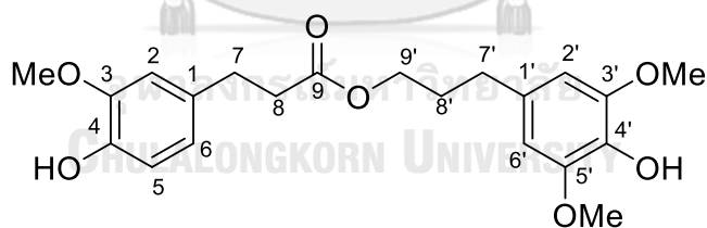
dihydrosinapyl dihydroferulate [340]
