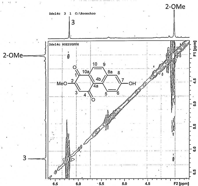
Figure 19 NOESY spectrum of compound DD3
