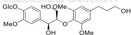
[301] Erythro-1-(4-O- \beta -D-glucopyranosyl-3-methoxyphenyl)-2-[4-(3-hydroxypropyl)-2,6-dimethoxyphenoxy]-1,3-propanediol
