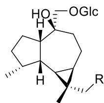
[214] Dendroside C; R = OH
