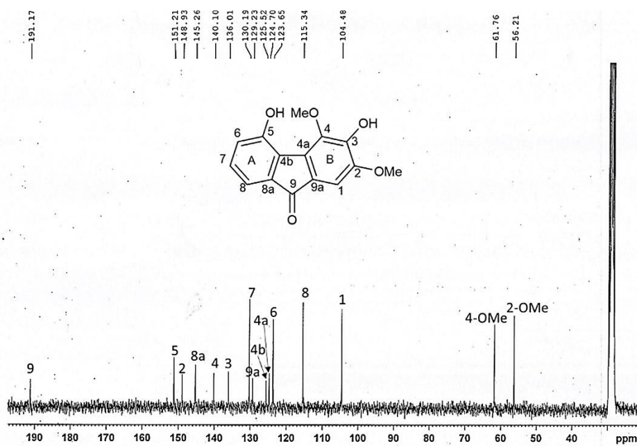
Figure 81 ^{13}\text{C-NMR} (75 MHz) spectrum of compound DG4
