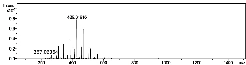
Figure 108 Mass spectrum of compound DG9
