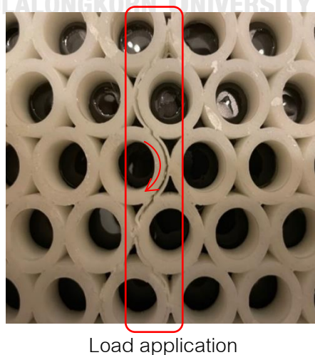
Figure 35 Enlarged picture of core failure morphology of circular core.
