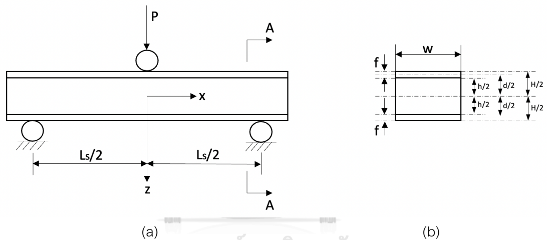
Figure 2 (a) Three-point bending and (b) Cross section A-A
