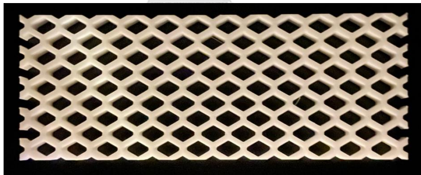
Figure 6 Printed hexagonal honeycomb core at relative density of 0.5
