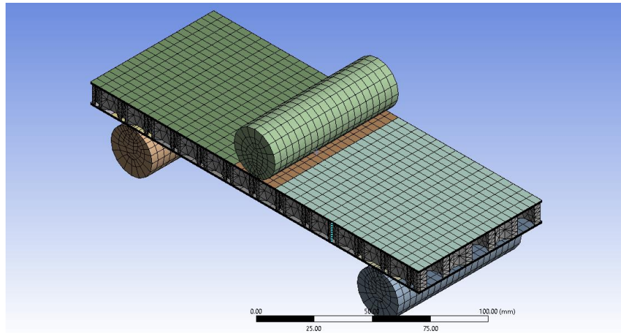
Figure 24 The meshing of the sandwich honeycomb structure.
