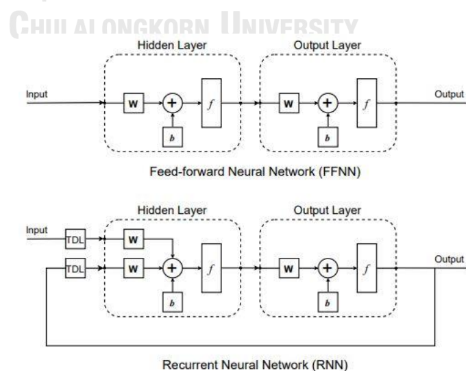
Figure 5 Feed forward and recurrent neural network structures[28]
