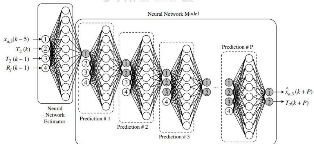
Figure 6 Feedforward neural network in NN MPC with neural network estimator [30]
