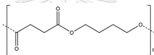
Figure 2 The molecular structure of polybutylene succinate (PBS) [17]
